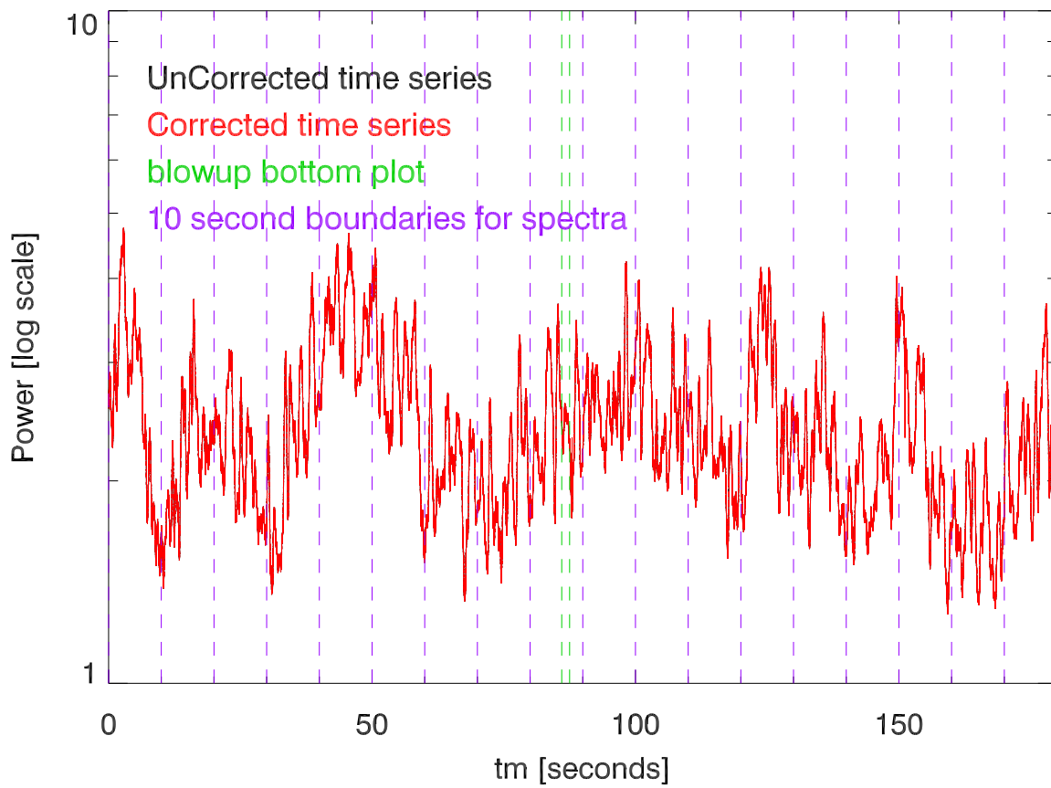
190903 327 B1005+077. PoIA TotPwr vs time on Source.
