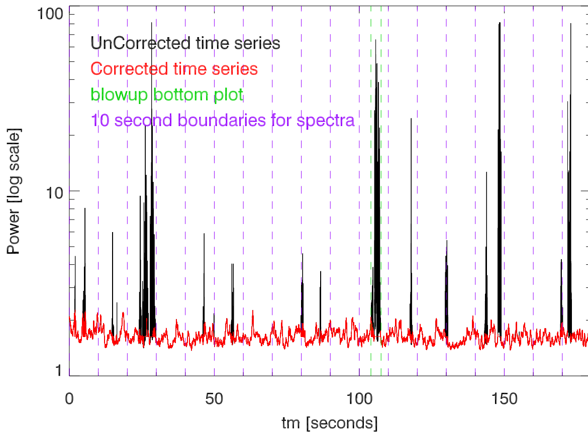
190819 327 B1040+123. PoIA TotPwr vs time on Source.
