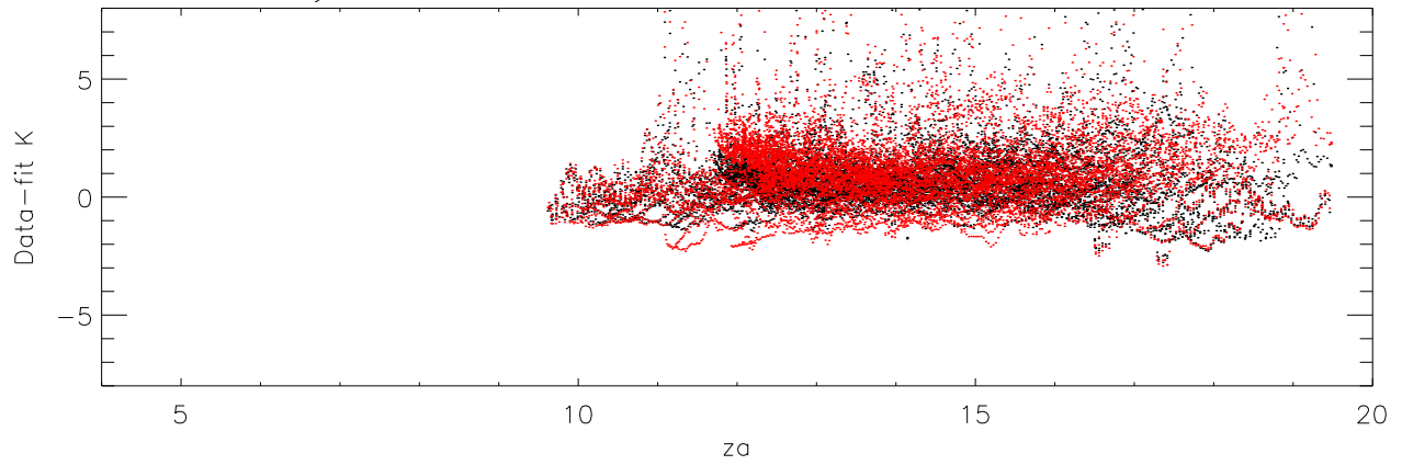
Tsys - fit for fieldField_D medDifA: -0.92 medDifB: 0.25
