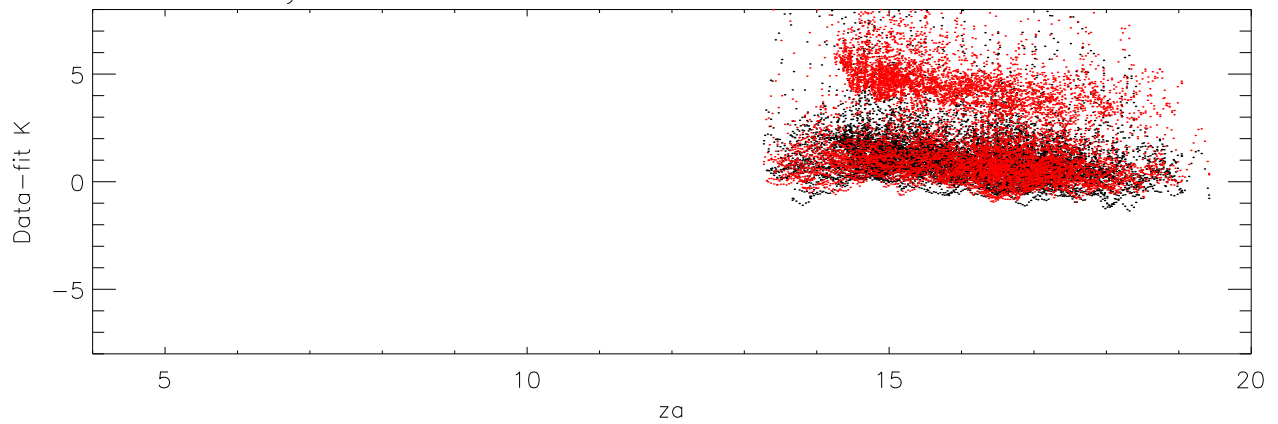
Tsys - fit for fieldField_C medDifA: 0.60 medDifB: 0.95
