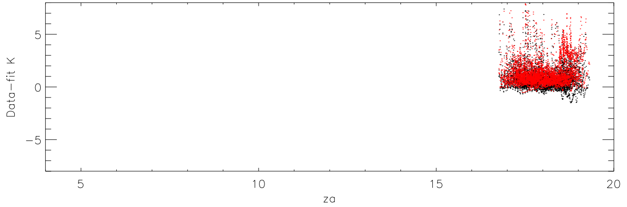
Tsys - fit for fieldField_B medDifA: 0.96 medDifB: 1.76
