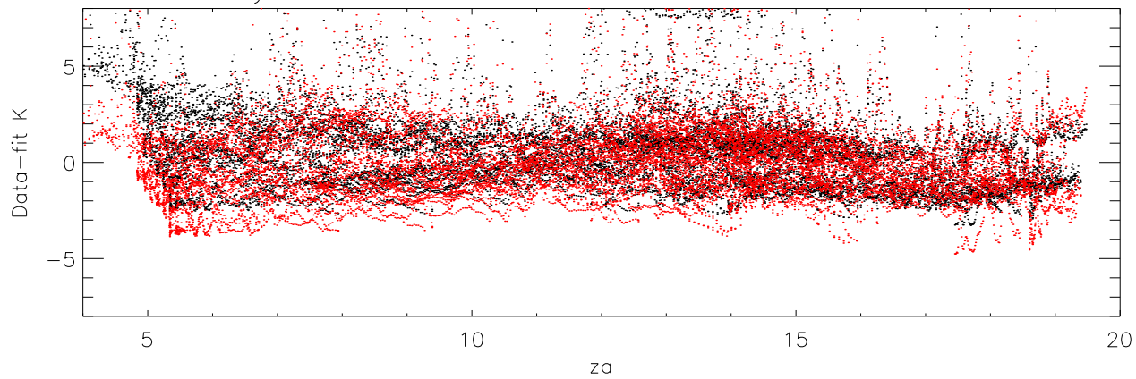
Tsys - fit for fieldField_M medDifA:-1.73 medDifB:-2.35
