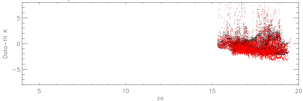
Tsys - fit for fieldField_J medDifA:-0.04 medDifB: 0.20
