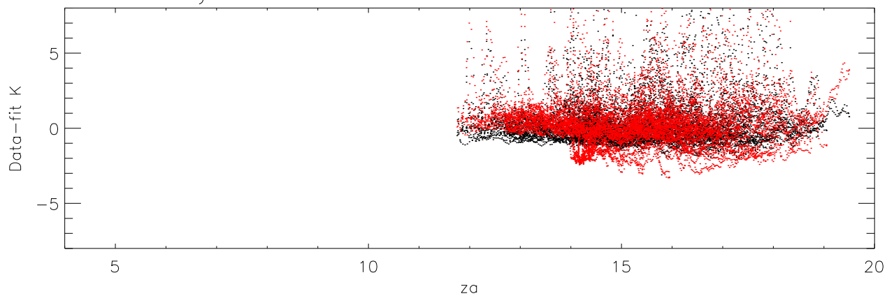
Tsys - fit for fieldField_L medDifA: 0.49 medDifB:-0.02
