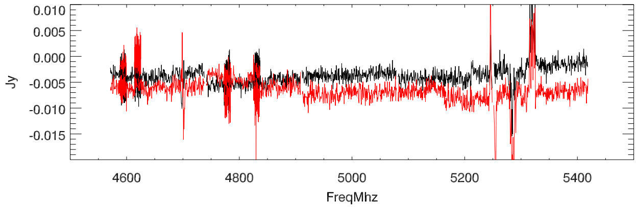
(on/off - 1) :G202.39+2.52 date:20101112 fNum:03200 patNum: 8 smo:51
