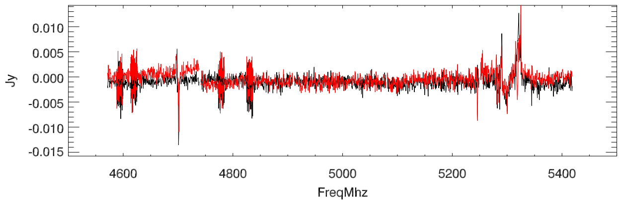
(on/off - 1) :G201.75+0.51 date:20101112 fNum:04400 patNum:11 smo:51
