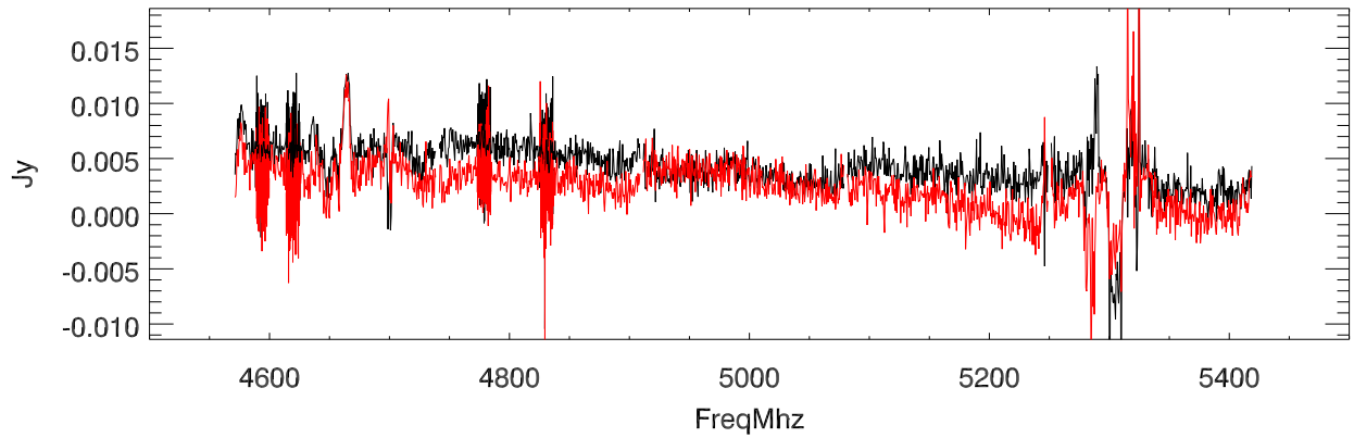
(on/off - 1) :G207.26-1.81 date:20101112 fNum:04000 patNum:10 smo:51
