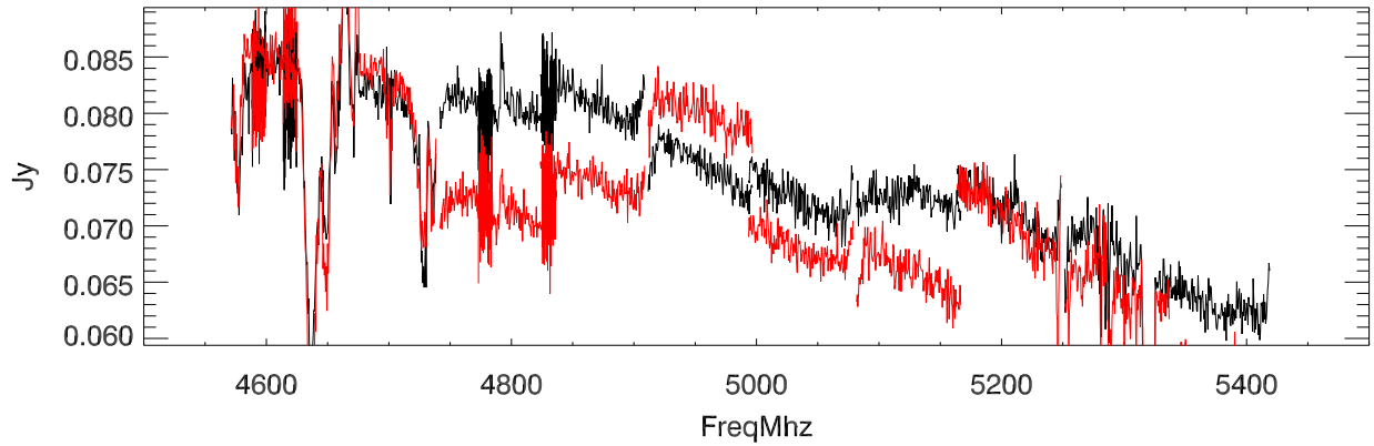
(on/off - 1) :G206.60-1.87 date:20101112 fNum:03600 patNum: 9 smo:51
