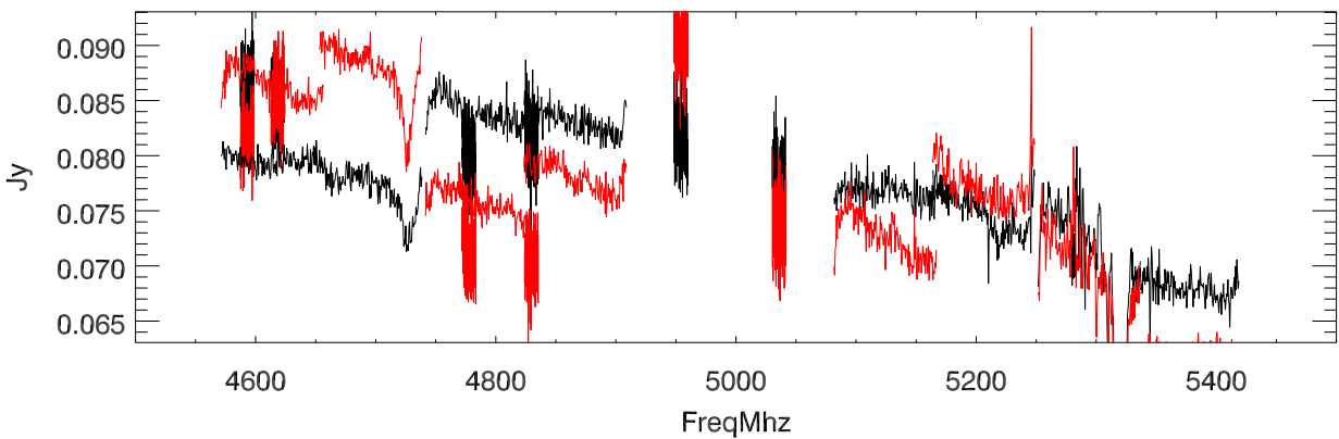
(on/off - 1) :G206.77-1.94 date:20101110 fNum:05800 patNum:12 smo:51
