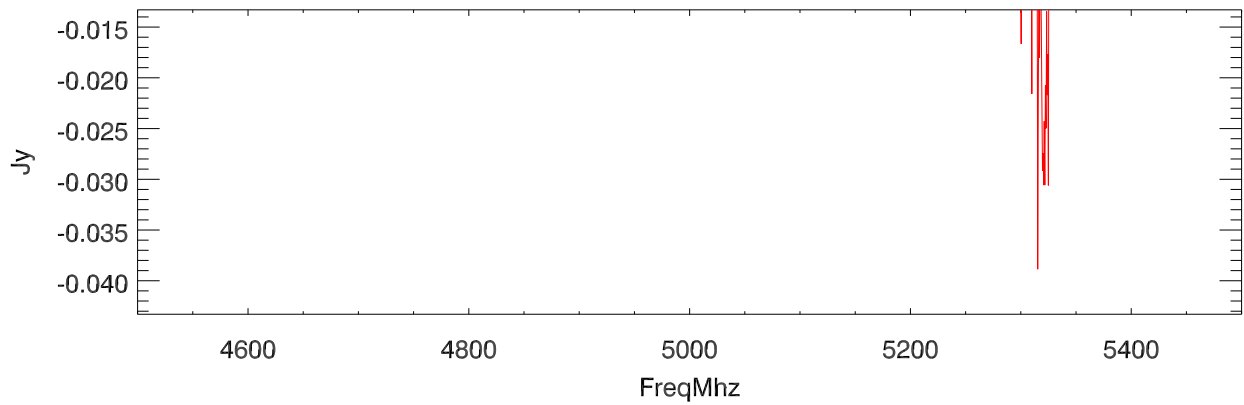
(on/off - 1) :G180.87+4.06 date:20101110 fNum:05000 patNum:10 smo:51
