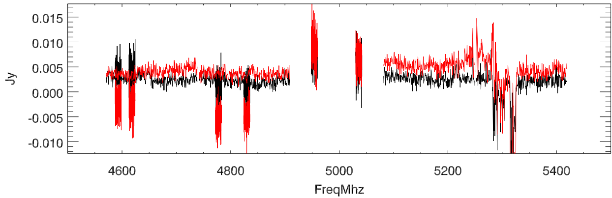
(on/off - 1) :G203.79+2.10 date:20101110 fNum:05400 patNum:11 smo:51
