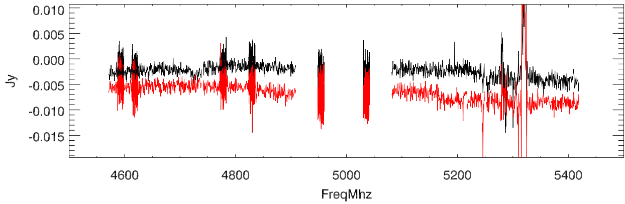
(on/off - 1) :G180.83+4.00 date:20101110 fNum:04600 patNum: 9 smo:51
