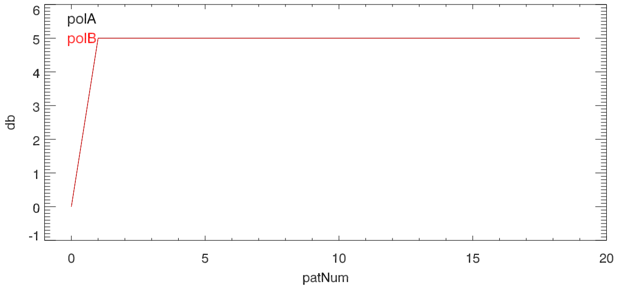
20110222 Rf attn vs pattern num
