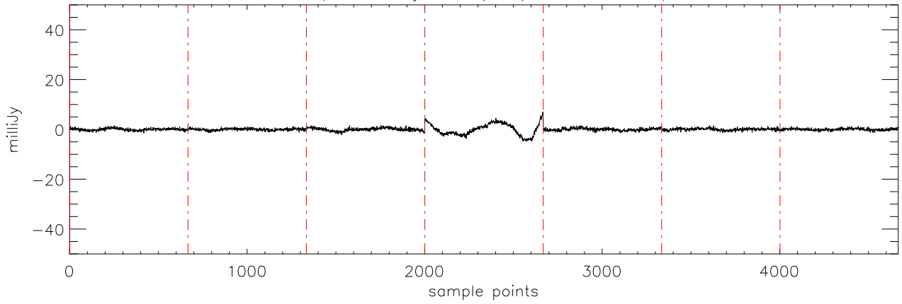
a2471 epsTau 08jan10 (AST) StokesU freq:4750.
