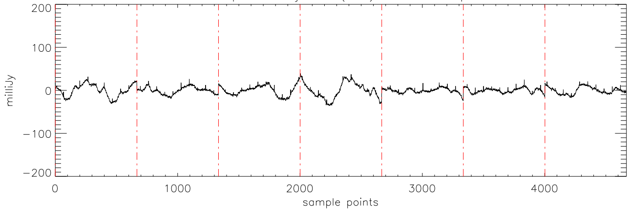
a2471 epsTau 08jan10 (AST) StokesI freq:5176.
