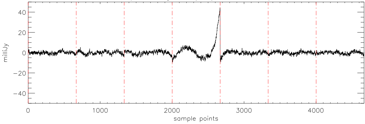
a2471 epsTau 08jan10 (AST) StokesQ freq:5176.
