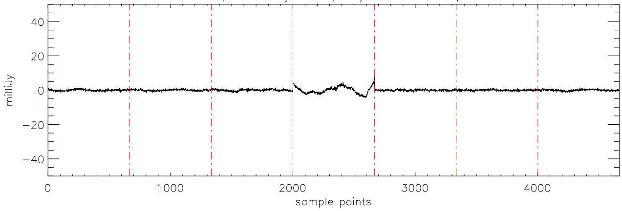
a2471 epsTau 08jan10 (AST) StokesU freq:4608.
