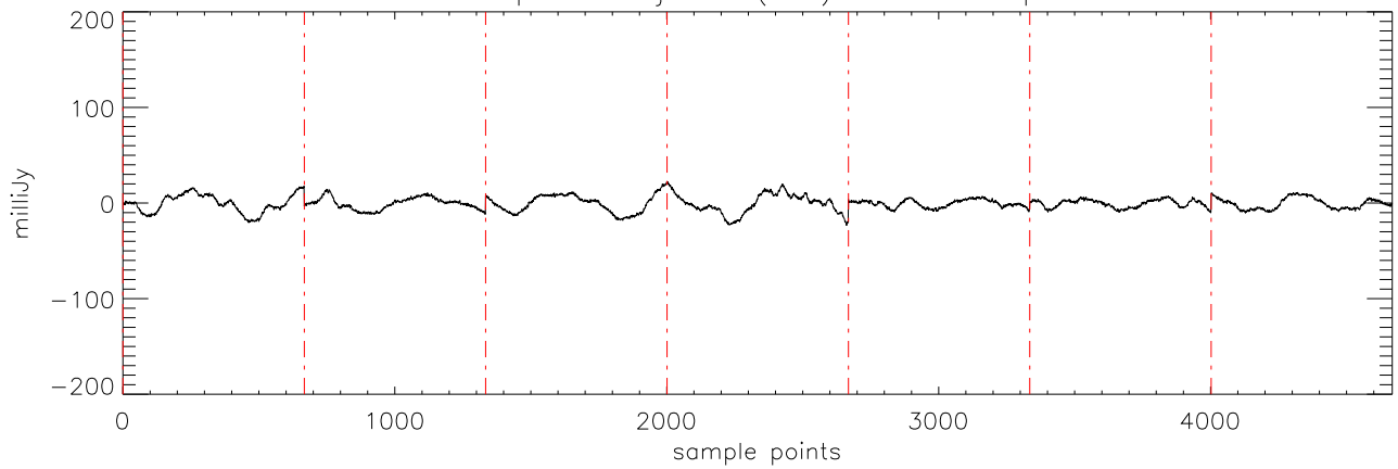
a2471 epsTau 08jan10 (AST) StokesI freq:4608.
