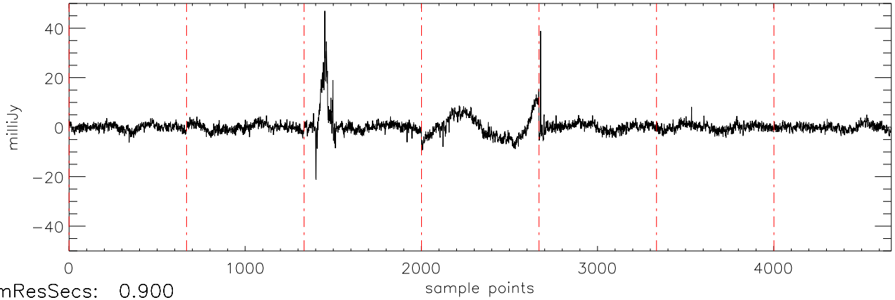
a2471 epsTau 08jan10 (AST) StokesQ freq:4466.
