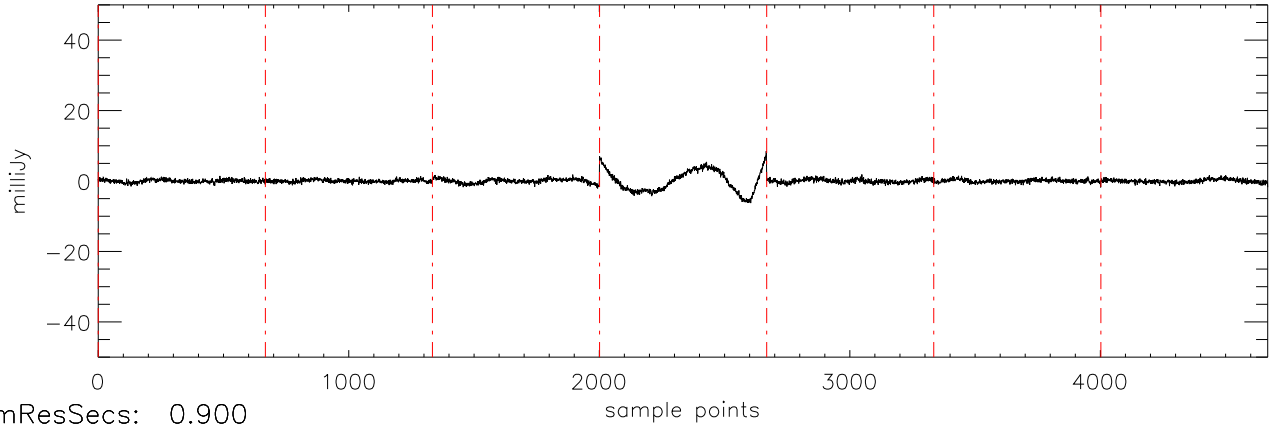
a2471 epsTau 08jan10 (AST) StokesU freq:5034.
