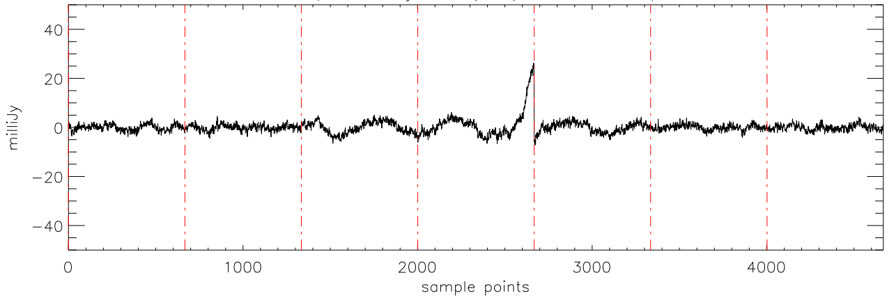
a2471 epsTau 08jan10 (AST) StokesQ freq:4750.
