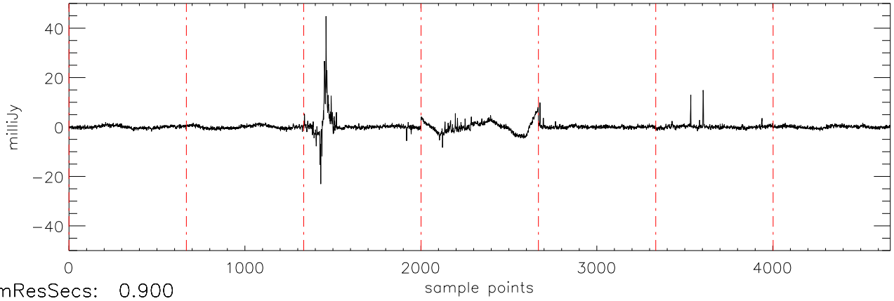
a2471 epsTau 08jan10 (AST) StokesU freq:4466.
