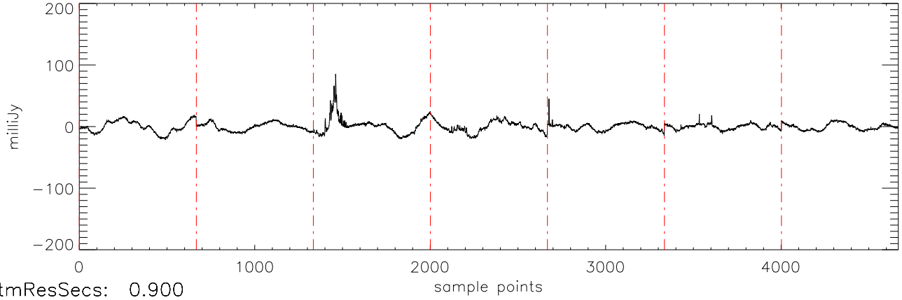
a2471 epsTau 08jan10 (AST) StokesI freq:4466.
