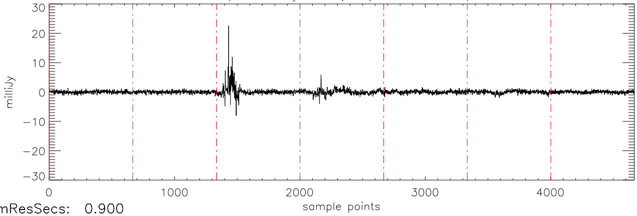
a2471 epsTau 08jan10 (AST) StokesV freq:4466.
