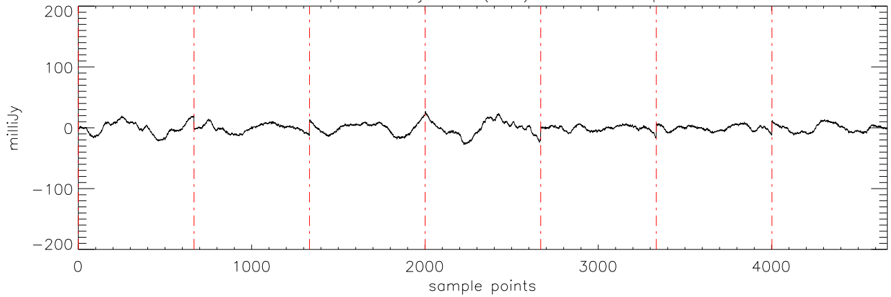
a2471 epsTau 08jan10 (AST) StokesI freq:4750.
