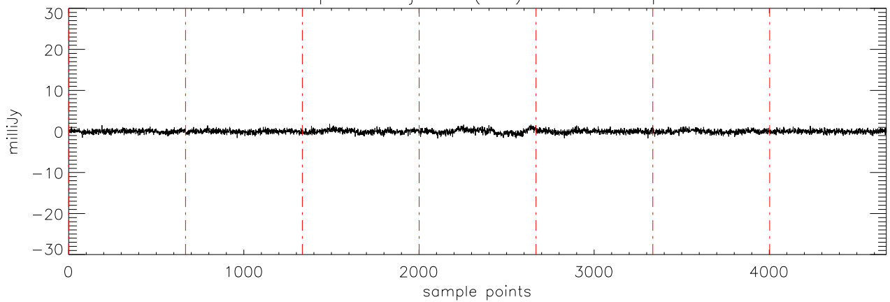
a2471 epsTau 08jan10 (AST) StokesV freq:4750.
