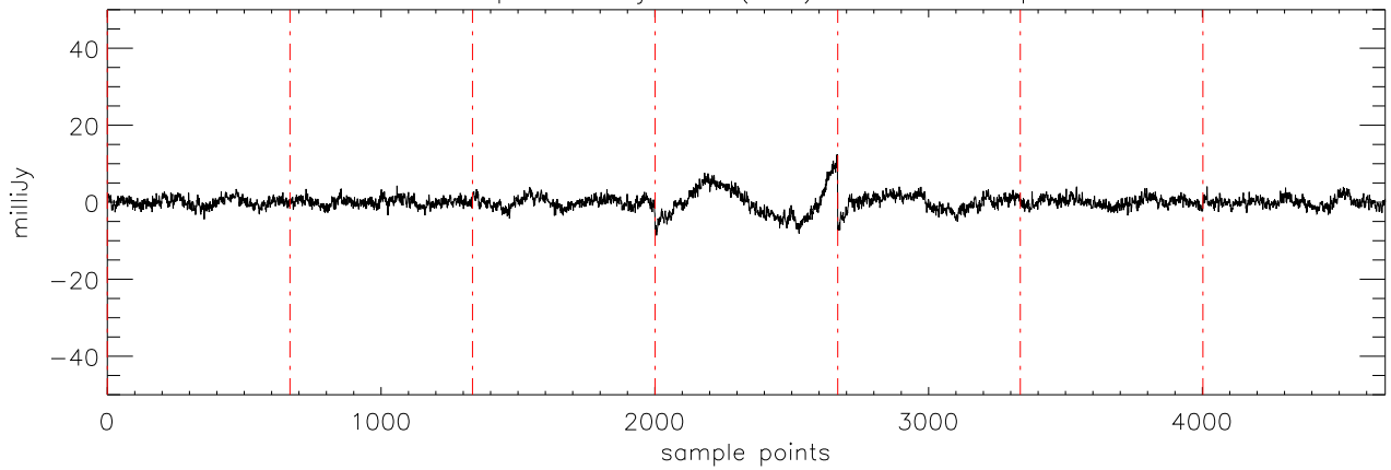
a2471 epsTau 08jan10 (AST) StokesQ freq:4608.
