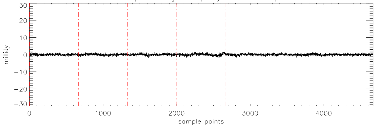
a2471 epsTau 08jan10 (AST) StokesV freq:5176.
