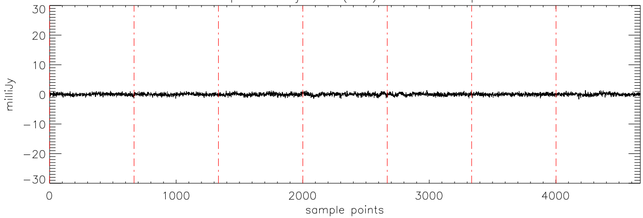
a2471 epsTau 08jan10 (AST) StokesV freq:4608.
