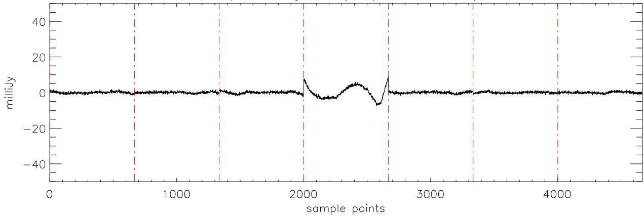
a2471 epsTau 08jan10 (AST) StokesU freq:5176.
