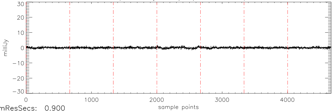
a2471 epsTau 08jan10 (AST) StokesV freq:5034.
