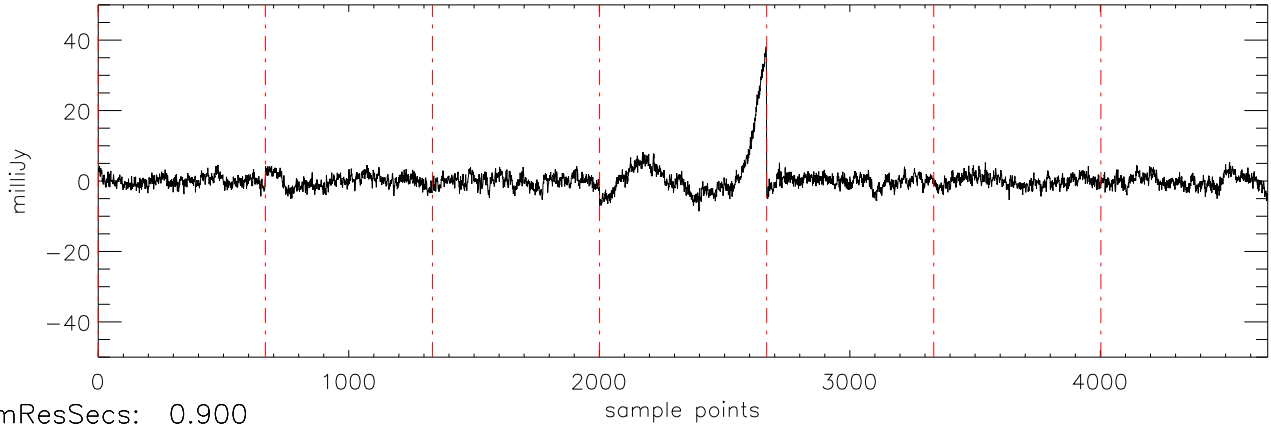
a2471 epsTau 08jan10 (AST) StokesQ freq:5034.
