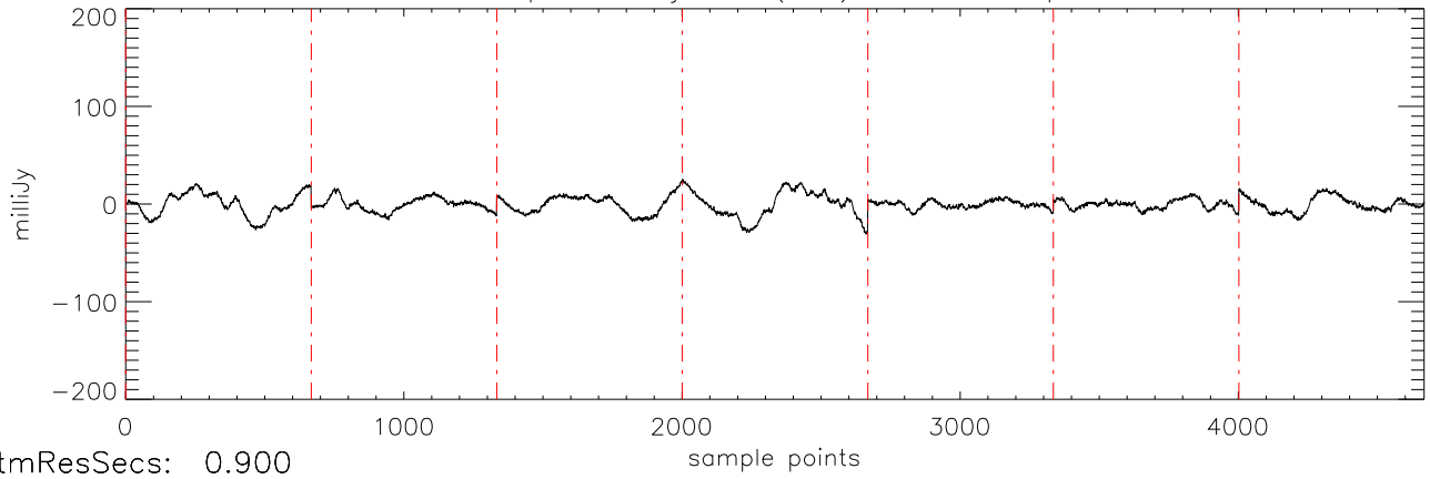
a2471 epsTau 08jan10 (AST) StokesI freq:5034.
