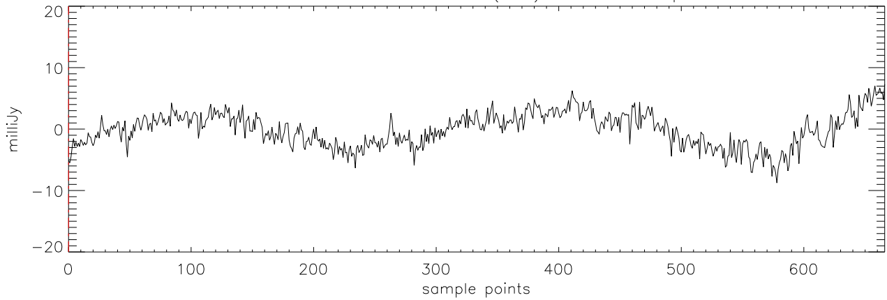
a2471 TVLM-513 11mar12 (AST) StokesQ freq:4750.
