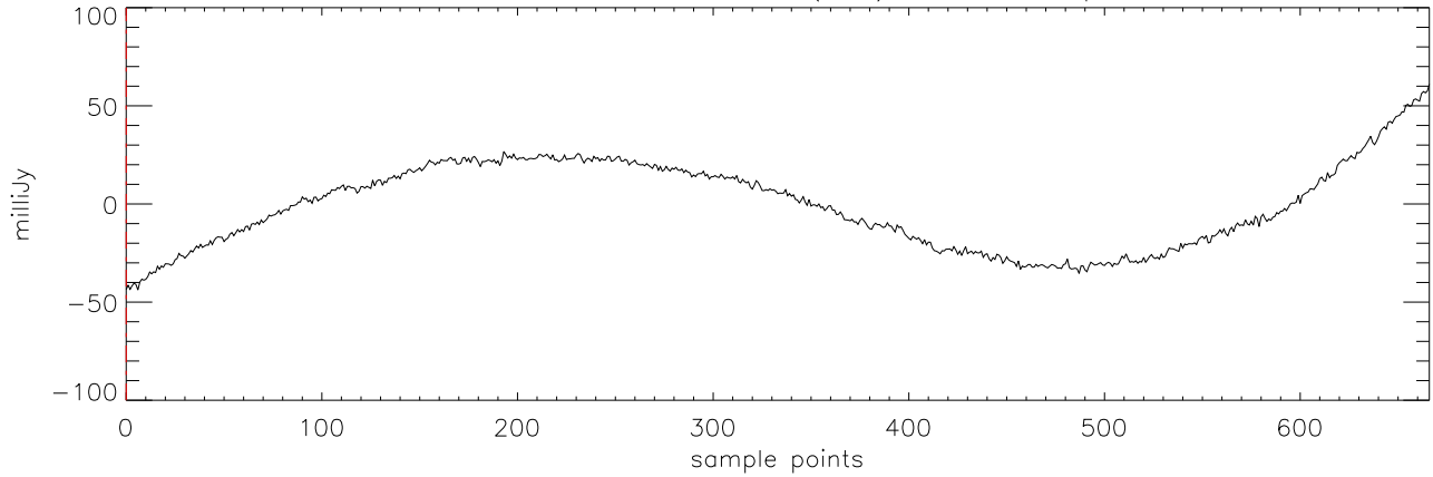
a2471 TVLM-513 11mar12 (AST) StokesI freq:4750.
