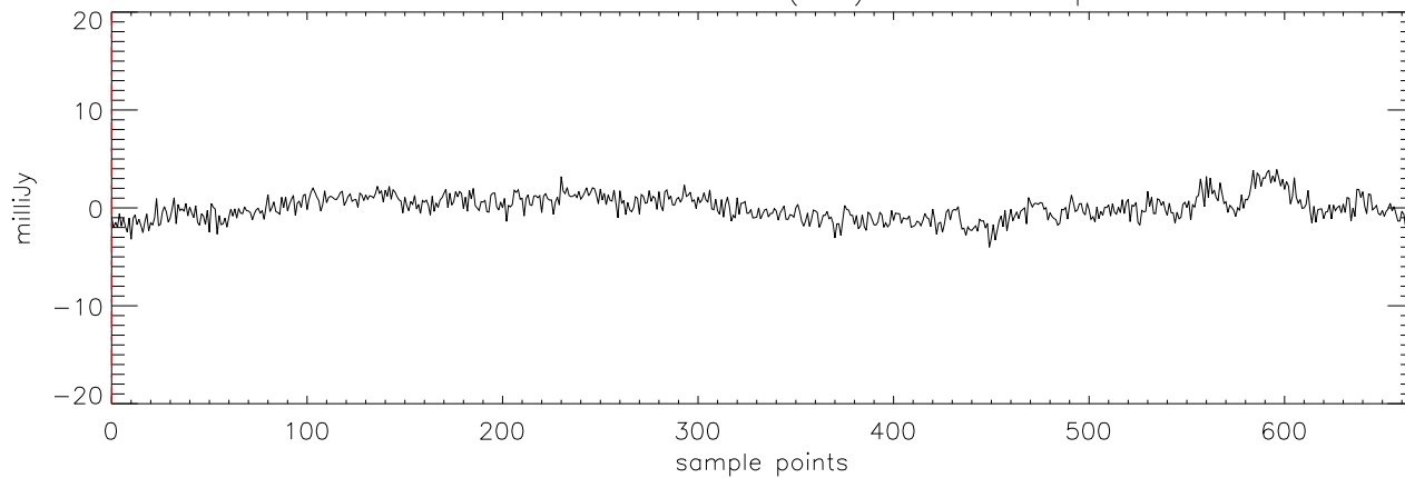
a2471 TVLM-513 11mar12 (AST) StokesU freq:5176.
