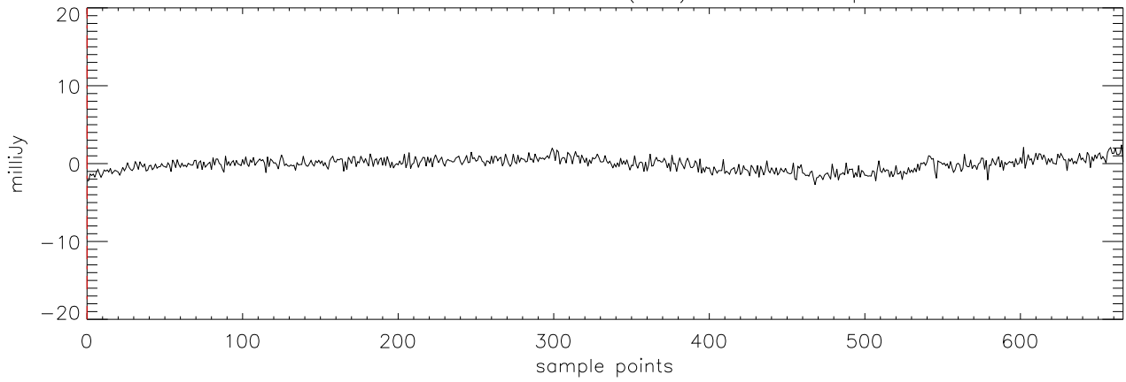
a2471 TVLM-513 11mar12 (AST) StokesV freq:4750.
