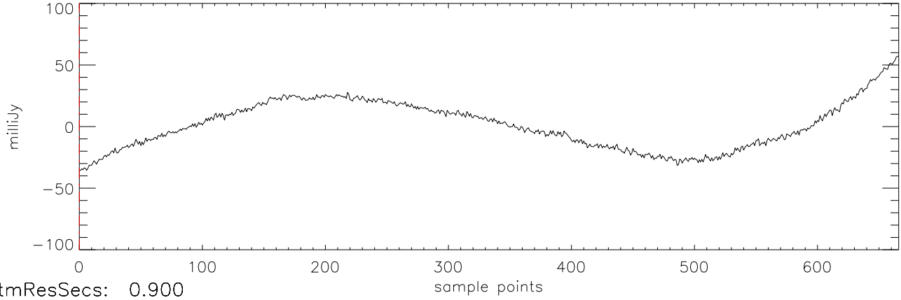
a2471 TVLM-513 11mar12 (AST) StokesI freq:4466.
