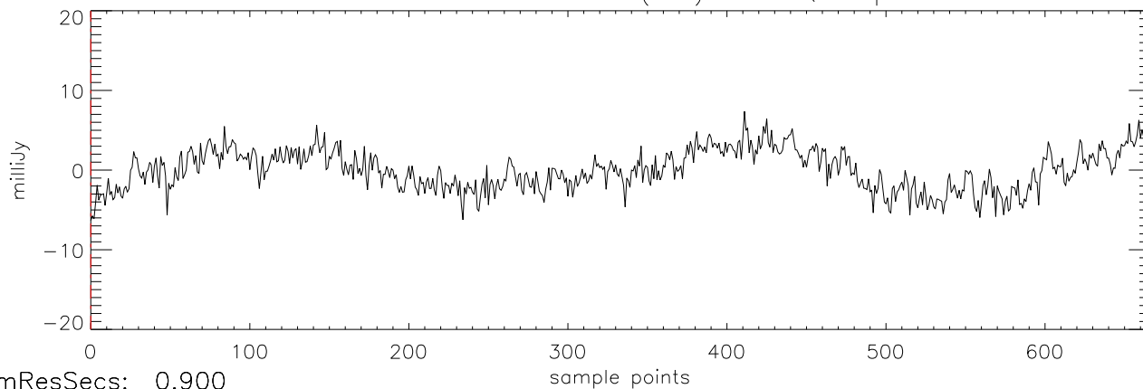
a2471 TVLM-513 11mar12 (AST) StokesQ freq:5034.
