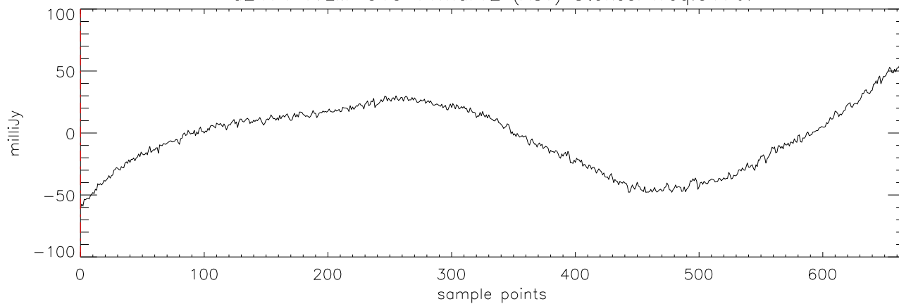
a2471 TVLM-513 11mar12 (AST) StokesI freq:5176.
