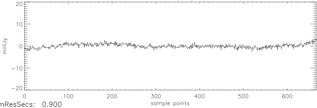
a2471 TVLM-513 11mar12 (AST) StokesV freq:5034.
