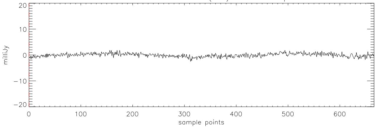
a2471 TVLM-513 11mar12 (AST) StokesV freq:4608.
