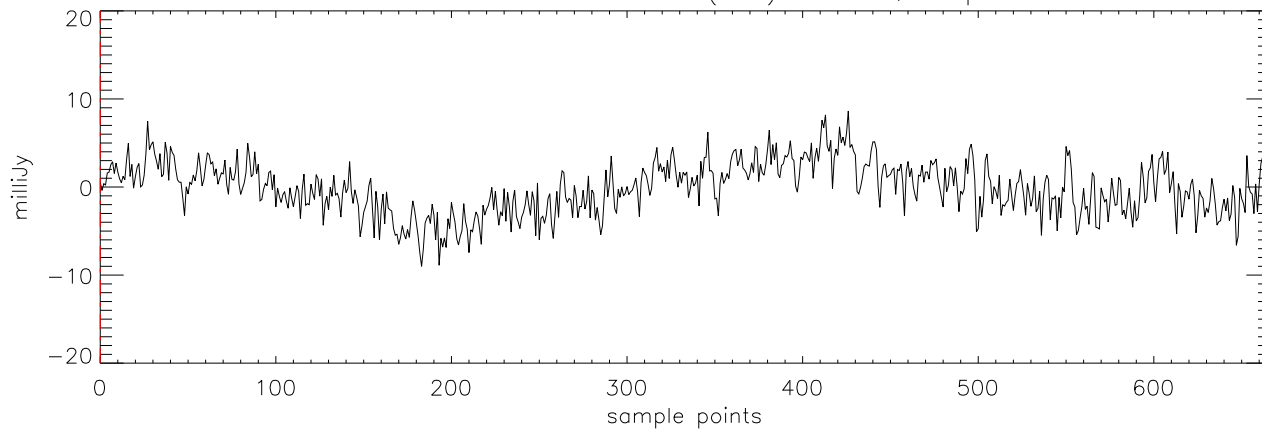
a2471 TVLM-513 11mar12 (AST) StokesQ freq:5176.
