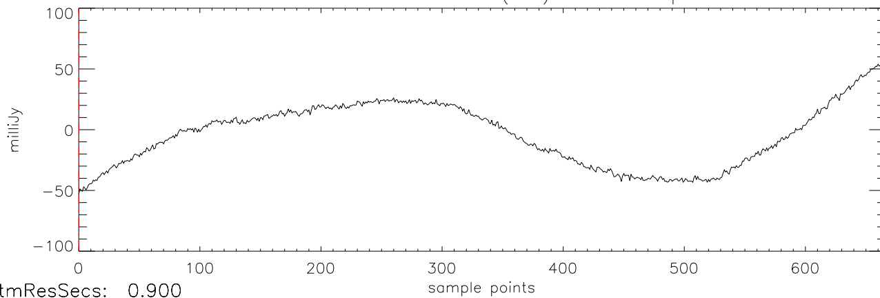
a2471 TVLM-513 11mar12 (AST) StokesI freq:5034.
