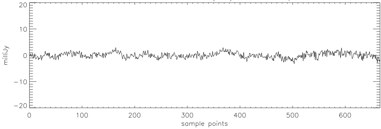
a2471 TVLM-513 11mar12 (AST) StokesV freq:5176.
