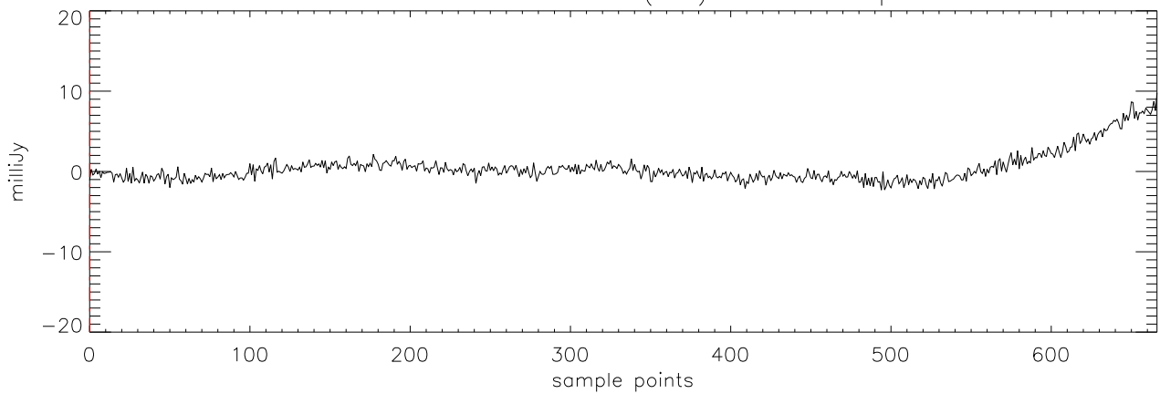
a2471 TVLM-513 11mar12 (AST) StokesU freq:4750.
