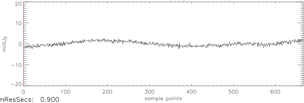
a2471 TVLM-513 11mar12 (AST) StokesV freq:4466.
