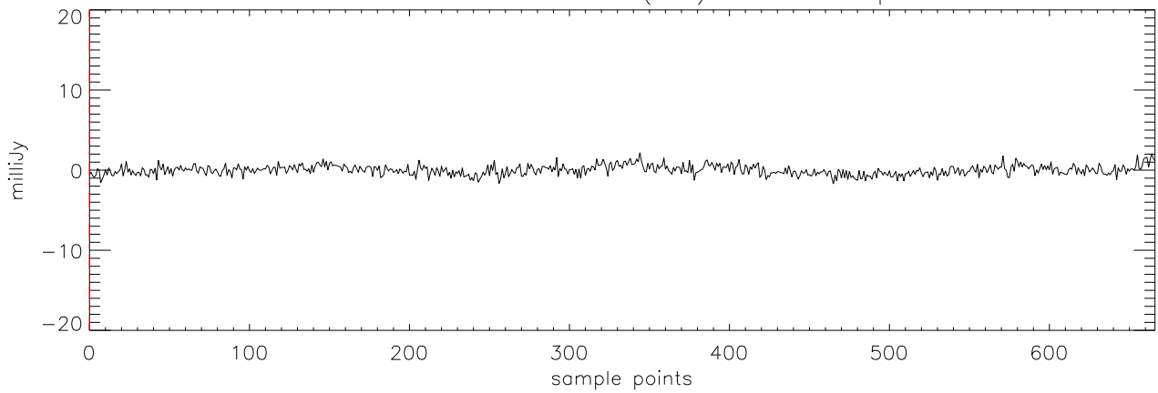
a2471 TVLM-513 11mar12 (AST) StokesU freq:4608.
