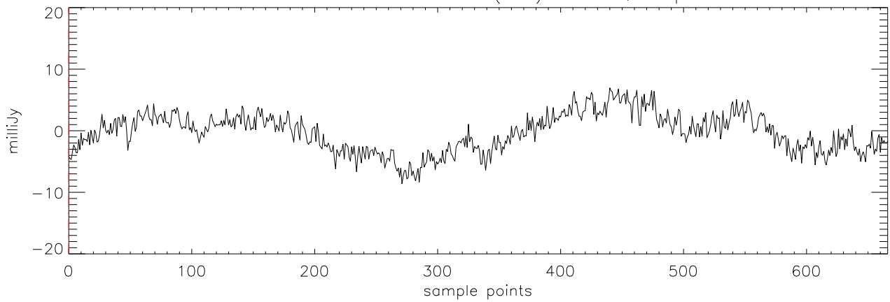
a2471 TVLM-513 11mar12 (AST) StokesQ freq:4608.
