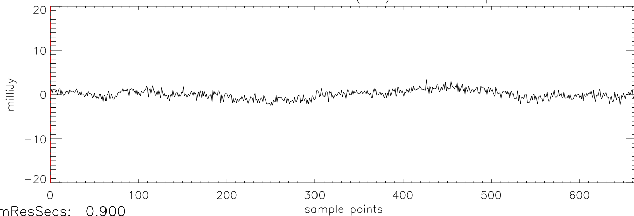
a2471 TVLM-513 11mar12 (AST) StokesU freq:5034.
