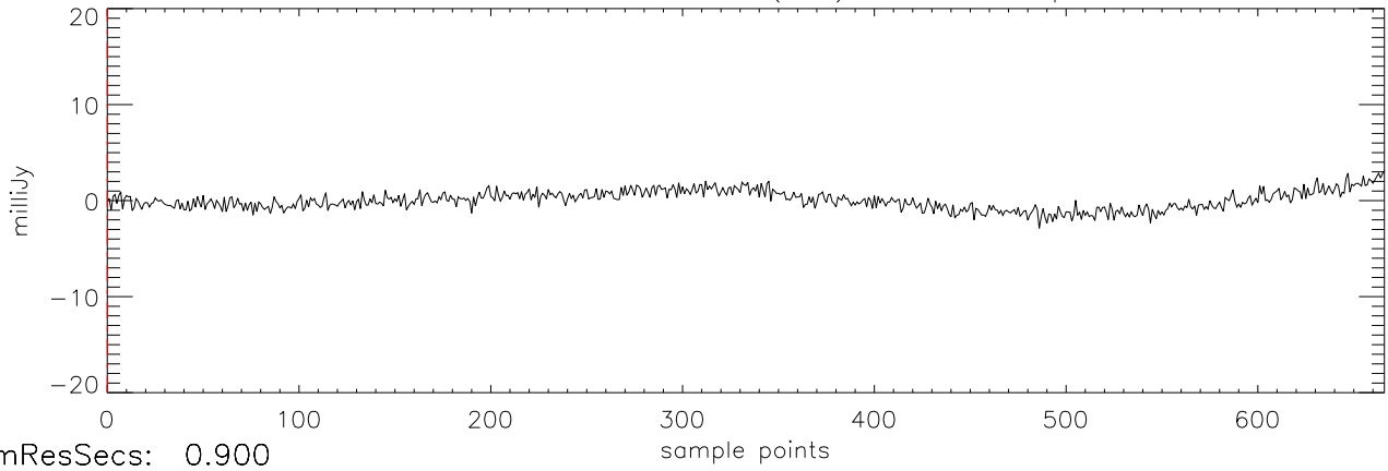
a2471 TVLM-513 11mar12 (AST) StokesU freq:4466.
