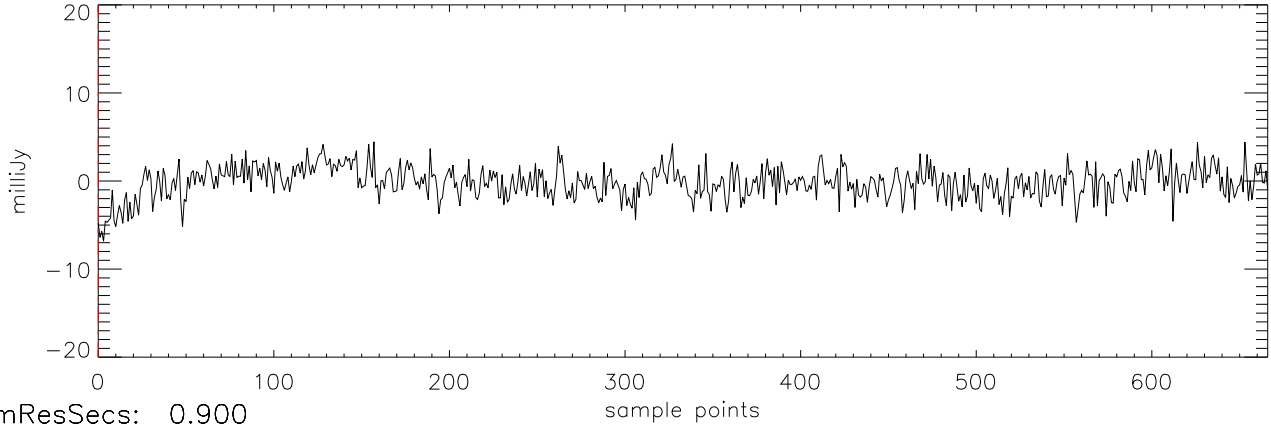
a2471 TVLM-513 11mar12 (AST) StokesQ freq:4466.
