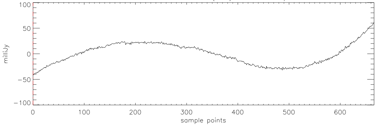
a2471 TVLM-513 11mar12 (AST) StokesI freq:4608.
