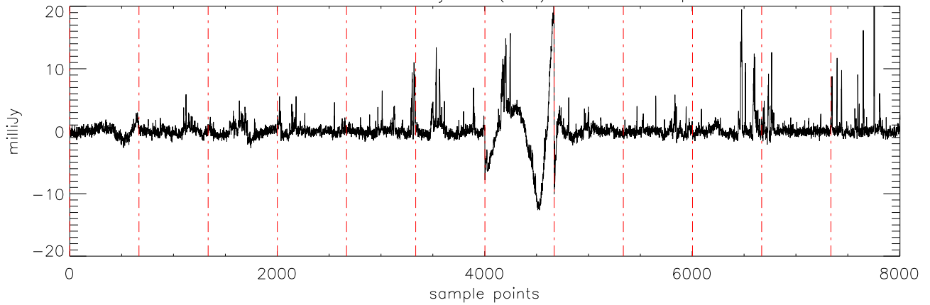
a2471 J21011544 19jul11 (AST) StokesU freq:4608.
