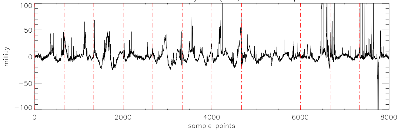
a2471 J21011544 19jul11 (AST) StokesI freq:4750.
