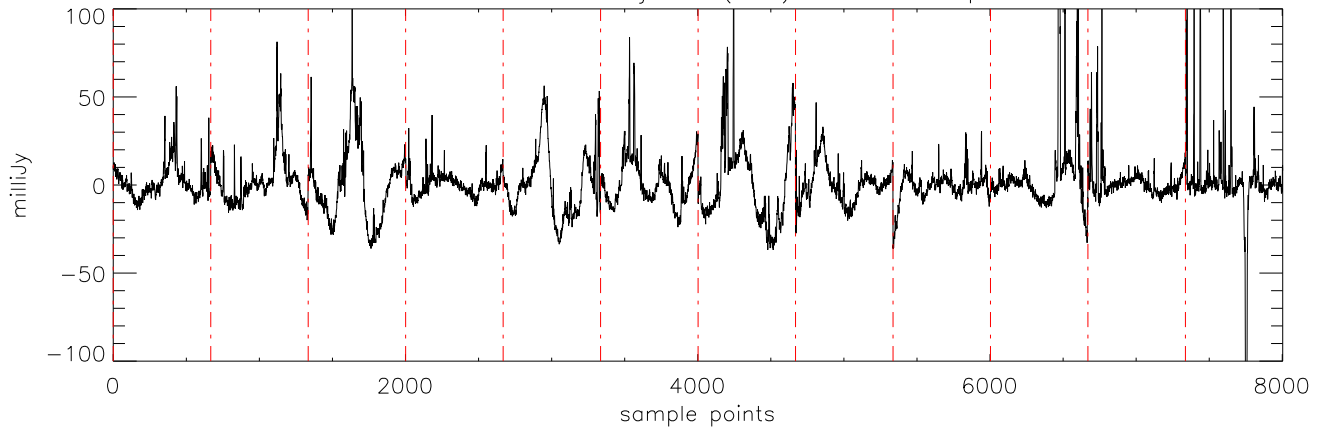
a2471 J21011544 19jul11 (AST) StokesI freq:5176.
