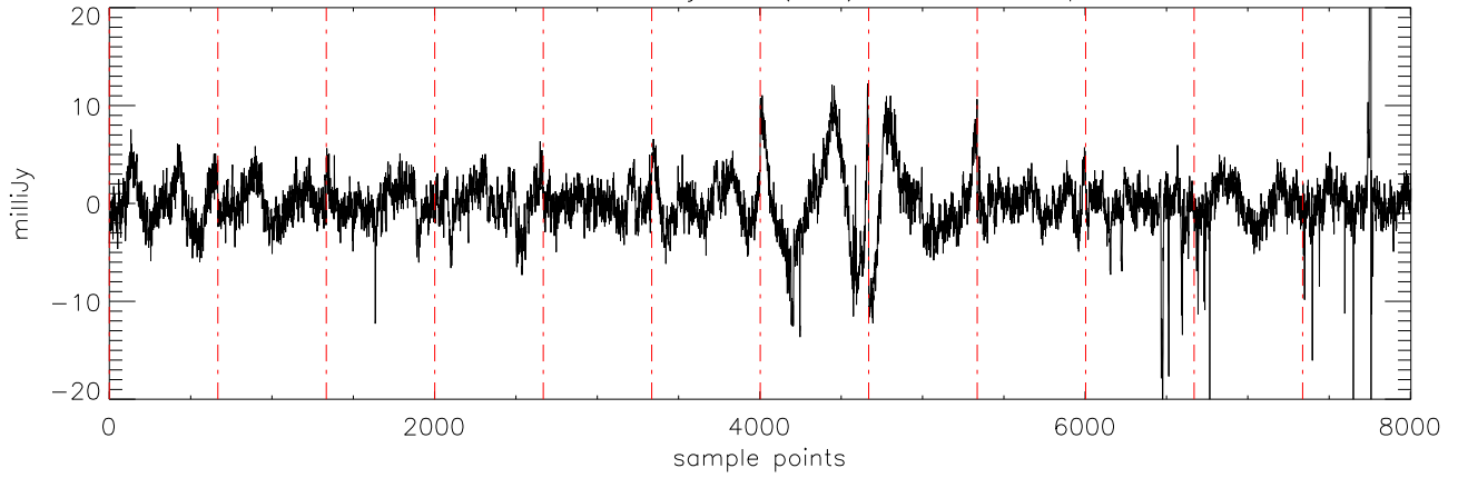
a2471 J21011544 19jul11 (AST) StokesQ freq:4750.
