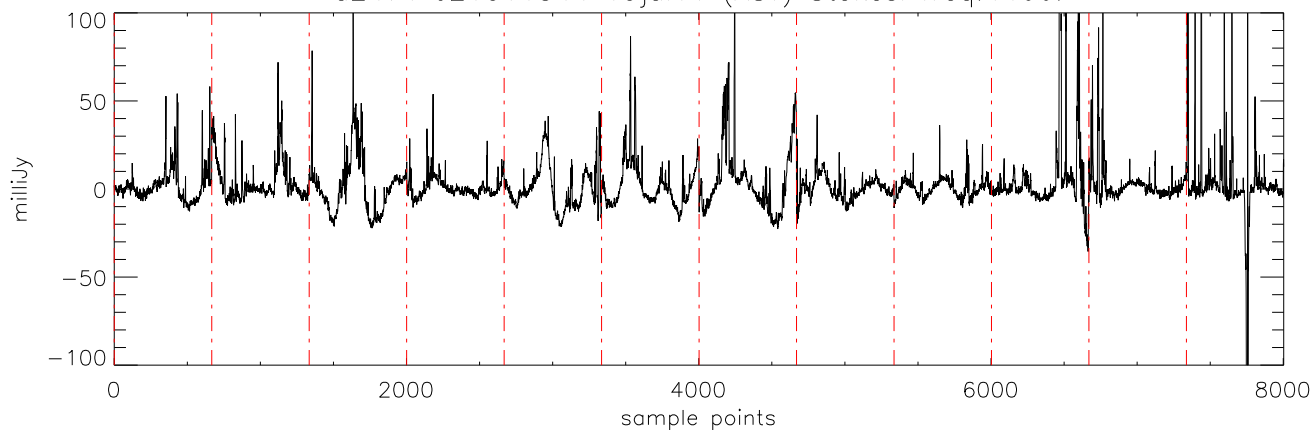
a2471 J21011544 19jul11 (AST) StokesI freq:4608.
