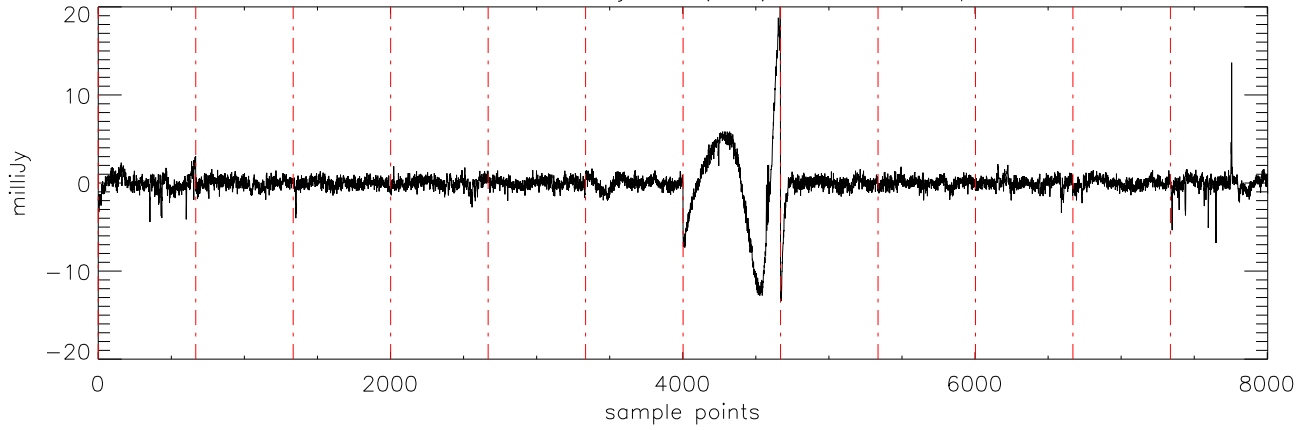
a2471 J21011544 19jul11 (AST) StokesU freq:4750.
