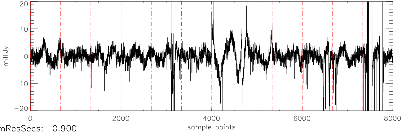
a2471 J21011544 19jul11 (AST) StokesQ freq:4466.
