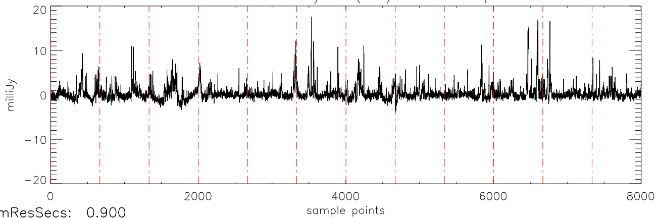
a2471 J21011544 19jul11 (AST) StokesV freq:5034.
