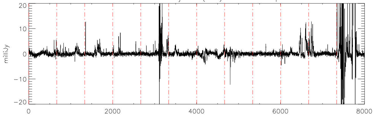
a2471 J21011544 19jul11 (AST) StokesV freq:4325.
