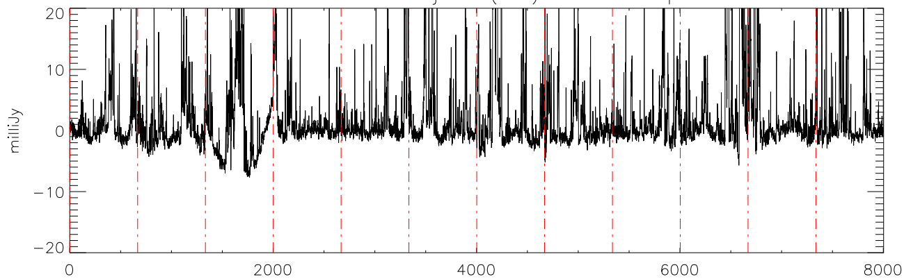
a2471 J21011544 19jul11 (AST) StokesV freq:4750.
