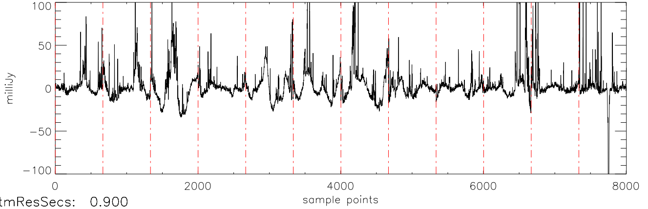
a2471 J21011544 19jul11 (AST) StokesI freq:5034.
