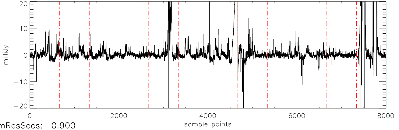
a2471 J21011544 19jul11 (AST) StokesU freq:4466.
