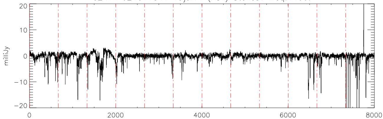
a2471 J21011544 19jul11 (AST) StokesV freq:4466.
