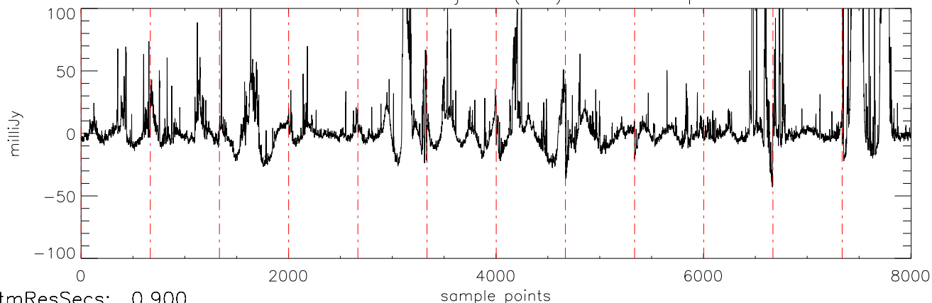
a2471 J21011544 19jul11 (AST) StokesI freq:4466.
