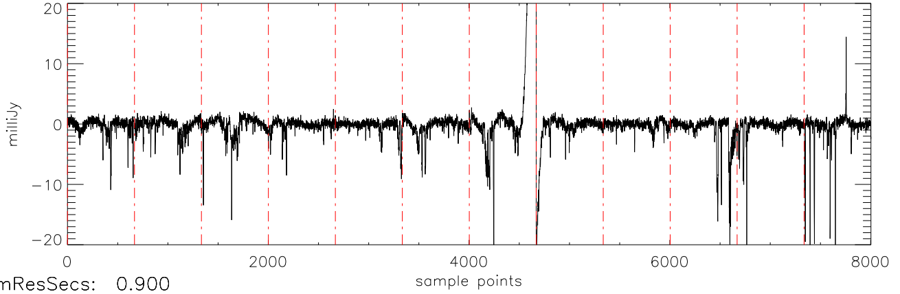
a2471 J21011544 19jul11 (AST) StokesU freq:5034.
