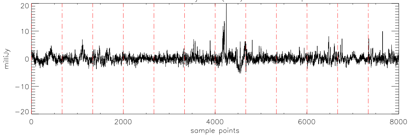
a2471 J21011544 19jul11 (AST) StokesV freq:5176.
