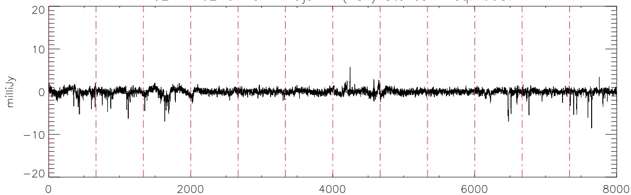
a2471 J21011544 19jul11 (AST) StokesV freq:4608.
