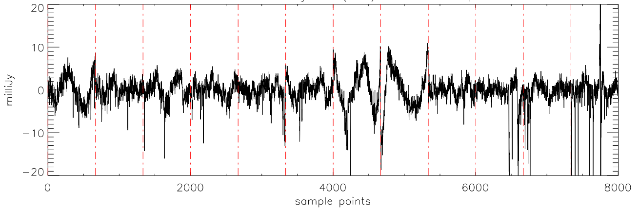
a2471 J21011544 19jul11 (AST) StokesQ freq:4608.
