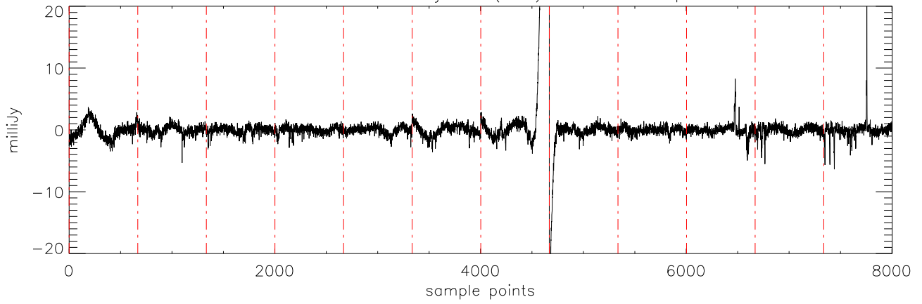
a2471 J21011544 19jul11 (AST) StokesU freq:5176.
