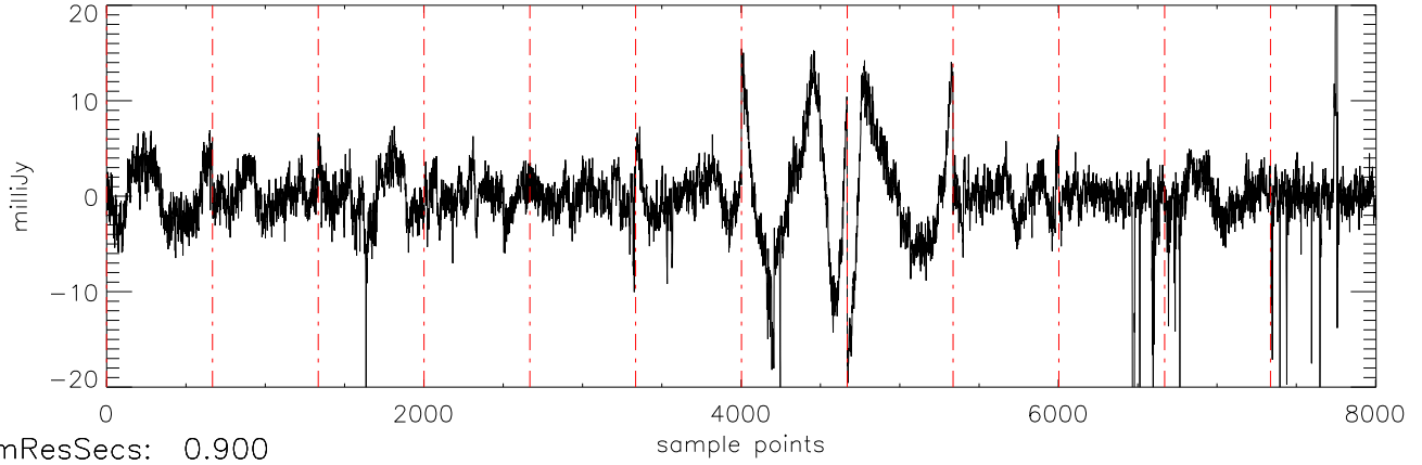
a2471 J21011544 19jul11 (AST) StokesQ freq:5034.
