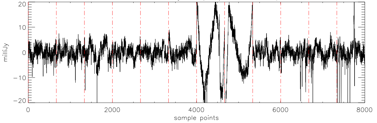
a2471 J21011544 19jul11 (AST) StokesQ freq:5176.
