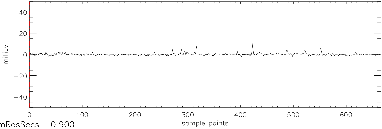
a2471 J2101+17 30dec09 (AST) StokesU freq:4466.
