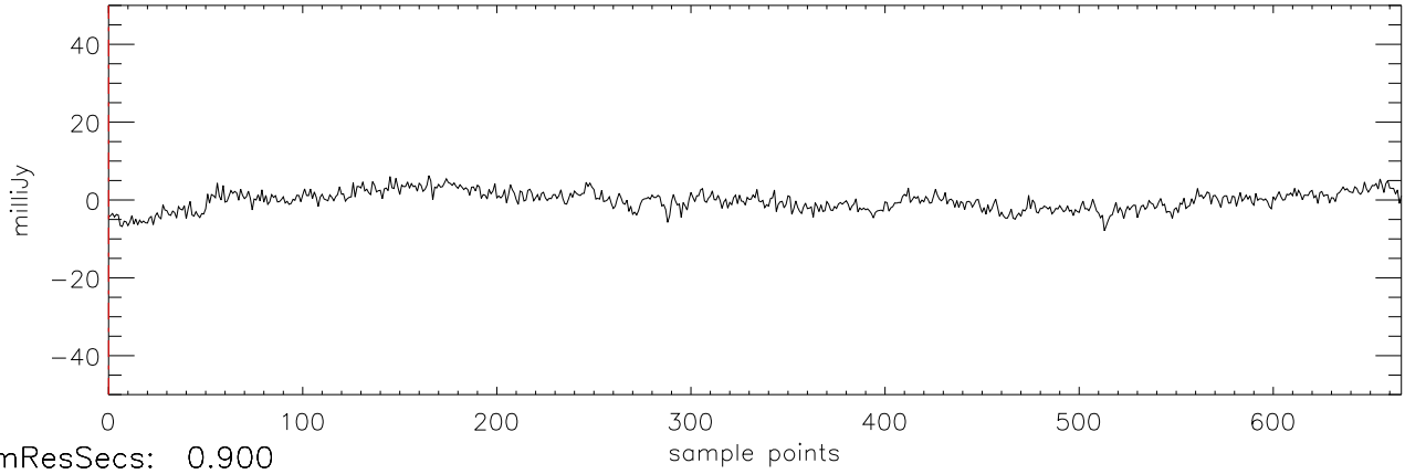
a2471 J2101+17 30dec09 (AST) StokesQ freq:4466.
