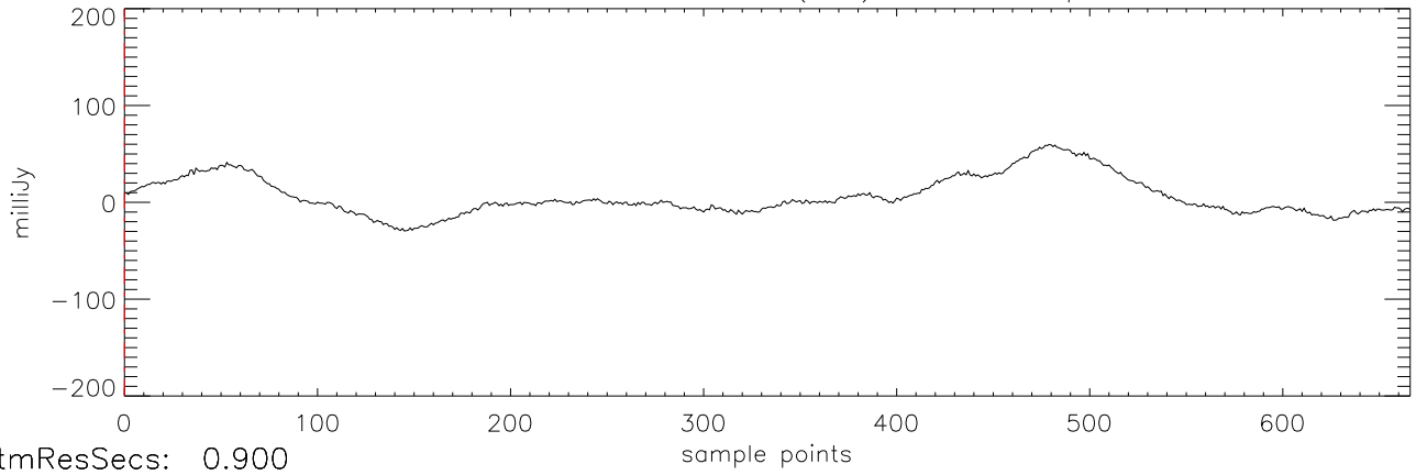
a2471 J2101+17 30dec09 (AST) StokesI freq:5034.
