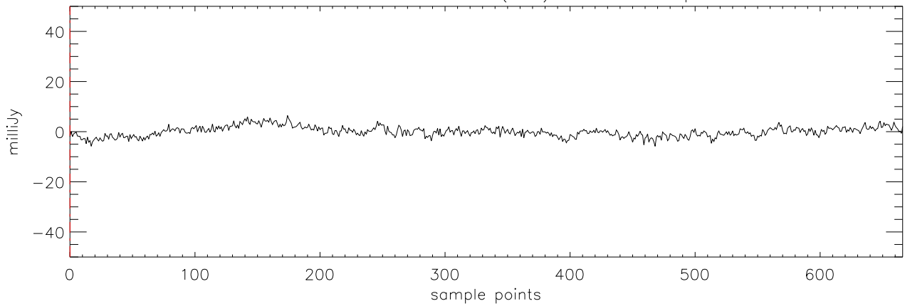
a2471 J2101+17 30dec09 (AST) StokesQ freq:5176.
