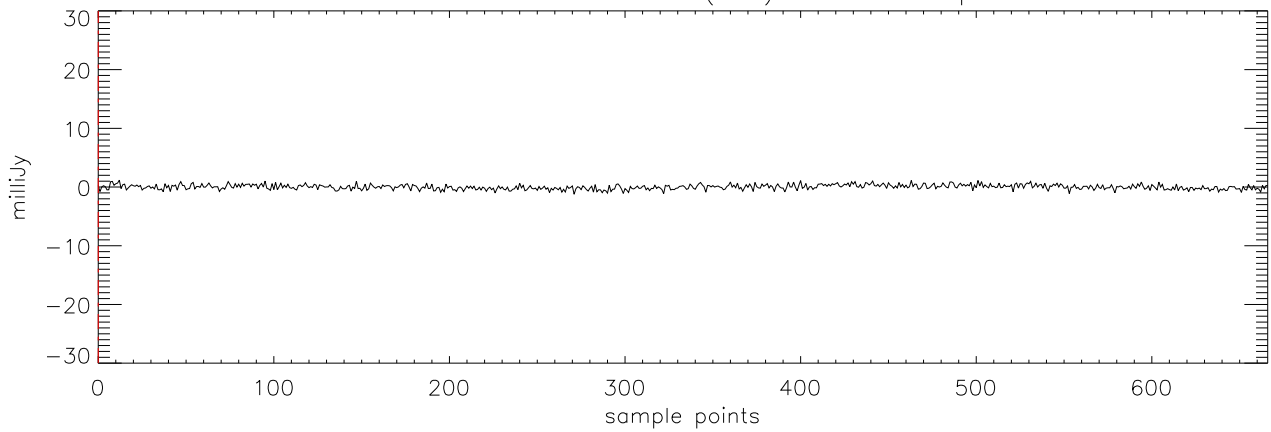
a2471 J2101+17 30dec09 (AST) StokesV freq:4608.
