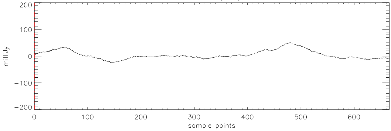
a2471 J2101+17 30dec09 (AST) StokesI freq:4750.
