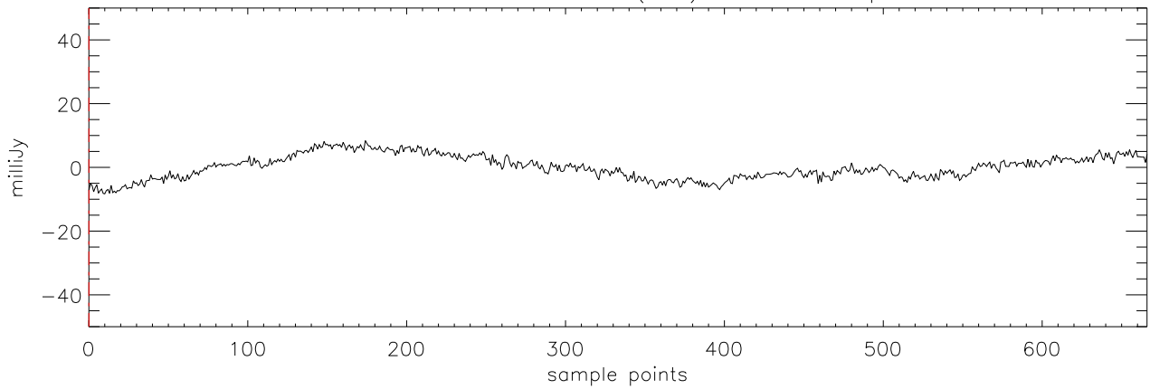
a2471 J2101+17 30dec09 (AST) StokesQ freq:4608.
