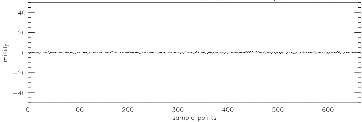
a2471 J2101+17 30dec09 (AST) StokesU freq:4750.
