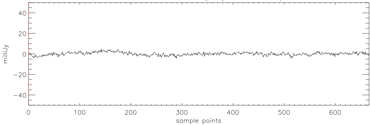
a2471 J2101+17 30dec09 (AST) StokesQ freq:4750.
