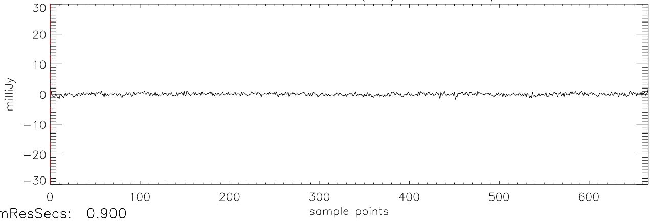
a2471 J2101+17 30dec09 (AST) StokesV freq:5034.
