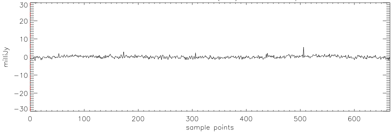
a2471 J2101+17 30dec09 (AST) StokesV freq:5176.
