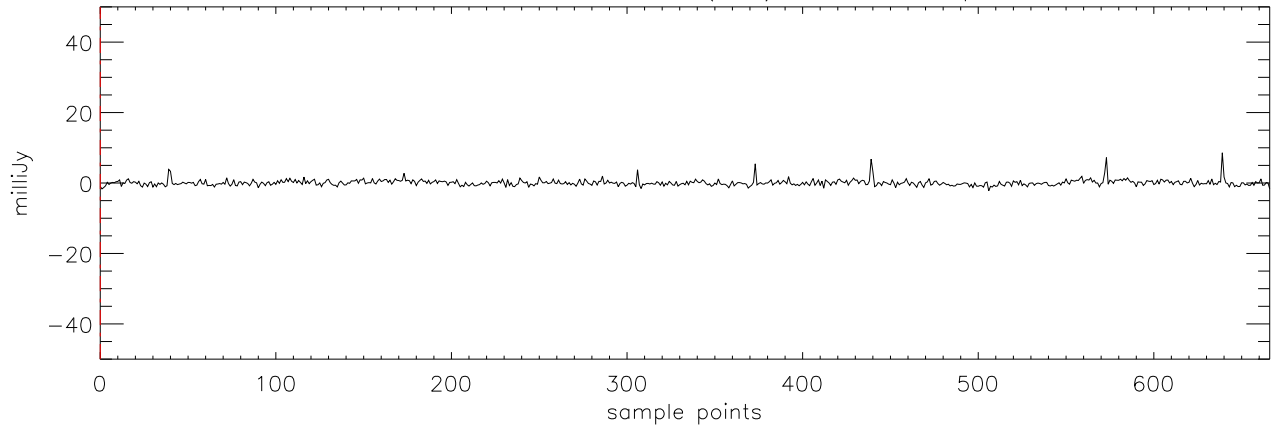
a2471 J2101+17 30dec09 (AST) StokesU freq:5176.
