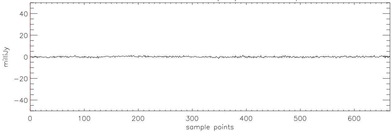
a2471 J2101+17 30dec09 (AST) StokesU freq:4608.
