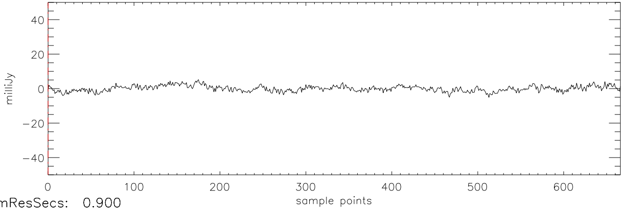
a2471 J2101+17 30dec09 (AST) StokesQ freq:5034.
