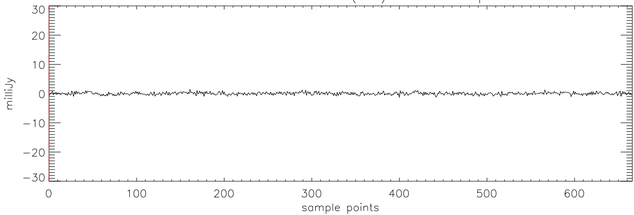
a2471 J2101+17 30dec09 (AST) StokesV freq:4750.
