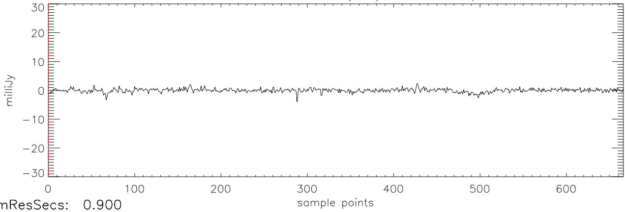
a2471 J2101+17 30dec09 (AST) StokesV freq:4466.
