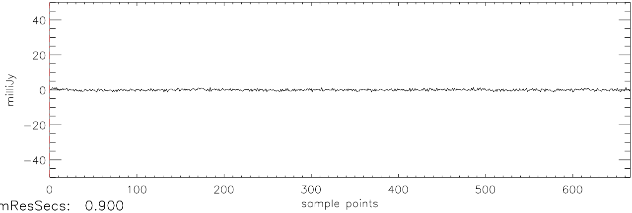
a2471 J2101+17 30dec09 (AST) StokesU freq:5034.
