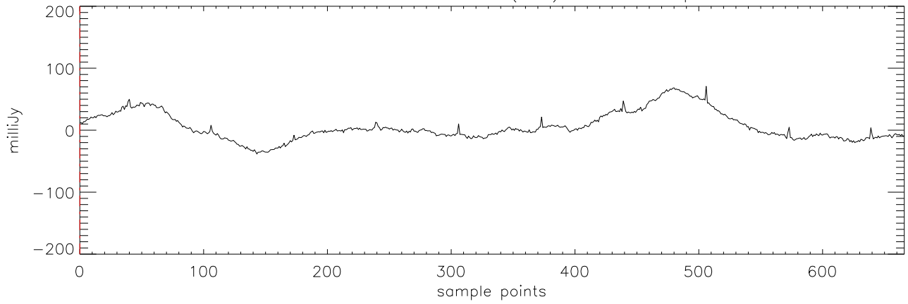
a2471 J2101+17 30dec09 (AST) StokesI freq:5176.
