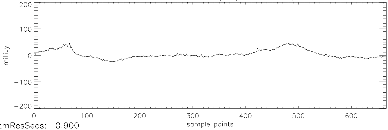
a2471 J2101+17 30dec09 (AST) StokesI freq:4466.
