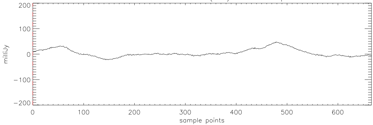
a2471 J2101+17 30dec09 (AST) StokesI freq:4608.
