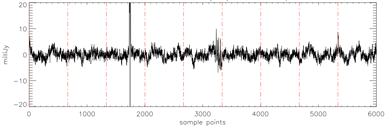
a2471 J1711457 30mar12 (AST) StokesQ freq:4750.
