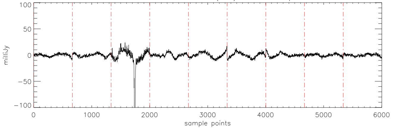
a2471 J1711457 30mar12 (AST) StokesI freq:5176.
