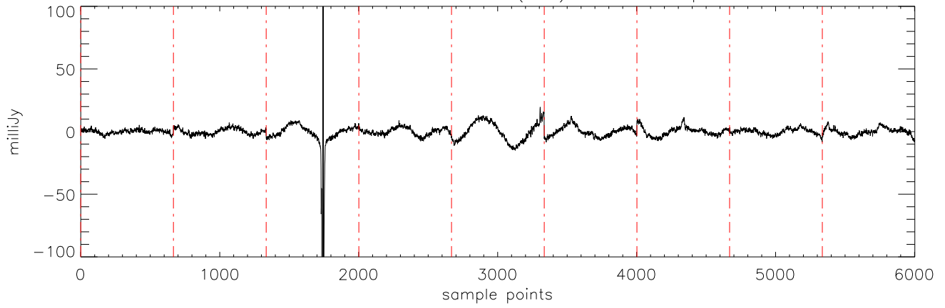
a2471 J1711457 30mar12 (AST) StokesI freq:4608.
