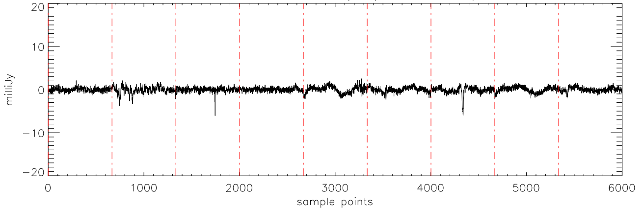
a2471 J1711457 30mar12 (AST) StokesU freq:4750.
