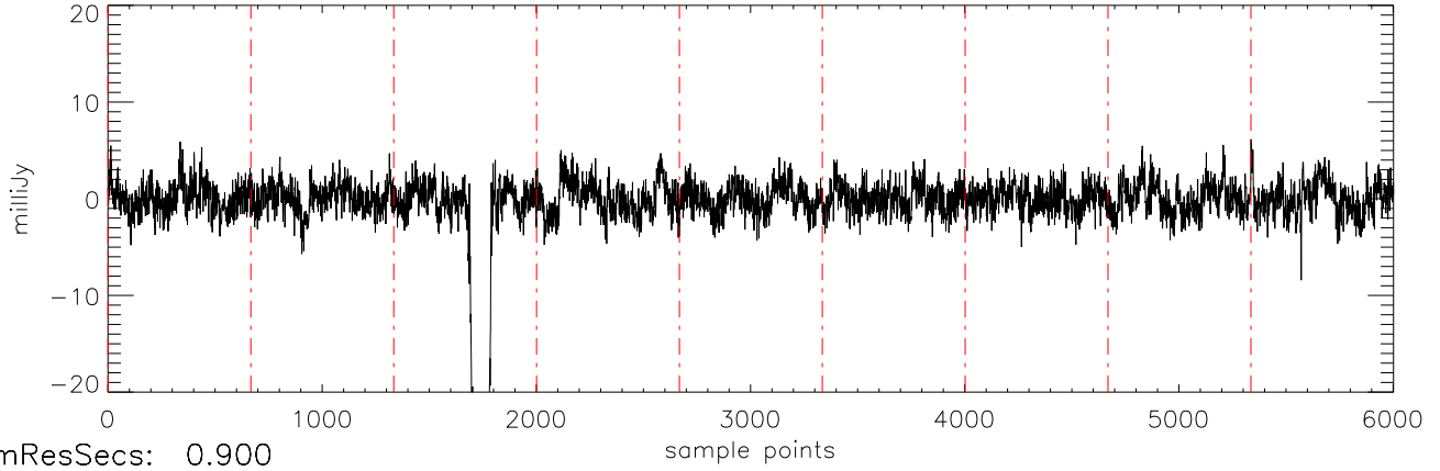
a2471 J1711457 30mar12 (AST) StokesQ freq:4466.
