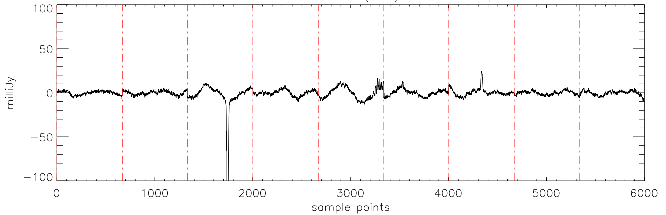
a2471 J1711457 30mar12 (AST) StokesI freq:4750.
