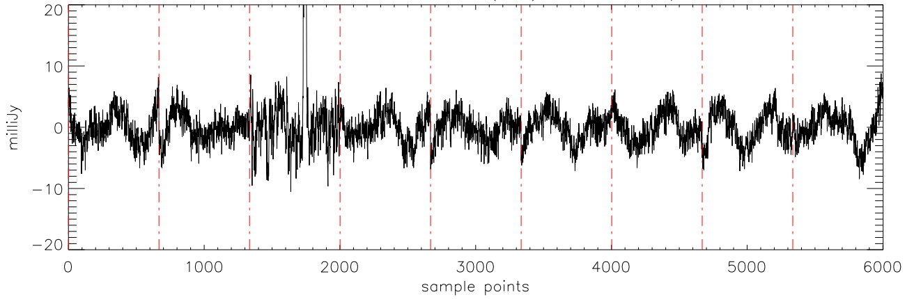
a2471 J1711457 30mar12 (AST) StokesQ freq:5176.
