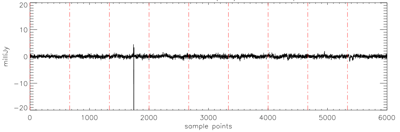
a2471 J1711457 30mar12 (AST) StokesV freq:4608.
