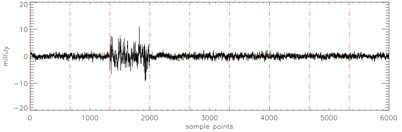
a2471 J1711457 30mar12 (AST) StokesV freq:5176.
