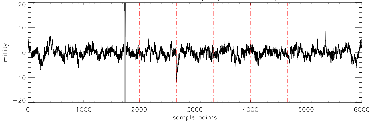
a2471 J1711457 30mar12 (AST) StokesQ freq:4608.
