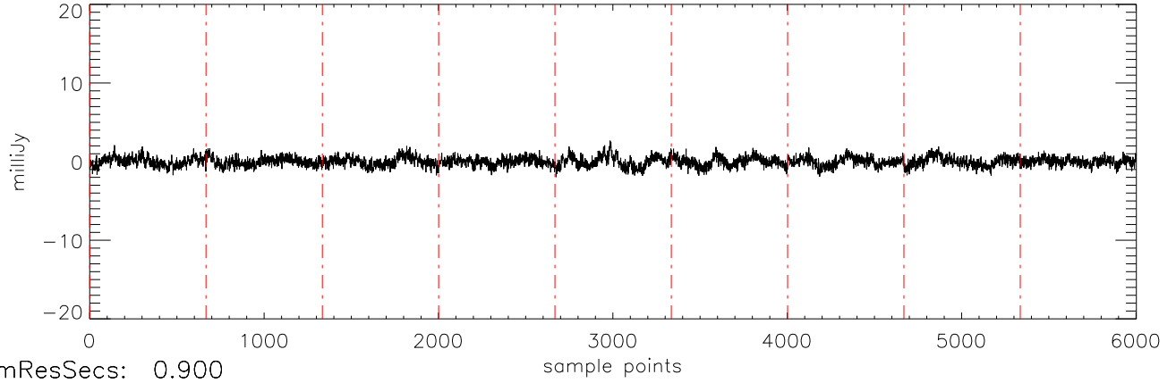
a2471 J1711457 30mar12 (AST) StokesU freq:5034.
