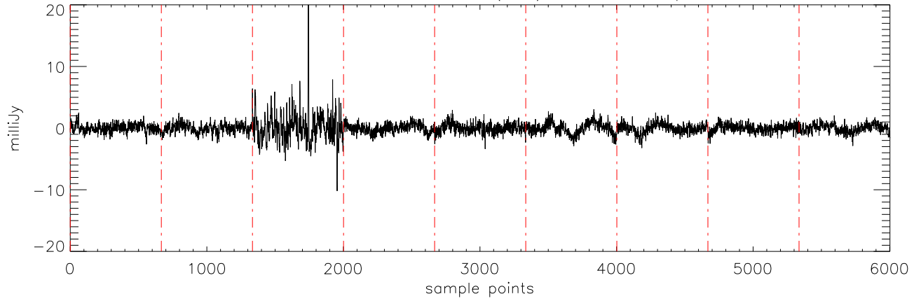
a2471 J1711457 30mar12 (AST) StokesU freq:5176.
