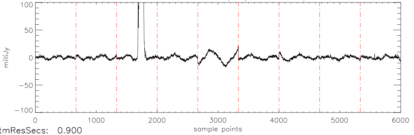
a2471 J1711457 30mar12 (AST) StokesI freq:4466.
