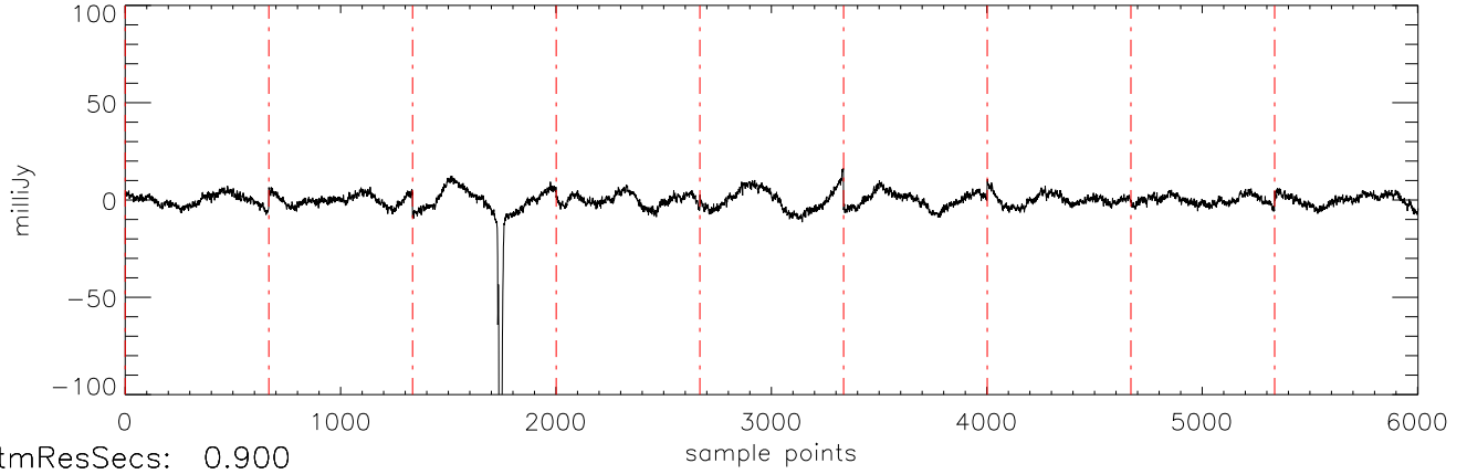
a2471 J1711457 30mar12 (AST) StokesI freq:5034.
