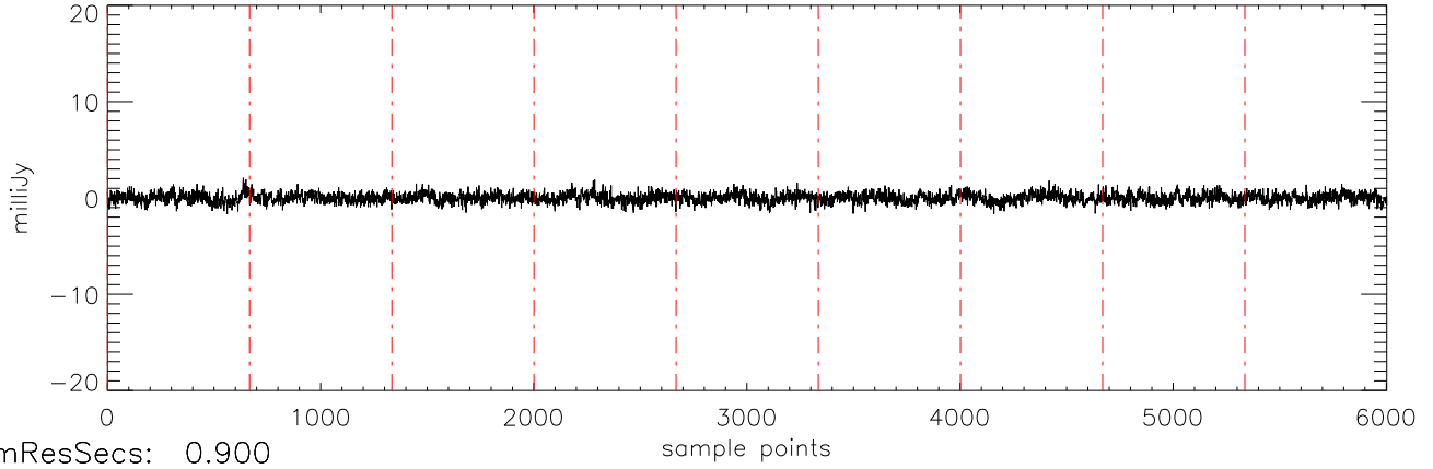
a2471 J1711457 30mar12 (AST) StokesV freq:5034.
