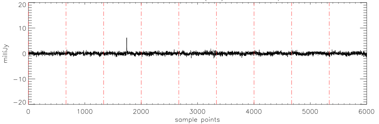
a2471 J1711457 30mar12 (AST) StokesV freq:4750.
