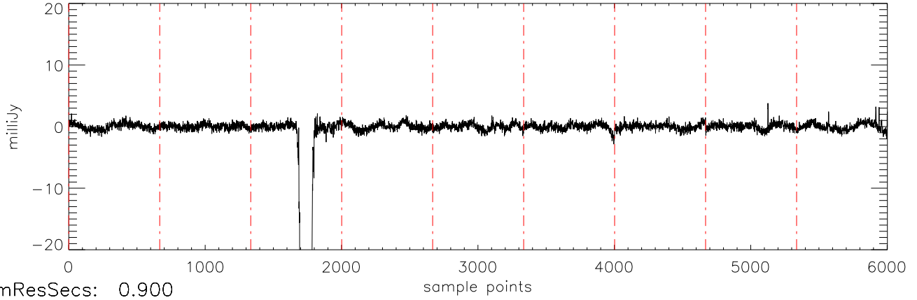
a2471 J1711457 30mar12 (AST) StokesU freq:4466.
