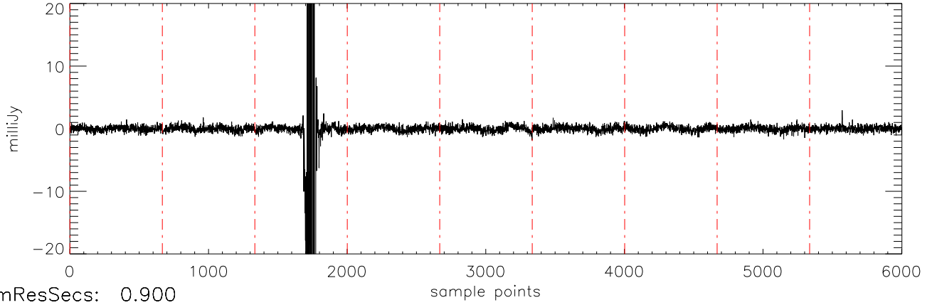
a2471 J1711457 30mar12 (AST) StokesV freq:4466.
