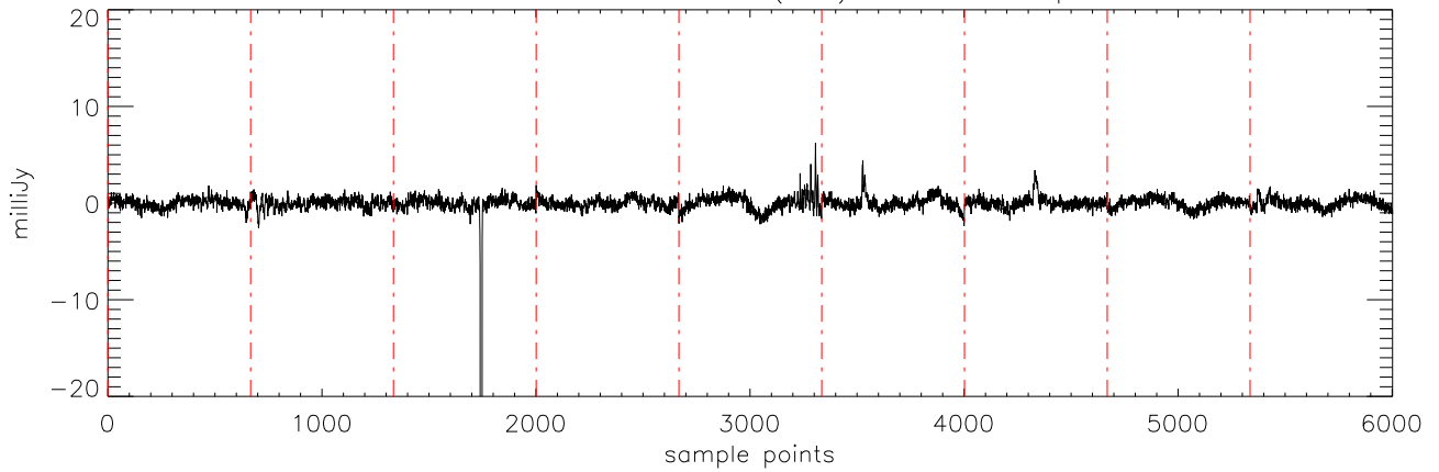
a2471 J1711457 30mar12 (AST) StokesU freq:4608.
