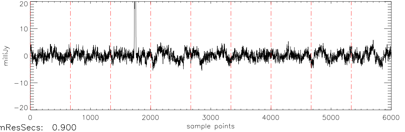
a2471 J1711457 30mar12 (AST) StokesQ freq:5034.
