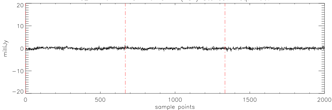
a2471 J1711457 16mar11 (AST) StokesV freq:4608.
