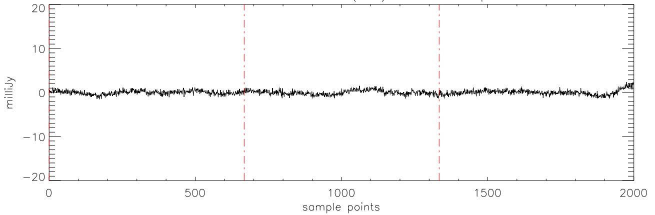
a2471 J1711457 16mar11 (AST) StokesU freq:4608.
