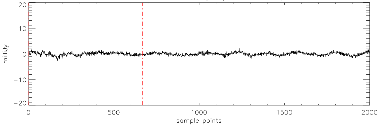
a2471 J1711457 16mar11 (AST) StokesU freq:4750.
