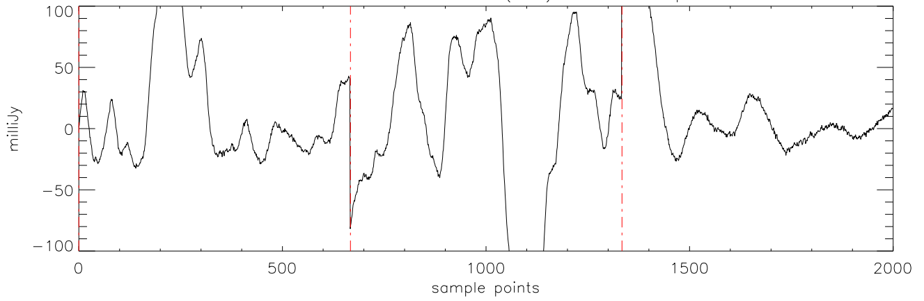
a2471 J1711457 16mar11 (AST) StokesI freq:5176.
