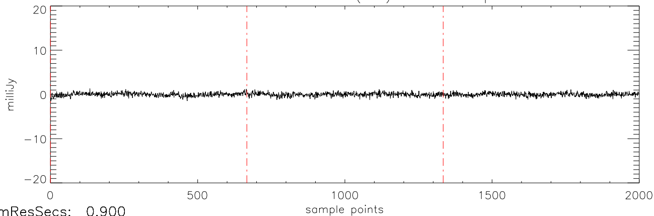
a2471 J1711457 16mar11 (AST) StokesV freq:4466.
