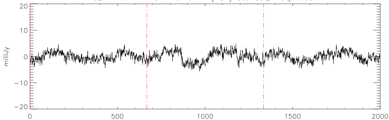
a2471 J1711457 16mar11 (AST) StokesQ freq:4608.
