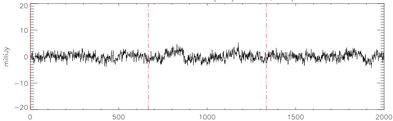
a2471 J1711457 16mar11 (AST) StokesQ freq:4750.
