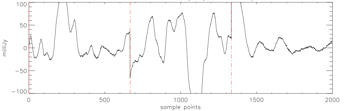
a2471 J1711457 16mar11 (AST) StokesI freq:4750.
