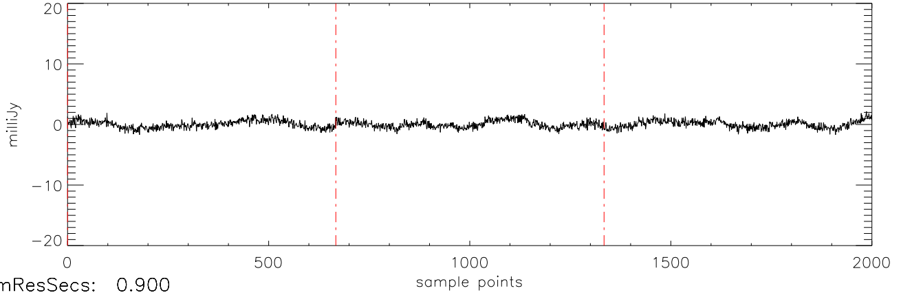
a2471 J1711457 16mar11 (AST) StokesU freq:4466.
