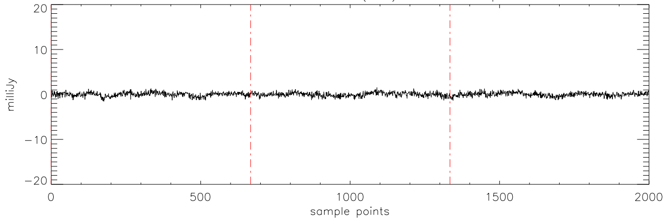
a2471 J1711457 16mar11 (AST) StokesV freq:4750.
