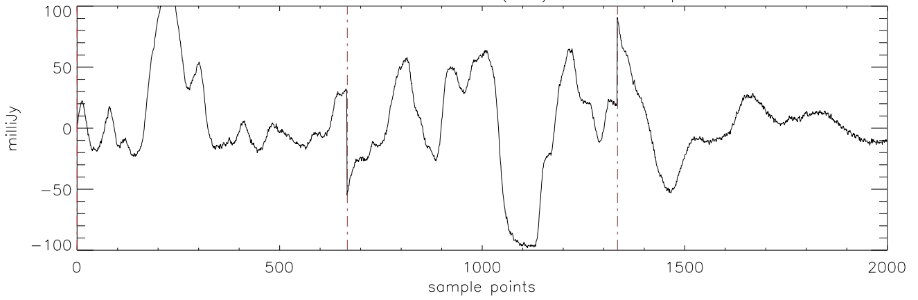
a2471 J1711457 16mar11 (AST) StokesI freq:4608.
