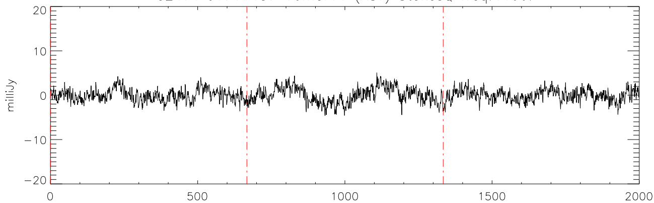
a2471 J1711457 16mar11 (AST) StokesQ freq:4466.
