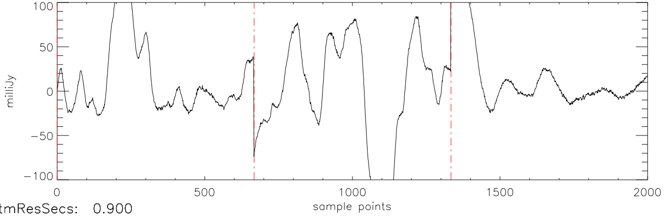
a2471 J1711457 16mar11 (AST) StokesI freq:5034.
