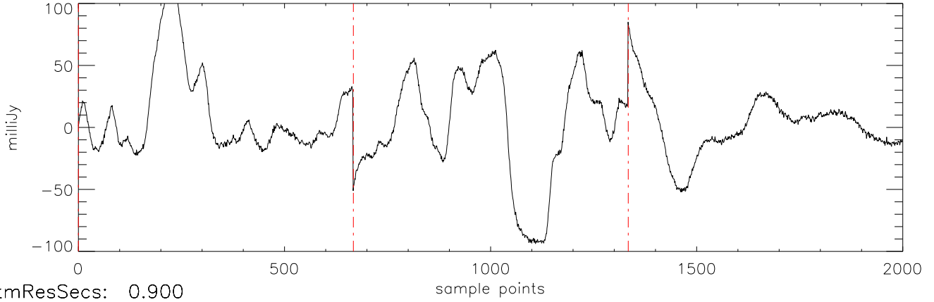
a2471 J1711457 16mar11 (AST) StokesI freq:4466.
