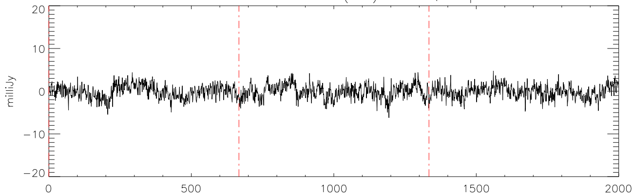
a2471 J1711457 16mar11 (AST) StokesQ freq:4325.
