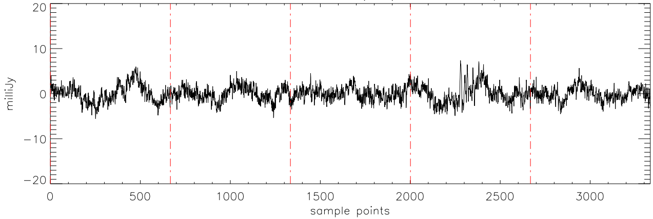
a2471 J1711457 15mar11 (AST) StokesQ freq:4750.
