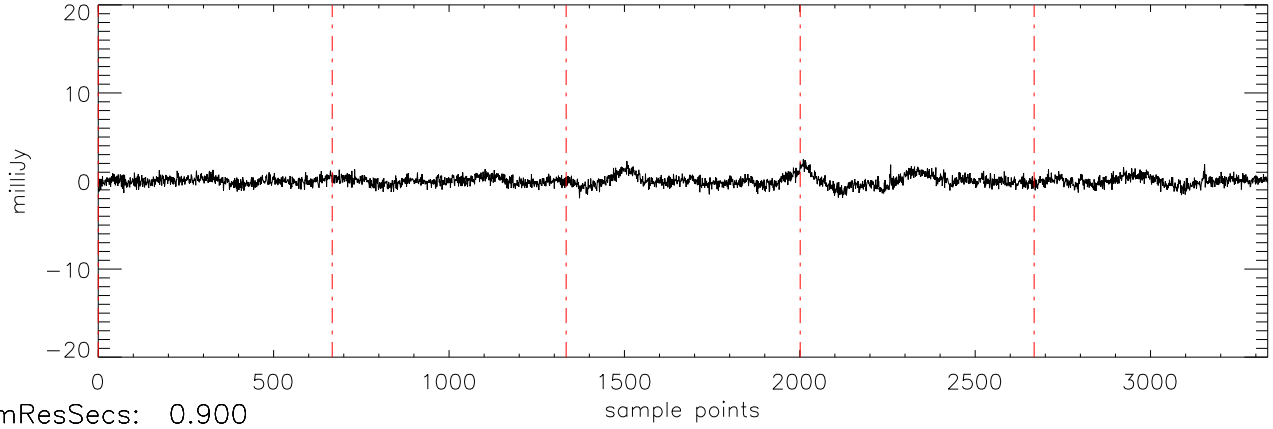
a2471 J1711457 15mar11 (AST) StokesU freq:4466.
