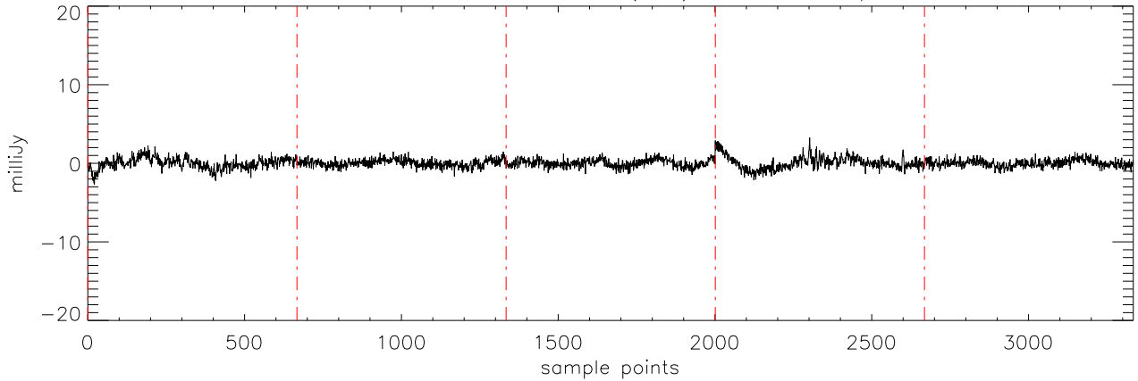
a2471 J1711457 15mar11 (AST) StokesU freq:4750.
