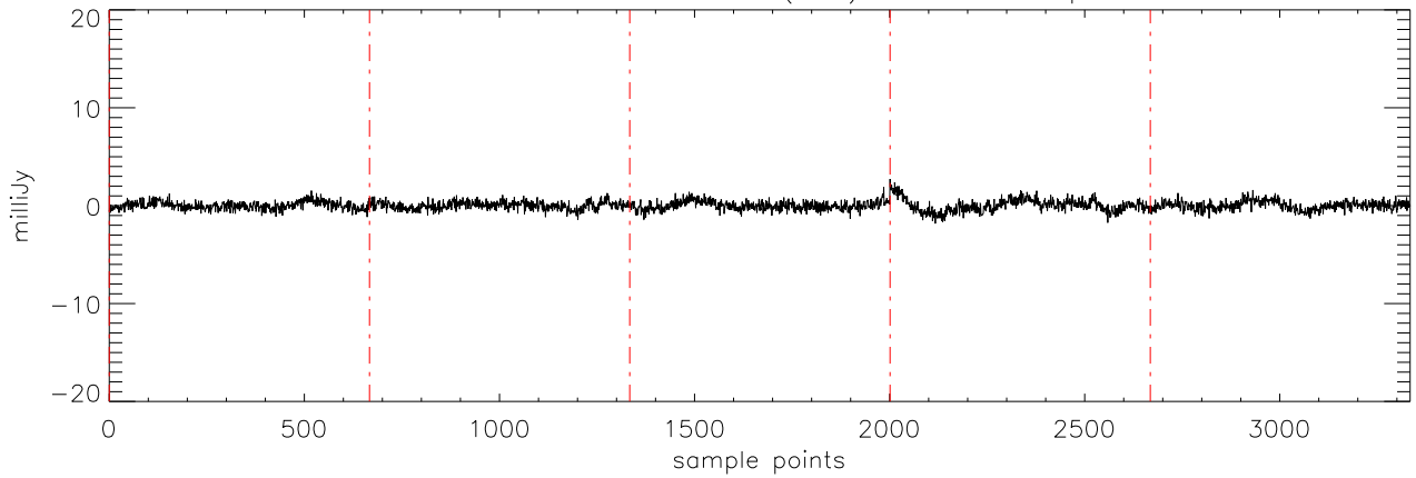
a2471 J1711457 15mar11 (AST) StokesU freq:4608.
