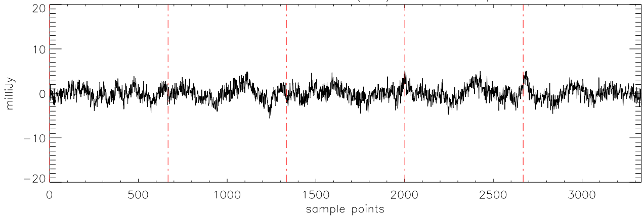
a2471 J1711457 15mar11 (AST) StokesQ freq:4608.
