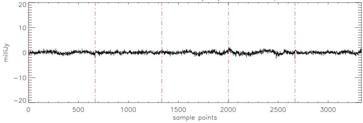
a2471 J1711457 15mar11 (AST) StokesU freq:5176.
