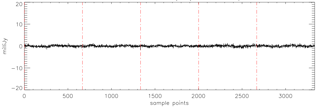
a2471 J1711457 15mar11 (AST) StokesV freq:4608.
