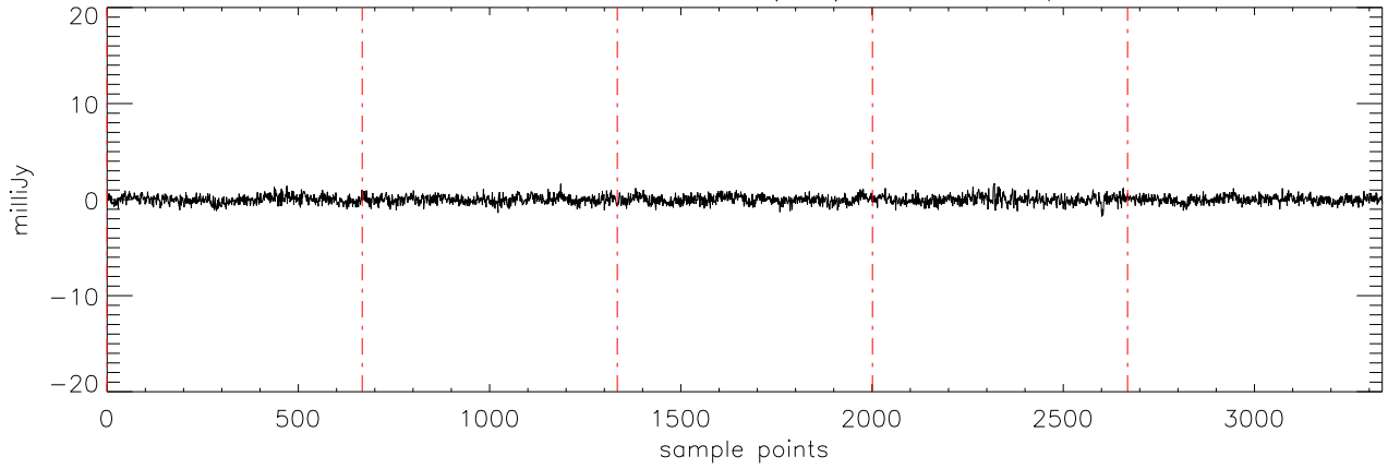
a2471 J1711457 15mar11 (AST) StokesV freq:4750.
