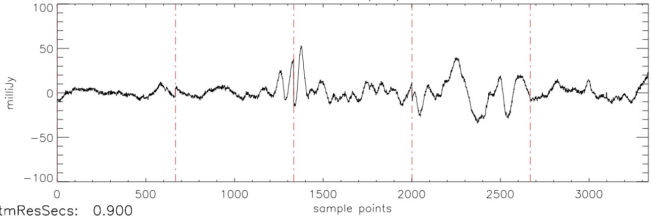
a2471 J1711457 15mar11 (AST) StokesI freq:4466.
