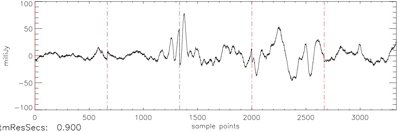
a2471 J1711457 15mar11 (AST) StokesI freq:5034.
