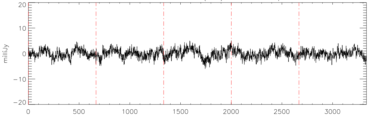
a2471 J1711457 15mar11 (AST) StokesQ freq:5034.
