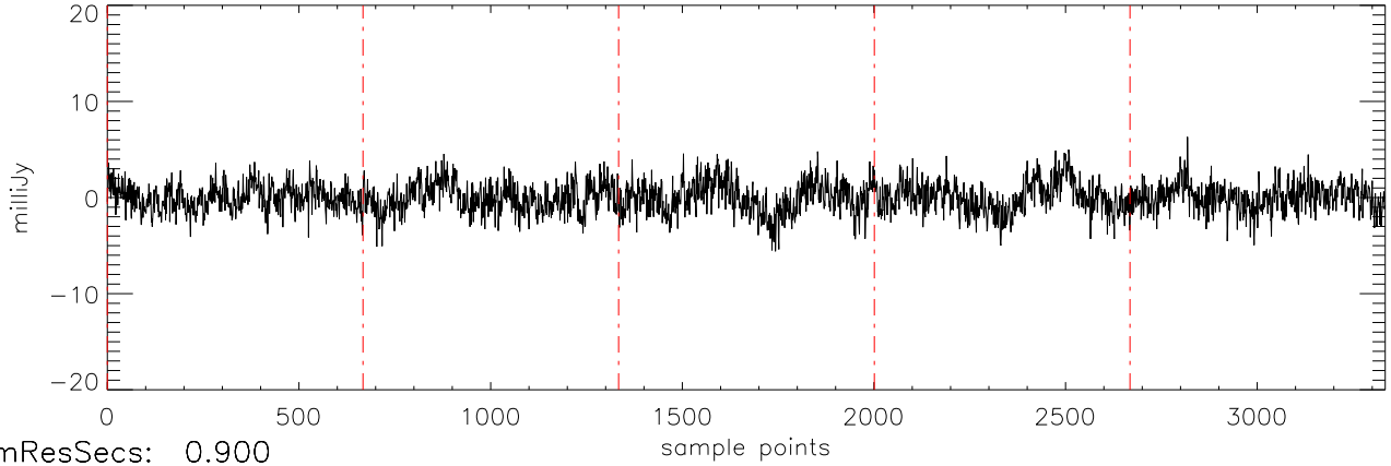
a2471 J1711457 15mar11 (AST) StokesQ freq:4466.
