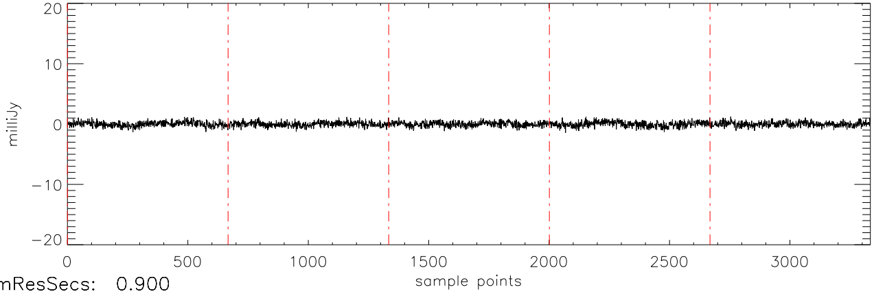
a2471 J1711457 15mar11 (AST) StokesV freq:4466.
