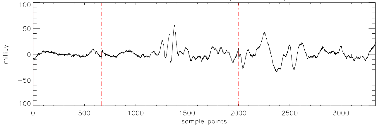
a2471 J1711457 15mar11 (AST) StokesI freq:4608.
