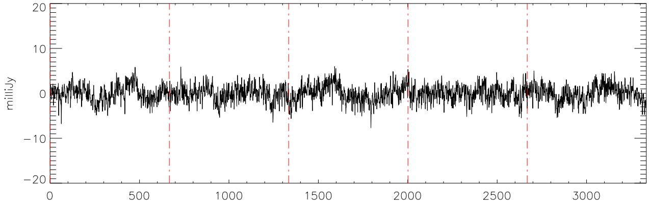
a2471 J1711457 15mar11 (AST) StokesQ freq:5176.
