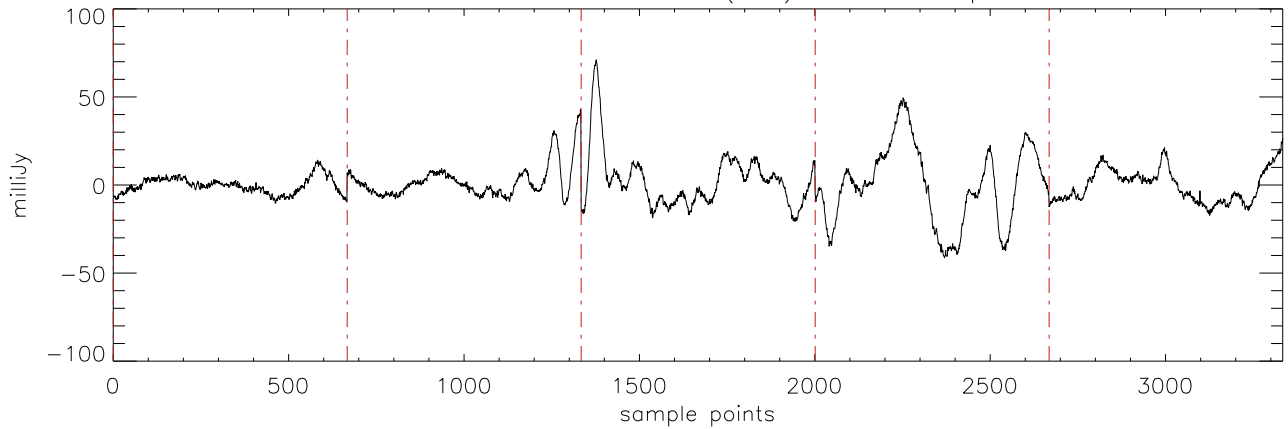
a2471 J1711457 15mar11 (AST) StokesI freq:4750.
