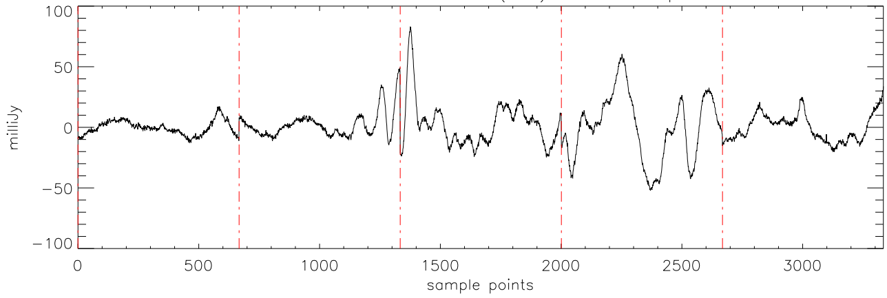
a2471 J1711457 15mar11 (AST) StokesI freq:5176.
