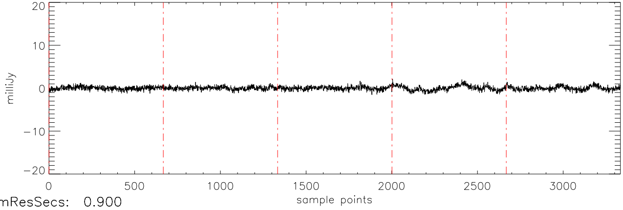
a2471 J1711457 15mar11 (AST) StokesU freq:5034.
