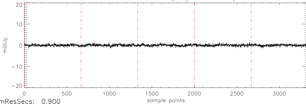
a2471 J1711457 15mar11 (AST) StokesV freq:5034.
