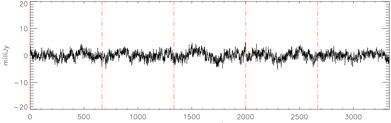
a2471 J1711457 15mar11 (AST) StokesQ freq:4892.
