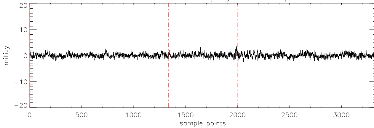
a2471 J1711457 15mar11 (AST) StokesV freq:5176.
