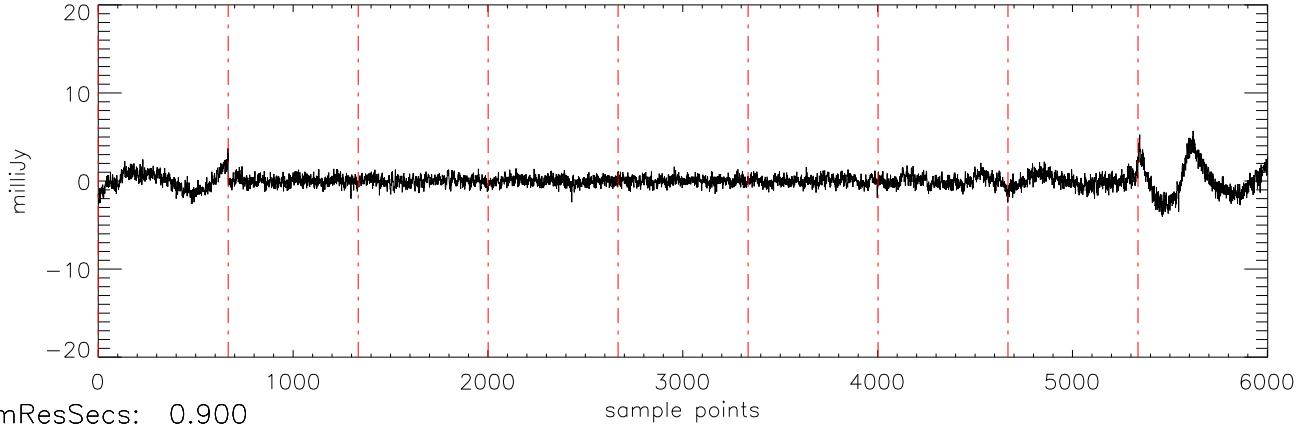
a2471 J16322911 31mar12 (AST) StokesV freq:5034.
