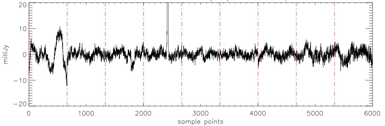
a2471 J16322911 31mar12 (AST) StokesQ freq:4750.
