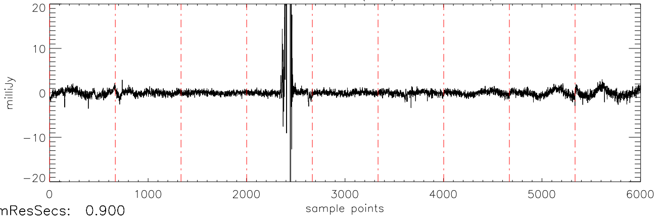
a2471 J16322911 31mar12 (AST) StokesV freq:4466.
