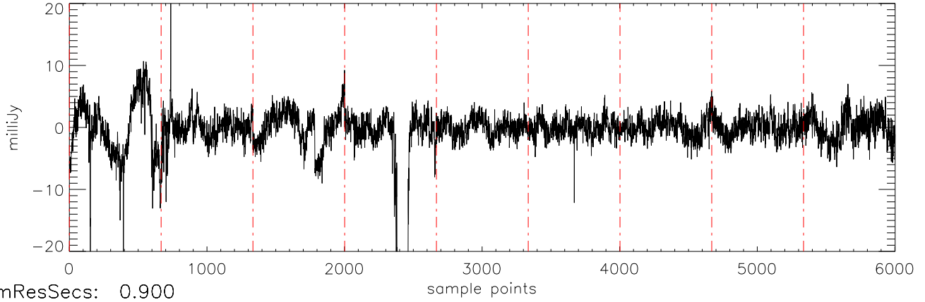
a2471 J16322911 31mar12 (AST) StokesQ freq:4466.
