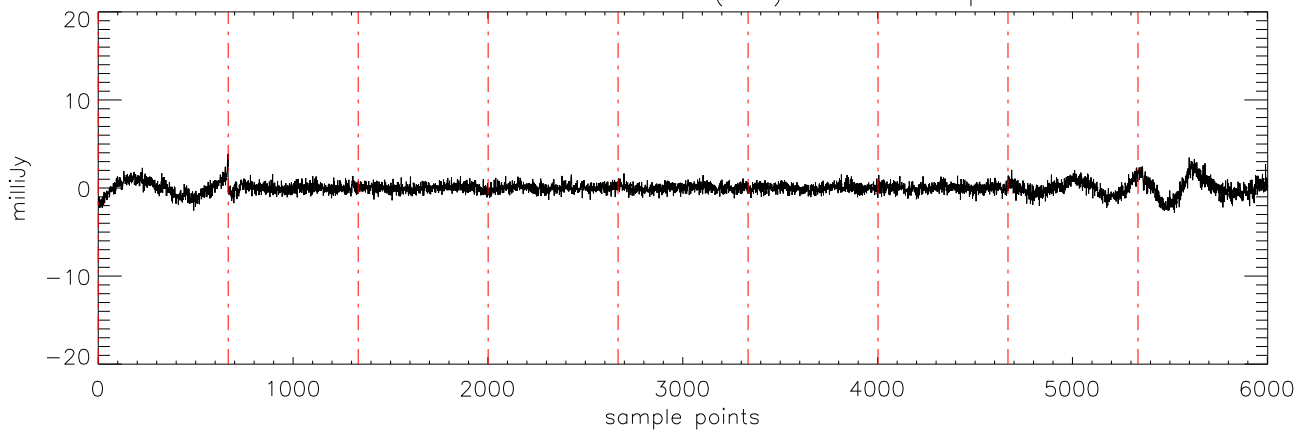
a2471 J16322911 31mar12 (AST) StokesV freq:4750.
