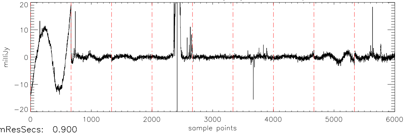
a2471 J16322911 31mar12 (AST) StokesU freq:4466.
