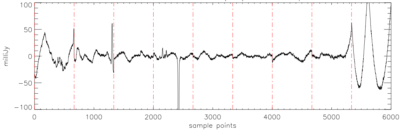
a2471 J16322911 31mar12 (AST) StokesI freq:4750.
