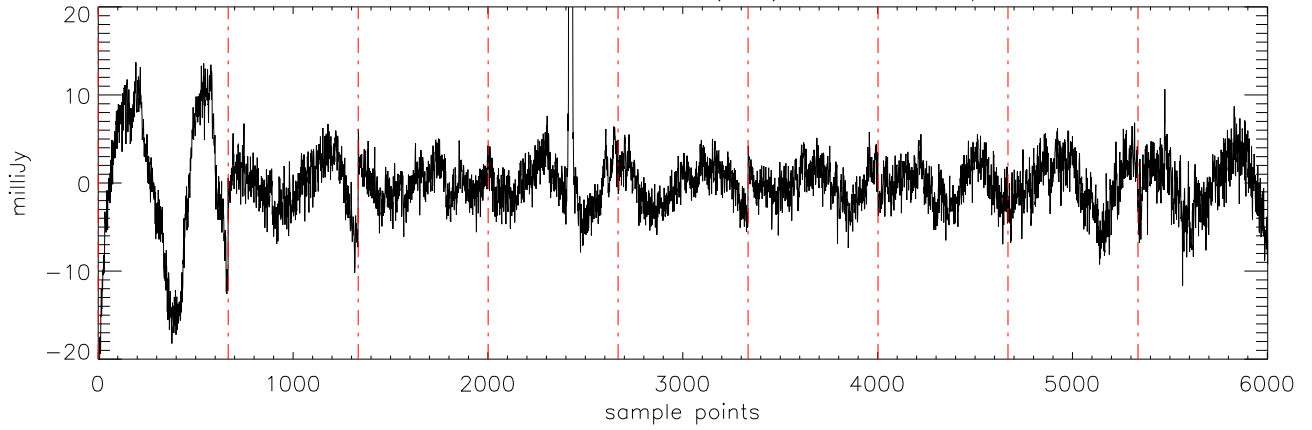
a2471 J16322911 31mar12 (AST) StokesQ freq:5176.
