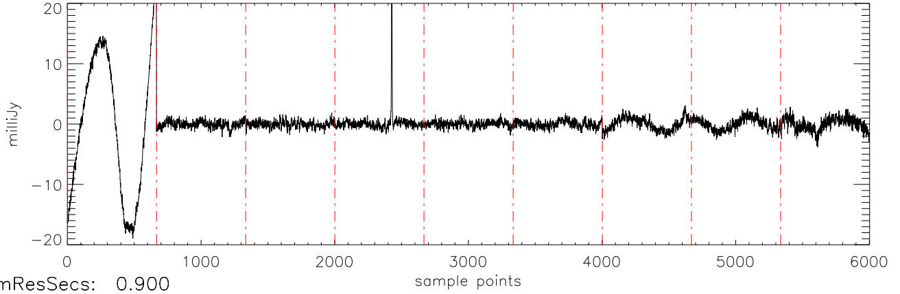
a2471 J16322911 31mar12 (AST) StokesU freq:5034.
