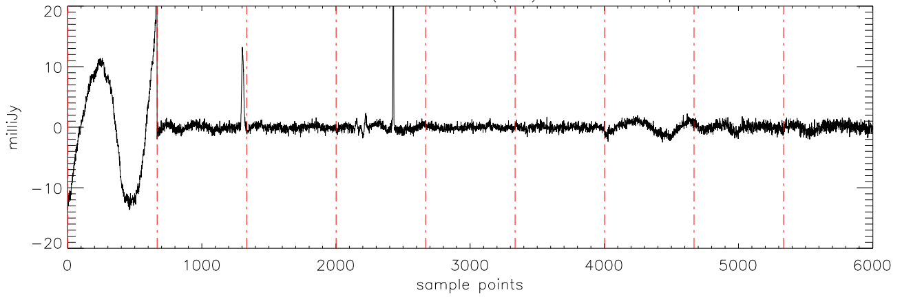
a2471 J16322911 31mar12 (AST) StokesU freq:4750.
