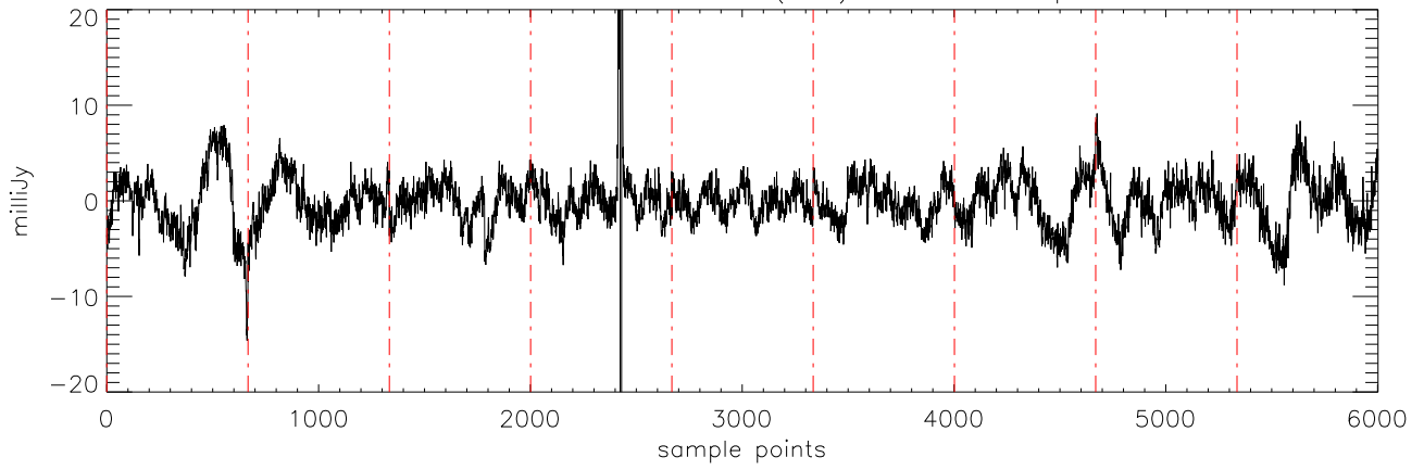
a2471 J16322911 31mar12 (AST) StokesQ freq:4608.
