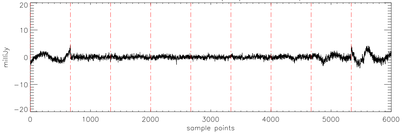
a2471 J16322911 31mar12 (AST) StokesV freq:5176.
