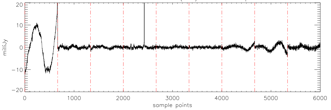
a2471 J16322911 31mar12 (AST) StokesU freq:4608.
