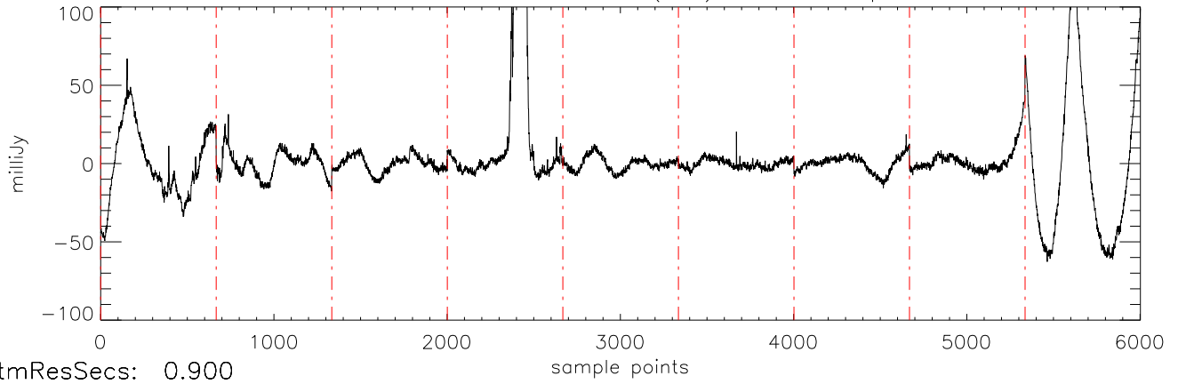
a2471 J16322911 31mar12 (AST) StokesI freq:4466.
