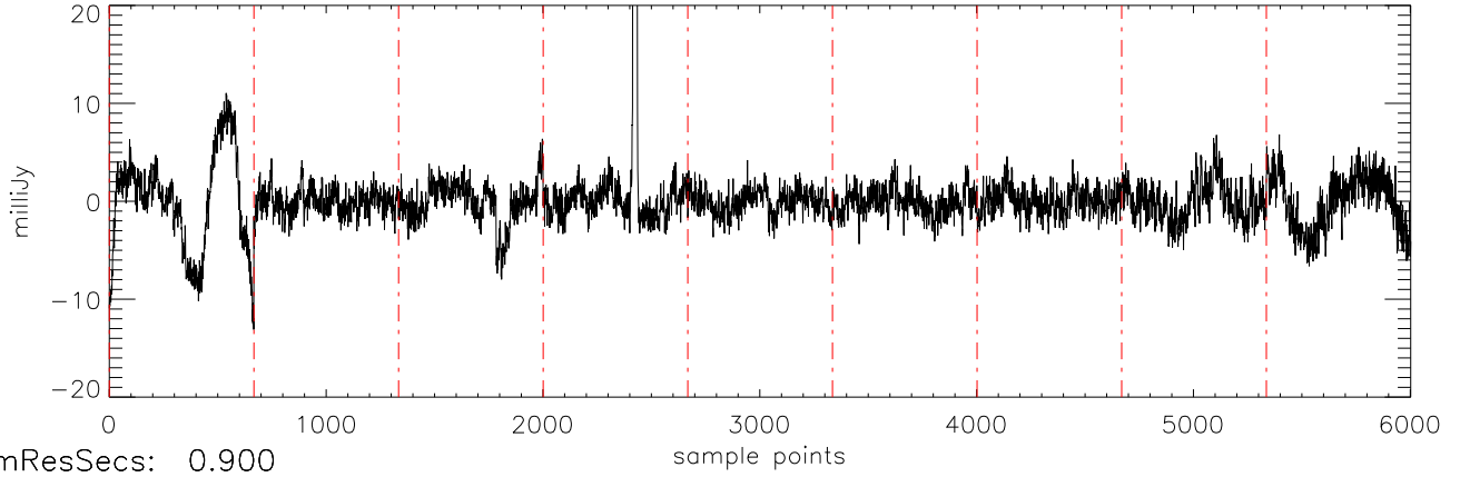
a2471 J16322911 31mar12 (AST) StokesQ freq:5034.
