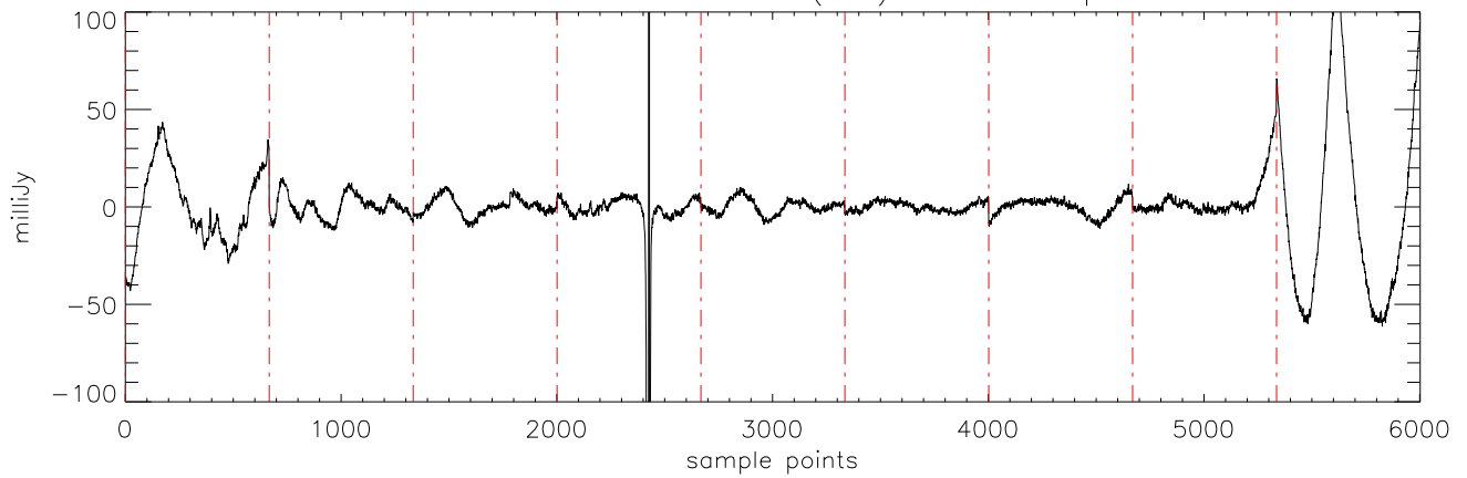
a2471 J16322911 31mar12 (AST) StokesI freq:4608.
