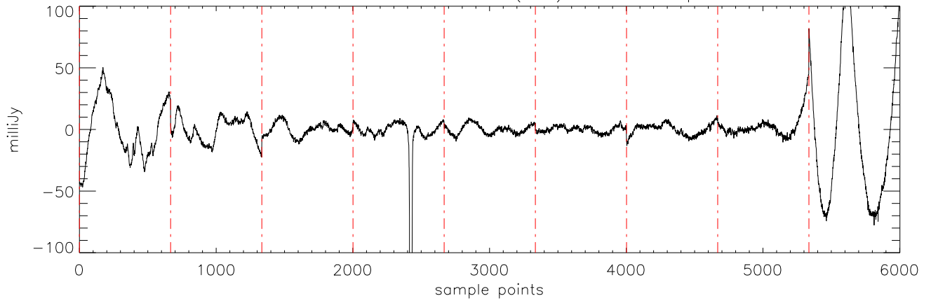
a2471 J16322911 31mar12 (AST) StokesI freq:5176.
