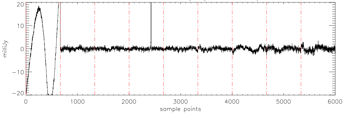
a2471 J16322911 31mar12 (AST) StokesU freq:5176.
