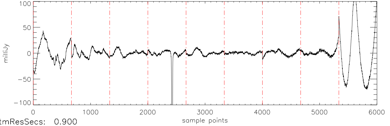
a2471 J16322911 31mar12 (AST) StokesI freq:5034.
