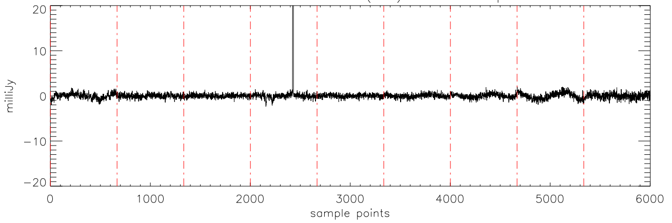
a2471 J16322911 31mar12 (AST) StokesV freq:4608.
