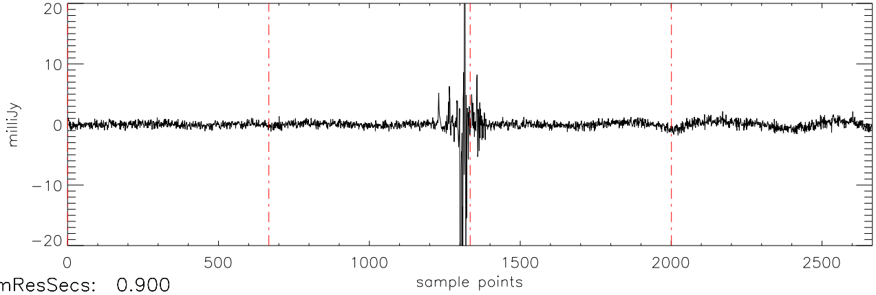
a2471 J16322911 09mar12 (AST) StokesV freq:4466.
