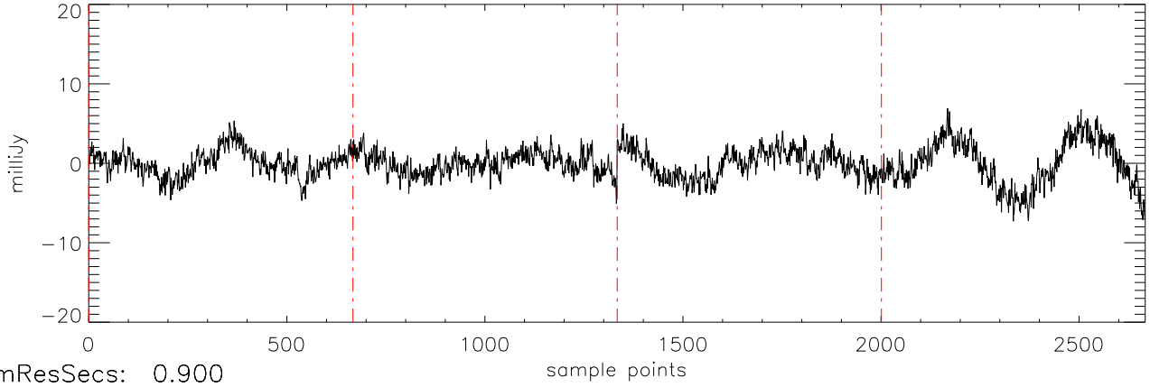
a2471 J16322911 09mar12 (AST) StokesQ freq:5034.
