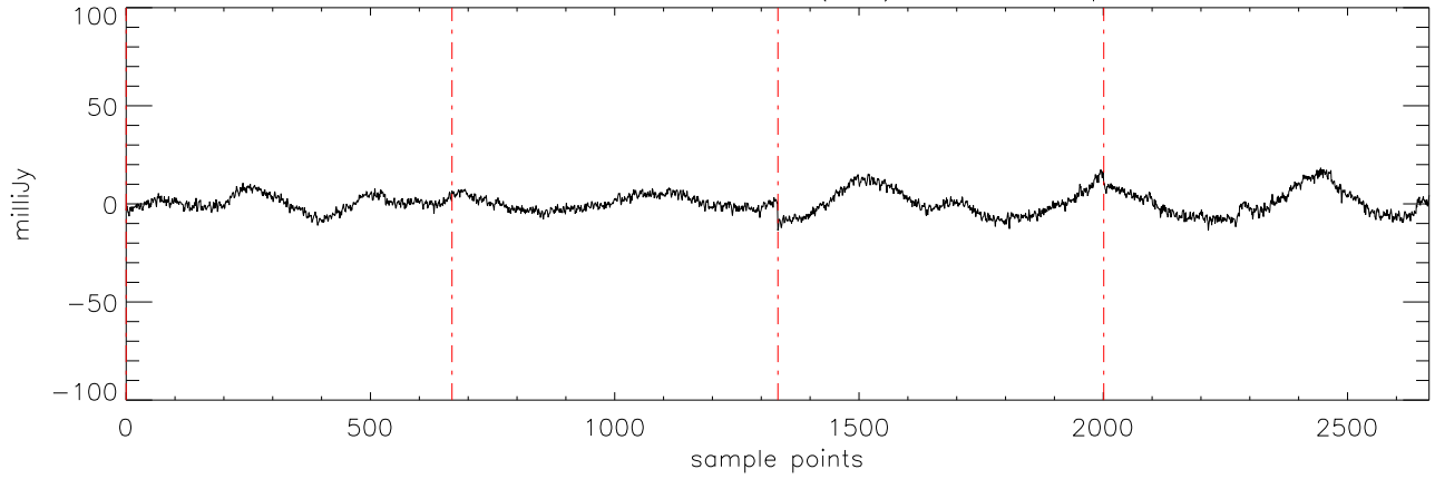
a2471 J16322911 09mar12 (AST) StokesI freq:5176.
