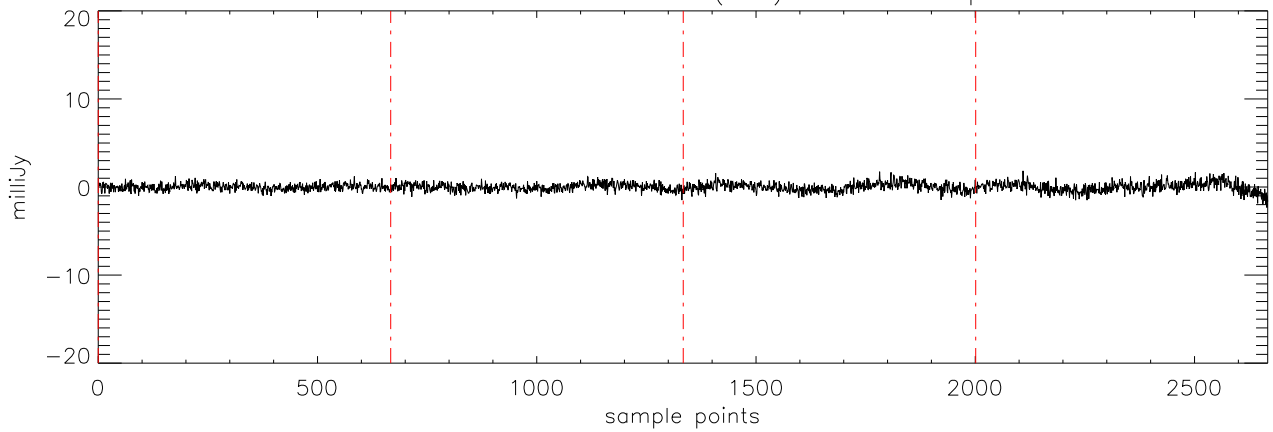
a2471 J16322911 09mar12 (AST) StokesV freq:4608.
