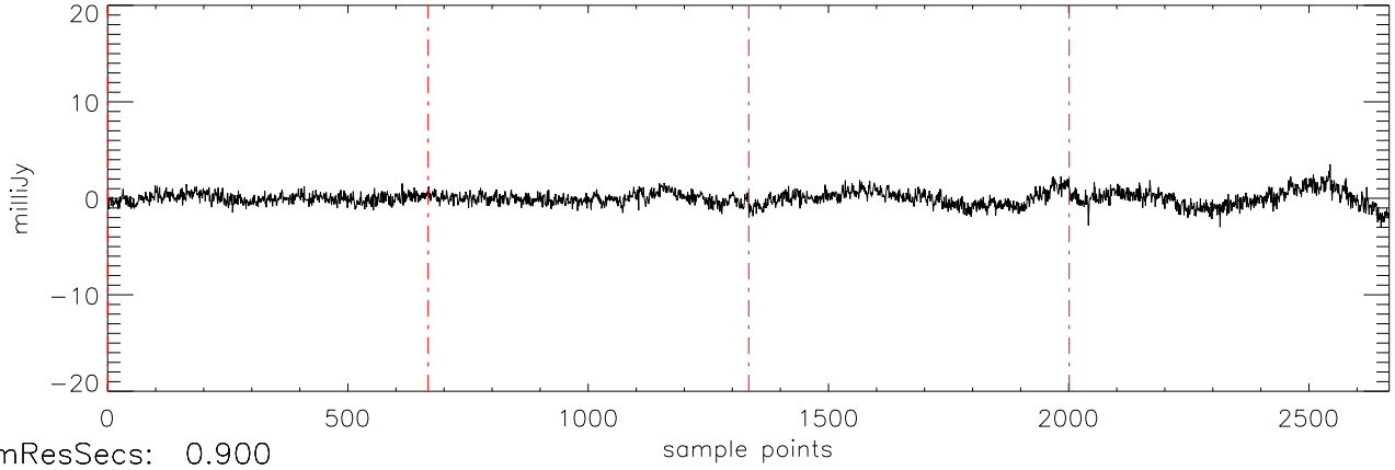
a2471 J16322911 09mar12 (AST) StokesU freq:5034.
