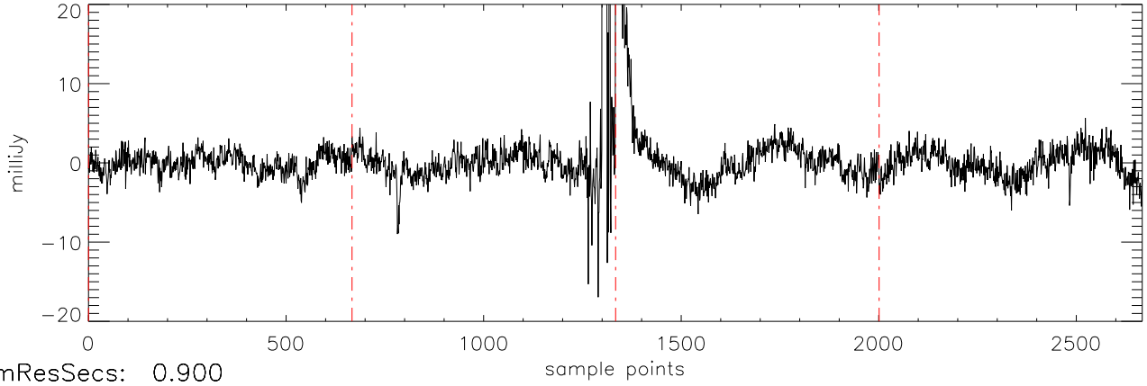
a2471 J16322911 09mar12 (AST) StokesQ freq:4466.
