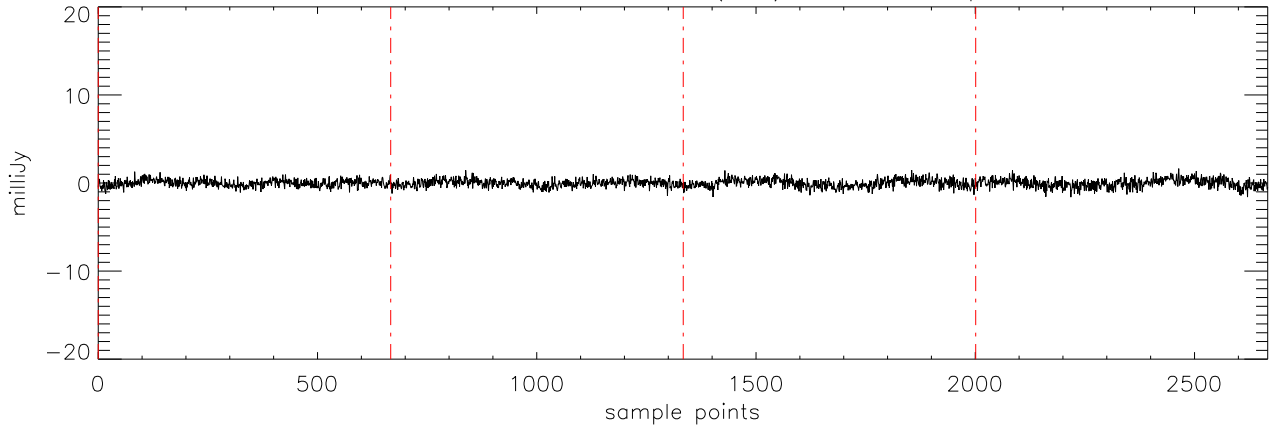
a2471 J16322911 09mar12 (AST) StokesV freq:4750.
