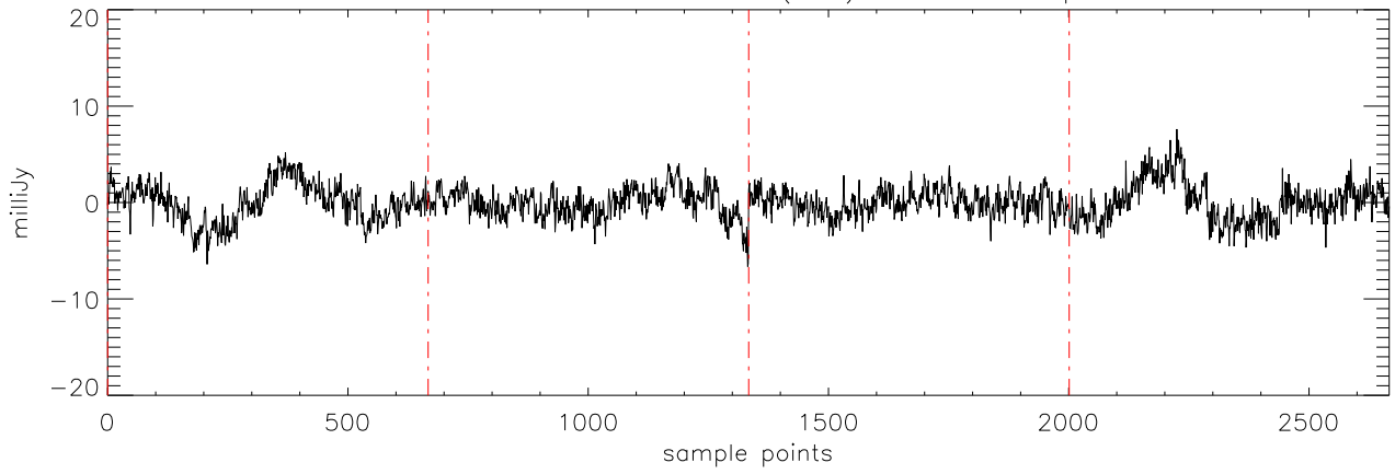
a2471 J16322911 09mar12 (AST) StokesQ freq:5176.
