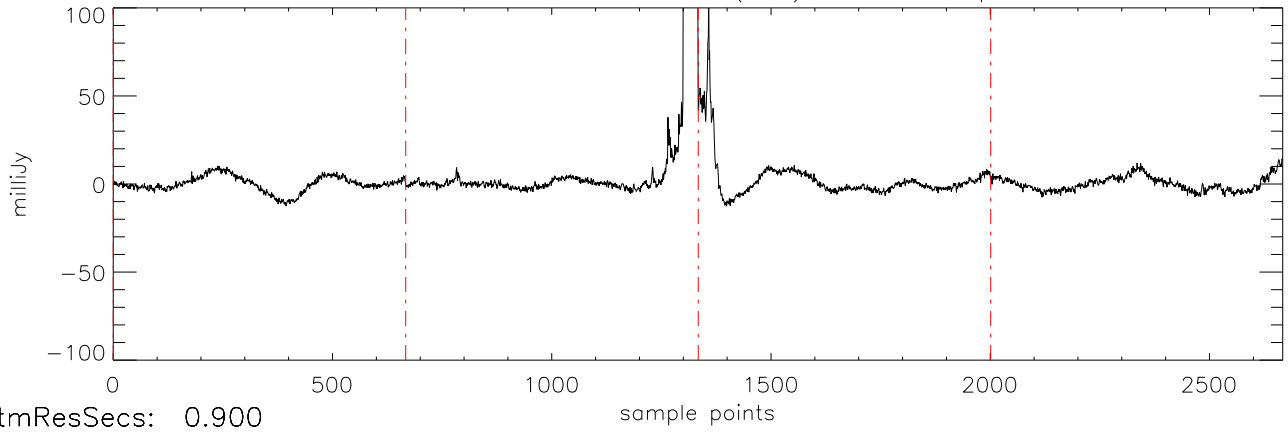
a2471 J16322911 09mar12 (AST) StokesI freq:4466.
