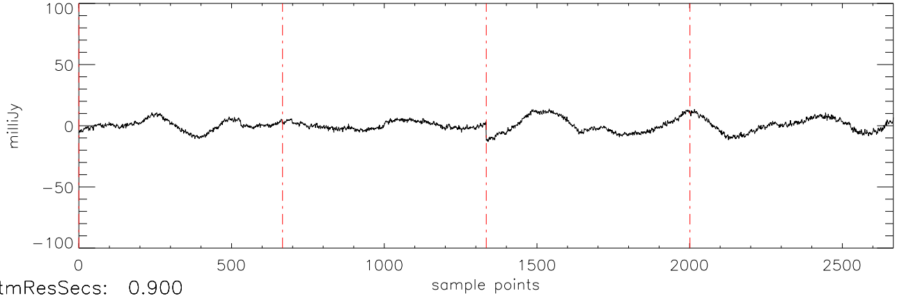
a2471 J16322911 09mar12 (AST) StokesI freq:5034.
