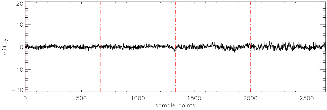
a2471 J16322911 09mar12 (AST) StokesV freq:5176.
