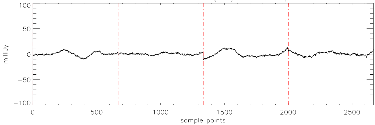
a2471 J16322911 09mar12 (AST) StokesI freq:4608.
