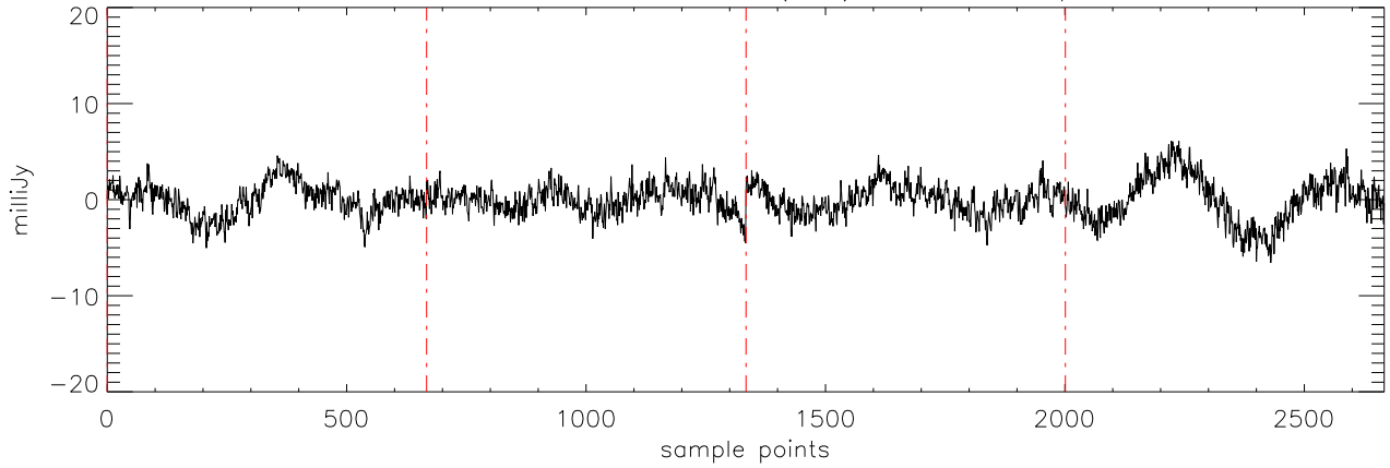
a2471 J16322911 09mar12 (AST) StokesQ freq:4750.
