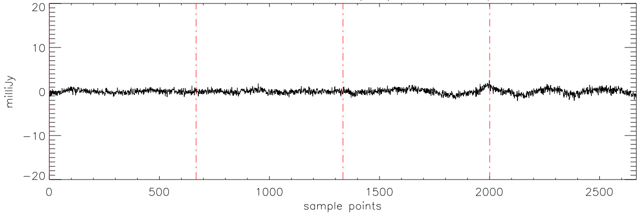
a2471 J16322911 09mar12 (AST) StokesU freq:4750.
