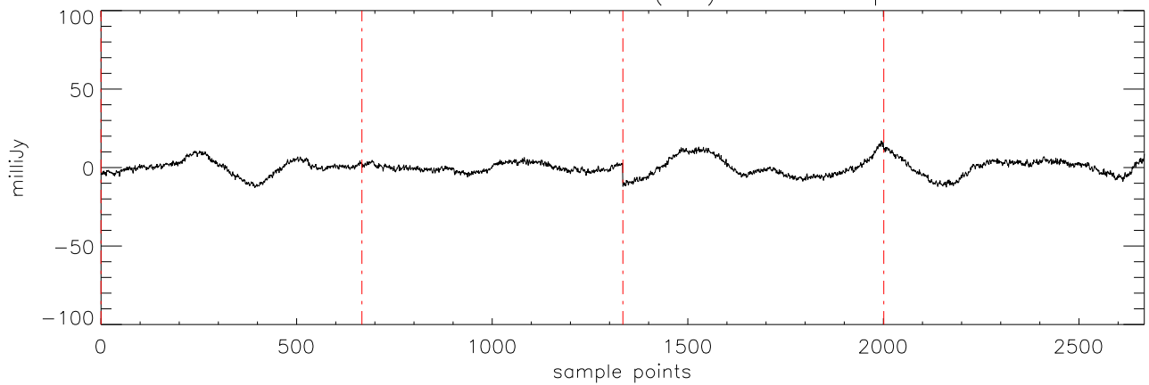
a2471 J16322911 09mar12 (AST) StokesI freq:4750.
