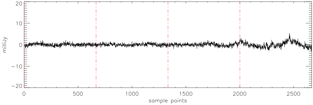
a2471 J16322911 09mar12 (AST) StokesU freq:5176.
