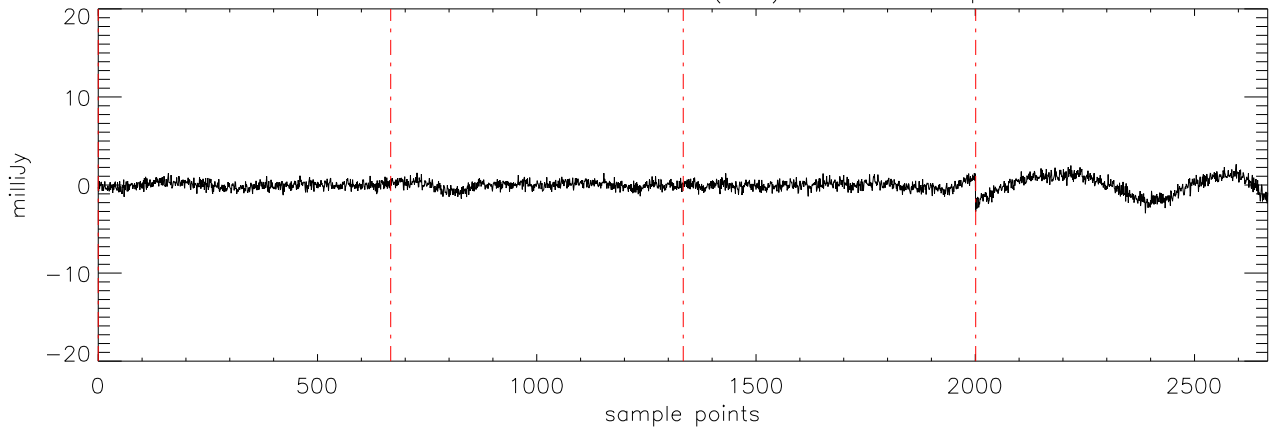
a2471 J16322911 09mar12 (AST) StokesU freq:4608.
