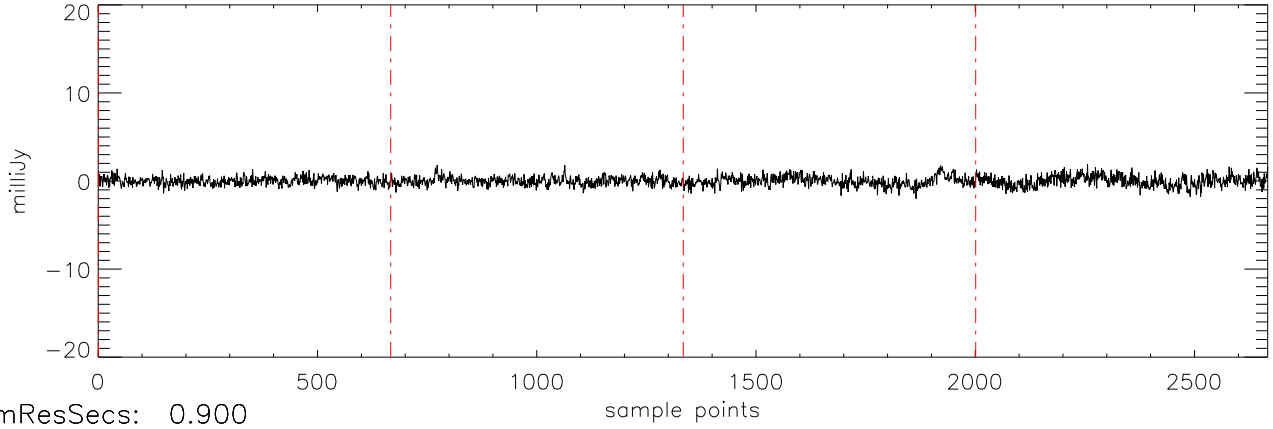
a2471 J16322911 09mar12 (AST) StokesV freq:5034.
