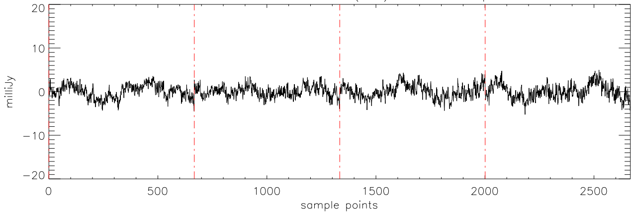
a2471 J16322911 09mar12 (AST) StokesQ freq:4608.
