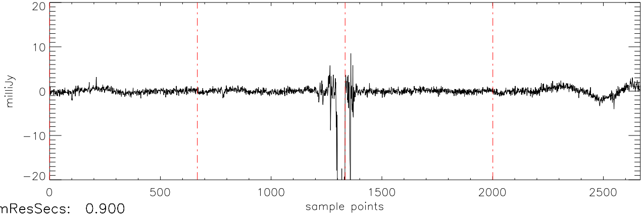
a2471 J16322911 09mar12 (AST) StokesU freq:4466.
