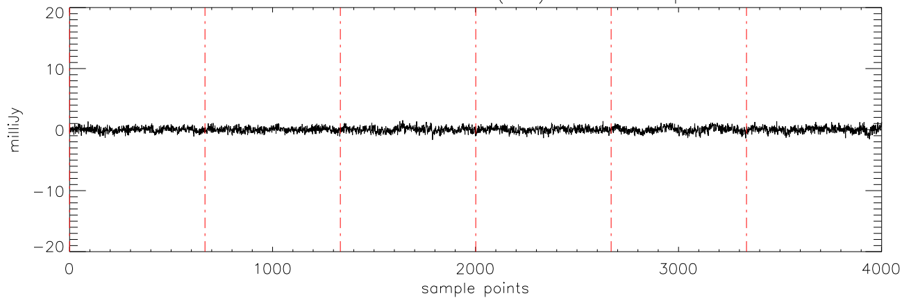
a2471 J16322911 15mar11 (AST) StokesV freq:4750.
