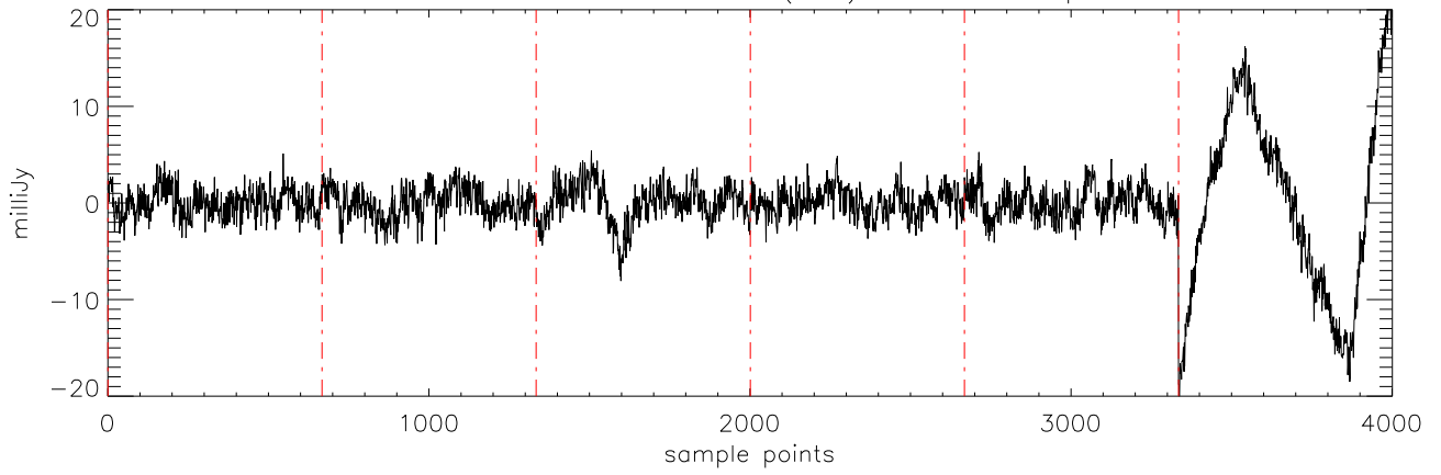
a2471 J16322911 15mar11 (AST) StokesQ freq:5176.
