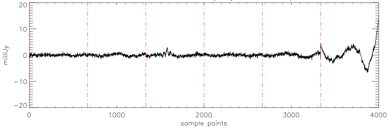
a2471 J16322911 15mar11 (AST) StokesU freq:4608.
