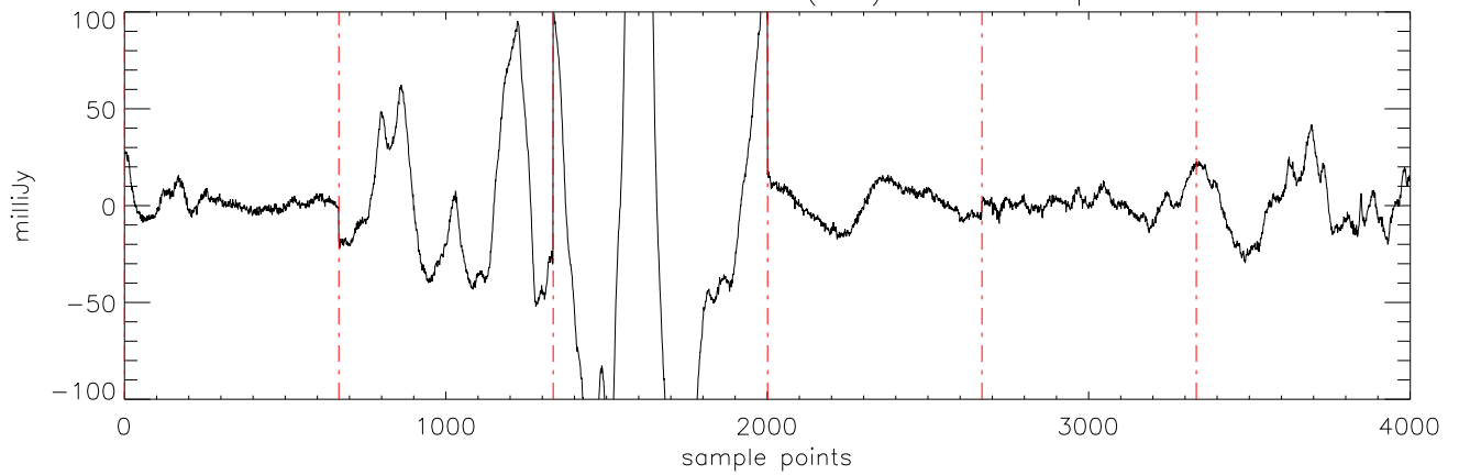
a2471 J16322911 15mar11 (AST) StokesI freq:5176.
