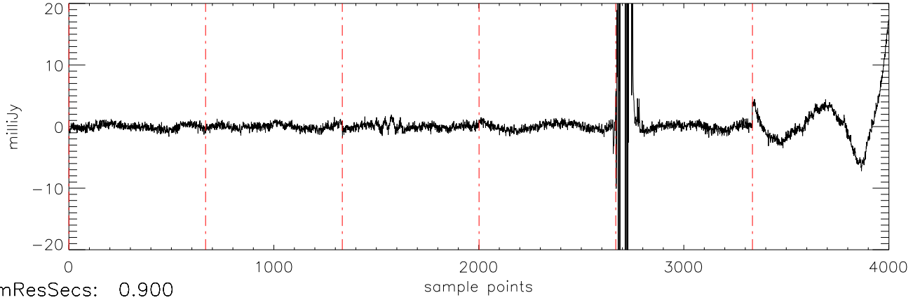
a2471 J16322911 15mar11 (AST) StokesU freq:4466.
