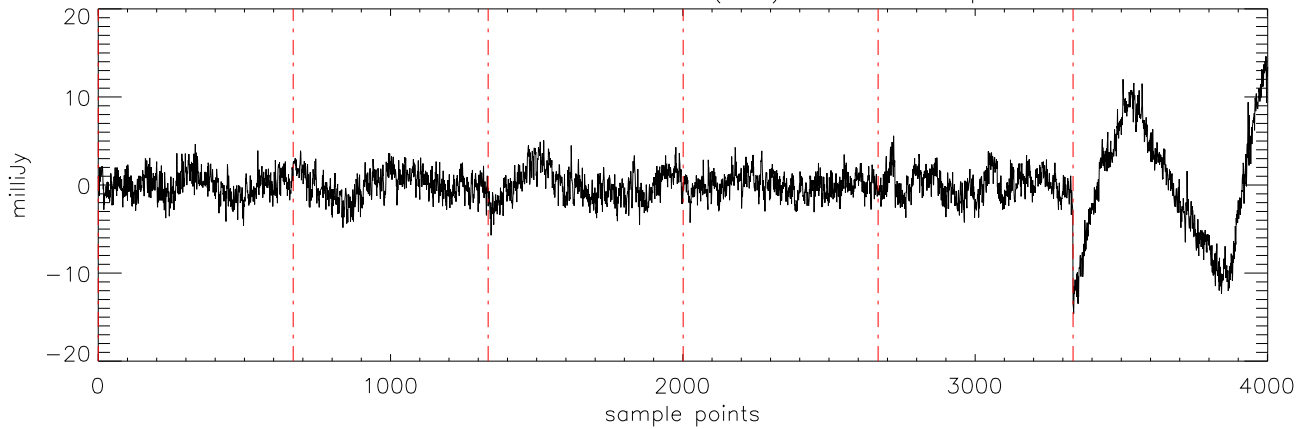
a2471 J16322911 15mar11 (AST) StokesQ freq:4750.
