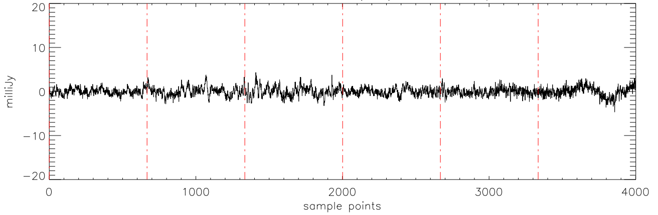
a2471 J16322911 15mar11 (AST) StokesV freq:5176.
