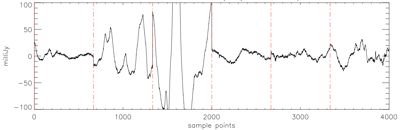
a2471 J16322911 15mar11 (AST) StokesI freq:4750.
