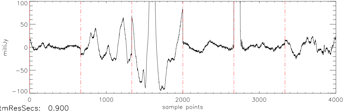
a2471 J16322911 15mar11 (AST) StokesI freq:4466.
