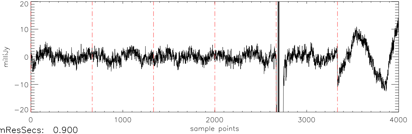
a2471 J16322911 15mar11 (AST) StokesQ freq:4466.
