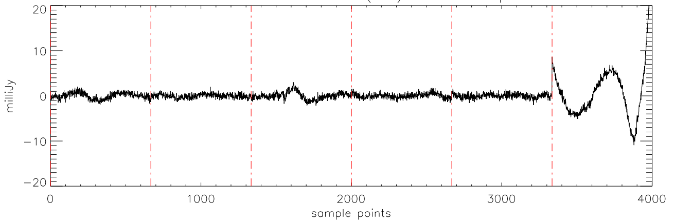
a2471 J16322911 15mar11 (AST) StokesU freq:5176.
