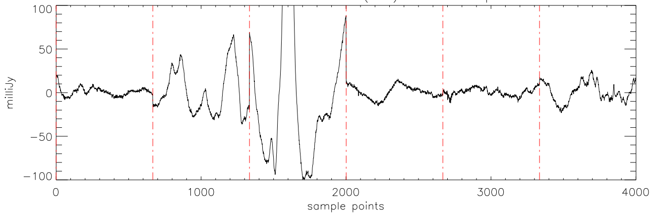
a2471 J16322911 15mar11 (AST) StokesI freq:4608.
