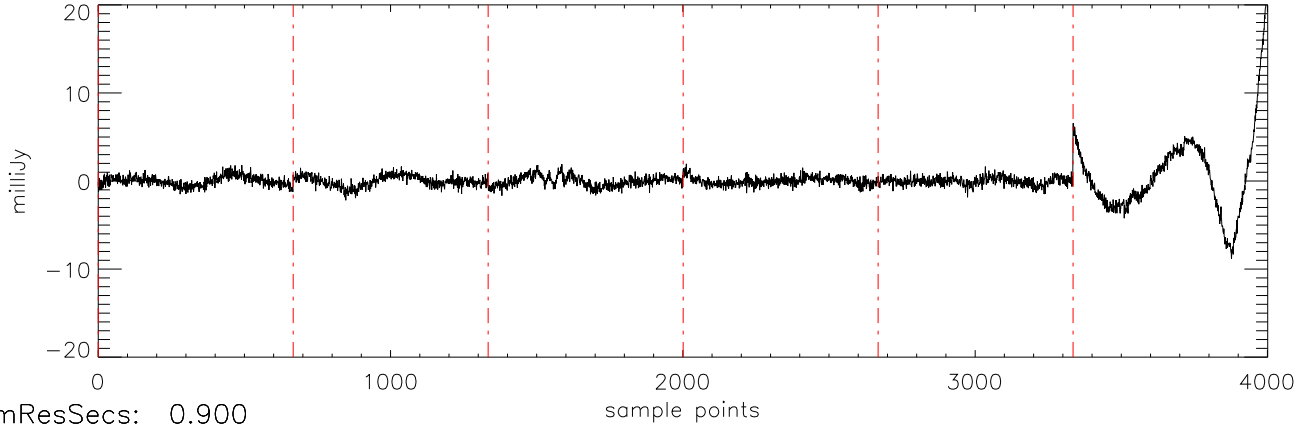
a2471 J16322911 15mar11 (AST) StokesU freq:5034.
