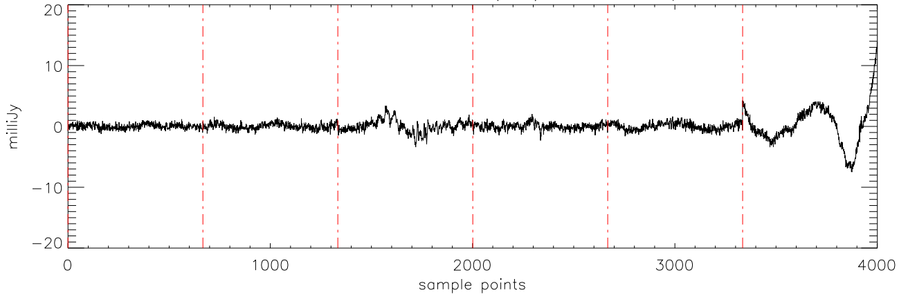
a2471 J16322911 15mar11 (AST) StokesU freq:4750.
