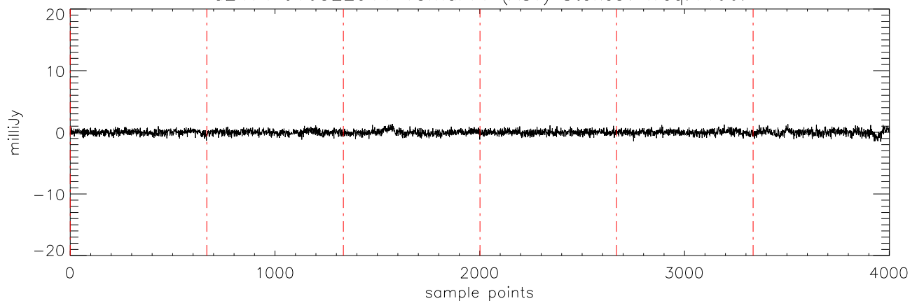
a2471 J16322911 15mar11 (AST) StokesV freq:4608.
