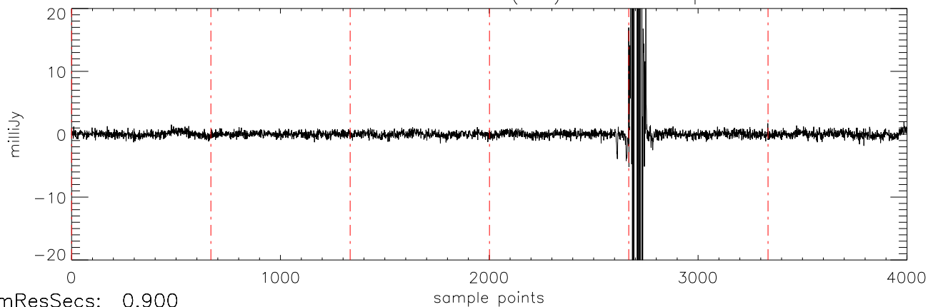
a2471 J16322911 15mar11 (AST) StokesV freq:4466.
