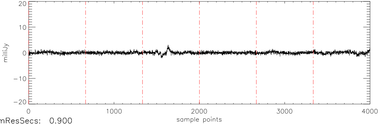
a2471 J16322911 15mar11 (AST) StokesV freq:5034.
