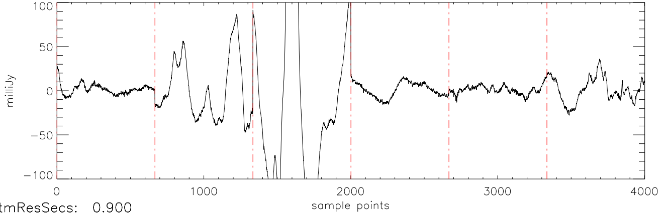
a2471 J16322911 15mar11 (AST) StokesI freq:5034.
