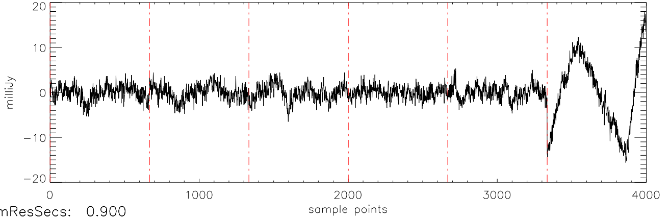
a2471 J16322911 15mar11 (AST) StokesQ freq:5034.
