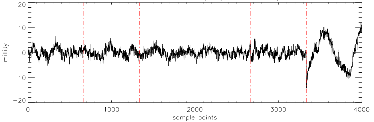
a2471 J16322911 15mar11 (AST) StokesQ freq:4608.
