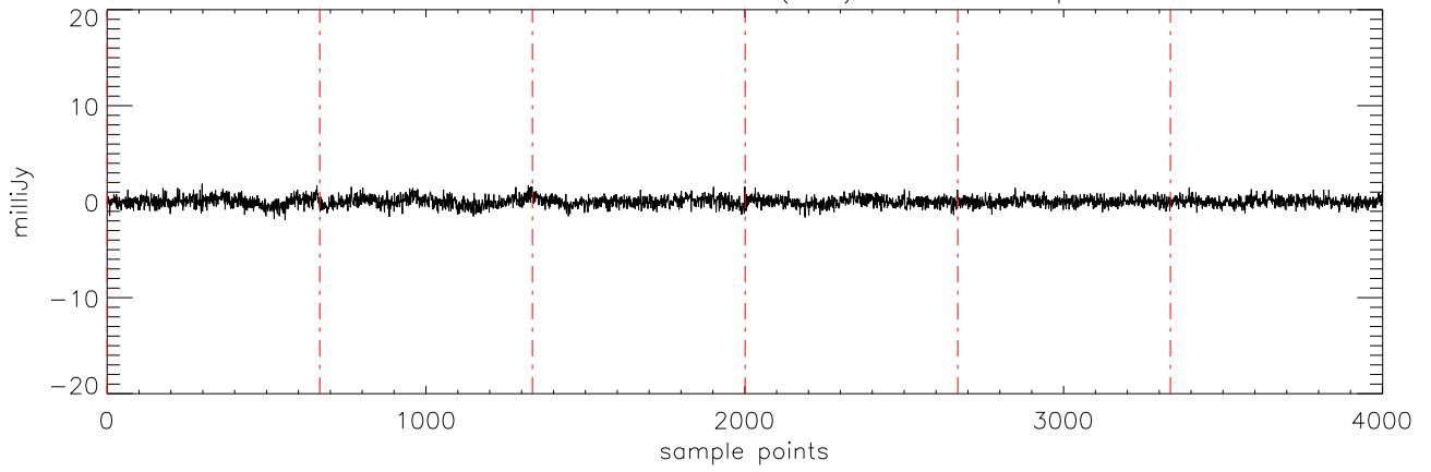
a2471 J15232263 15mar11 (AST) StokesV freq:5176.
