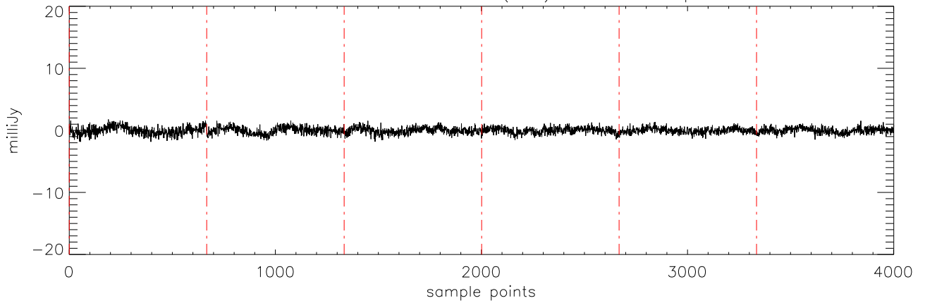
a2471 J15232263 15mar11 (AST) StokesU freq:5176.
