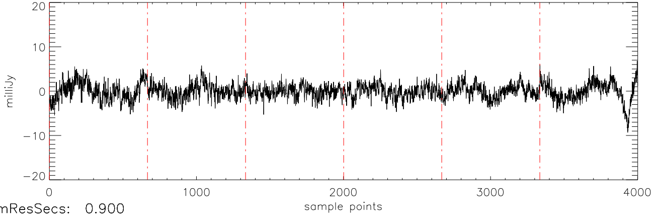
a2471 J15232263 15mar11 (AST) StokesQ freq:5034.
