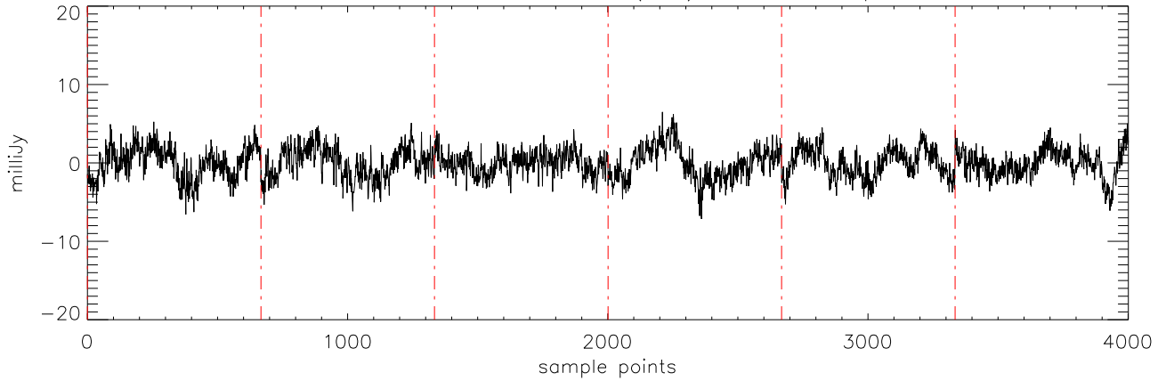
a2471 J15232263 15mar11 (AST) StokesQ freq:4608.
