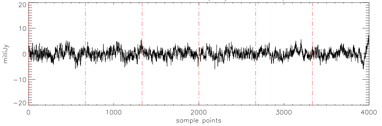
a2471 J15232263 15mar11 (AST) StokesQ freq:5176.
