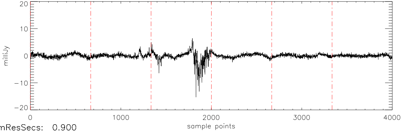
a2471 J15232263 15mar11 (AST) StokesU freq:4466.
