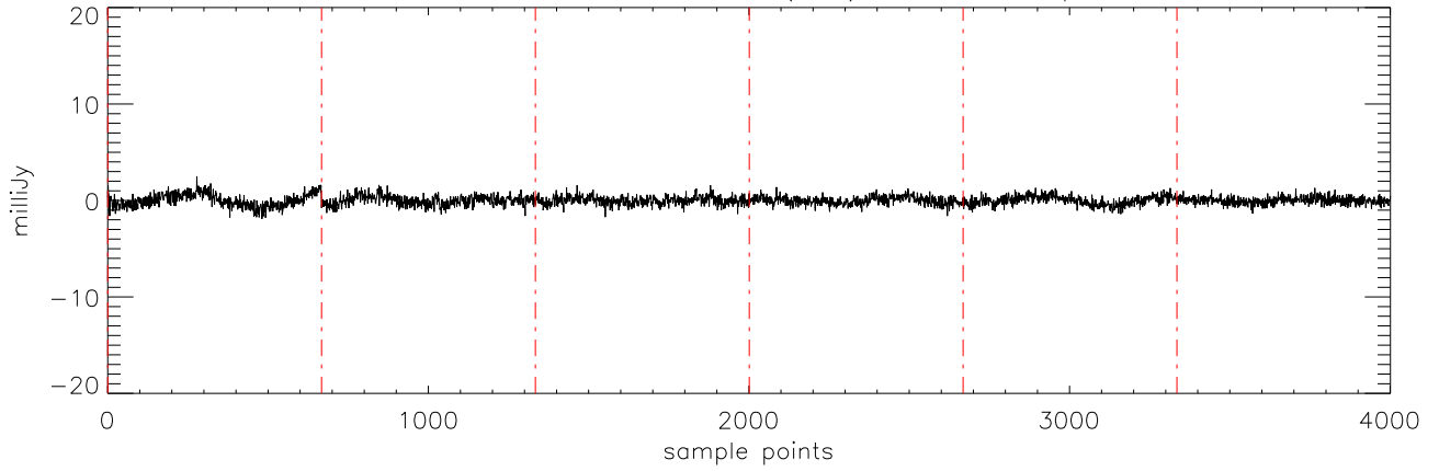
a2471 J15232263 15mar11 (AST) StokesV freq:4750.
