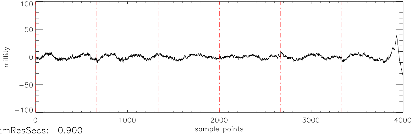
a2471 J15232263 15mar11 (AST) StokesI freq:5034.
