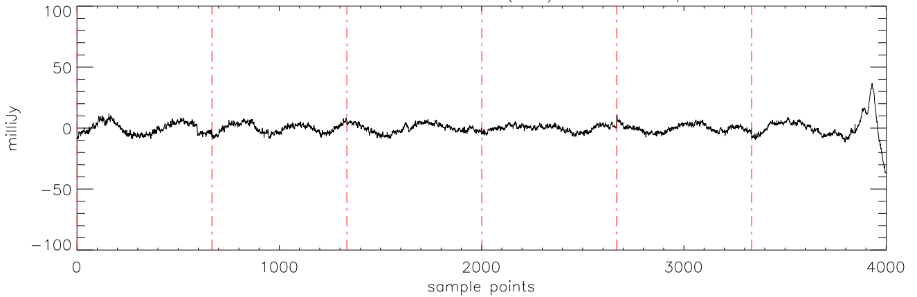
a2471 J15232263 15mar11 (AST) StokesI freq:4750.
