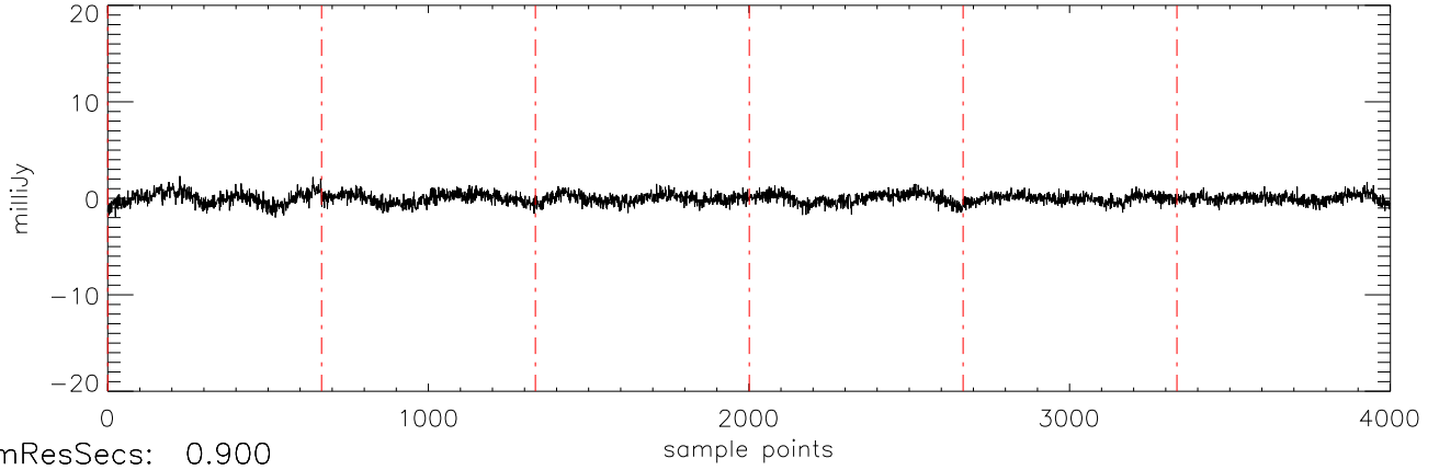
a2471 J15232263 15mar11 (AST) StokesU freq:5034.
