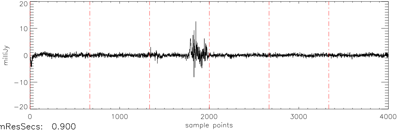
a2471 J15232263 15mar11 (AST) StokesV freq:4466.
