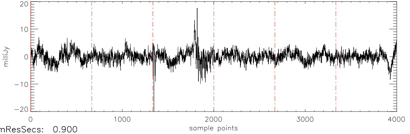
a2471 J15232263 15mar11 (AST) StokesQ freq:4466.
