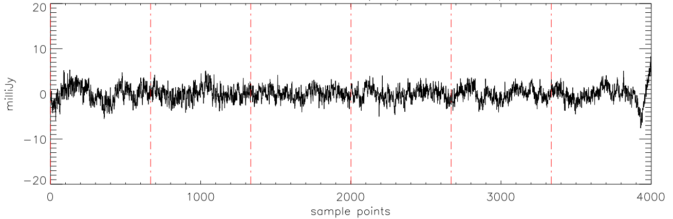
a2471 J15232263 15mar11 (AST) StokesQ freq:4750.
