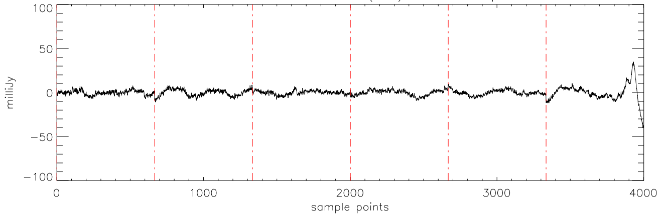
a2471 J15232263 15mar11 (AST) StokesI freq:5176.
