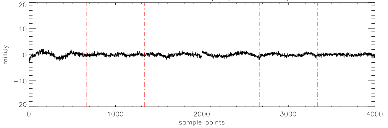
a2471 J15232263 15mar11 (AST) StokesU freq:4608.
