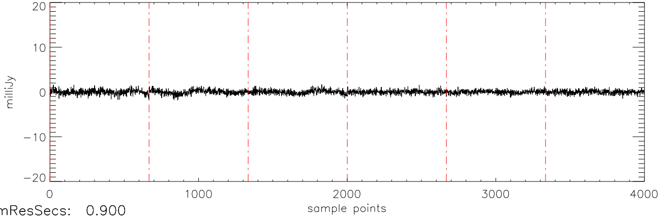
a2471 J15232263 15mar11 (AST) StokesV freq:5034.
