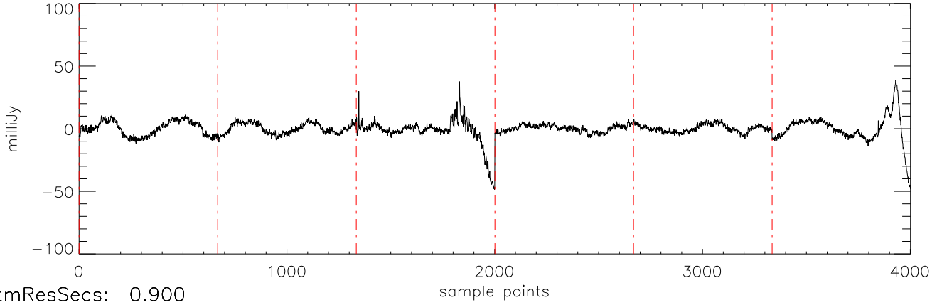
a2471 J15232263 15mar11 (AST) StokesI freq:4466.
