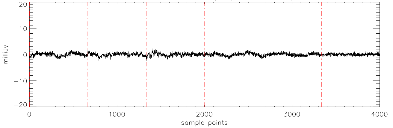
a2471 J15232263 15mar11 (AST) StokesU freq:4750.
