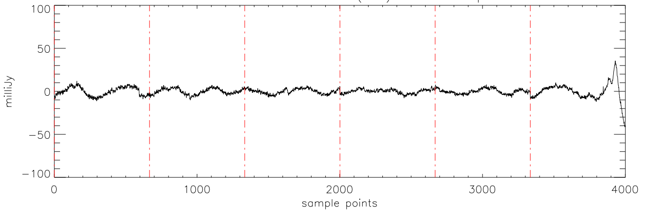
a2471 J15232263 15mar11 (AST) StokesI freq:4608.
