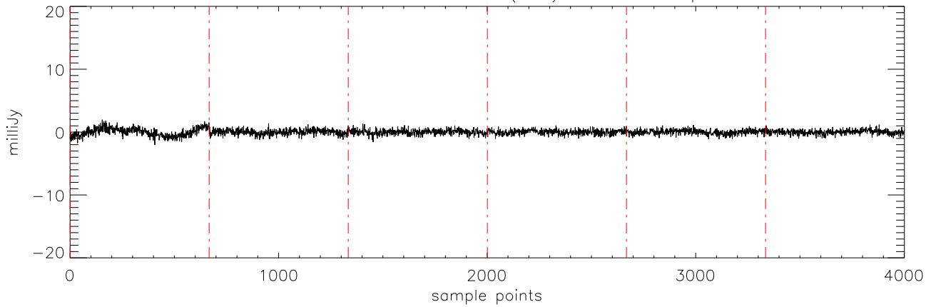
a2471 J15232263 15mar11 (AST) StokesV freq:4608.
