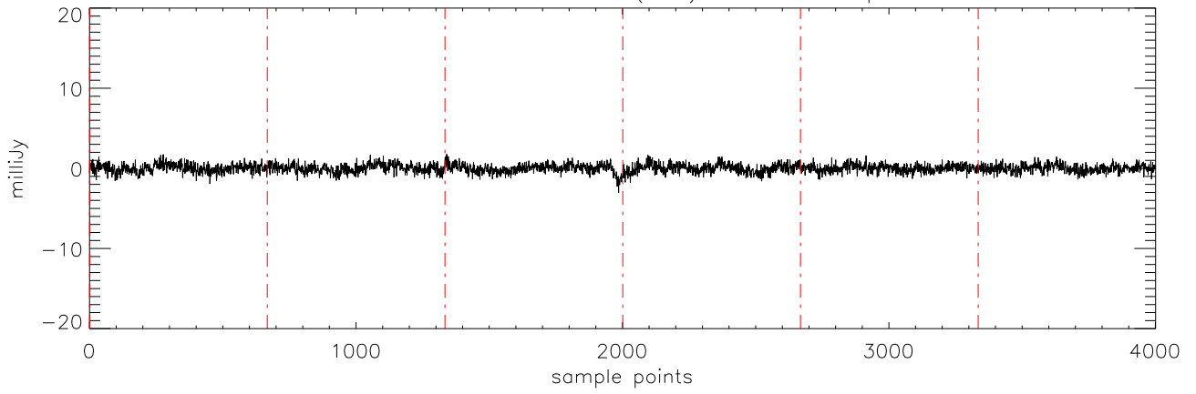
a2471 J144601 16mar11 (AST) StokesV freq:5176.
