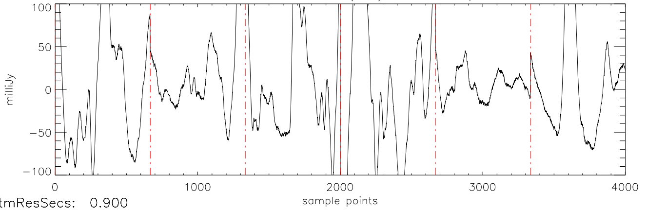
a2471 J144601 16mar11 (AST) StokesI freq:5034.
