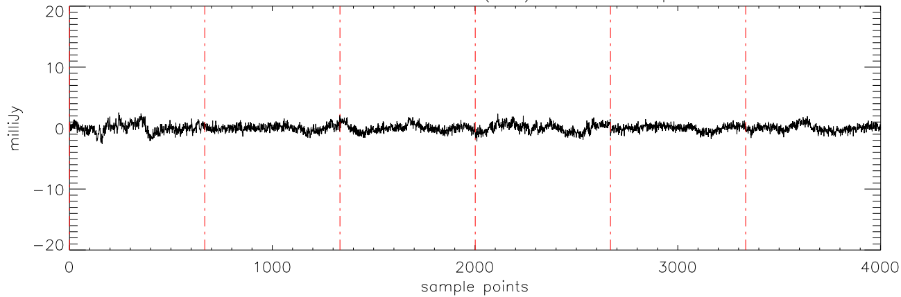
a2471 J144601 16mar11 (AST) StokesU freq:4750.
