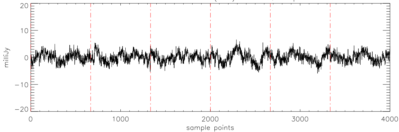
a2471 J144601 16mar11 (AST) StokesQ freq:4750.
