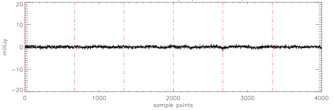
a2471 J144601 16mar11 (AST) StokesV freq:4608.
