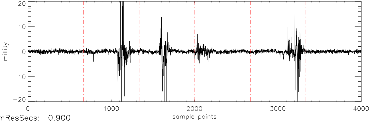
a2471 J144601 16mar11 (AST) StokesV freq:4466.
