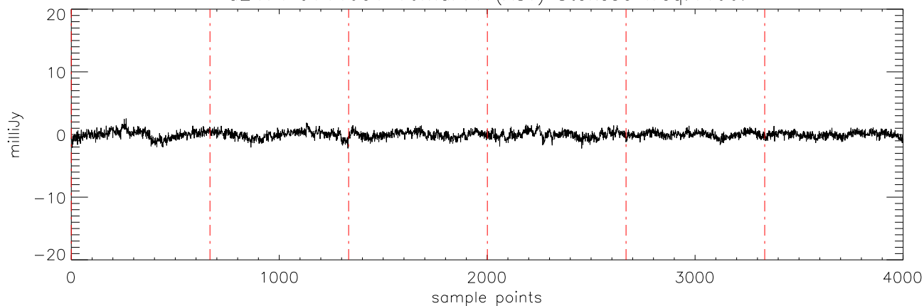
a2471 J144601 16mar11 (AST) StokesU freq:4608.
