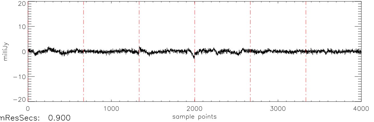
a2471 J144601 16mar11 (AST) StokesV freq:5034.
