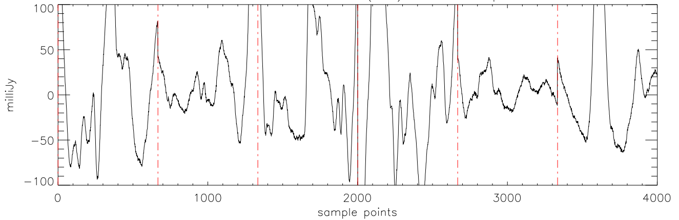
a2471 J144601 16mar11 (AST) StokesI freq:4750.
