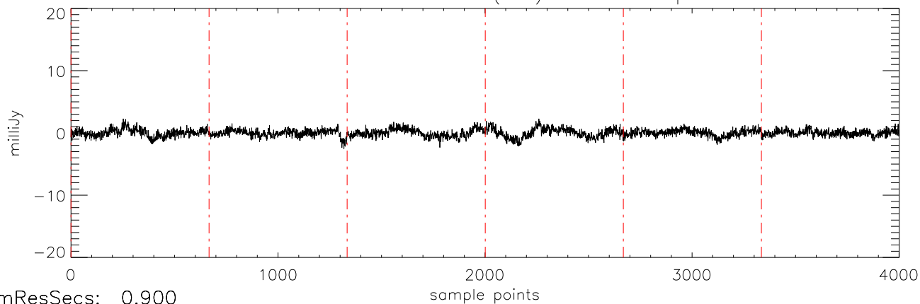
a2471 J144601 16mar11 (AST) StokesU freq:5034.
