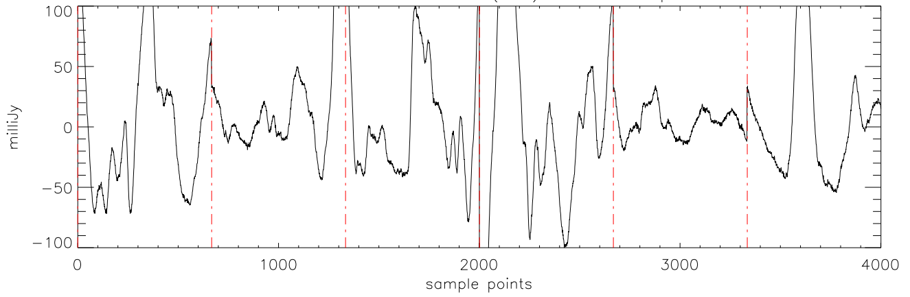
a2471 J144601 16mar11 (AST) StokesI freq:4608.
