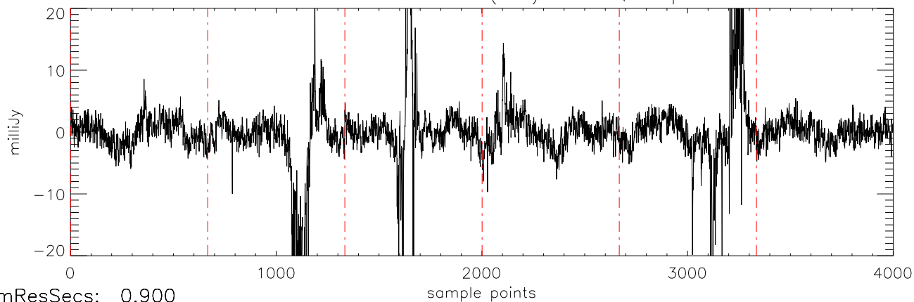
a2471 J144601 16mar11 (AST) StokesQ freq:4466.
