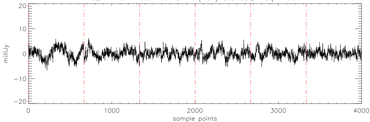
a2471 J144601 16mar11 (AST) StokesQ freq:4608.
