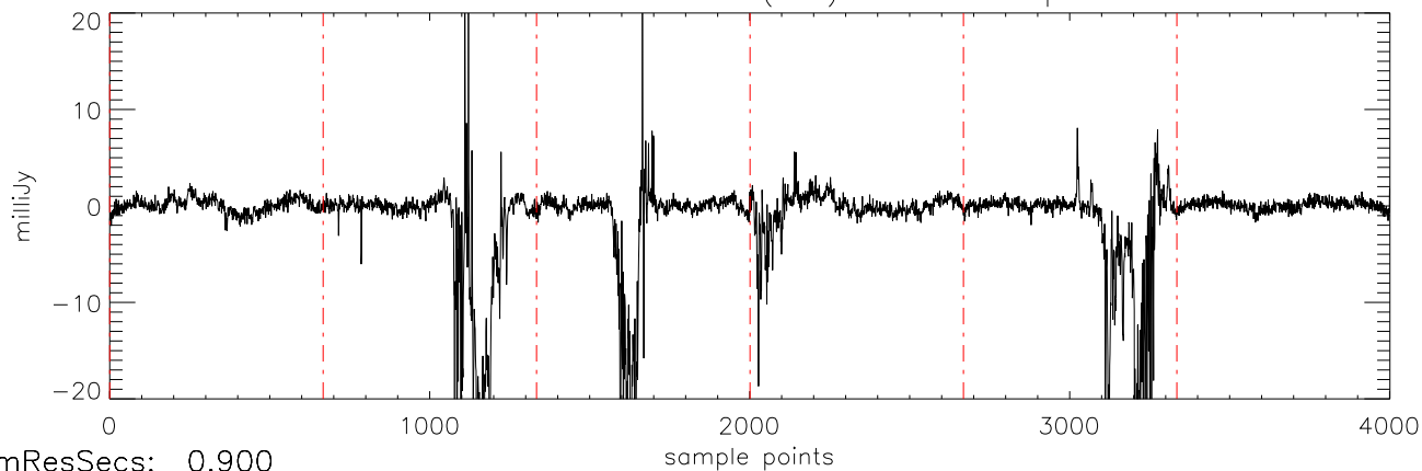
a2471 J144601 16mar11 (AST) StokesU freq:4466.
