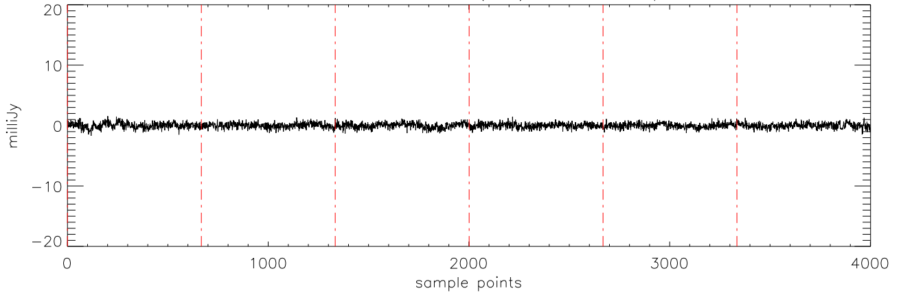
a2471 J144601 16mar11 (AST) StokesV freq:4750.
