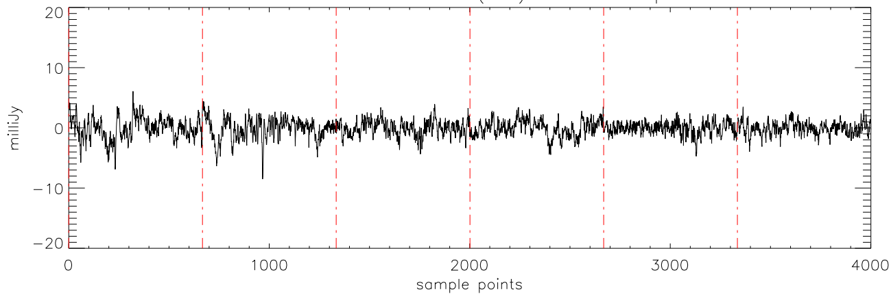
a2471 J144601 16mar11 (AST) StokesU freq:5176.
