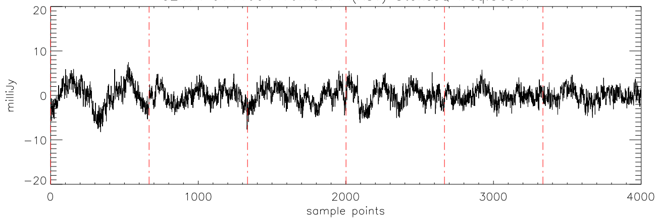
a2471 J144601 16mar11 (AST) StokesQ freq:5176.
