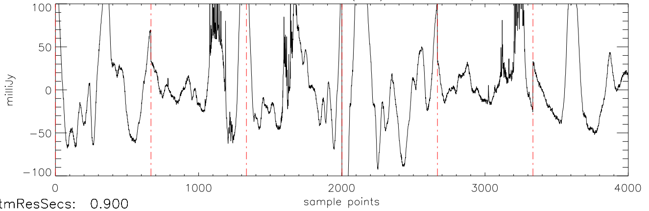
a2471 J144601 16mar11 (AST) StokesI freq:4466.
