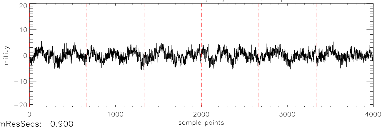
a2471 J144601 16mar11 (AST) StokesQ freq:5034.
