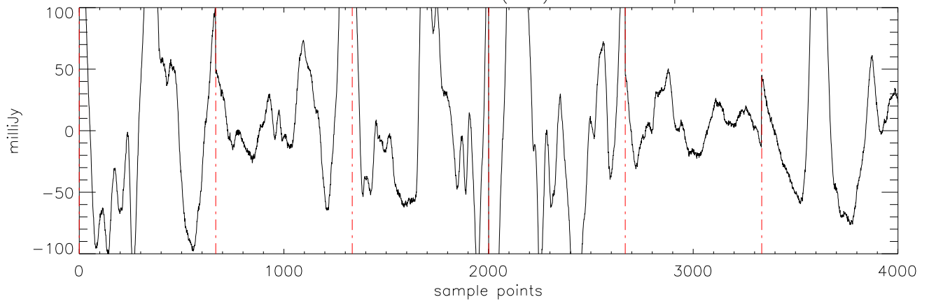
a2471 J144601 16mar11 (AST) StokesI freq:5176.
