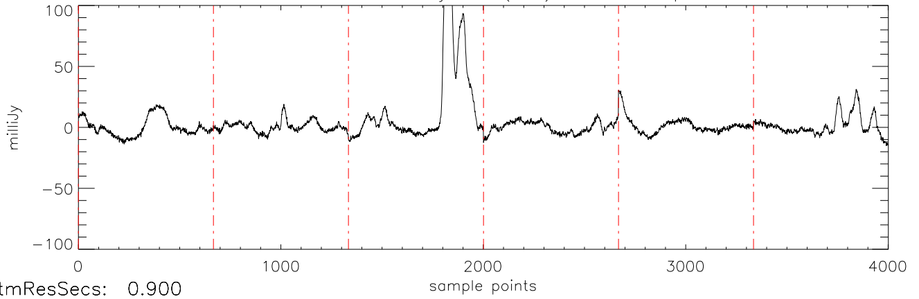
a2471 J12382851 03jan11 (AST) StokesI freq:5034.
