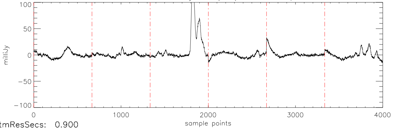
a2471 J12382851 03jan11 (AST) StokesI freq:4466.
