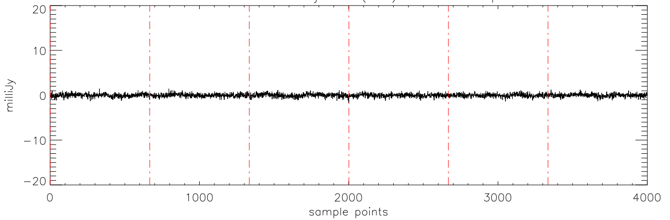
a2471 J12382851 03jan11 (AST) StokesV freq:4608.
