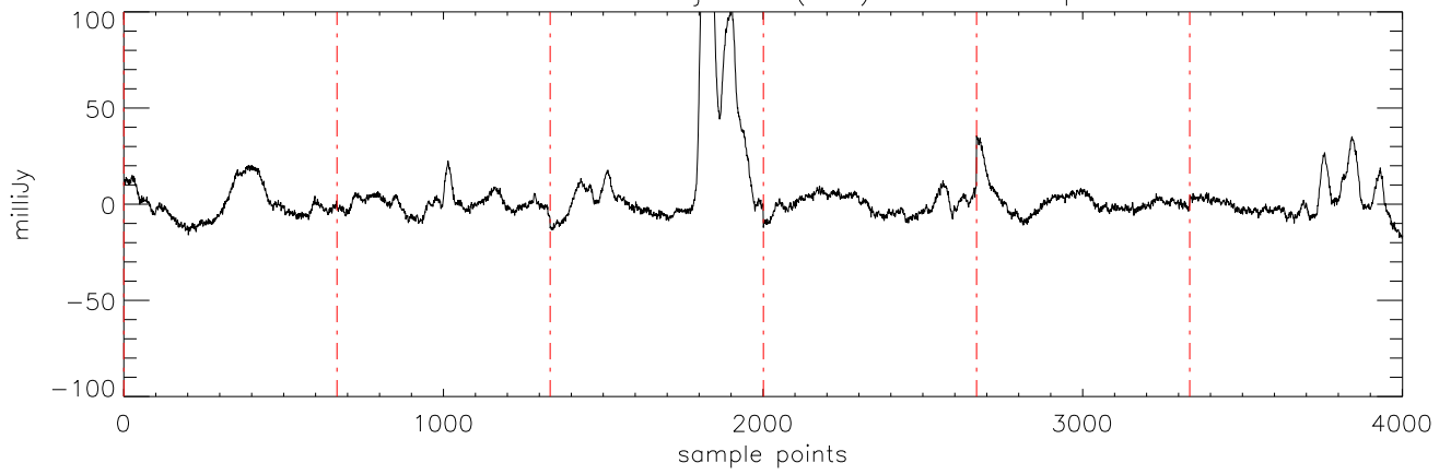
a2471 J12382851 03jan11 (AST) StokesI freq:5176.
