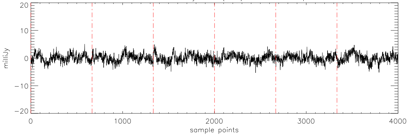
a2471 J12382851 03jan11 (AST) StokesQ freq:4608.
