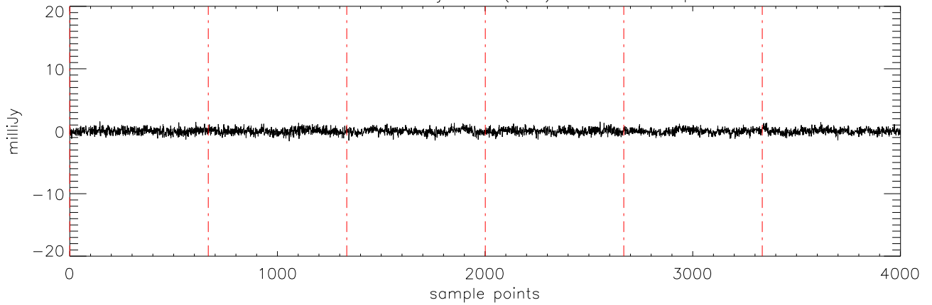
a2471 J12382851 03jan11 (AST) StokesV freq:4750.
