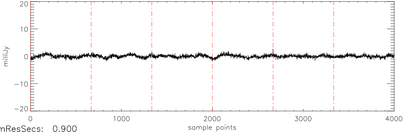
a2471 J12382851 03jan11 (AST) StokesU freq:5034.
