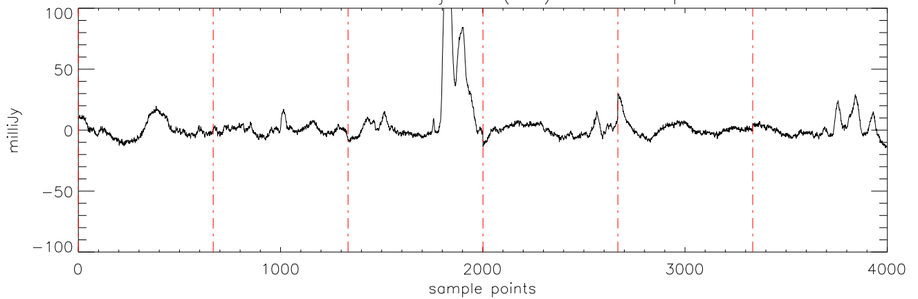
a2471 J12382851 03jan11 (AST) StokesI freq:4750.
