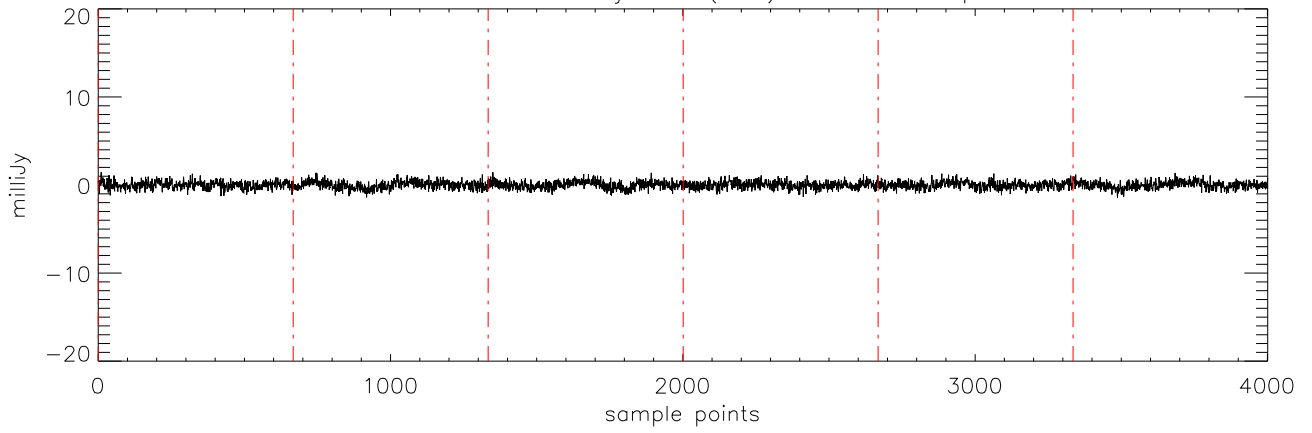
a2471 J12382851 03jan11 (AST) StokesV freq:5176.
