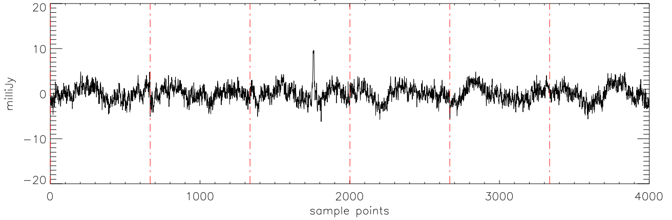
a2471 J12382851 03jan11 (AST) StokesQ freq:4750.
