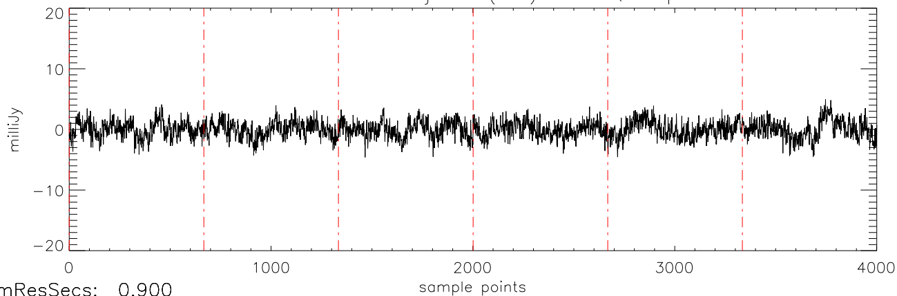
a2471 J12382851 03jan11 (AST) StokesQ freq:5034.
