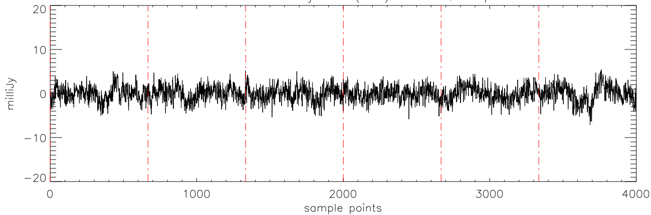
a2471 J12382851 03jan11 (AST) StokesQ freq:5176.
