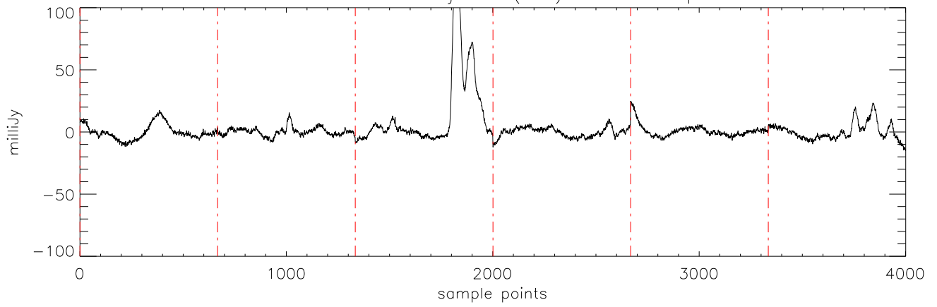
a2471 J12382851 03jan11 (AST) StokesI freq:4608.
