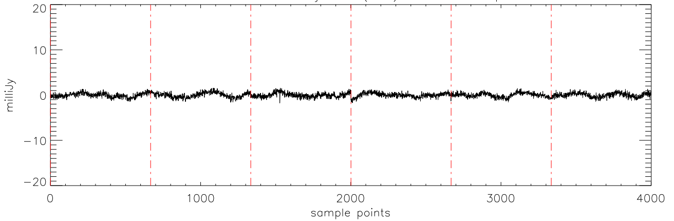
a2471 J12382851 03jan11 (AST) StokesU freq:4608.
