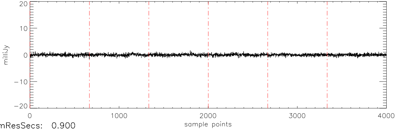
a2471 J12382851 03jan11 (AST) StokesV freq:4466.
