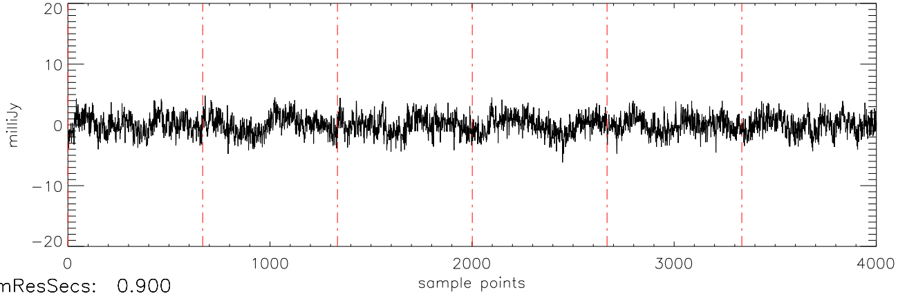
a2471 J12382851 03jan11 (AST) StokesQ freq:4466.
