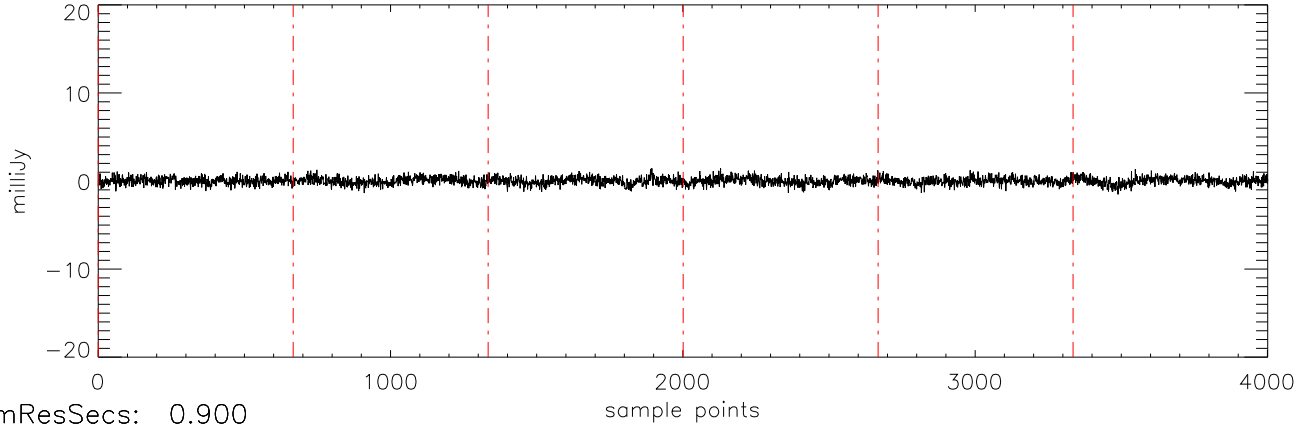
a2471 J12382851 03jan11 (AST) StokesV freq:5034.
