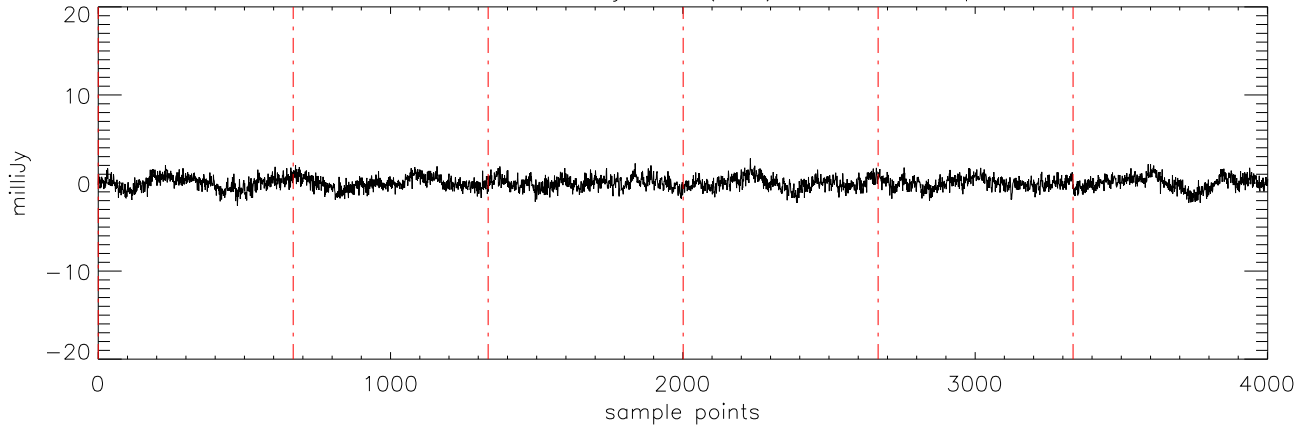
a2471 J12382851 03jan11 (AST) StokesU freq:5176.
