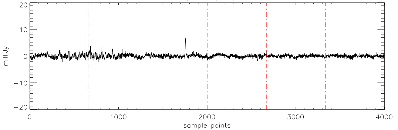
a2471 J12382851 03jan11 (AST) StokesU freq:4750.
