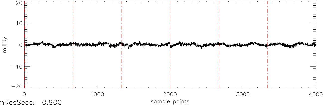
a2471 J12382851 03jan11 (AST) StokesU freq:4466.
