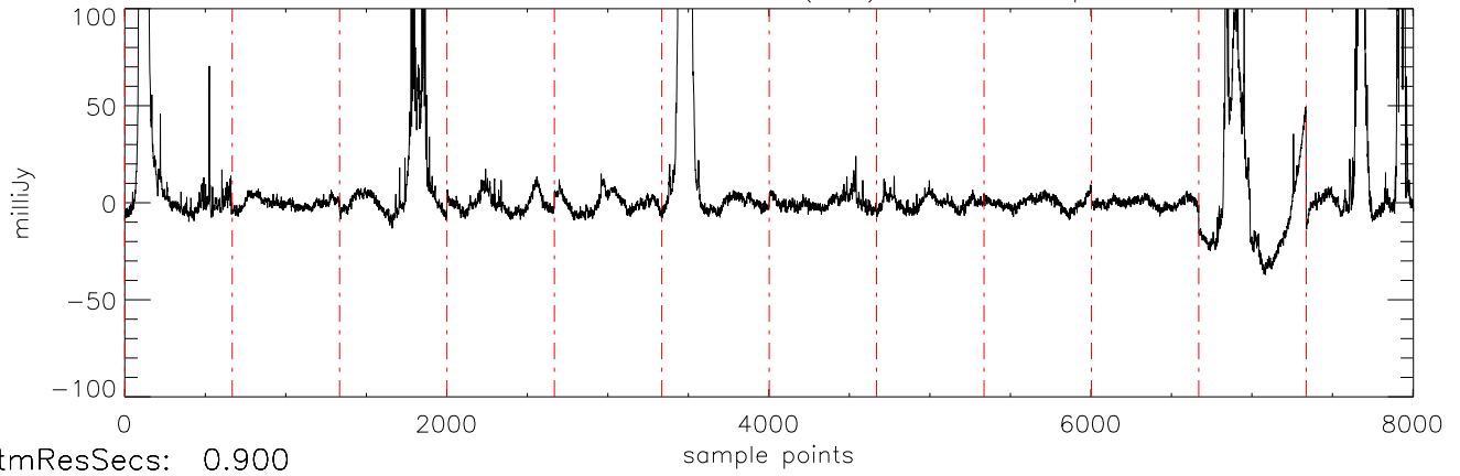
α2471 J11463449 07feb12 (AST) StokesI freq:4466.
