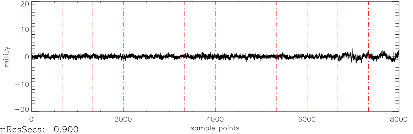
a2471 J11463449 07feb12 (AST) StokesV freq:5034.
