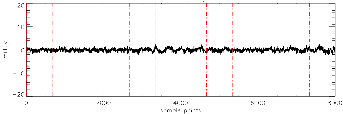
a2471 J11463449 07feb12 (AST) StokesU freq:5176.
