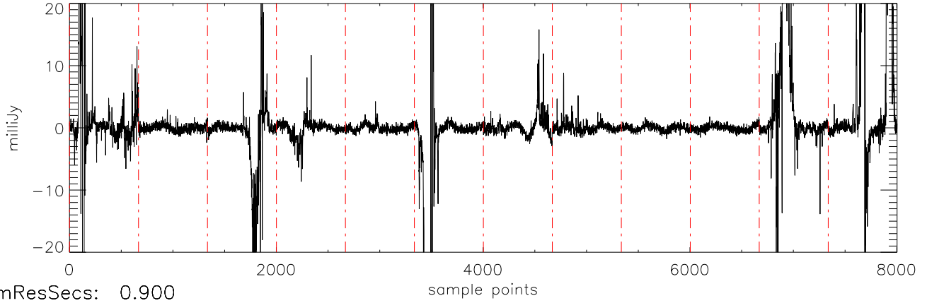
a2471 J11463449 07feb12 (AST) StokesU freq:4466.
