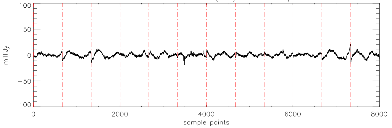
α2471 J11463449 07feb12 (AST) StokesI freq:4608.
