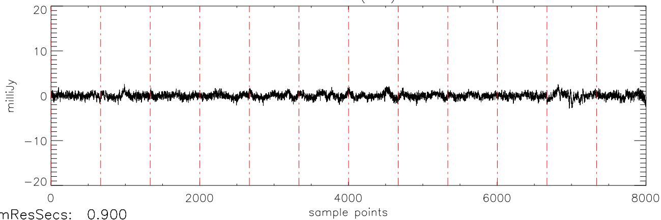
a2471 J11463449 07feb12 (AST) StokesU freq:5034.
