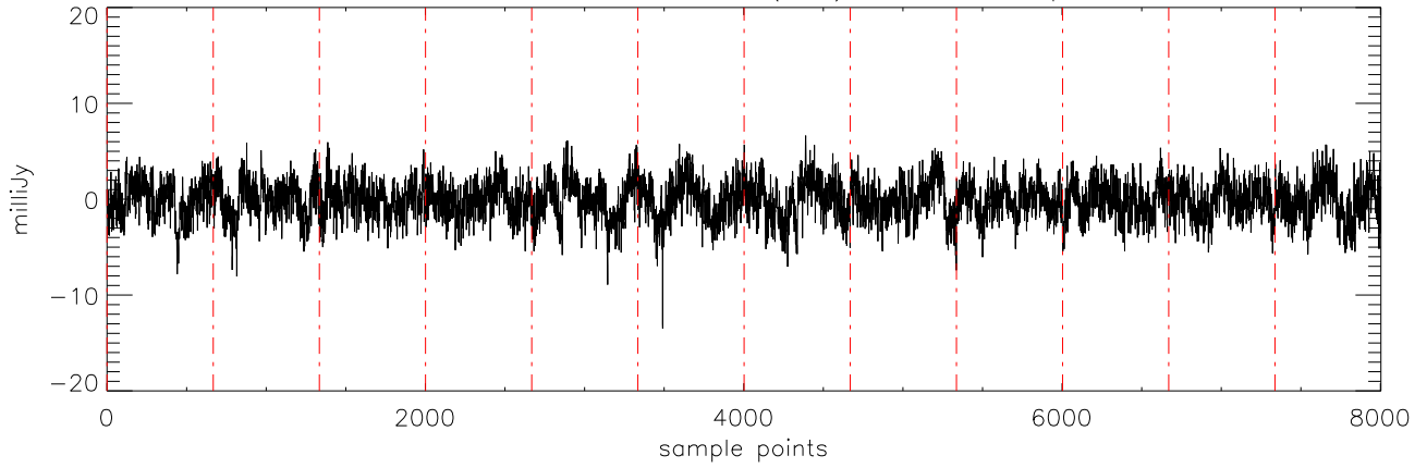
a2471 J11463449 07feb12 (AST) StokesQ freq:5176.
