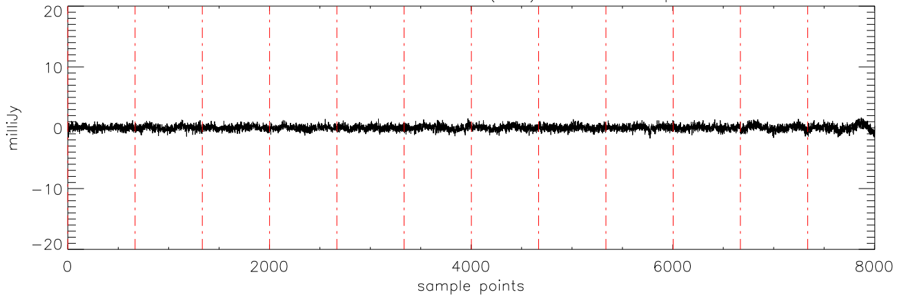
a2471 J11463449 07feb12 (AST) StokesV freq:4608.
