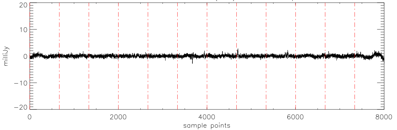
a2471 J11463449 07feb12 (AST) StokesV freq:4750.
