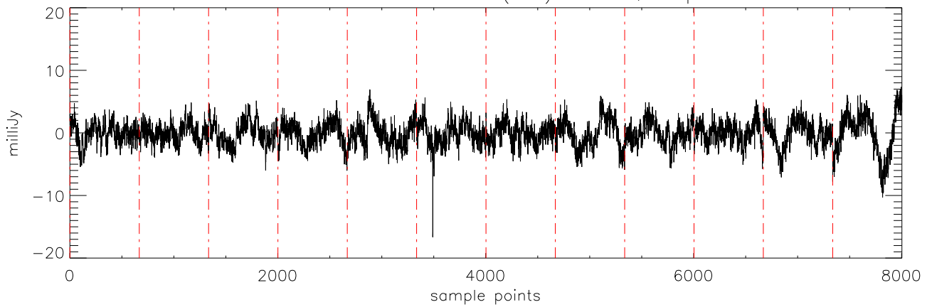
a2471 J11463449 07feb12 (AST) StokesQ freq:4608.
