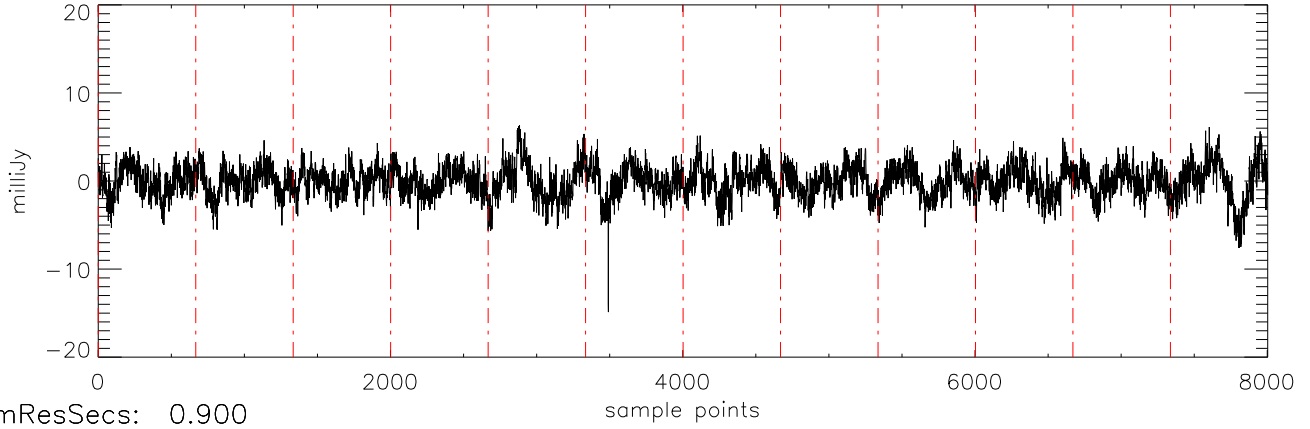
a2471 J11463449 07feb12 (AST) StokesQ freq:5034.
