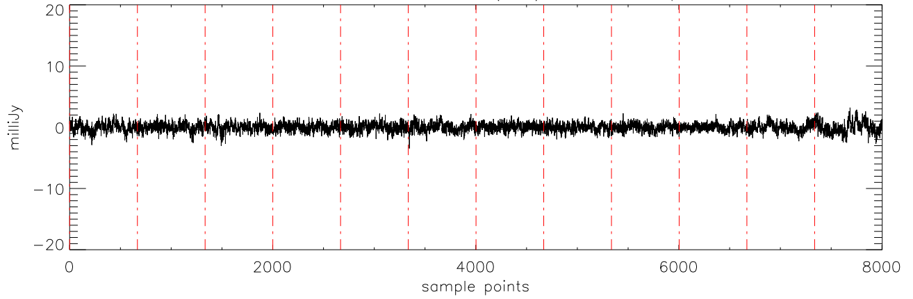
a2471 J11463449 07feb12 (AST) StokesV freq:5176.
