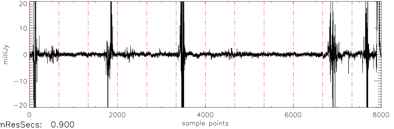
a2471 J11463449 07feb12 (AST) StokesV freq:4466.
