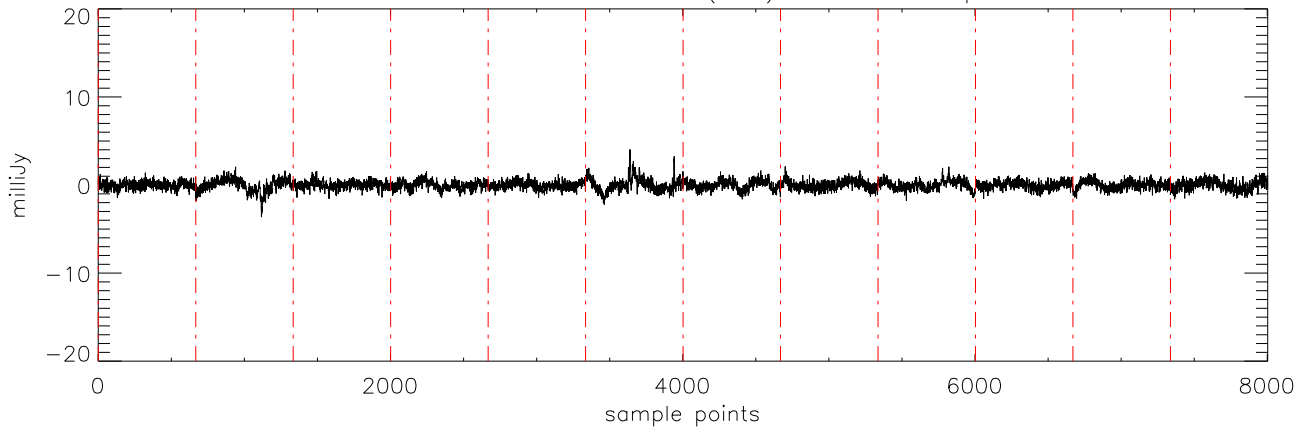
a2471 J11463449 07feb12 (AST) StokesU freq:4608.
