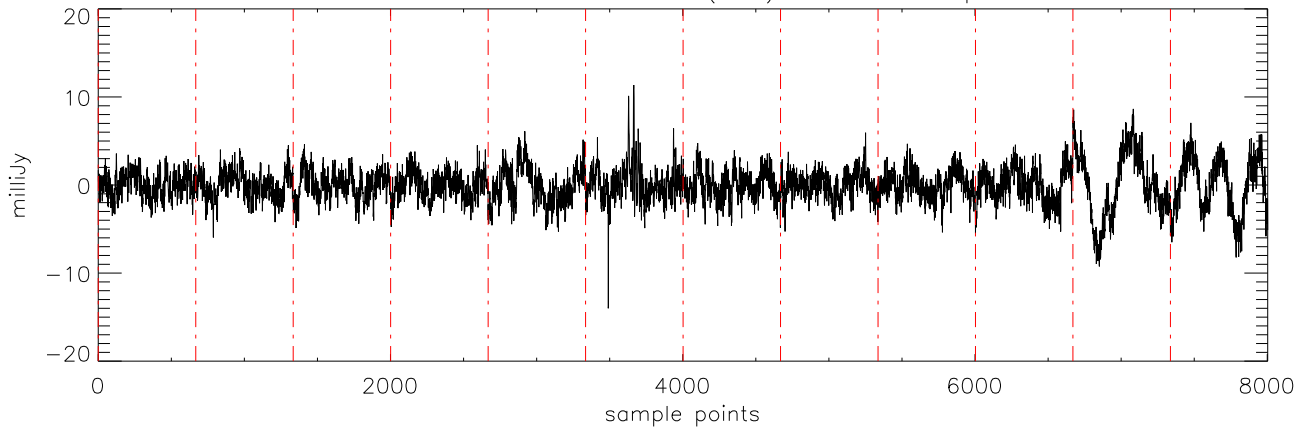
a2471 J11463449 07feb12 (AST) StokesQ freq:4750.
