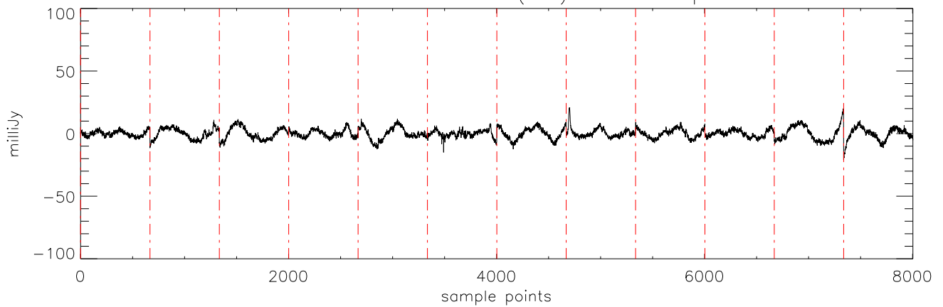
α2471 J11463449 07feb12 (AST) StokesI freq:4750.
