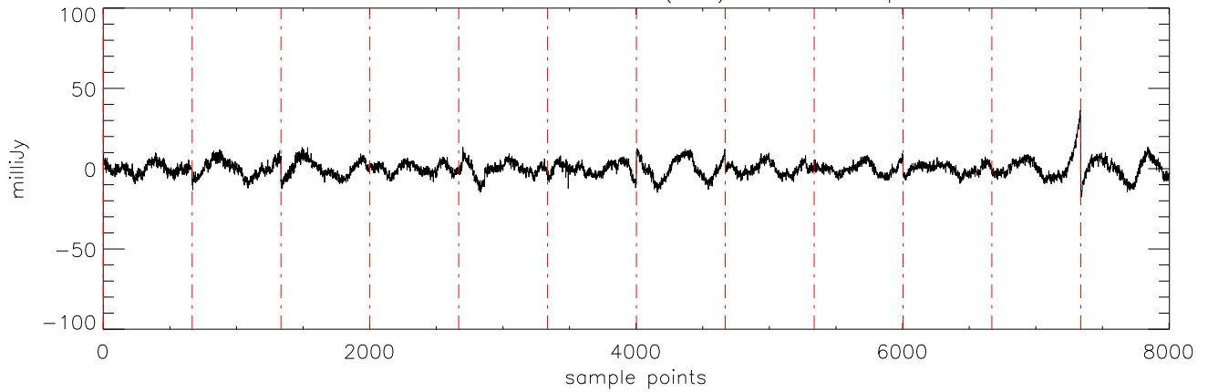
α2471 J11463449 07feb12 (AST) StokesI freq:5176.
