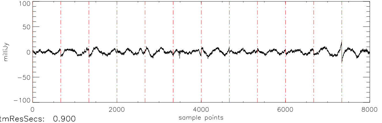
α2471 J11463449 07feb12 (AST) StokesI freq:5034.
