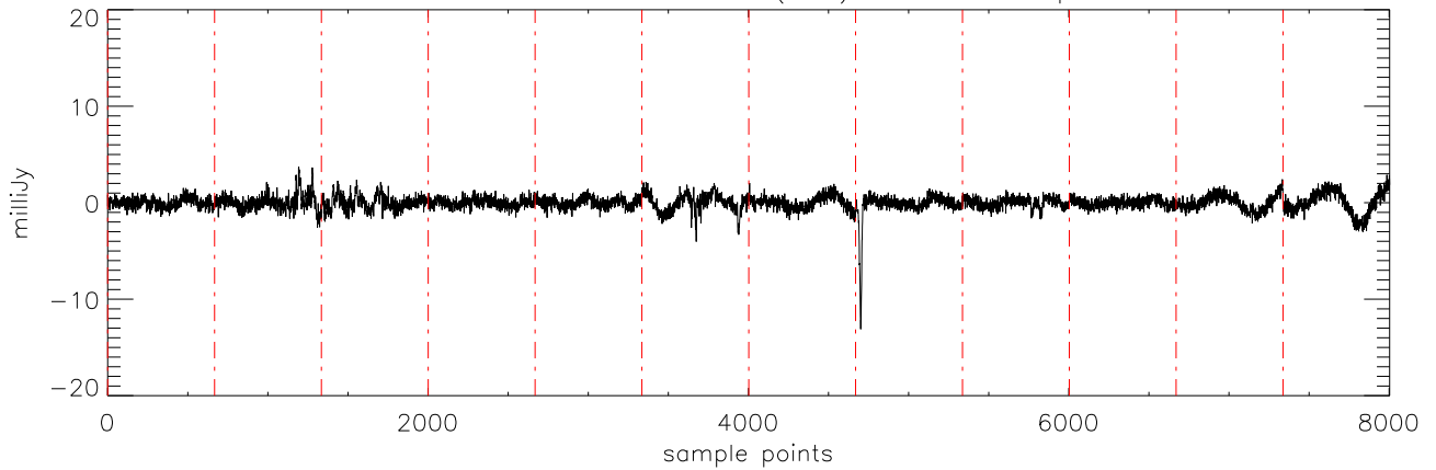
a2471 J11463449 07feb12 (AST) StokesU freq:4750.
