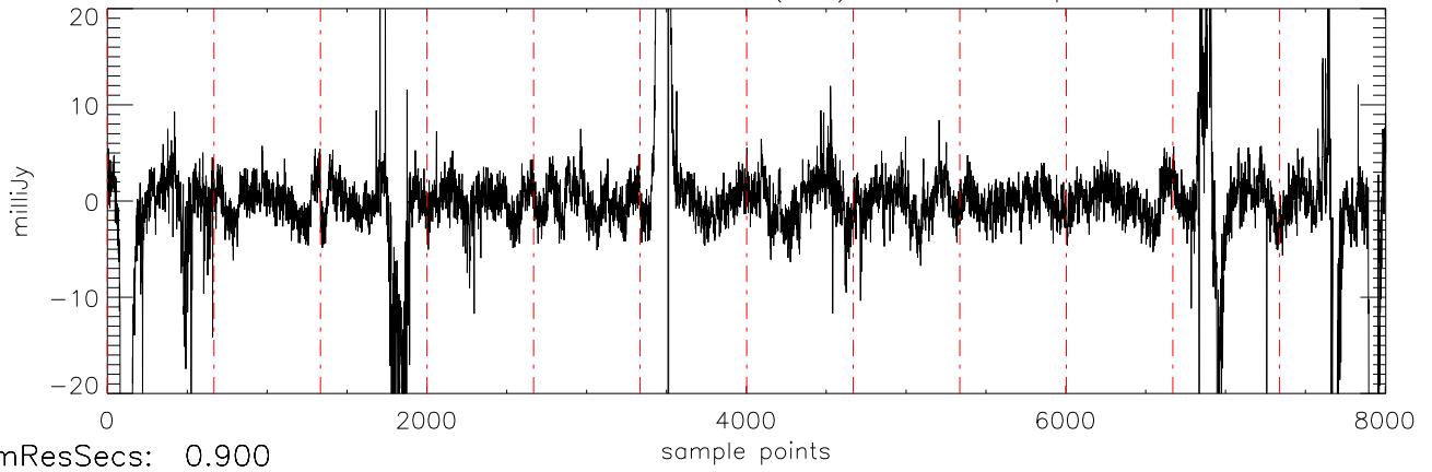
a2471 J11463449 07feb12 (AST) StokesQ freq:4466.
