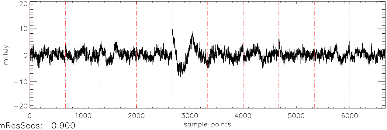
a2471 J10475385 17dec10 (AST) StokesQ freq:5034.
