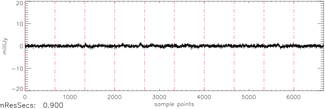
a2471 J10475385 17dec10 (AST) StokesV freq:5034.
