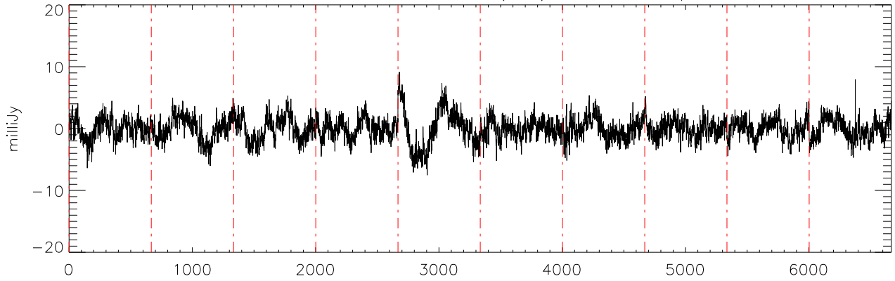
a2471 J10475385 17dec10 (AST) StokesQ freq:4608.
