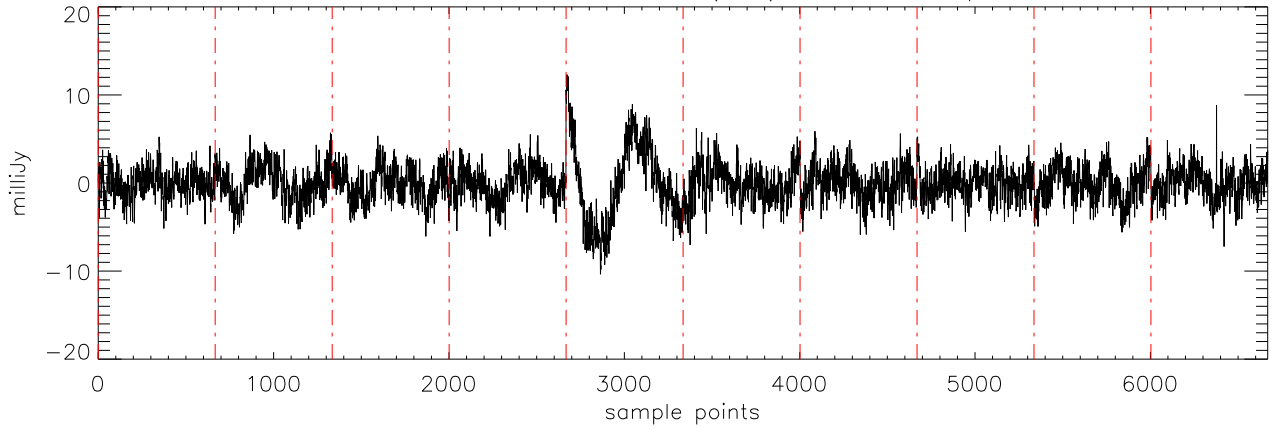
a2471 J10475385 17dec10 (AST) StokesQ freq:5176.
