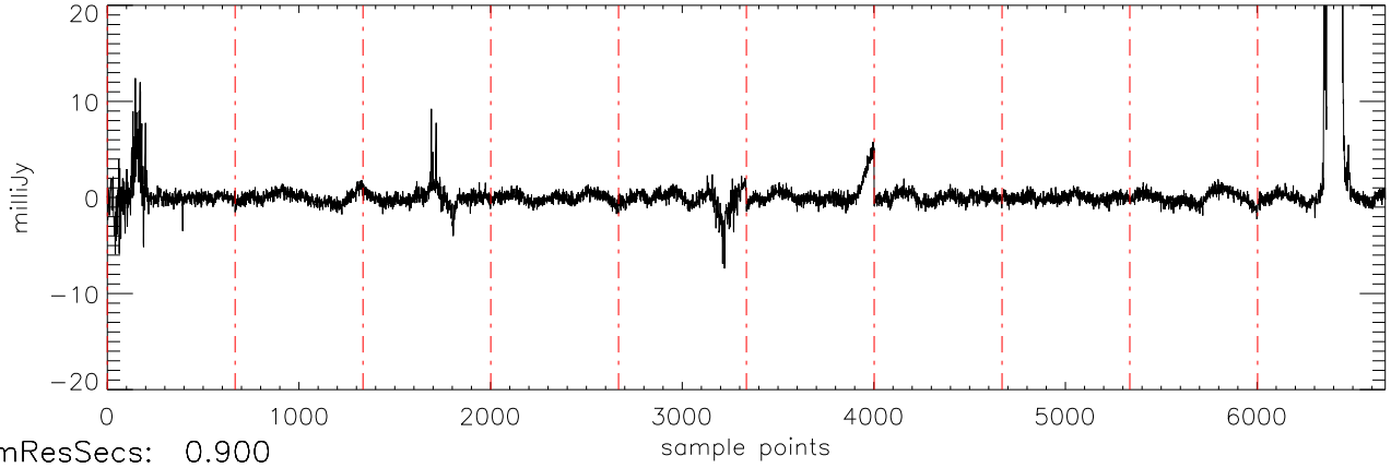
a2471 J10475385 17dec10 (AST) StokesU freq:4466.
