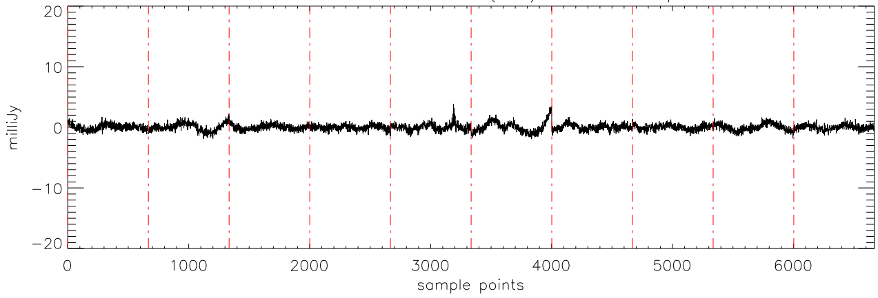
a2471 J10475385 17dec10 (AST) StokesU freq:4608.
