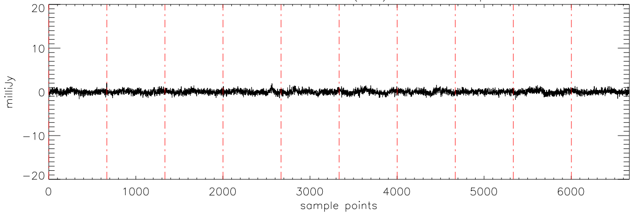
a2471 J10475385 17dec10 (AST) StokesV freq:5176.
