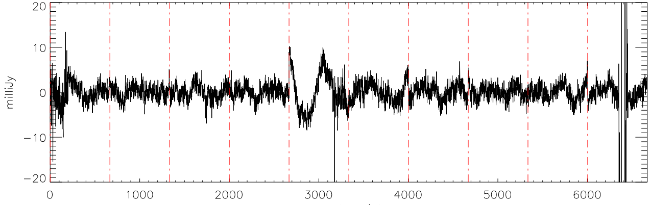
a2471 J10475385 17dec10 (AST) StokesQ freq:4325.
