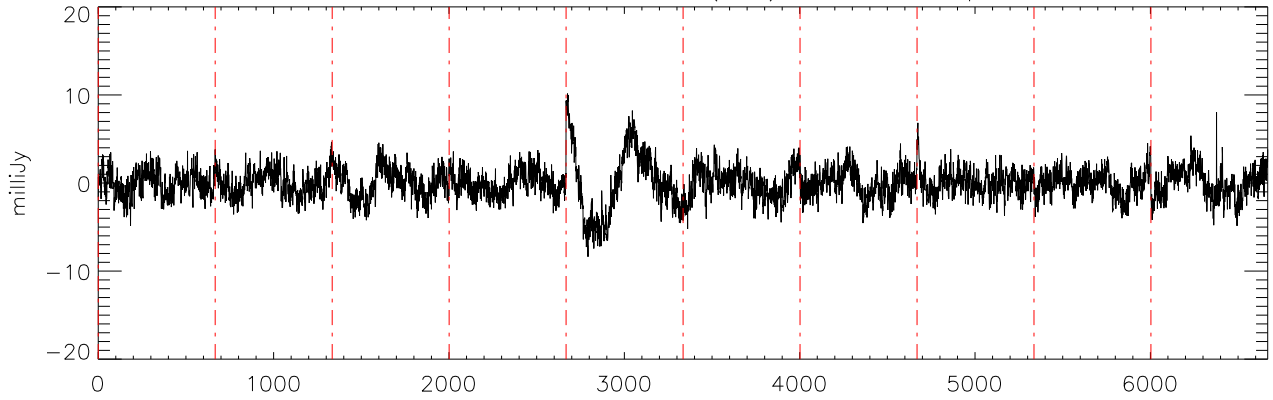
a2471 J10475385 17dec10 (AST) StokesQ freq:4750.
