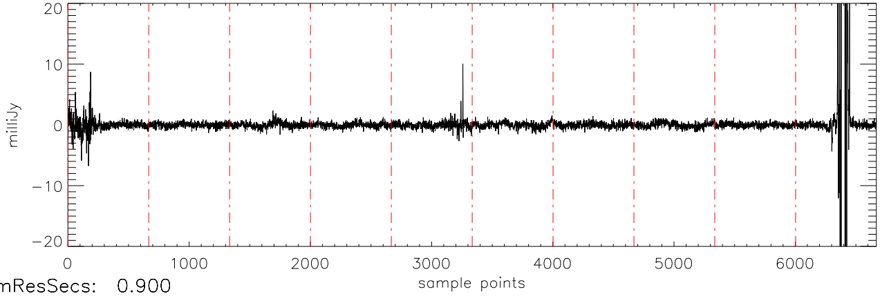
a2471 J10475385 17dec10 (AST) StokesV freq:4466.
