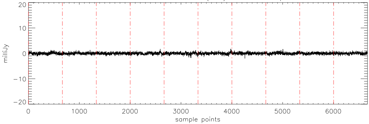
a2471 J10475385 17dec10 (AST) StokesV freq:4608.
