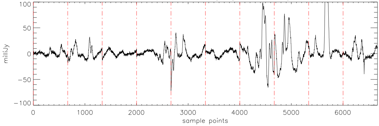
α2471 J10475385 17dec10 (AST) StokesI freq:5176.
