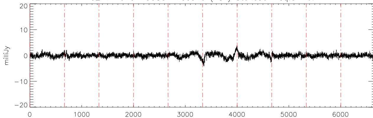
a2471 J10475385 17dec10 (AST) StokesU freq:5176.
