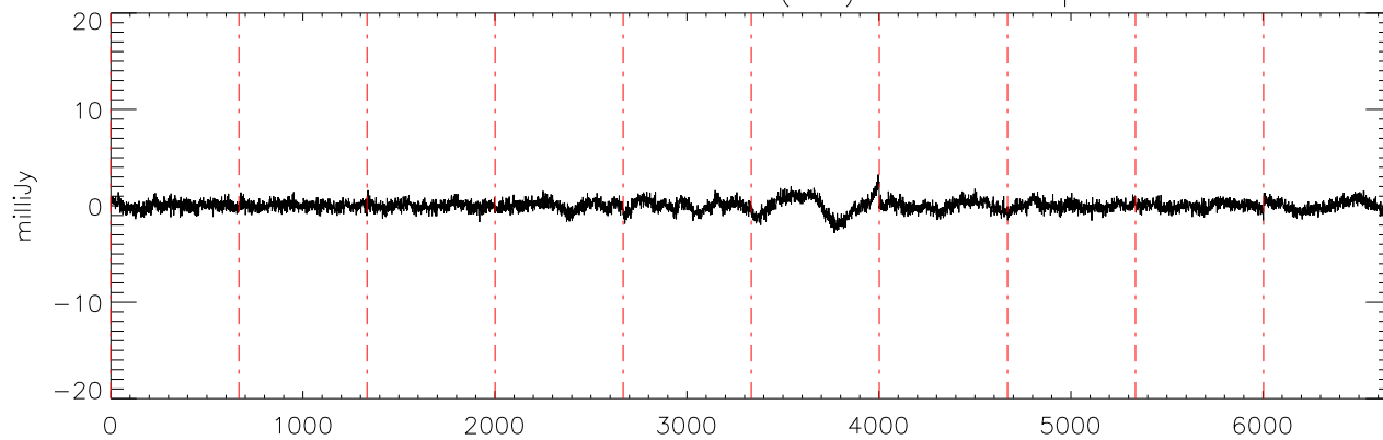
a2471 J10475385 17dec10 (AST) StokesU freq:4892.
