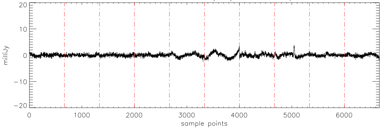
a2471 J10475385 17dec10 (AST) StokesU freq:4750.
