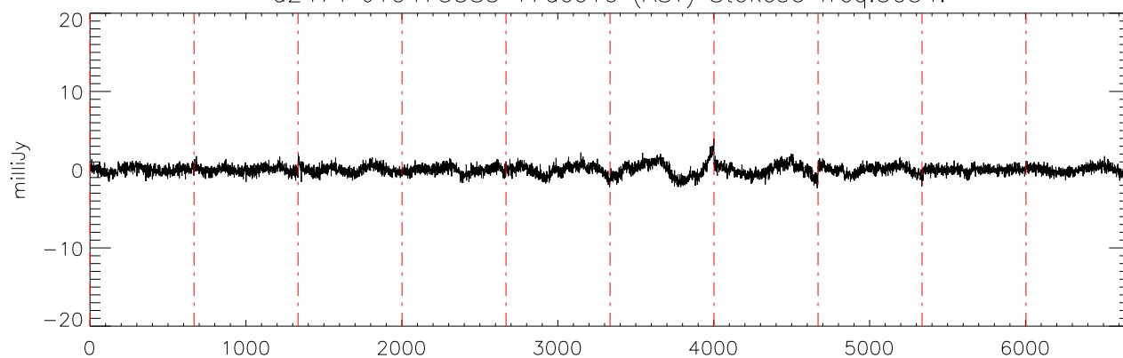
a2471 J10475385 17dec10 (AST) StokesU freq:5034.
