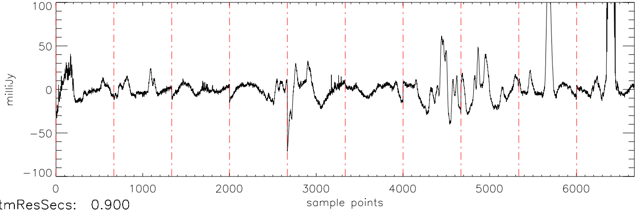
a2471 J10475385 17dec10 (AST) StokesI freq:4466.
