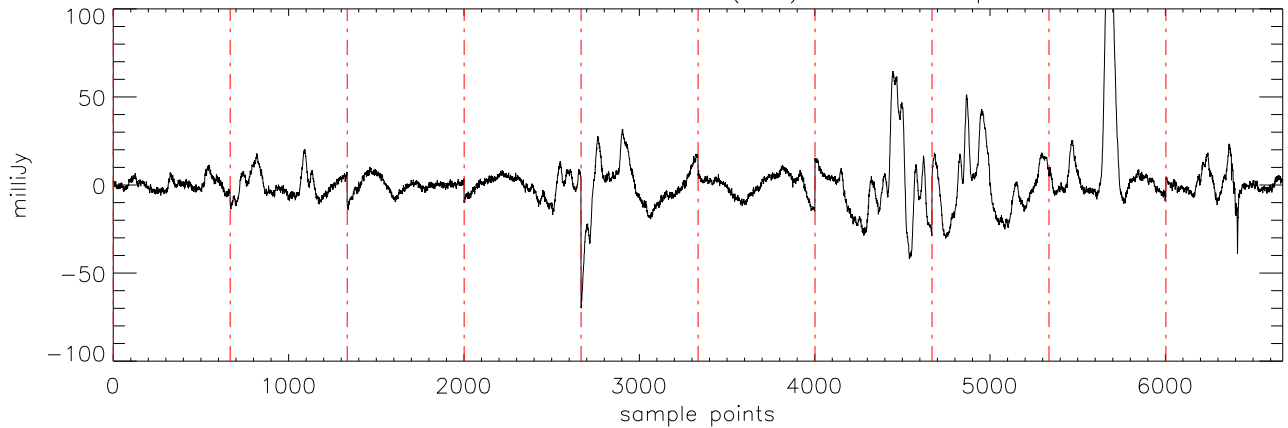
a2471 J10475385 17dec10 (AST) StokesI freq:4608.
