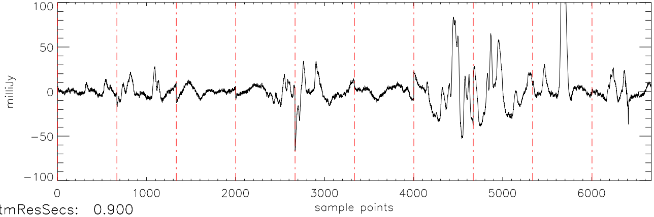
α2471 J10475385 17dec10 (AST) StokesI freq:5034.
