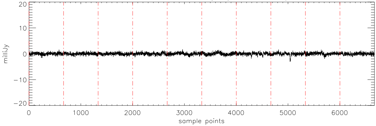
a2471 J10475385 17dec10 (AST) StokesV freq:4750.
