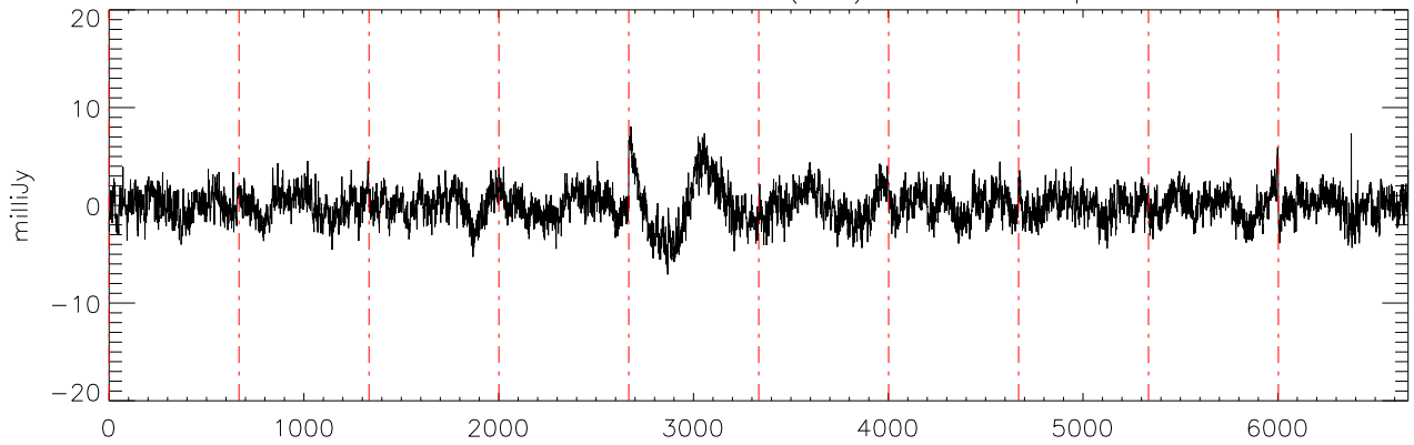
a2471 J10475385 17dec10 (AST) StokesQ freq:4466.
