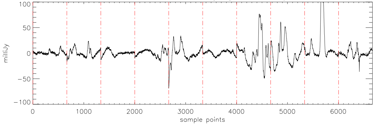
a2471 J10475385 17dec10 (AST) StokesI freq:4750.
