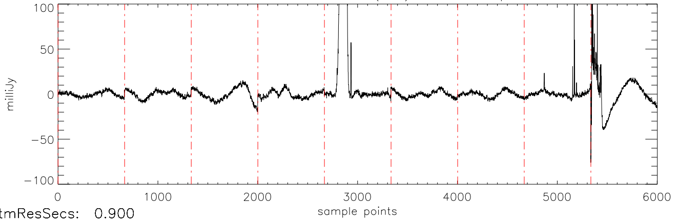
a2471 J10475385 06dec10 (AST) StokesI freq:4466.
