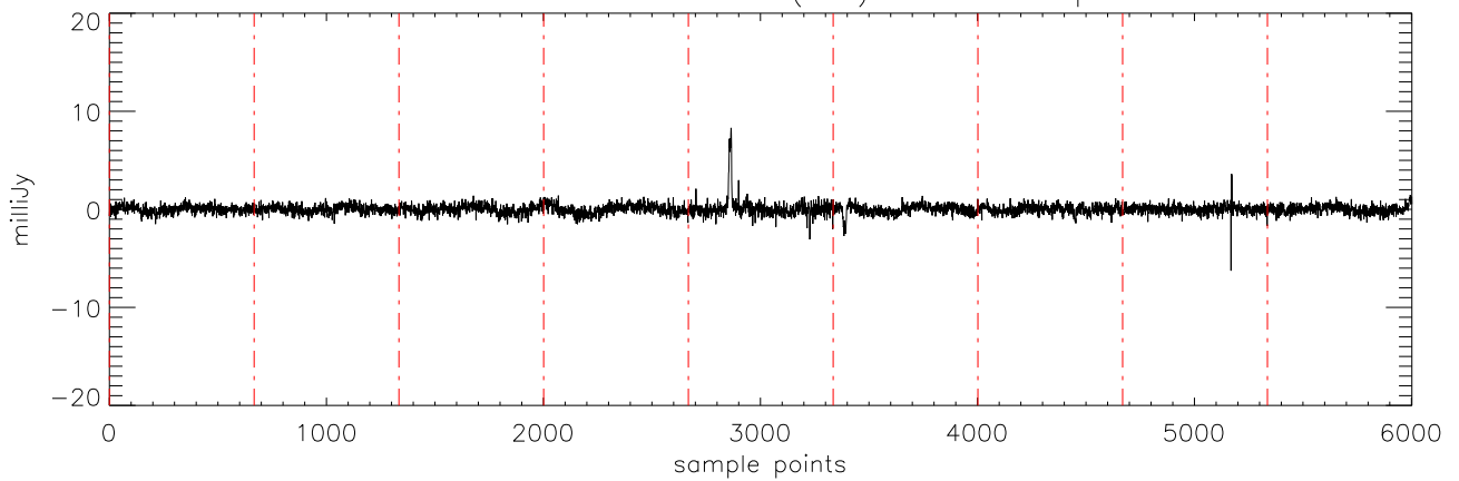
a2471 J10475385 06dec10 (AST) StokesV freq:4750.
