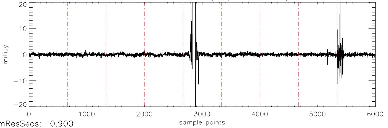
a2471 J10475385 06dec10 (AST) StokesV freq:4466.
