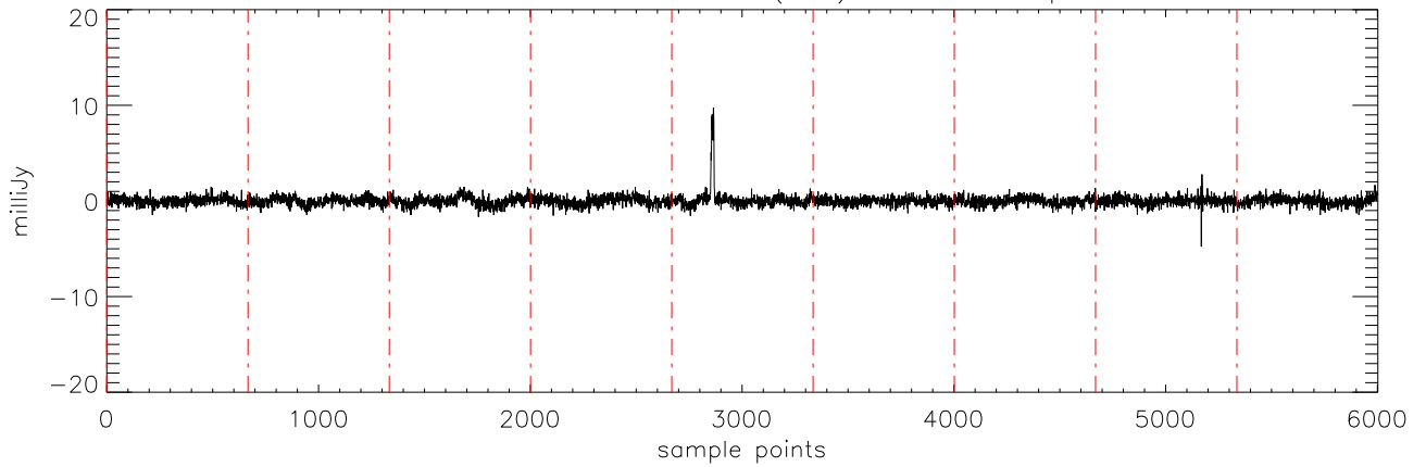
a2471 J10475385 06dec10 (AST) StokesV freq:5176.
