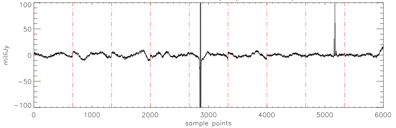
a2471 J10475385 06dec10 (AST) StokesI freq:4608.
