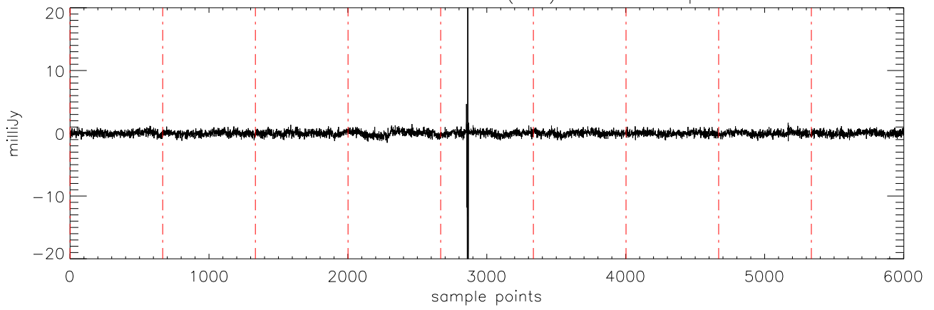
a2471 J10475385 06dec10 (AST) StokesV freq:4608.
