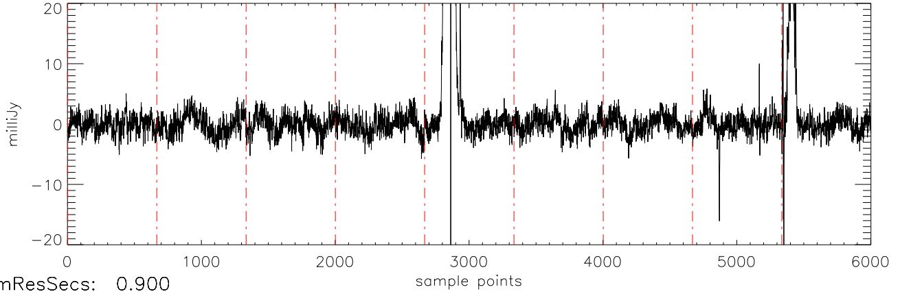
a2471 J10475385 06dec10 (AST) StokesQ freq:4466.
