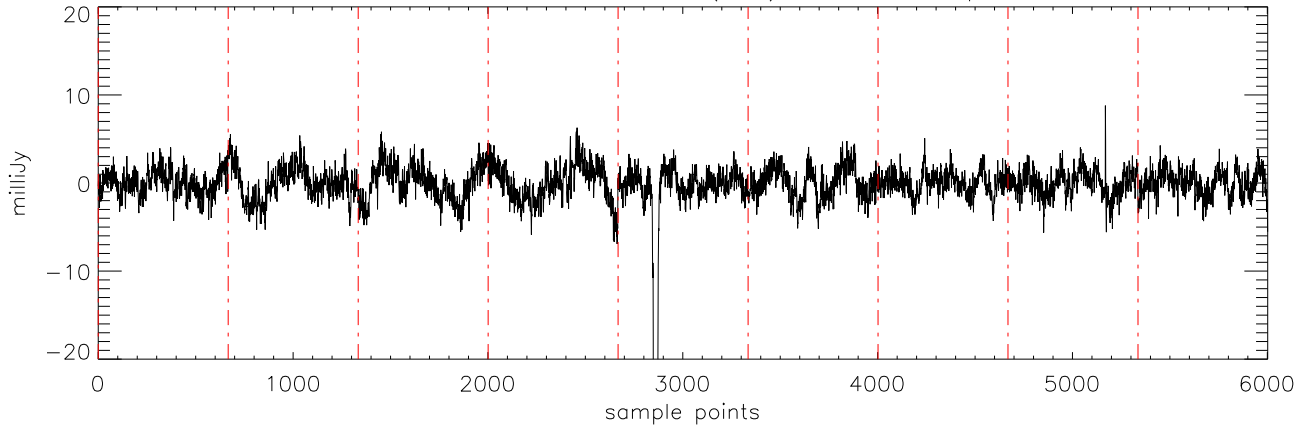
a2471 J10475385 06dec10 (AST) StokesQ freq:4750.
