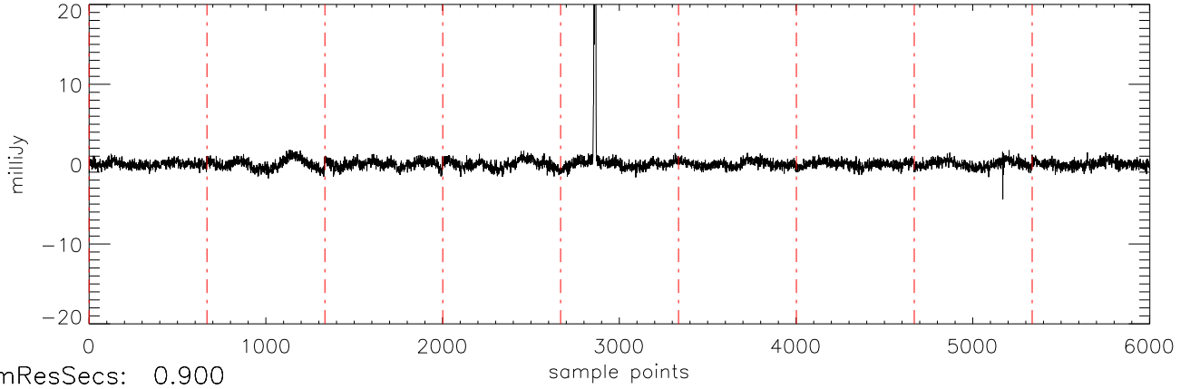
a2471 J10475385 06dec10 (AST) StokesU freq:5034.
