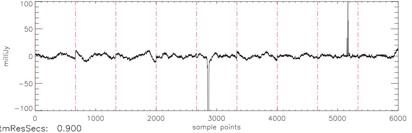
a2471 J10475385 06dec10 (AST) StokesI freq:5034.
