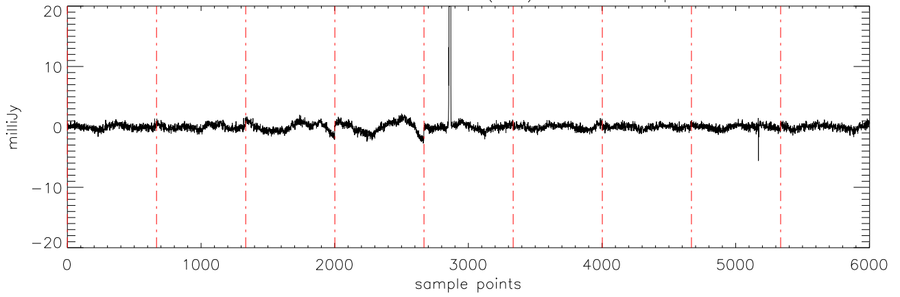
a2471 J10475385 06dec10 (AST) StokesU freq:4608.
