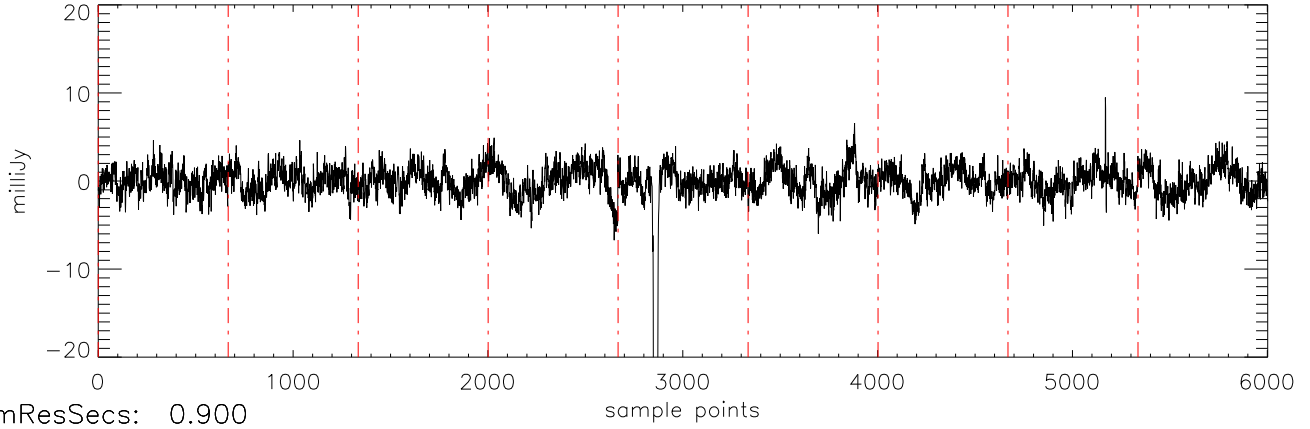
a2471 J10475385 06dec10 (AST) StokesQ freq:5034.
