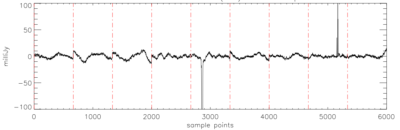
a2471 J10475385 06dec10 (AST) StokesI freq:5176.
