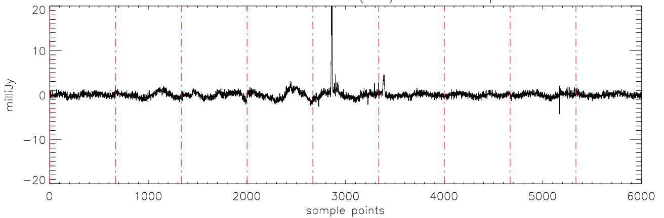
a2471 J10475385 06dec10 (AST) StokesU freq:4750.
