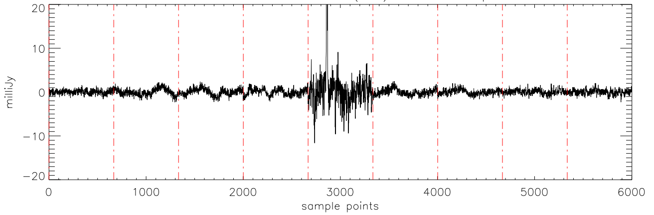
a2471 J10475385 06dec10 (AST) StokesU freq:5176.
