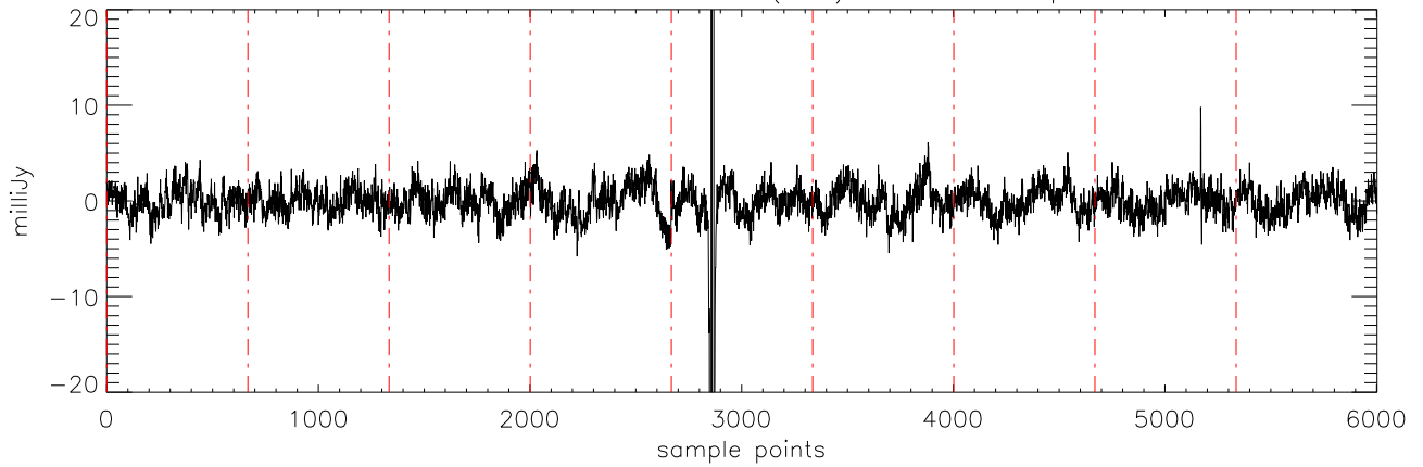
a2471 J10475385 06dec10 (AST) StokesQ freq:4608.
