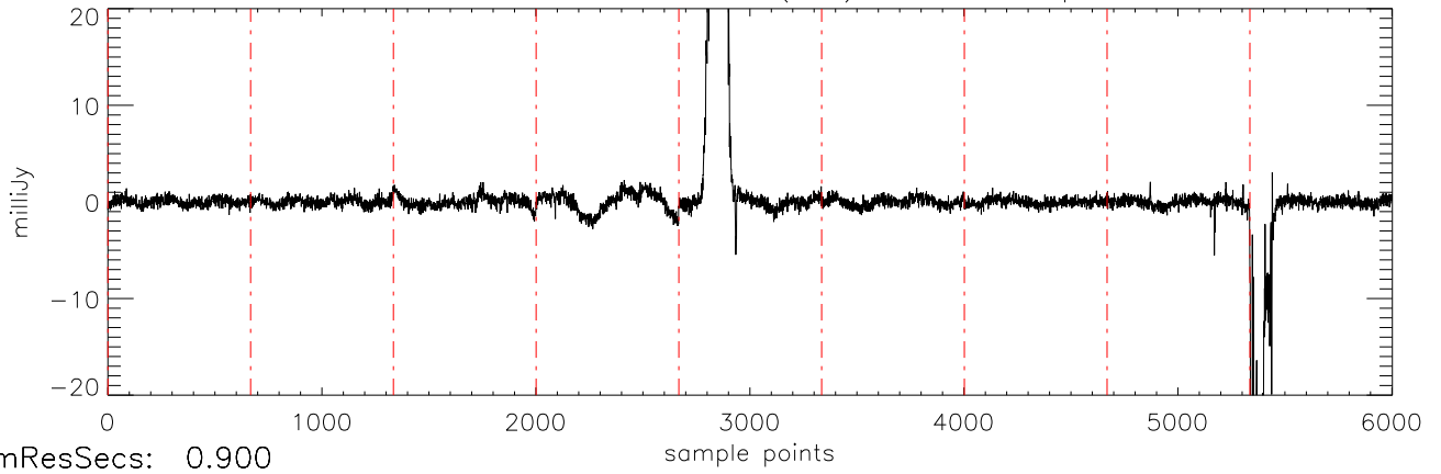
a2471 J10475385 06dec10 (AST) StokesU freq:4466.
