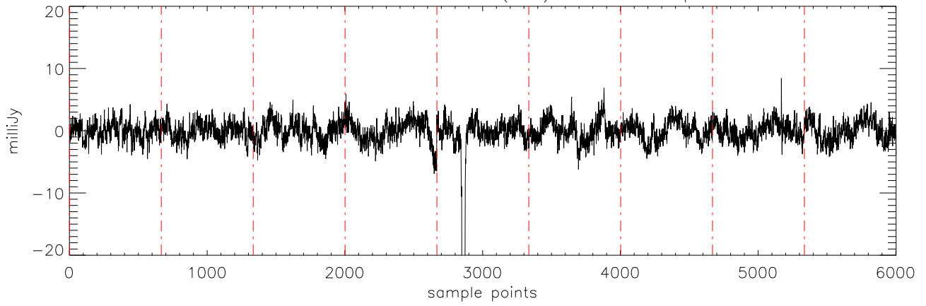
a2471 J10475385 06dec10 (AST) StokesQ freq:5176.
