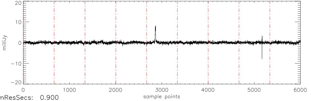
a2471 J10475385 06dec10 (AST) StokesV freq:5034.
