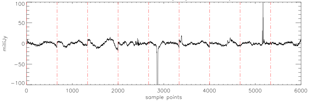
a2471 J10475385 06dec10 (AST) StokesI freq:4750.
