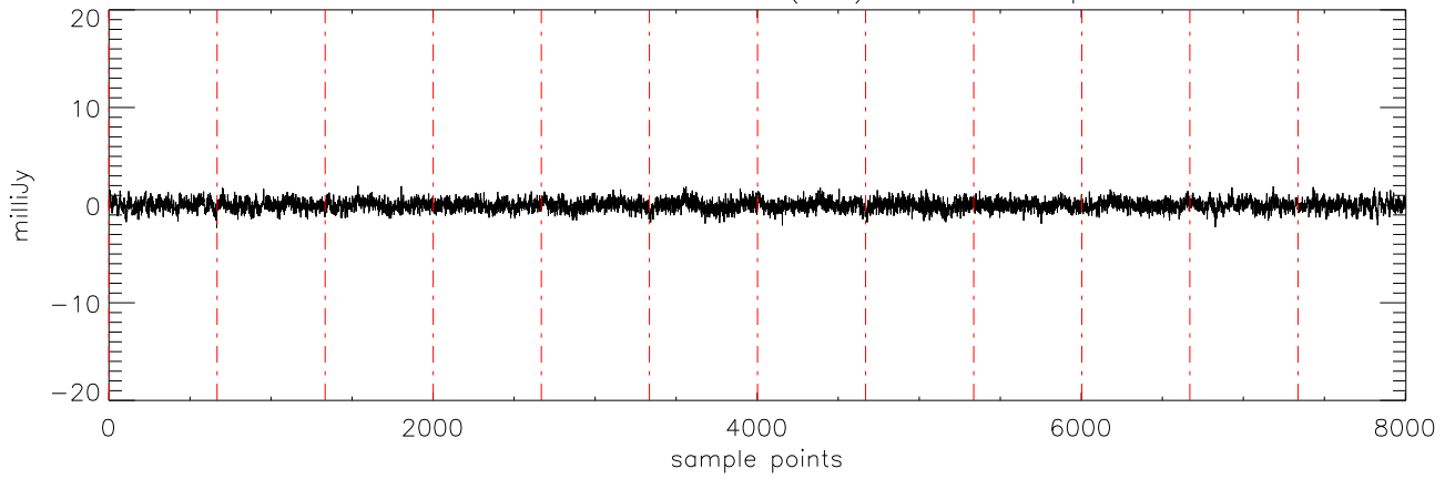
a2471 J10475385 04dec10 (AST) StokesV freq:5176.
