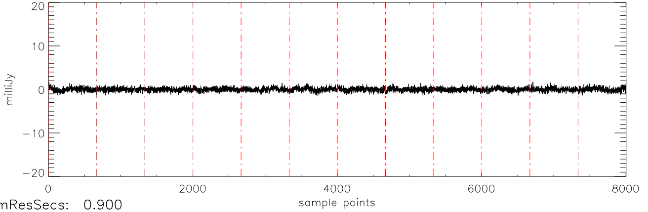
a2471 J10475385 04dec10 (AST) StokesV freq:5034.
