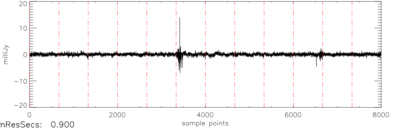
a2471 J10475385 04dec10 (AST) StokesV freq:4466.
