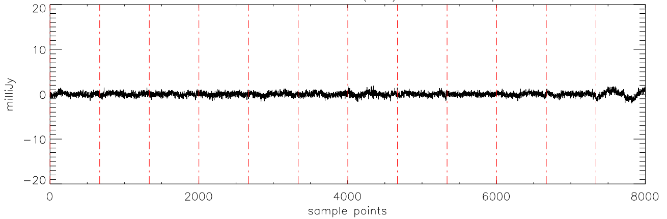
a2471 J10475385 04dec10 (AST) StokesV freq:4750.
