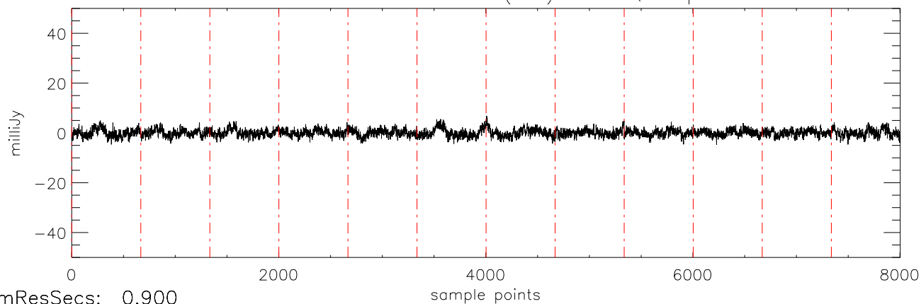
a2471 J10475385 04dec10 (AST) StokesQ freq:5034.
