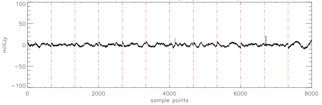
a2471 J10475385 04dec10 (AST) StokesI freq:4608.
