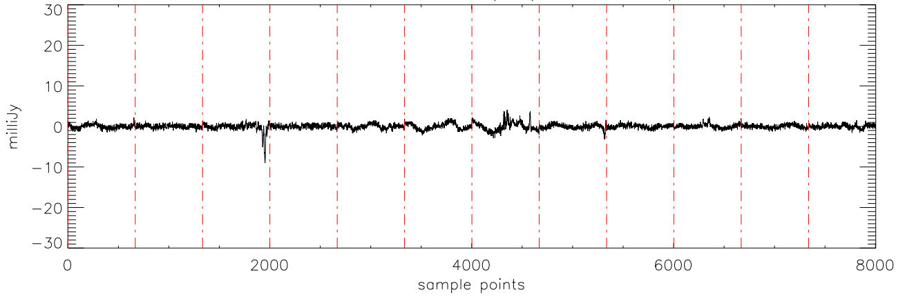
a2471 J10475385 04dec10 (AST) StokesU freq:4750.
