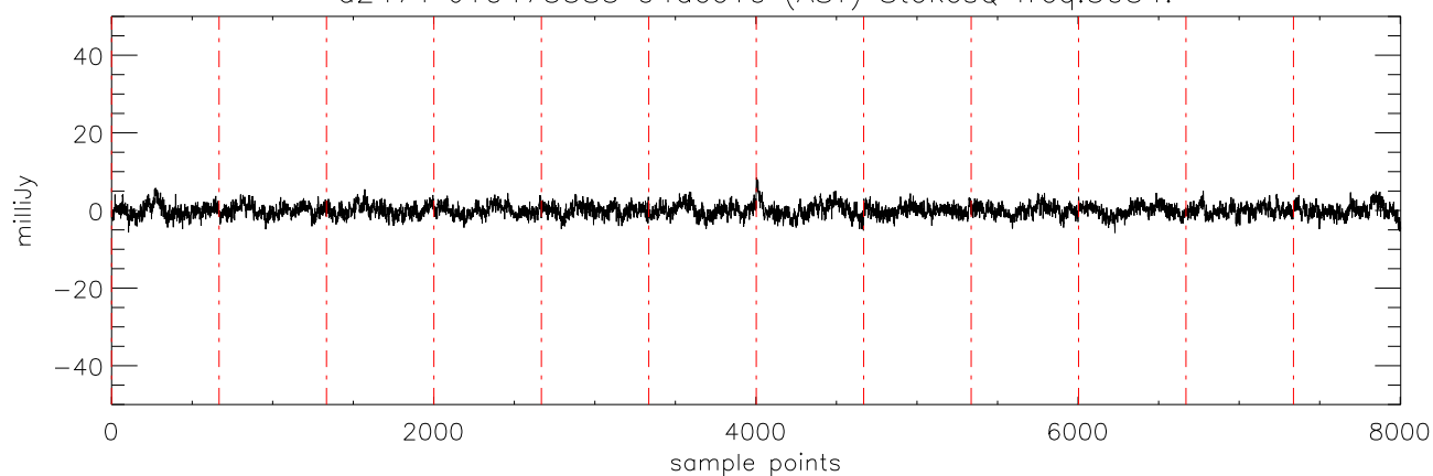
a2471 J10475385 04dec10 (AST) StokesQ freq:5176.
