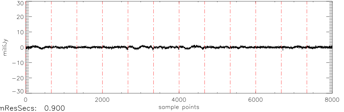
a2471 J10475385 04dec10 (AST) StokesU freq:5034.
