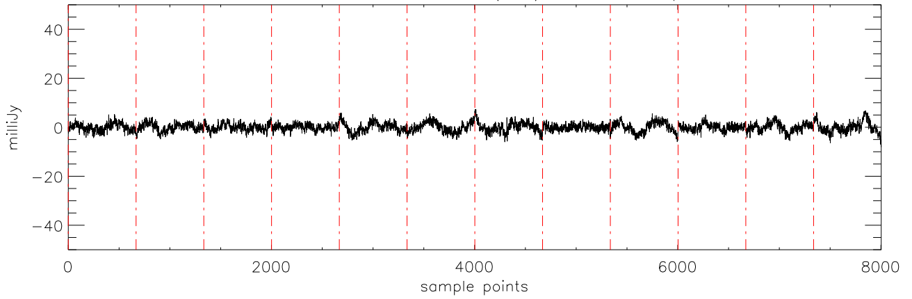
a2471 J10475385 04dec10 (AST) StokesQ freq:4750.
