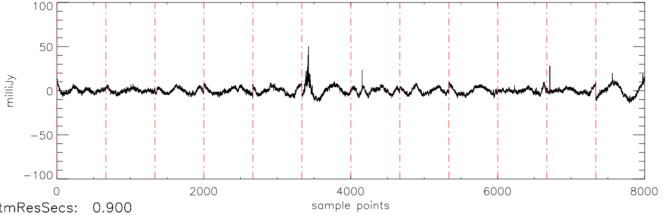
a2471 J10475385 04dec10 (AST) StokesI freq:4466.
