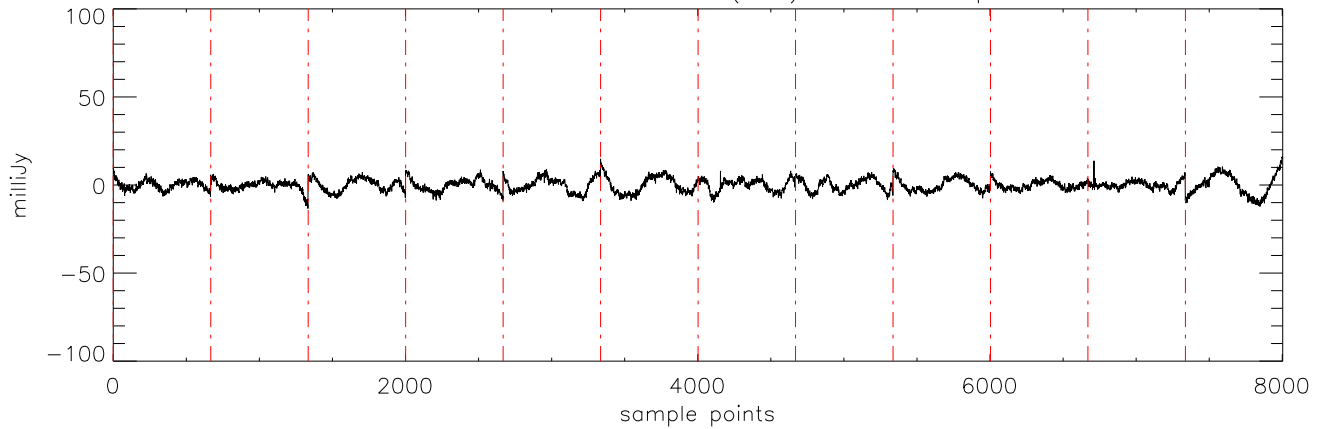
a2471 J10475385 04dec10 (AST) StokesI freq:4750.
