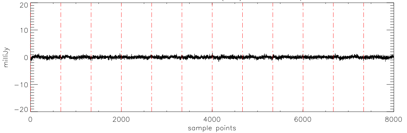
a2471 J10475385 04dec10 (AST) StokesV freq:4608.
