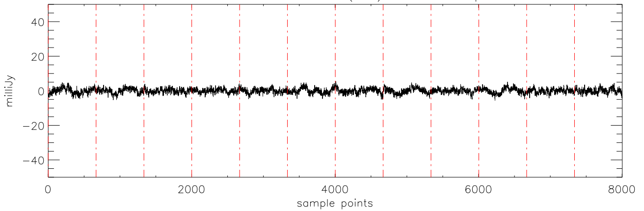
a2471 J10475385 04dec10 (AST) StokesQ freq:4608.
