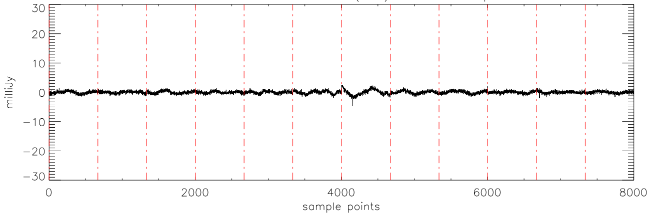
a2471 J10475385 04dec10 (AST) StokesU freq:4608.
