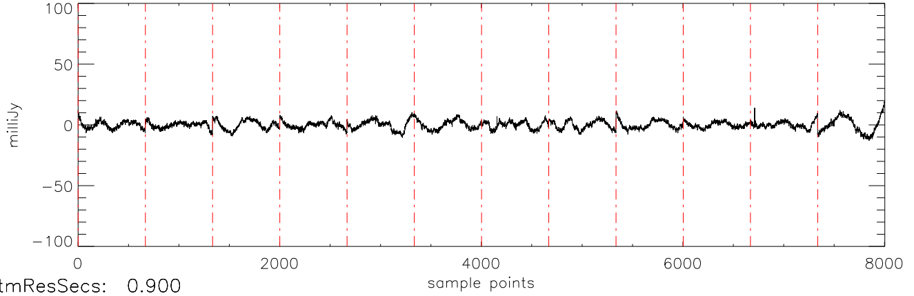
a2471 J10475385 04dec10 (AST) StokesI freq:5034.
