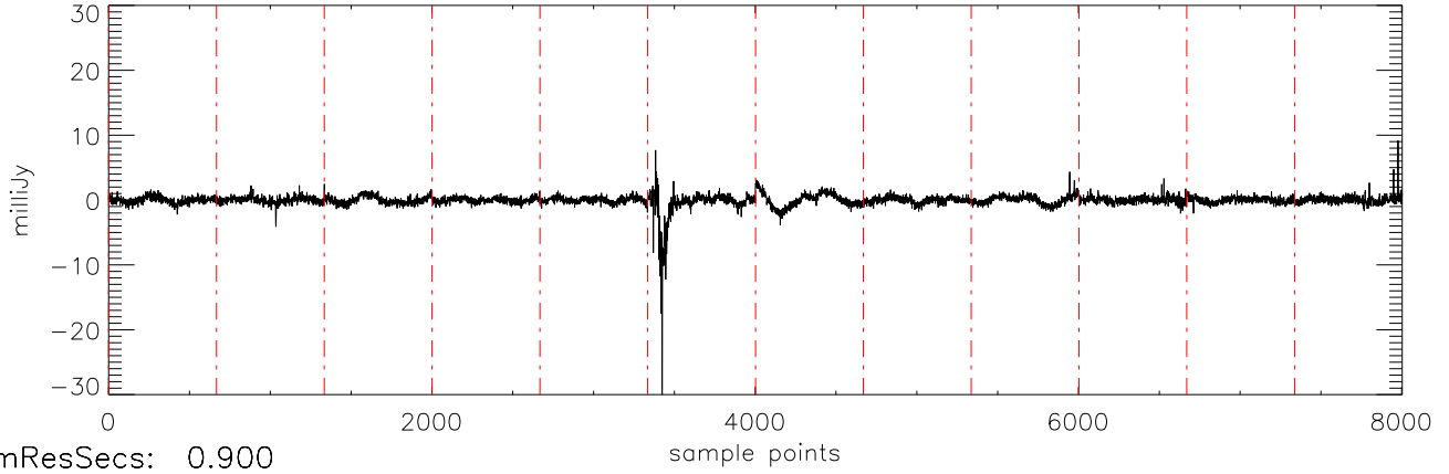
a2471 J10475385 04dec10 (AST) StokesU freq:4466.
