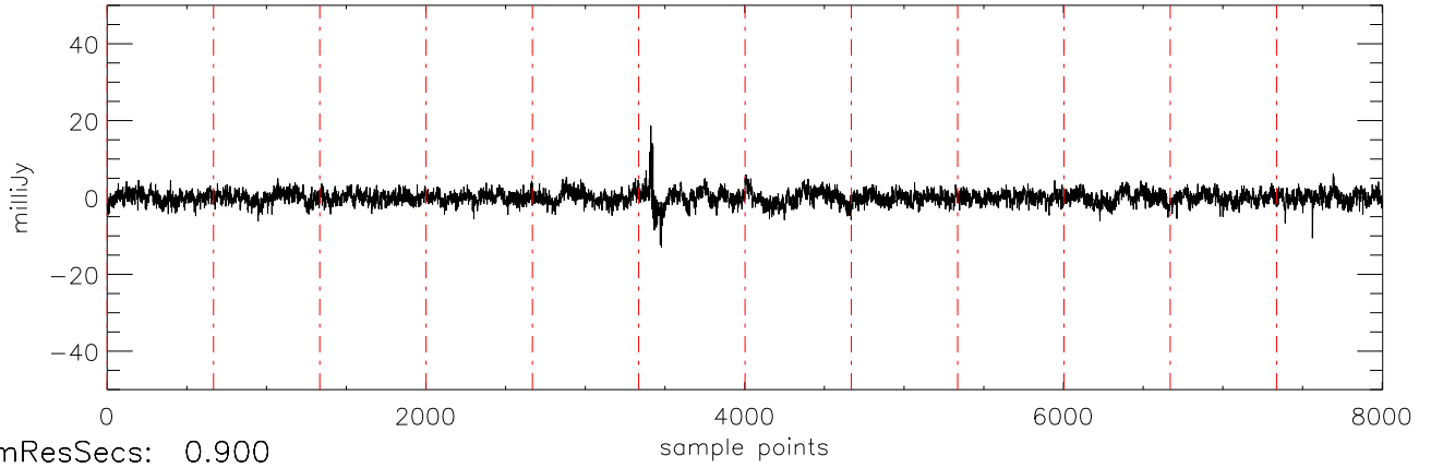
a2471 J10475385 04dec10 (AST) StokesQ freq:4466.
