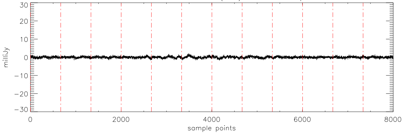
a2471 J10475385 04dec10 (AST) StokesU freq:5176.
