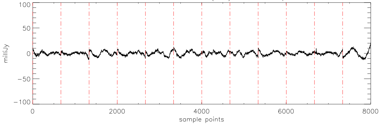
a2471 J10475385 04dec10 (AST) StokesI freq:5176.
