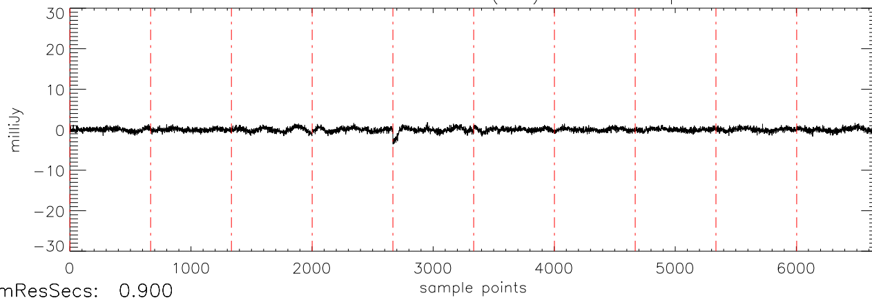
a2471 J10475385 02dec10 (AST) StokesU freq:5034.
