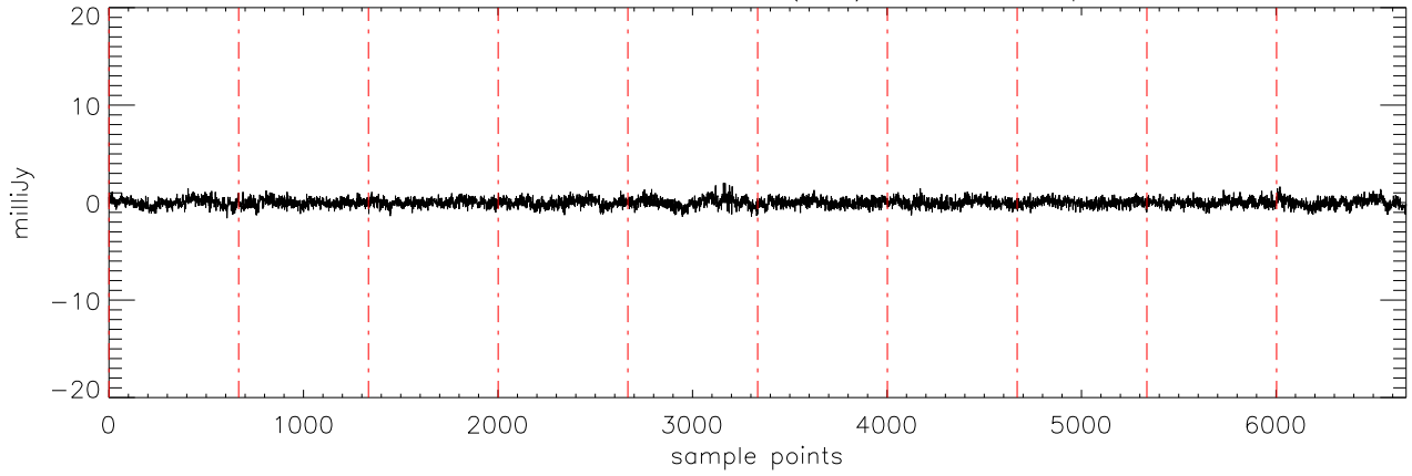
a2471 J10475385 02dec10 (AST) StokesV freq:4750.
