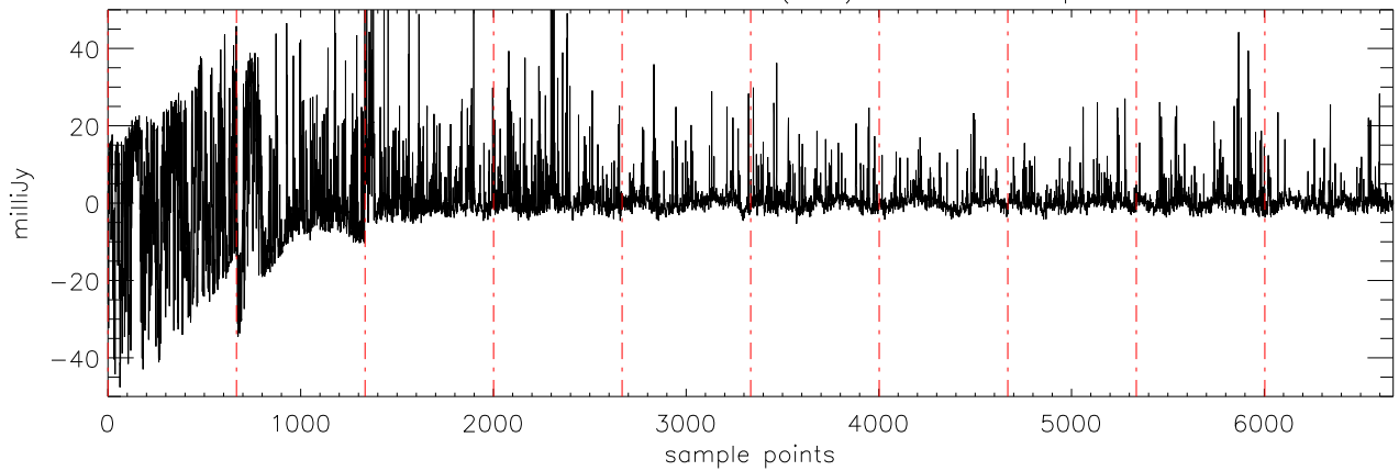
a2471 J10475385 02dec10 (AST) StokesQ freq:4750.
