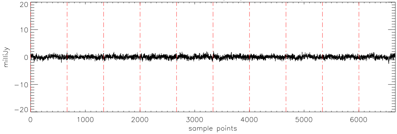
a2471 J10475385 02dec10 (AST) StokesV freq:5176.
