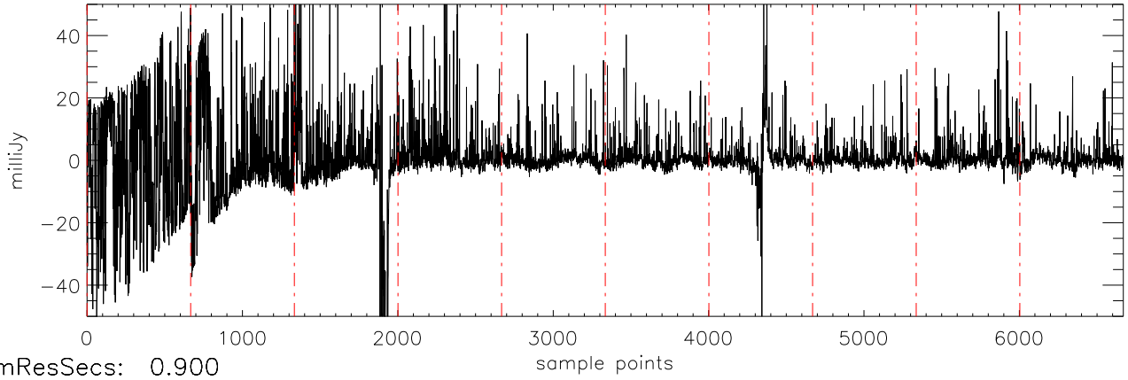
a2471 J10475385 02dec10 (AST) StokesQ freq:4466.
