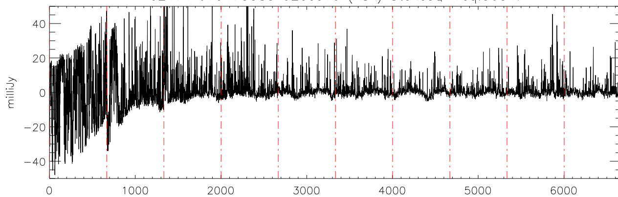
a2471 J10475385 02dec10 (AST) StokesQ freq:5034.
