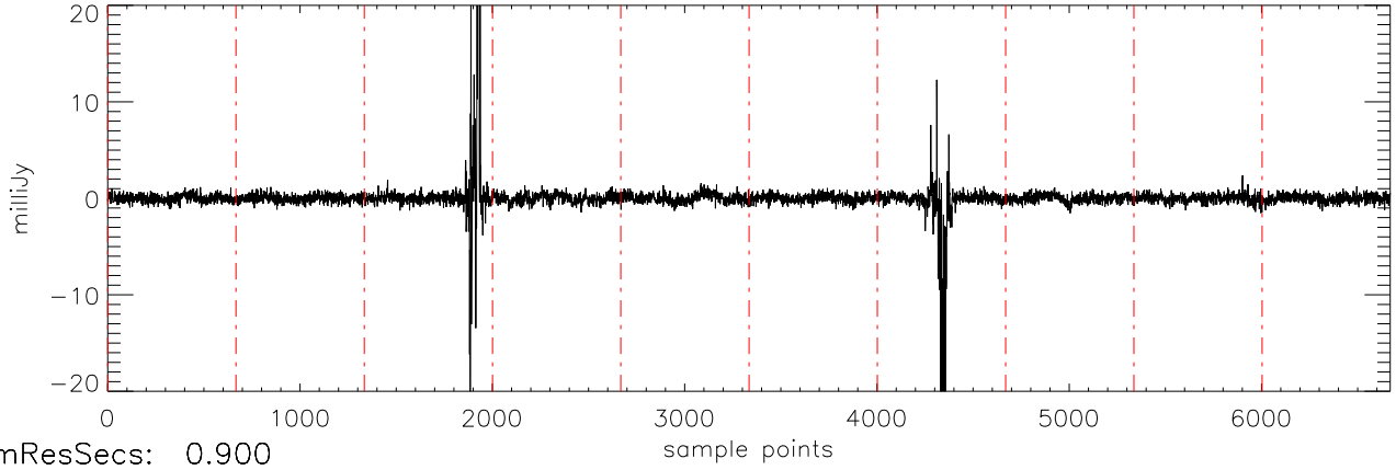
a2471 J10475385 02dec10 (AST) StokesV freq:4466.
