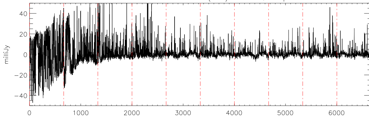
a2471 J10475385 02dec10 (AST) StokesQ freq:5176.
