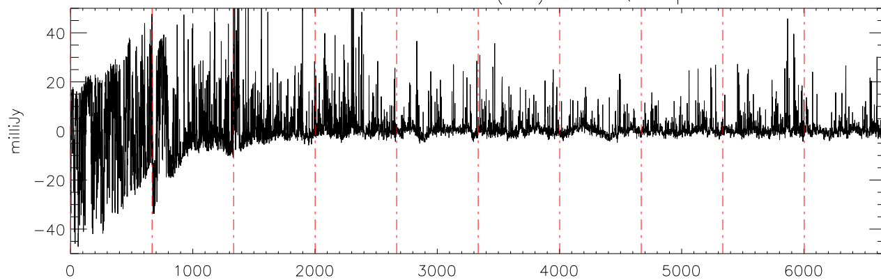
a2471 J10475385 02dec10 (AST) StokesQ freq:4892.
