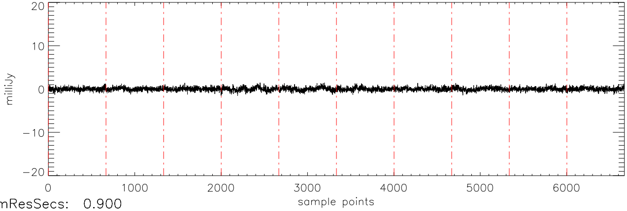
a2471 J10475385 02dec10 (AST) StokesV freq:5034.
