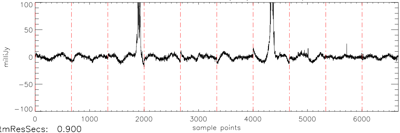
a2471 J10475385 02dec10 (AST) 2*PolA freq:4466.
