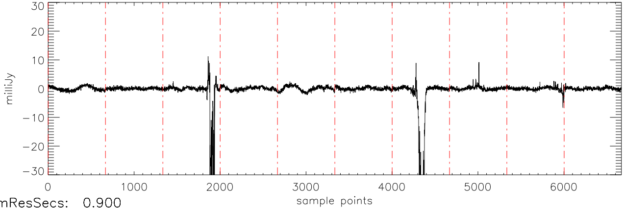
a2471 J10475385 02dec10 (AST) StokesU freq:4466.
