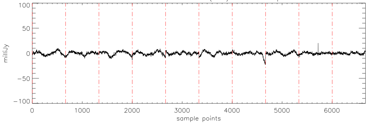
a2471 J10475385 02dec10 (AST) 2*PolA freq:4608.
