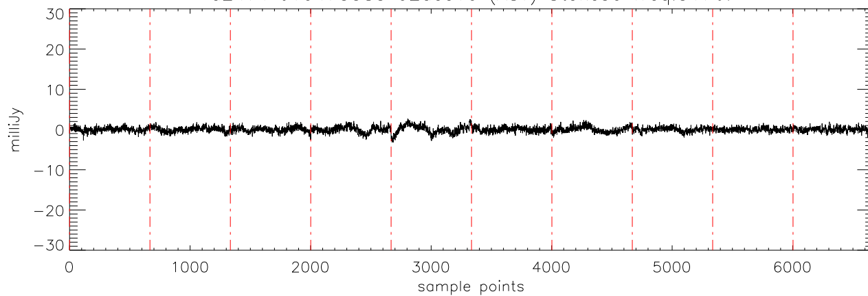
a2471 J10475385 02dec10 (AST) StokesU freq:5176.
