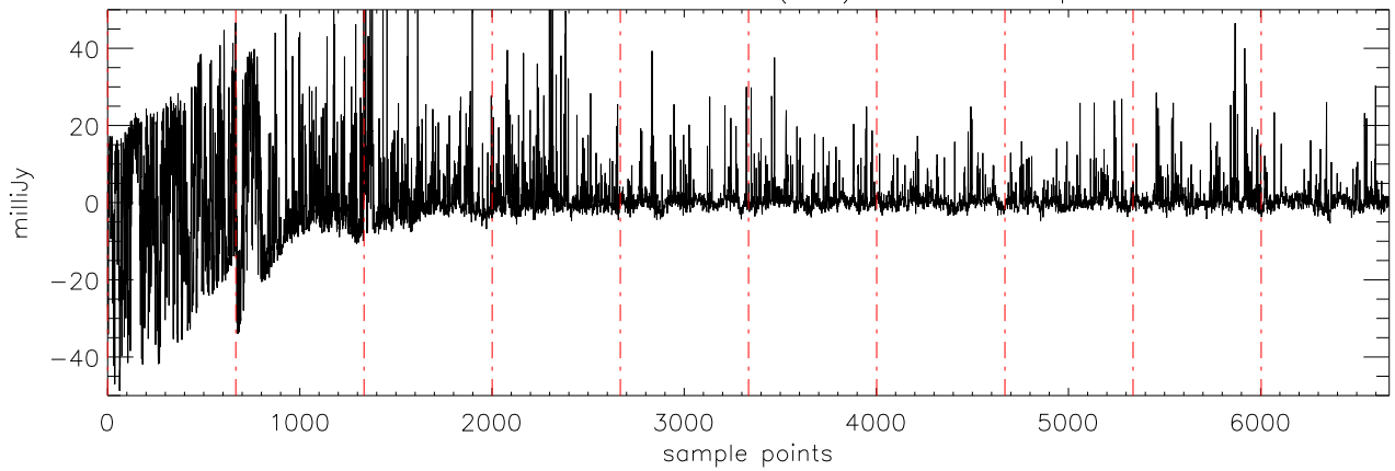
a2471 J10475385 02dec10 (AST) StokesQ freq:4608.
