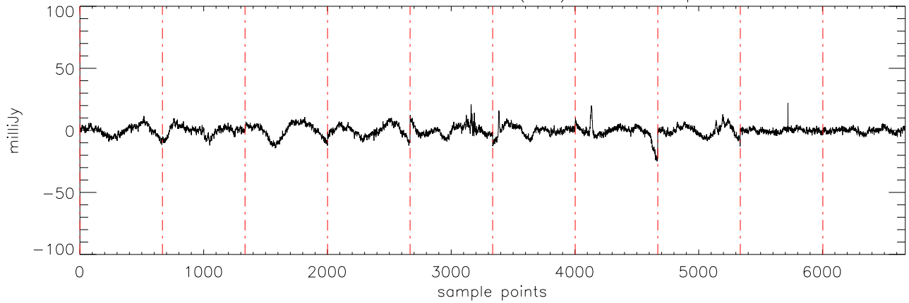
a2471 J10475385 02dec10 (AST) 2*PolA freq:4750.
