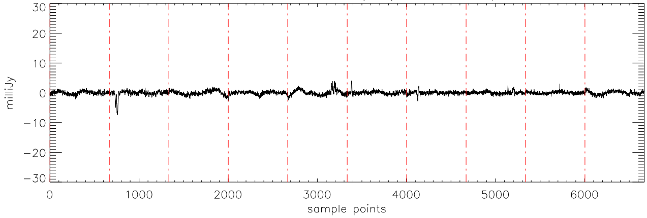
a2471 J10475385 02dec10 (AST) StokesU freq:4750.
