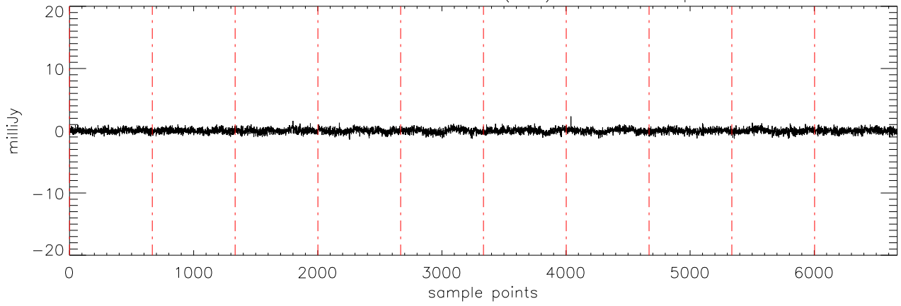
a2471 J10475385 02dec10 (AST) StokesV freq:4608.
