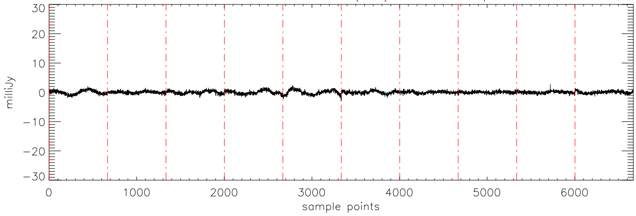
a2471 J10475385 02dec10 (AST) StokesU freq:4608.
