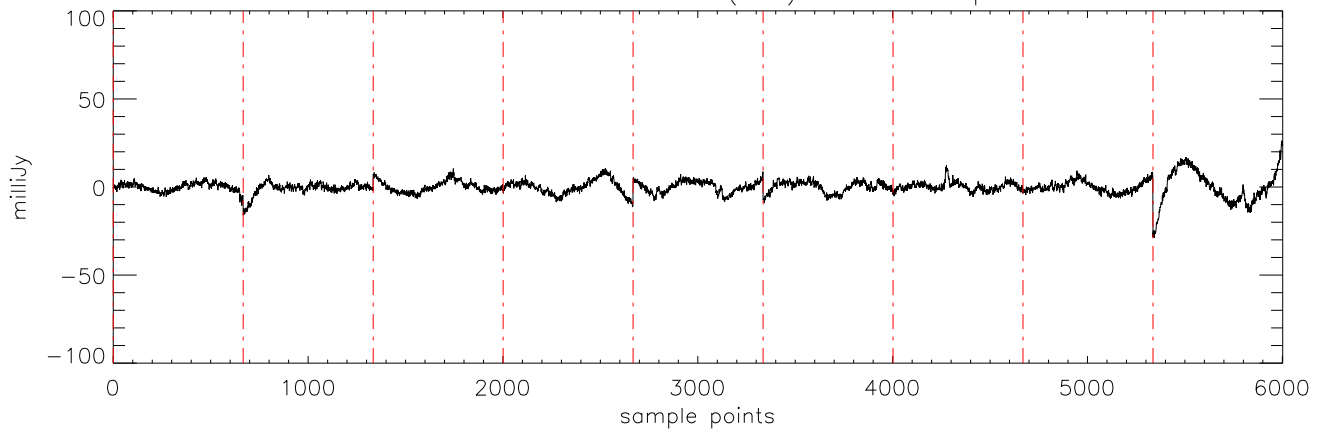
a2471 J09373487 07feb12 (AST) StokesI freq:4608.
