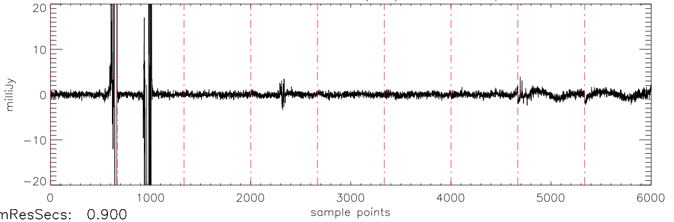
a2471 J09373487 07feb12 (AST) StokesV freq:4466.
