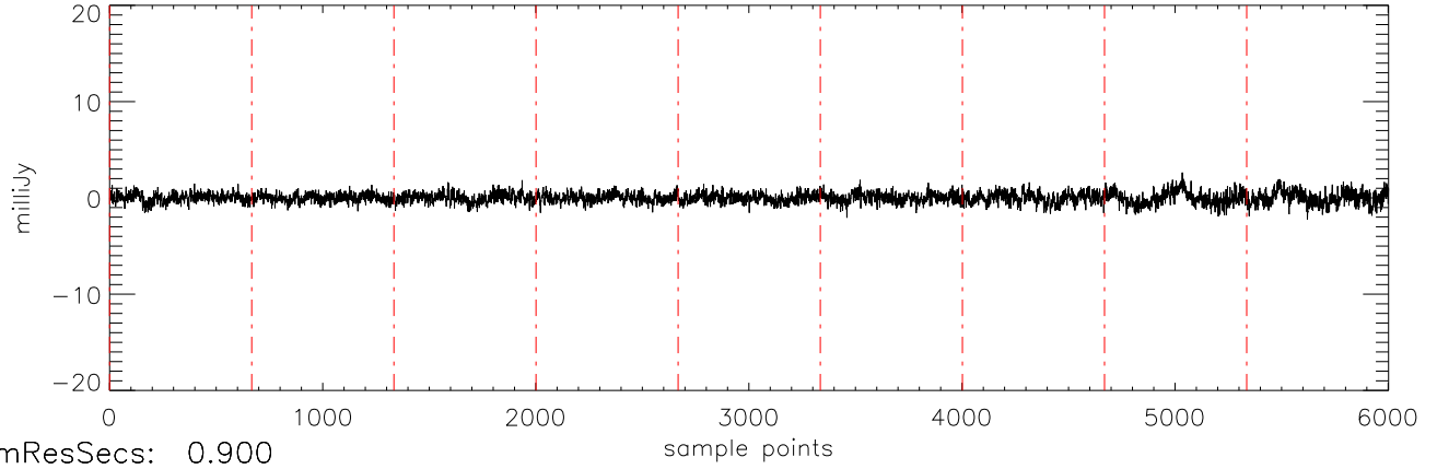
a2471 J09373487 07feb12 (AST) StokesV freq:5034.
