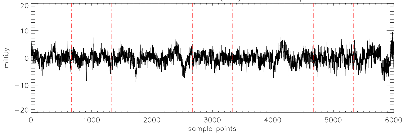
a2471 J09373487 07feb12 (AST) StokesQ freq:5176.
