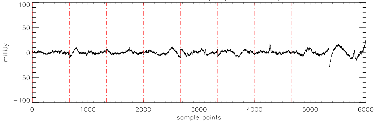
a2471 J09373487 07feb12 (AST) StokesI freq:4750.
