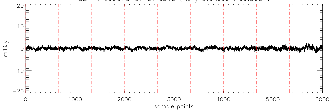
a2471 J09373487 07feb12 (AST) StokesU freq:5176.
