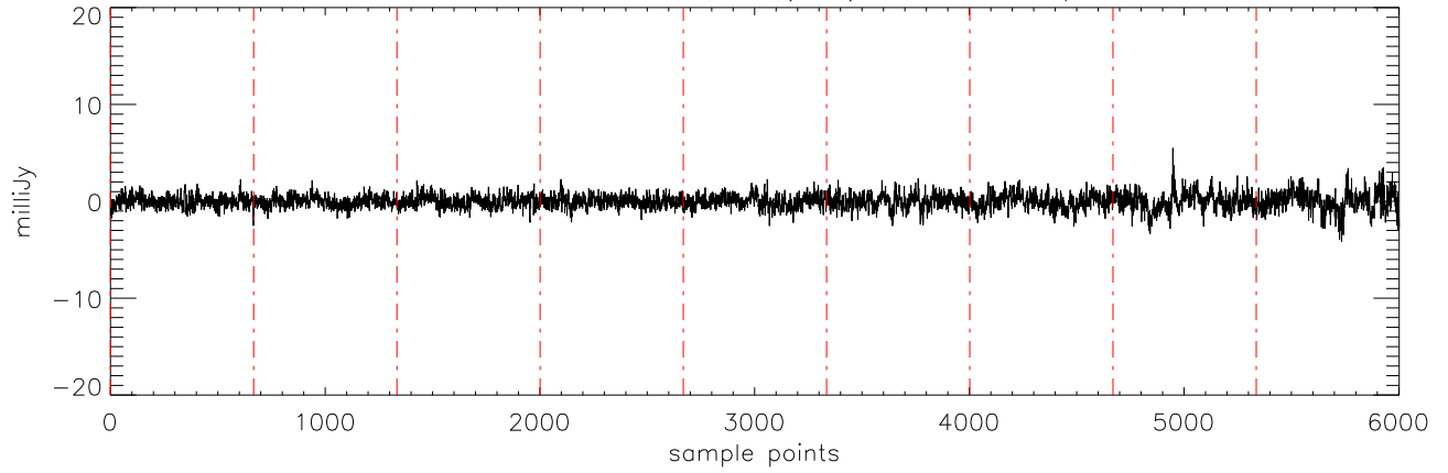
a2471 J09373487 07feb12 (AST) StokesV freq:5176.
