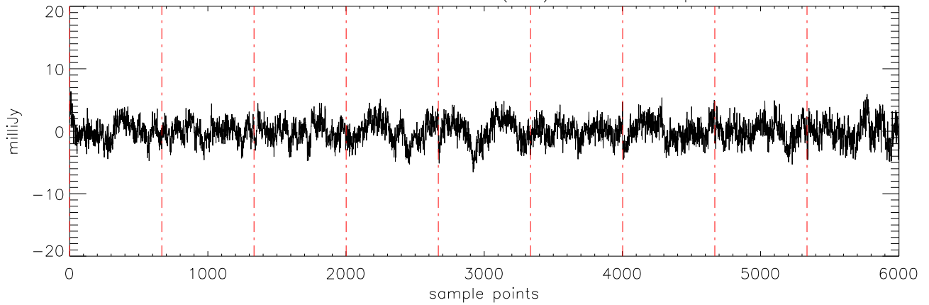
a2471 J09373487 07feb12 (AST) StokesQ freq:4608.
