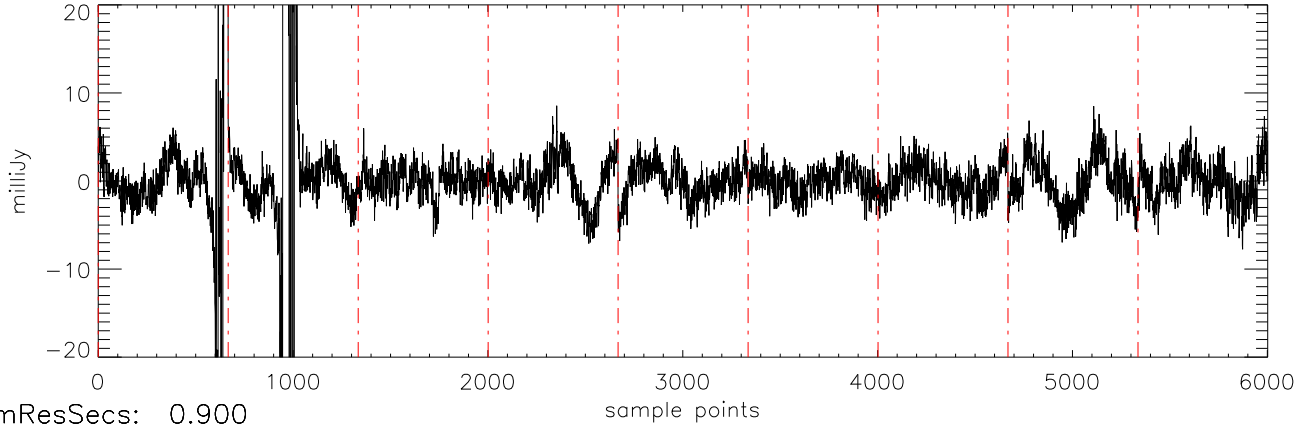
a2471 J09373487 07feb12 (AST) StokesQ freq:4466.
