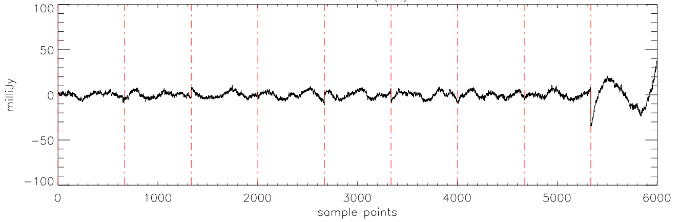
a2471 J09373487 07feb12 (AST) StokesI freq:5176.
