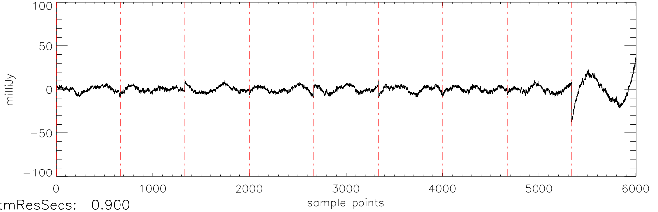
a2471 J09373487 07feb12 (AST) StokesI freq:5034.
