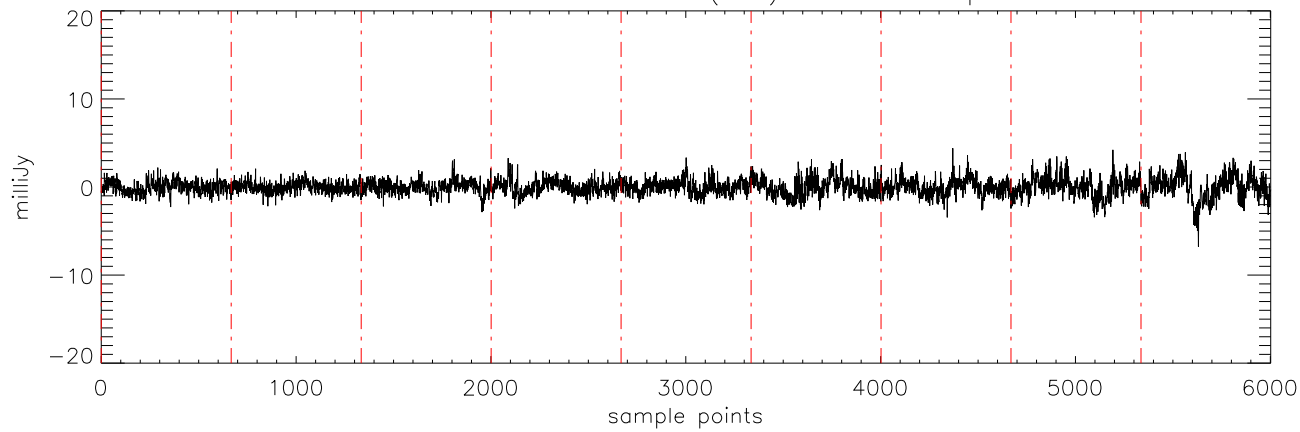
a2471 J09373487 07feb12 (AST) StokesU freq:5176.
