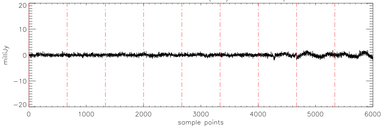
a2471 J09373487 07feb12 (AST) StokesV freq:4608.
