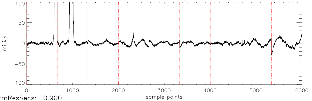
a2471 J09373487 07feb12 (AST) StokesI freq:4466.
