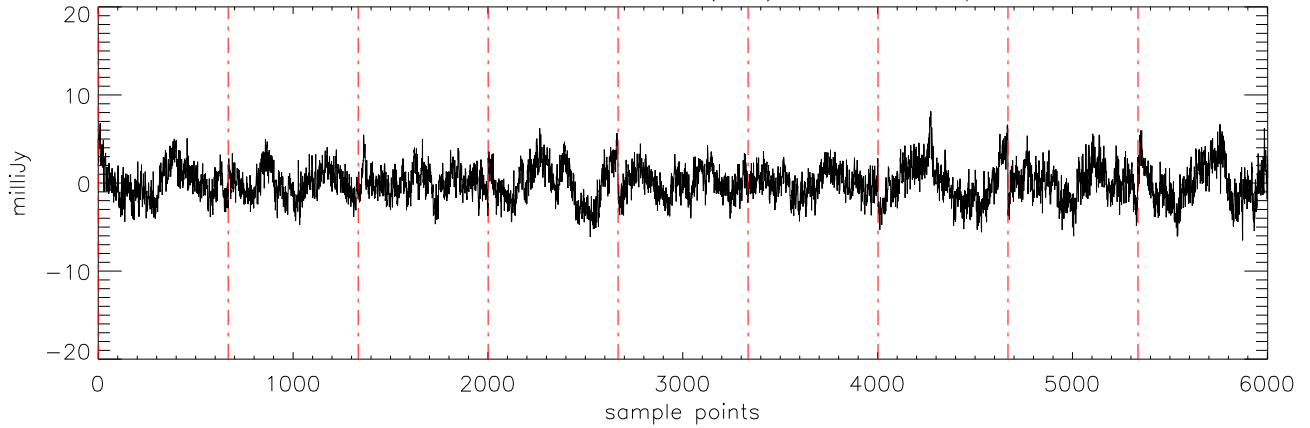
a2471 J09373487 07feb12 (AST) StokesQ freq:4750.
