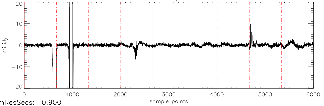
a2471 J09373487 07feb12 (AST) StokesU freq:4466.
