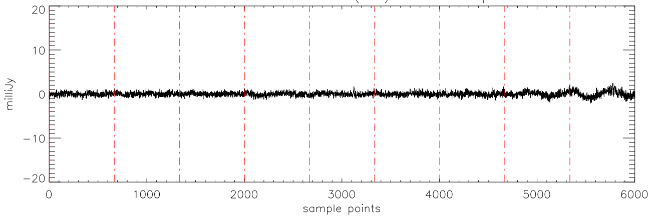
a2471 J09373487 07feb12 (AST) StokesV freq:4750.
