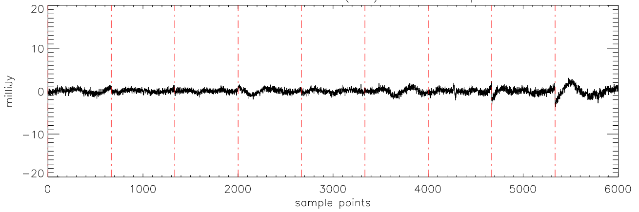
a2471 J09373487 07feb12 (AST) StokesU freq:4608.
