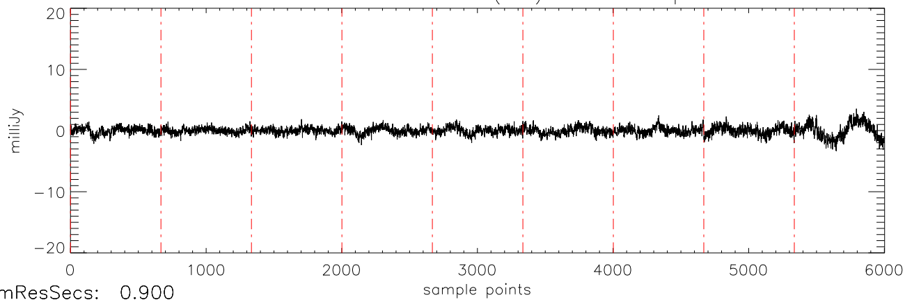
a2471 J09373487 07feb12 (AST) StokesU freq:5034.
