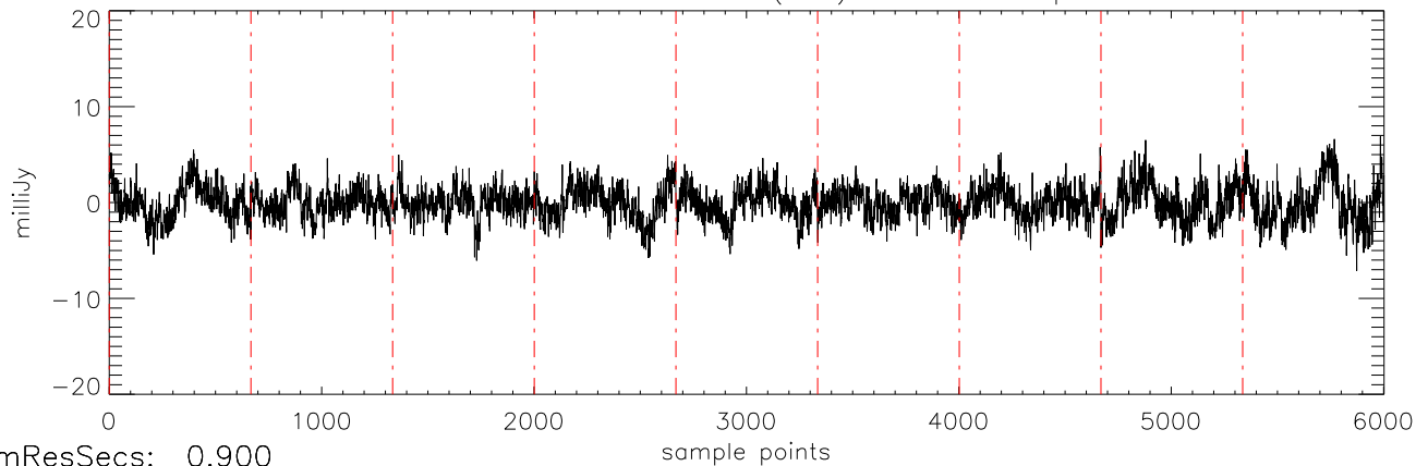
a2471 J09373487 07feb12 (AST) StokesQ freq:5034.
