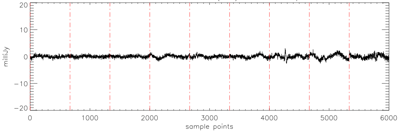
a2471 J09373487 07feb12 (AST) StokesU freq:4750.
