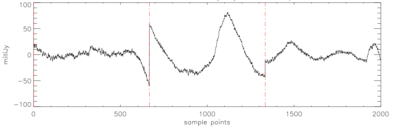
a2471 J08251958 09feb12 (AST) StokesI freq:5176.
