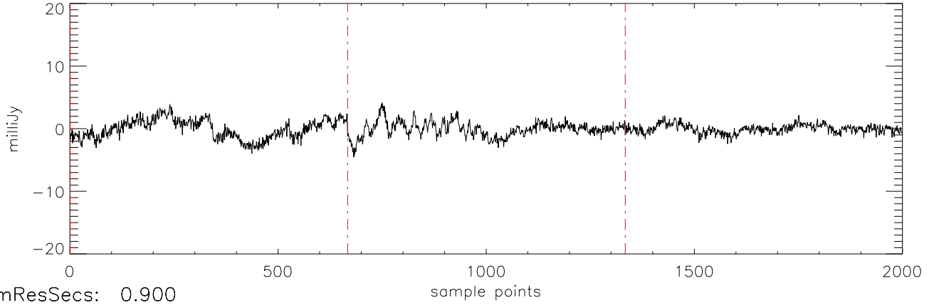
a2471 J08251958 09feb12 (AST) StokesU freq:5034.
