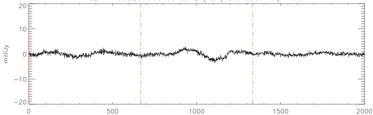
a2471 J08251958 09feb12 (AST) StokesU freq:4466.
