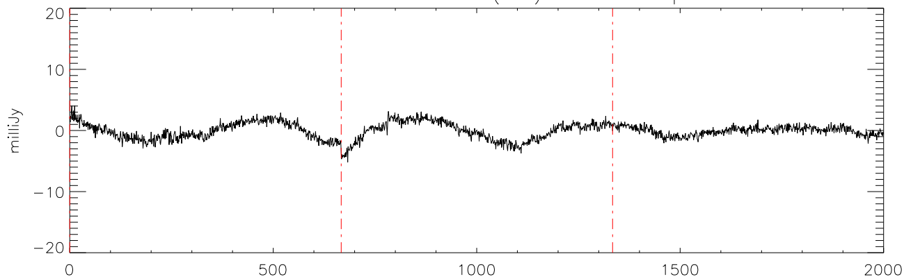
a2471 J08251958 09feb12 (AST) StokesU freq:4750.
