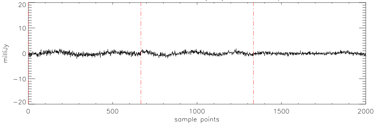
a2471 J08251958 09feb12 (AST) StokesV freq:4608.
