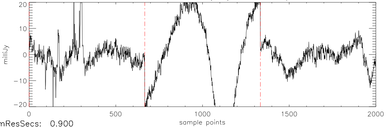
a2471 J08251958 09feb12 (AST) StokesQ freq:4466.
