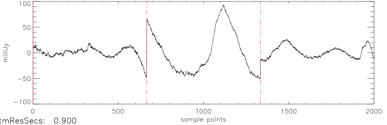
a2471 J08251958 09feb12 (AST) StokesI freq:5034.
