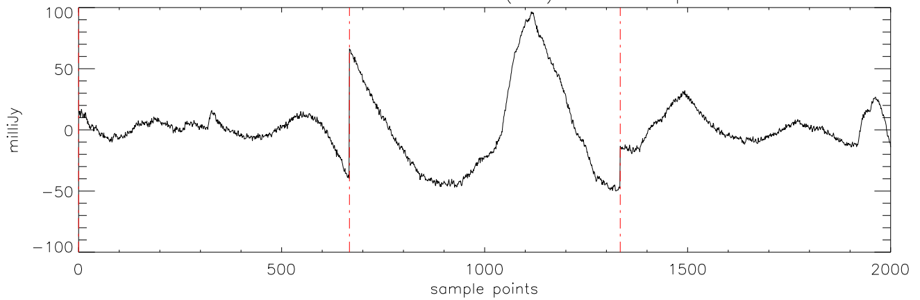
a2471 J08251958 09feb12 (AST) StokesI freq:4608.
