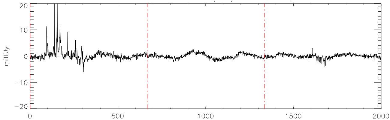
a2471 J08251958 09feb12 (AST) StokesU freq:4325.
