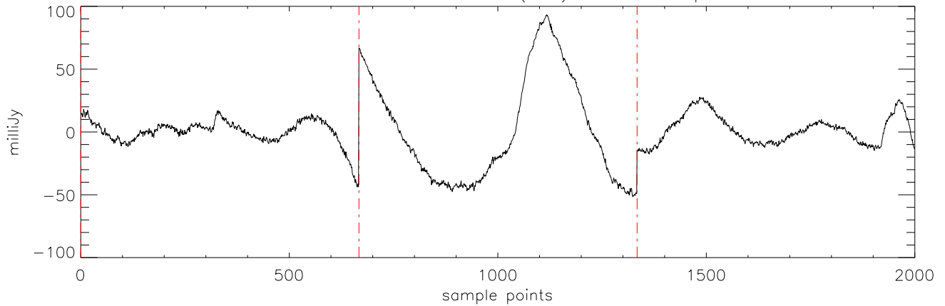
a2471 J08251958 09feb12 (AST) StokesI freq:4750.
