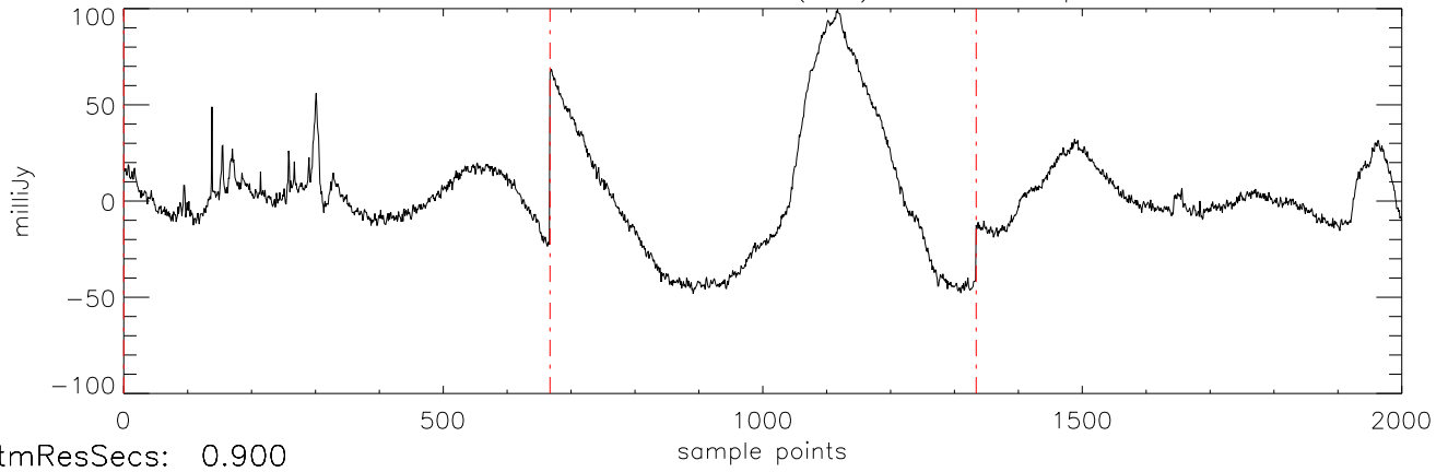
a2471 J08251958 09feb12 (AST) StokesI freq:4466.
