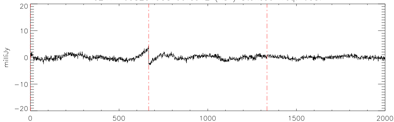
a2471 J08251958 09feb12 (AST) StokesU freq:4608.
