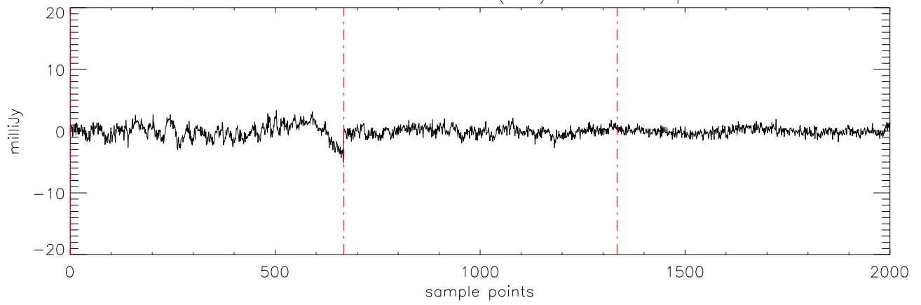
a2471 J08251958 09feb12 (AST) StokesV freq:5176.
