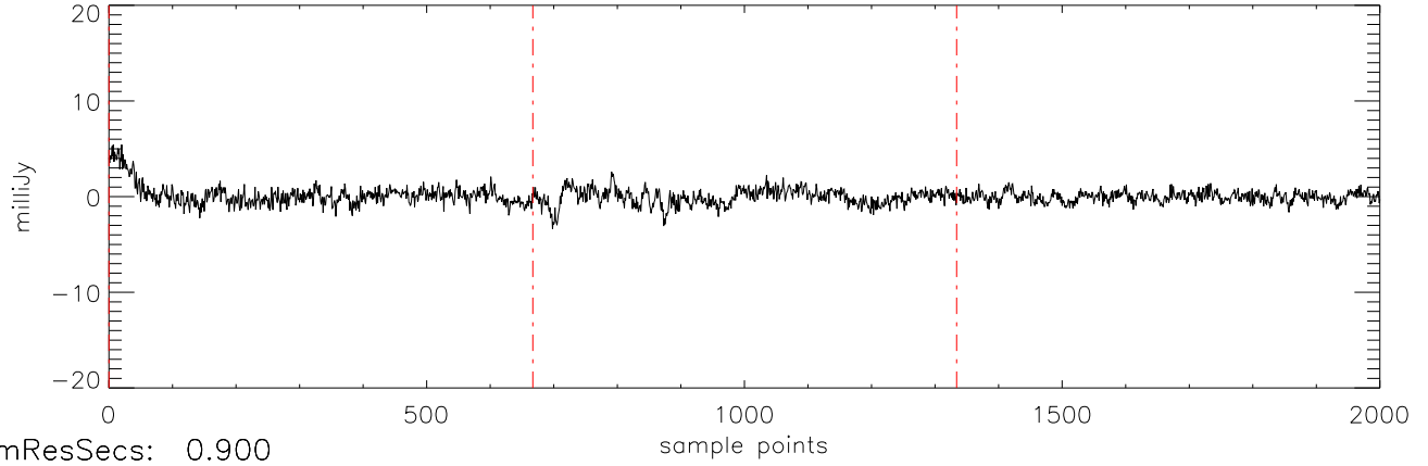
a2471 J08251958 09feb12 (AST) StokesV freq:5034.
