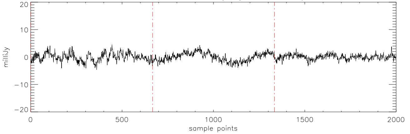
a2471 J08251958 09feb12 (AST) StokesU freq:5176.
