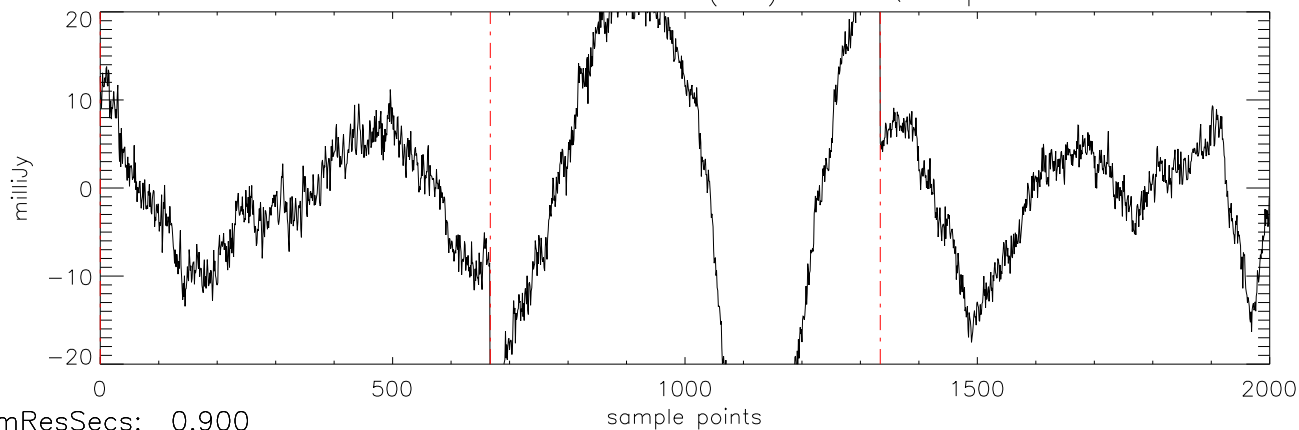
a2471 J08251958 09feb12 (AST) StokesQ freq:5034.
