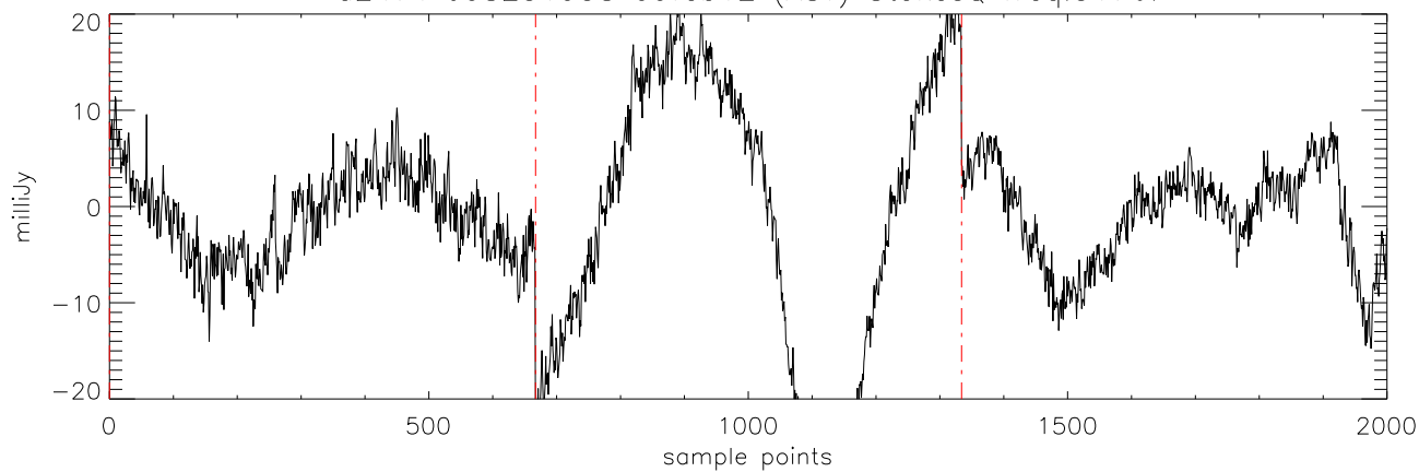
a2471 J08251958 09feb12 (AST) StokesQ freq:5176.
