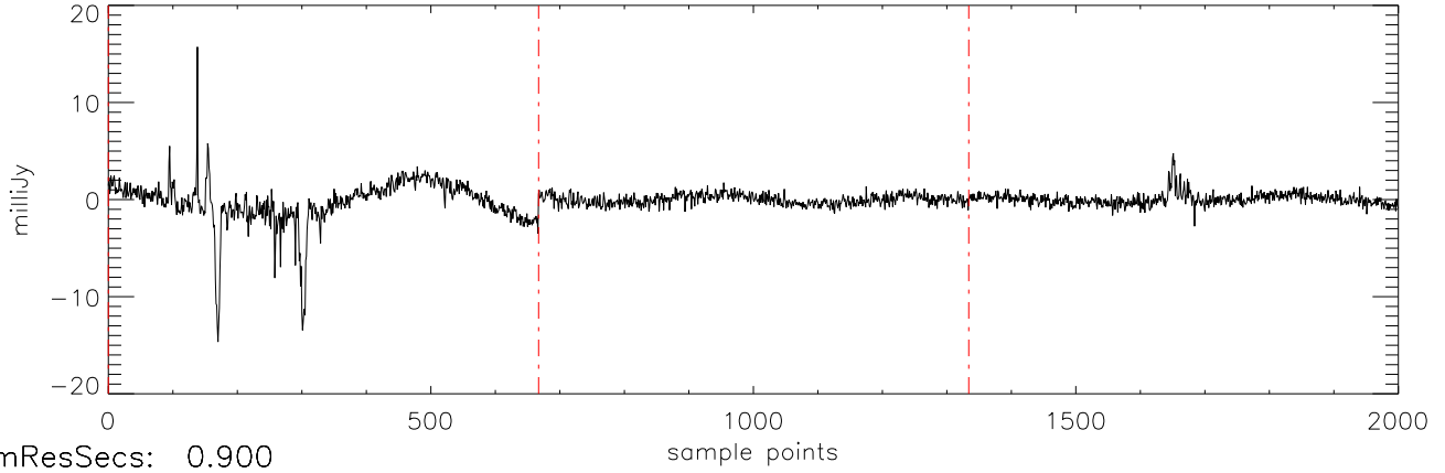
a2471 J08251958 09feb12 (AST) StokesV freq:4466.
