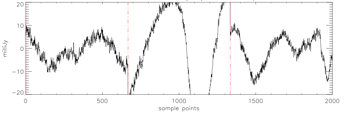
a2471 J08251958 09feb12 (AST) StokesQ freq:4750.
