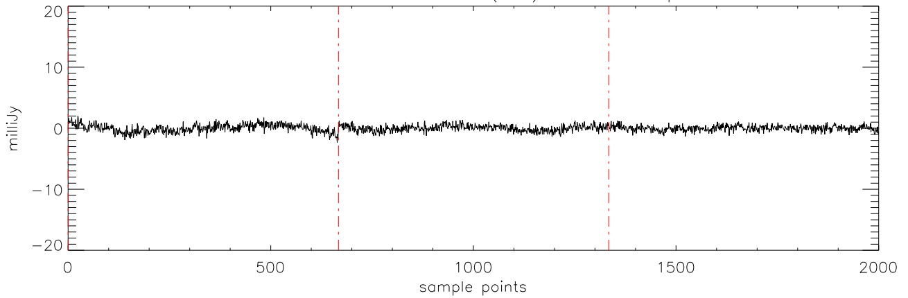
a2471 J08251958 09feb12 (AST) StokesV freq:4750.
