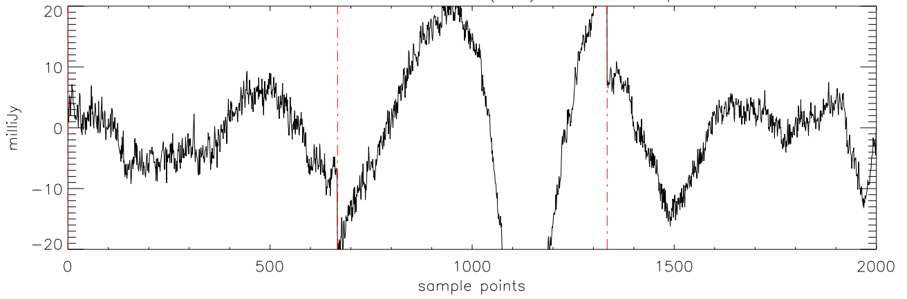
a2471 J08251958 09feb12 (AST) StokesQ freq:4608.
