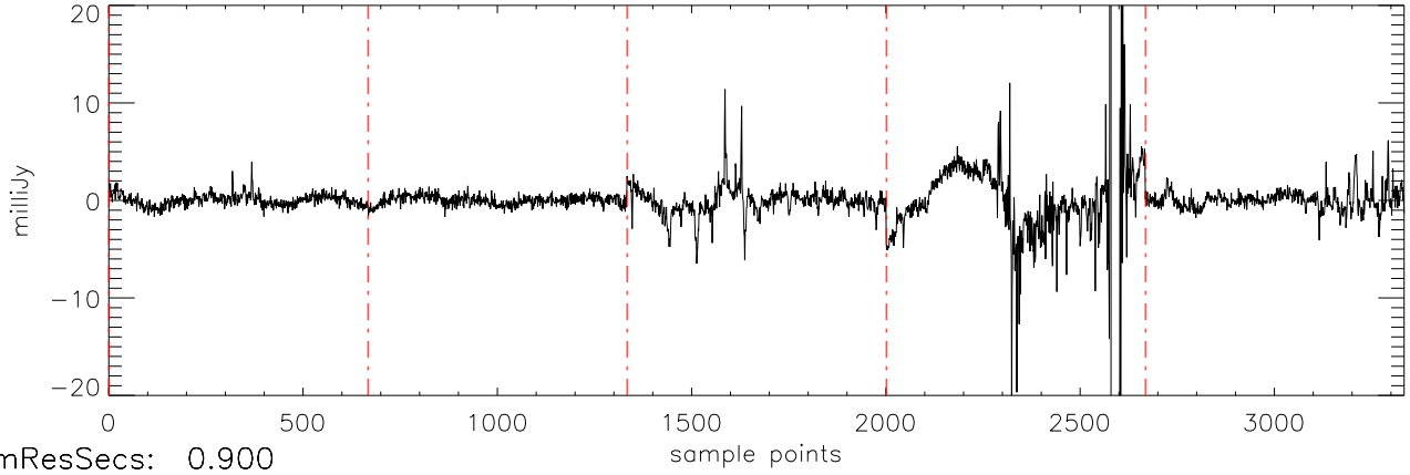
a2471 J07464256 06apr12 (AST) StokesU freq:4466.
