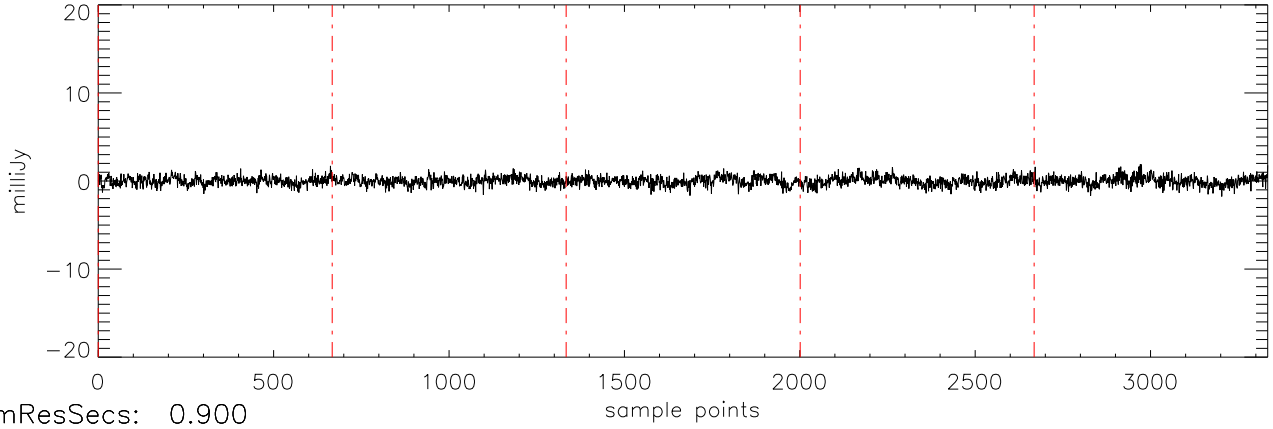
a2471 J07464256 06apr12 (AST) StokesV freq:5034.
