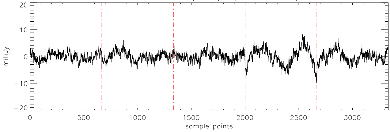
a2471 J07464256 06apr12 (AST) StokesQ freq:5176.
