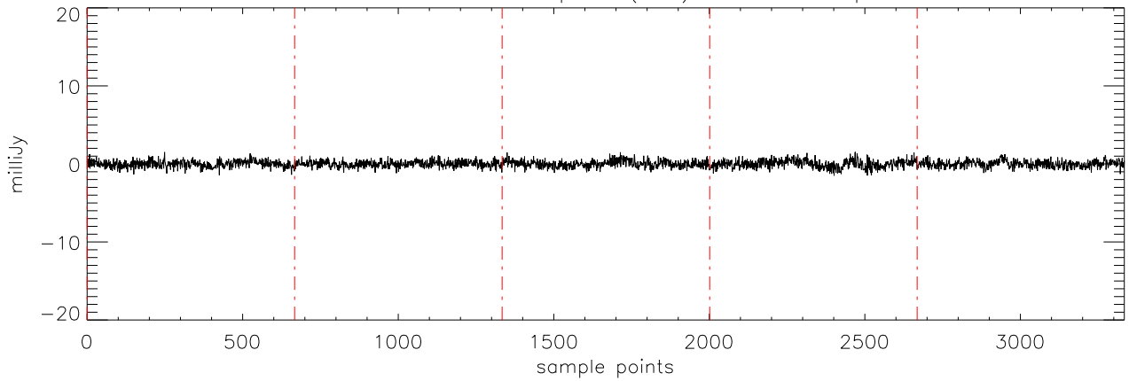
a2471 J07464256 06apr12 (AST) StokesV freq:4608.
