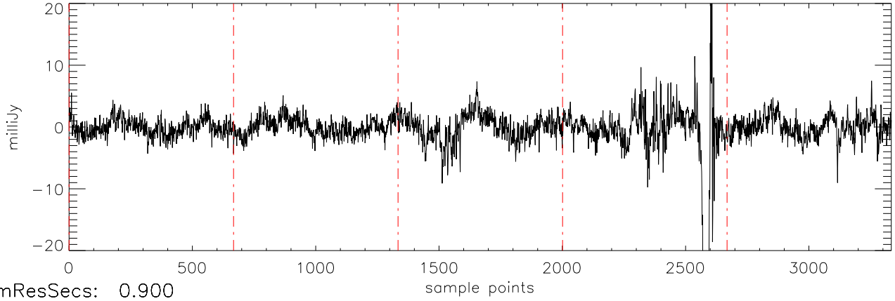
a2471 J07464256 06apr12 (AST) StokesQ freq:4466.
