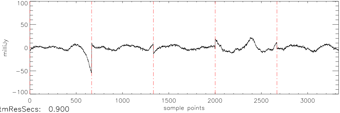
a2471 J07464256 06apr12 (AST) StokesI freq:5034.
