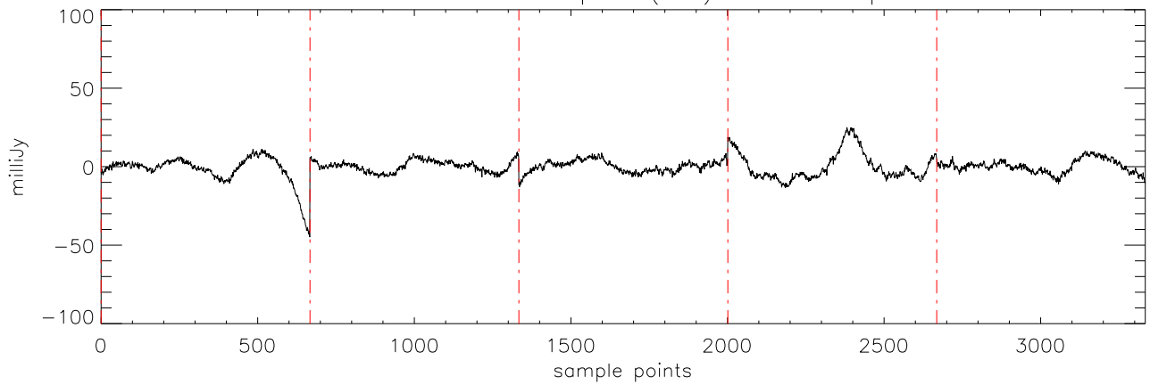
a2471 J07464256 06apr12 (AST) StokesI freq:5176.
