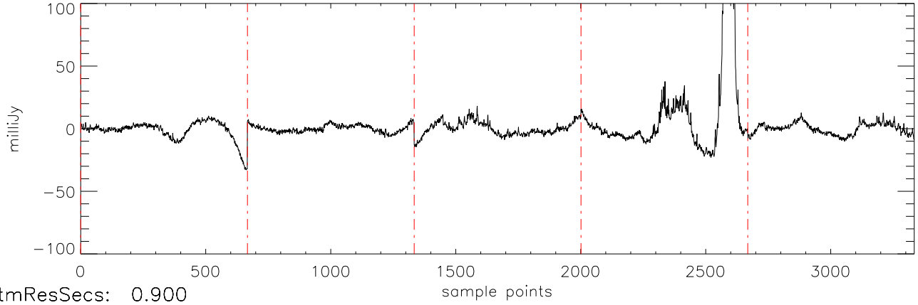
a2471 J07464256 06apr12 (AST) StokesI freq:4466.
