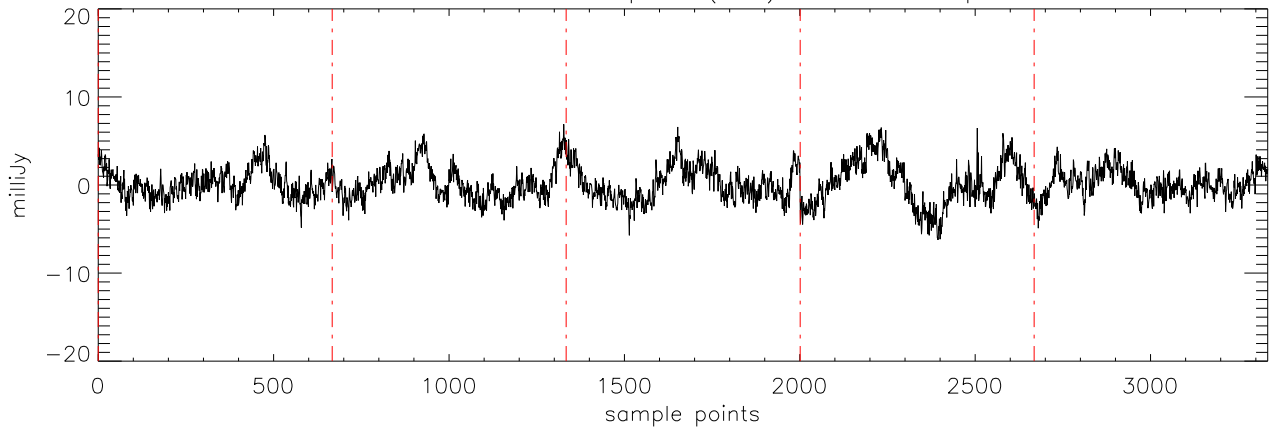
a2471 J07464256 06apr12 (AST) StokesQ freq:4608.
