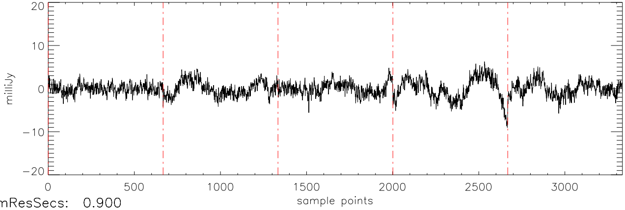
a2471 J07464256 06apr12 (AST) StokesQ freq:5034.
