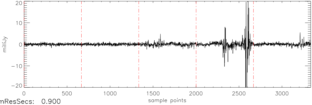
a2471 J07464256 06apr12 (AST) StokesV freq:4466.
