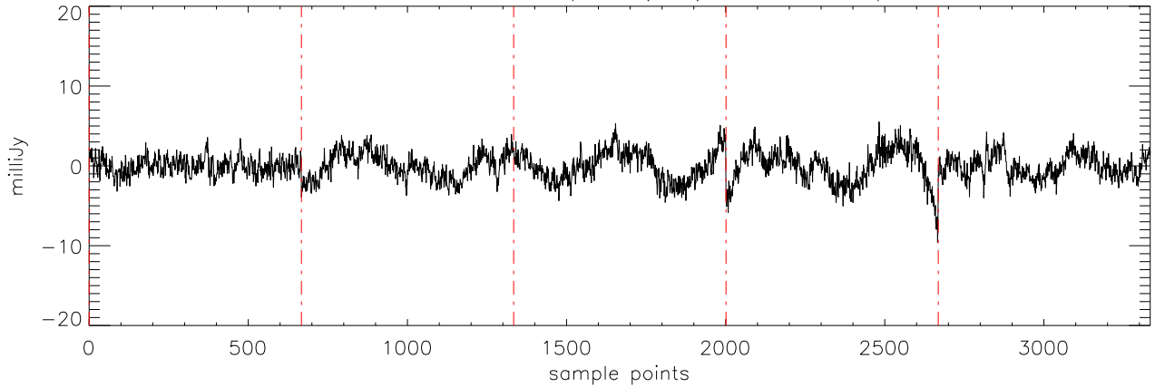
a2471 J07464256 06apr12 (AST) StokesQ freq:4750.
