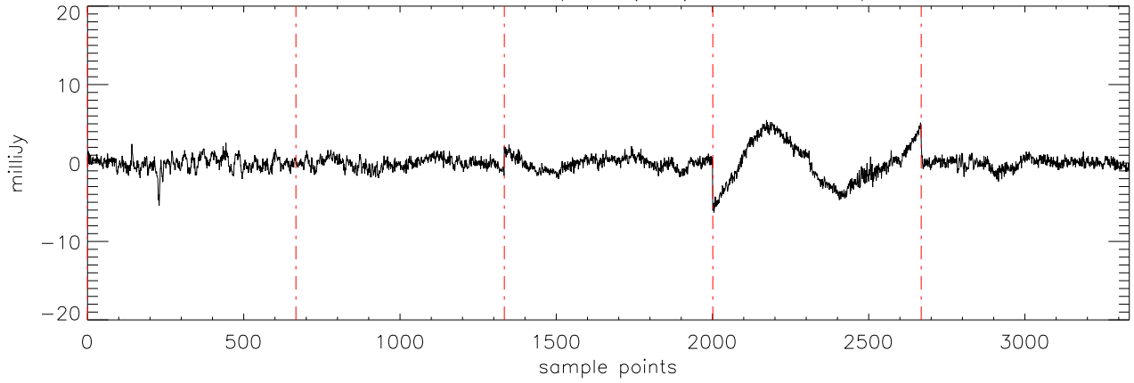
a2471 J07464256 06apr12 (AST) StokesU freq:4750.
