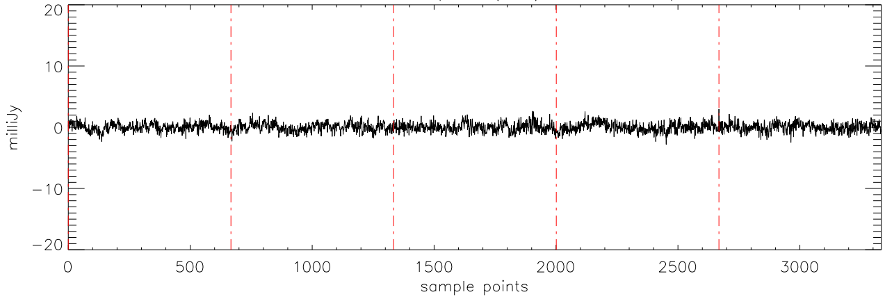
a2471 J07464256 06apr12 (AST) StokesV freq:5176.
