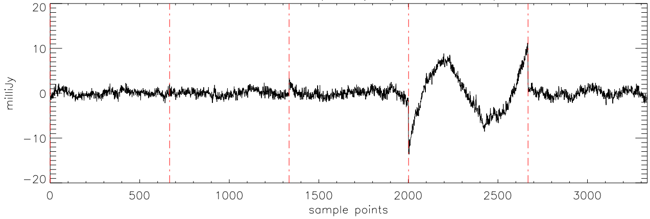
a2471 J07464256 06apr12 (AST) StokesU freq:5176.
