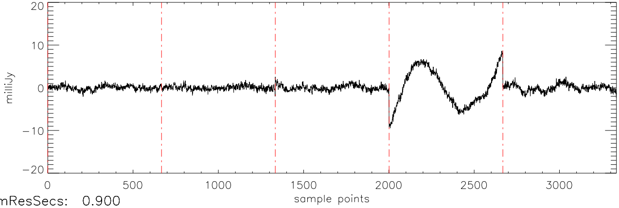
a2471 J07464256 06apr12 (AST) StokesU freq:5034.
