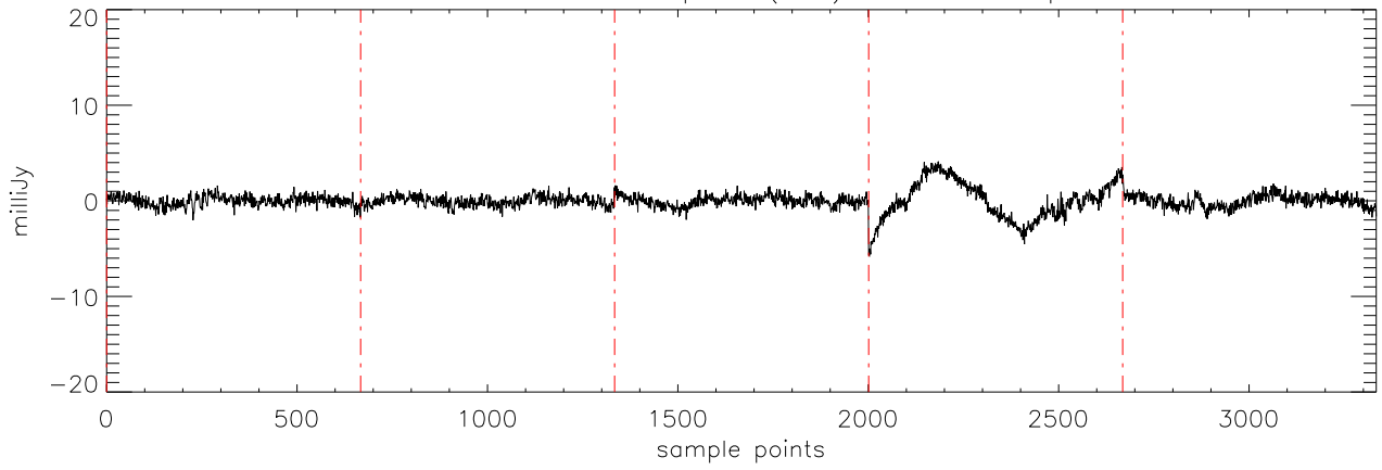
a2471 J07464256 06apr12 (AST) StokesU freq:4608.
