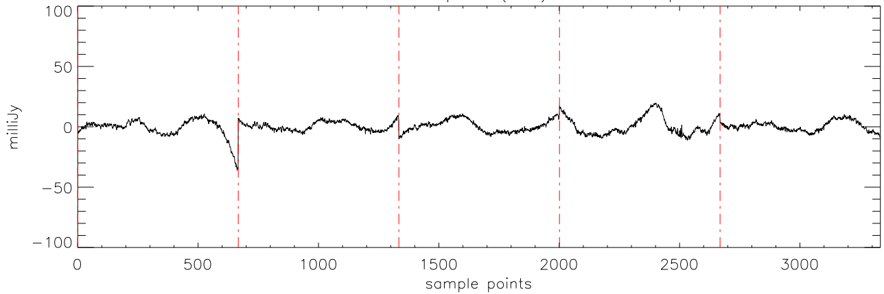
a2471 J07464256 06apr12 (AST) StokesI freq:4750.
