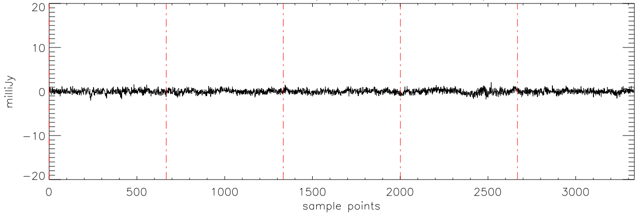
a2471 J07464256 06apr12 (AST) StokesV freq:4750.
