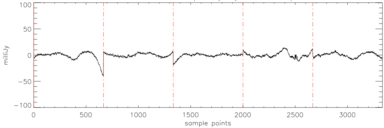
a2471 J07464256 06apr12 (AST) StokesI freq:4608.
