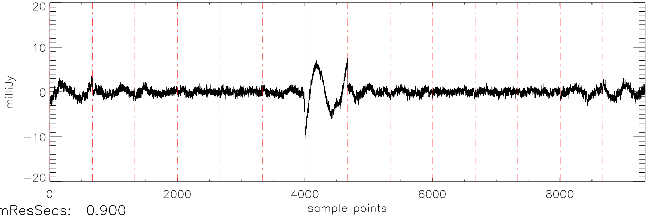
a2471 J07464256 07feb12 (AST) StokesU freq:5034.
