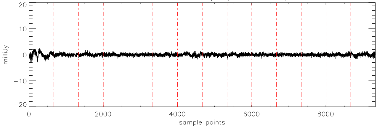
a2471 J07464256 07feb12 (AST) StokesV freq:4608.
