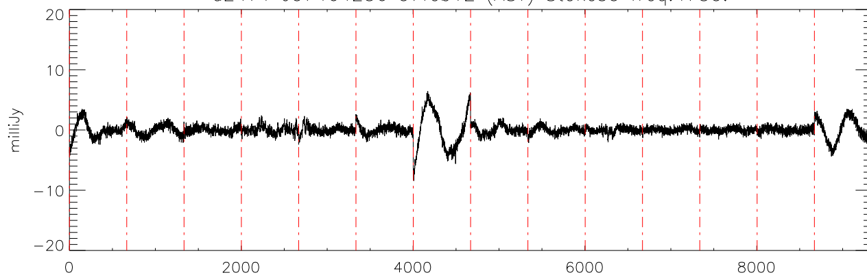
a2471 J07464256 07feb12 (AST) StokesU freq:4750.
