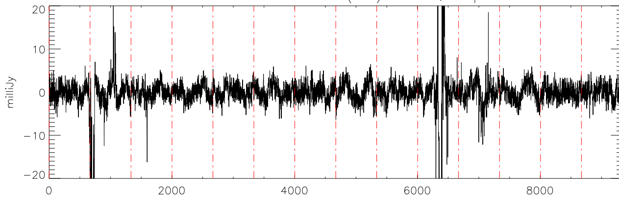
a2471 J07464256 07feb12 (AST) StokesQ freq:4325.
