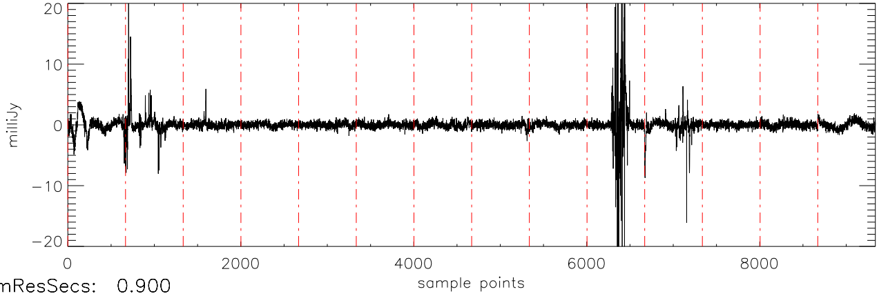
a2471 J07464256 07feb12 (AST) StokesV freq:4466.
