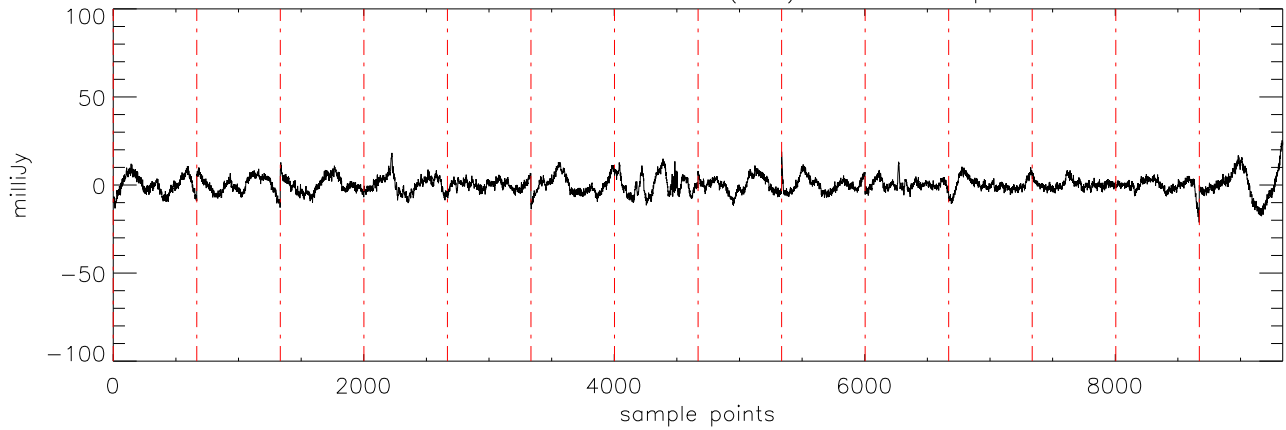
α2471 J07464256 07feb12 (AST) StokesI freq:4750.
