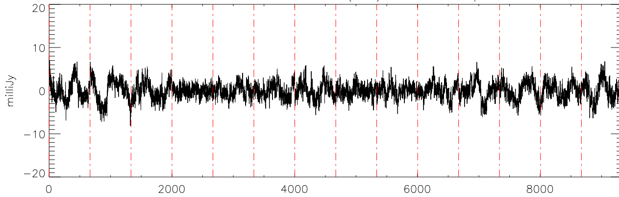
a2471 J07464256 07feb12 (AST) StokesQ freq:4750.
