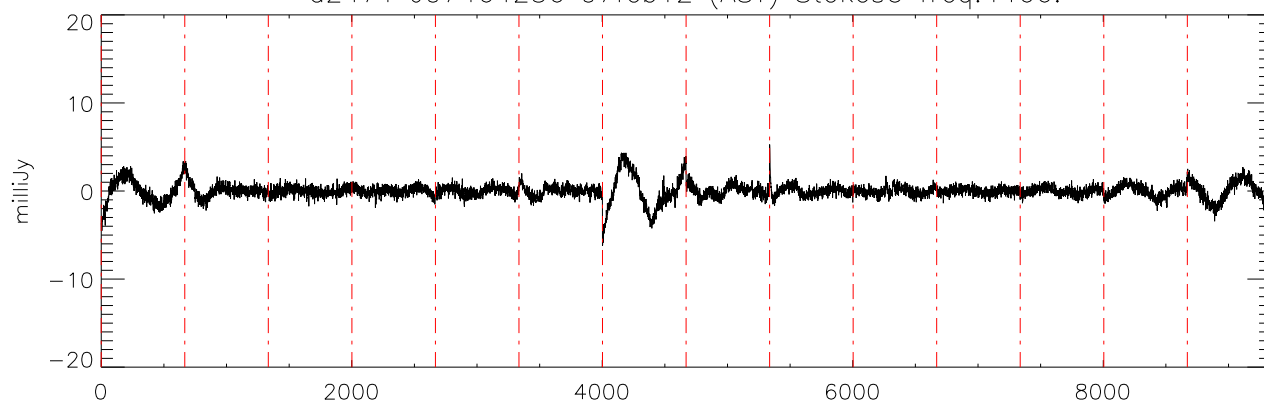
a2471 J07464256 07feb12 (AST) StokesU freq:4466.
