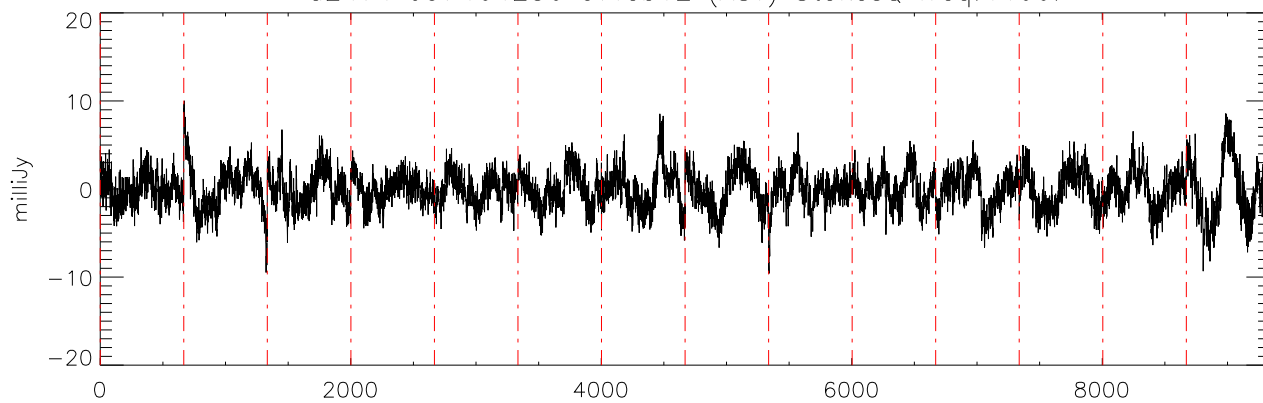
a2471 J07464256 07feb12 (AST) StokesQ freq:4466.
