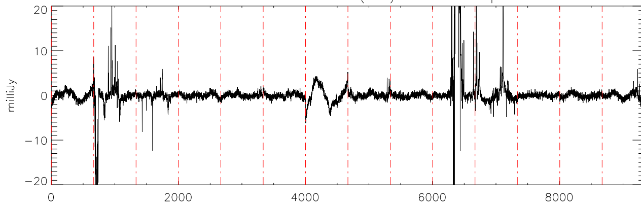
a2471 J07464256 07feb12 (AST) StokesU freq:4325.
