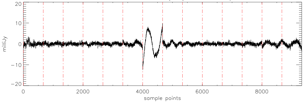
a2471 J07464256 07feb12 (AST) StokesU freq:5176.
