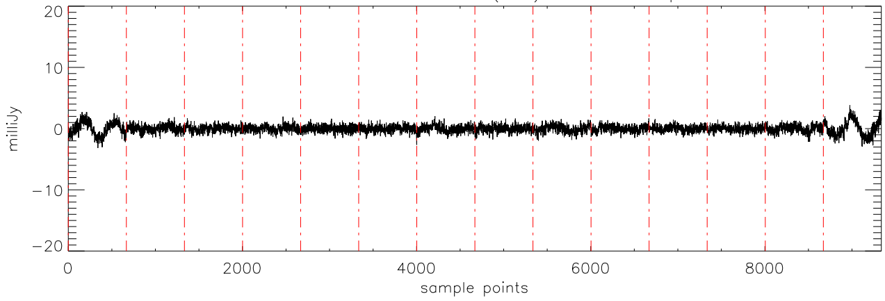
a2471 J07464256 07feb12 (AST) StokesV freq:5176.
