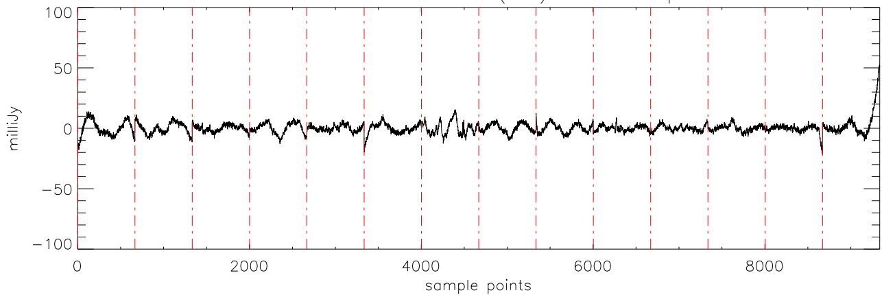
α2471 J07464256 07feb12 (AST) StokesI freq:4608.
