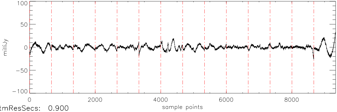
a2471 J07464256 07feb12 (AST) StokesI freq:5034.
