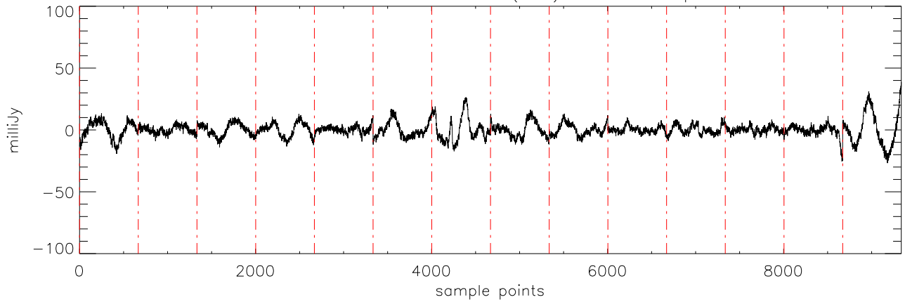
a2471 J07464256 07feb12 (AST) StokesI freq:5176.
