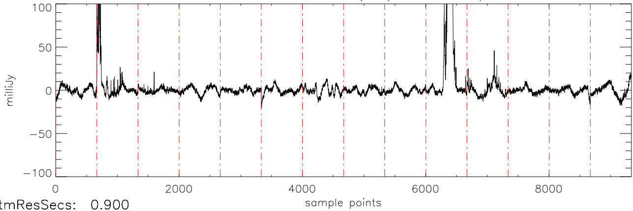
α2471 J07464256 07feb12 (AST) StokesI freq:4466.
