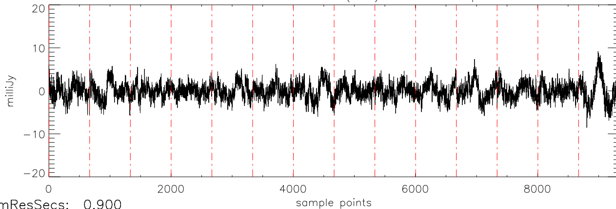
a2471 J07464256 07feb12 (AST) StokesQ freq:5034.
