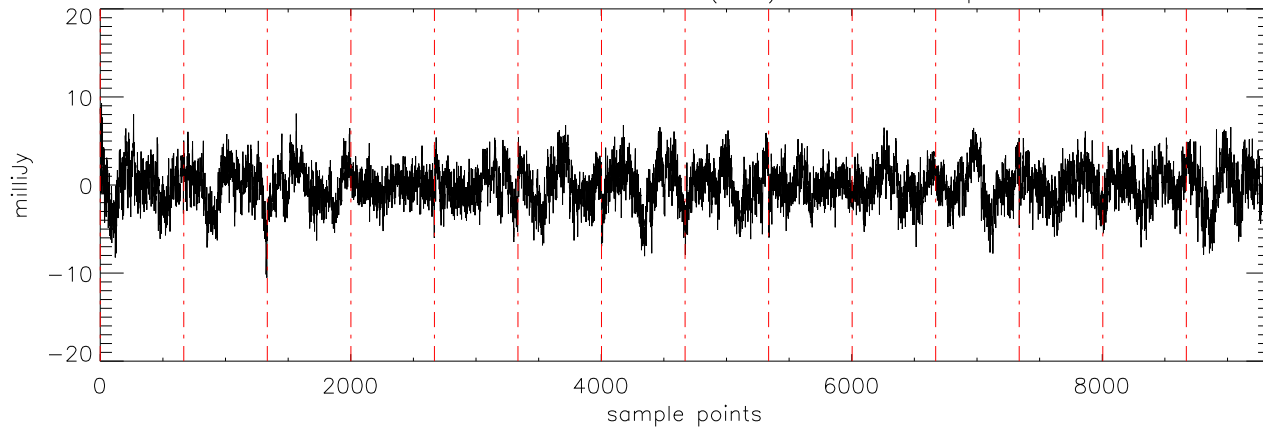
a2471 J07464256 07feb12 (AST) StokesQ freq:5176.
