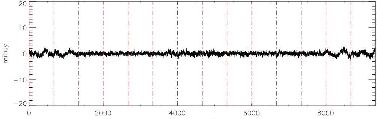
a2471 J07464256 07feb12 (AST) StokesV freq:4892.
