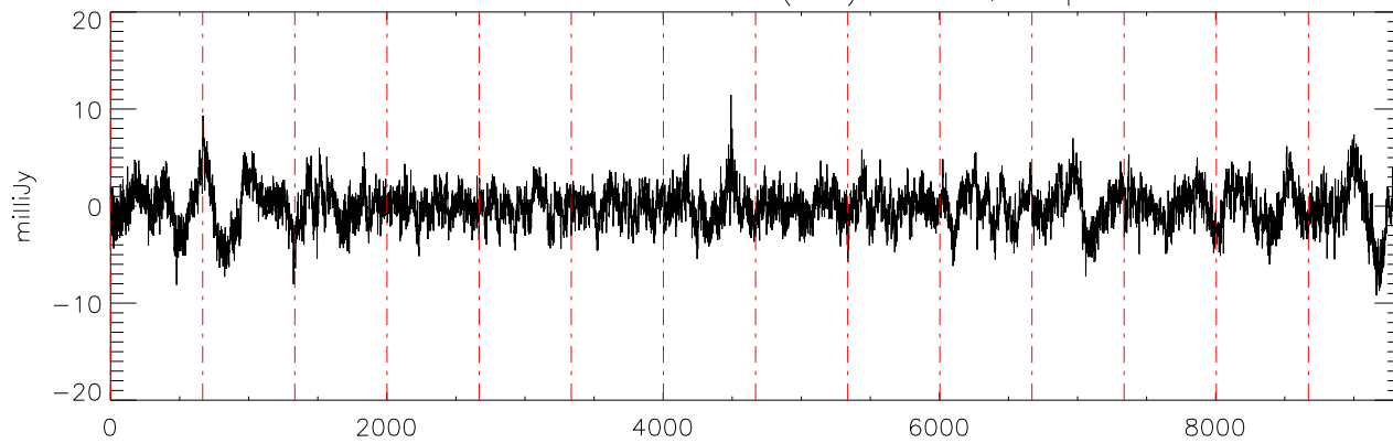
a2471 J07464256 07feb12 (AST) StokesQ freq:4608.
