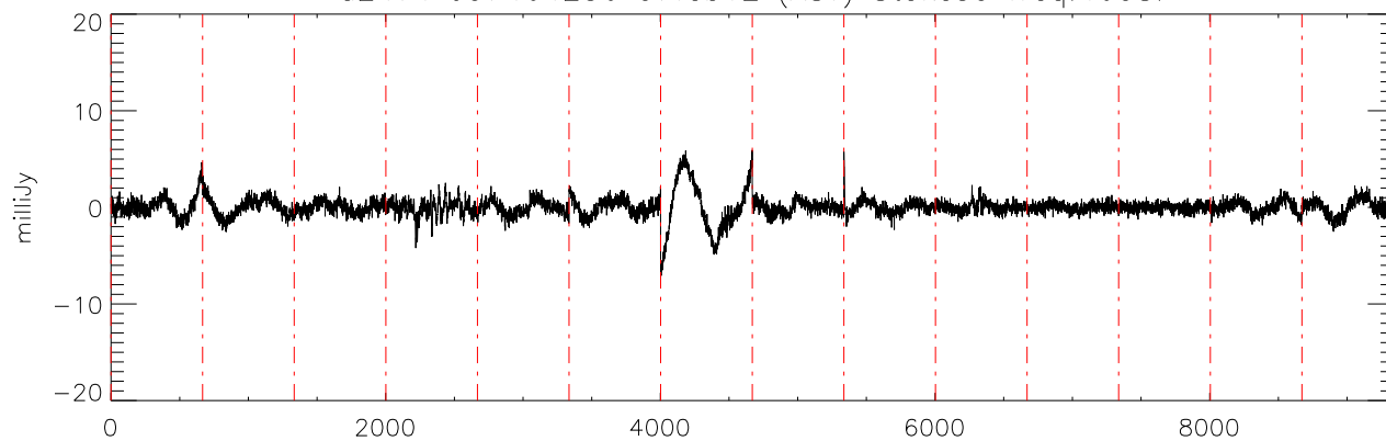
a2471 J07464256 07feb12 (AST) StokesU freq:4608.
