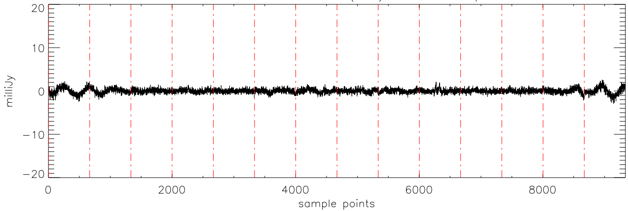
a2471 J07464256 07feb12 (AST) StokesV freq:4750.
