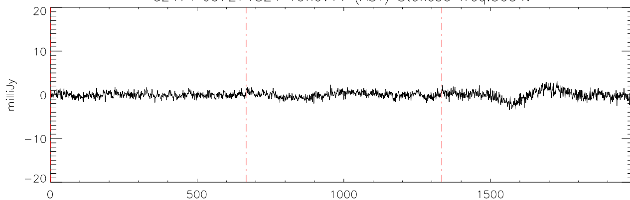
a2471 J07271824 19nov11 (AST) StokesU freq:5034.
