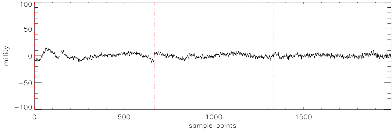
a2471 J07271824 19nov11 (AST) StokesI freq:4750.
