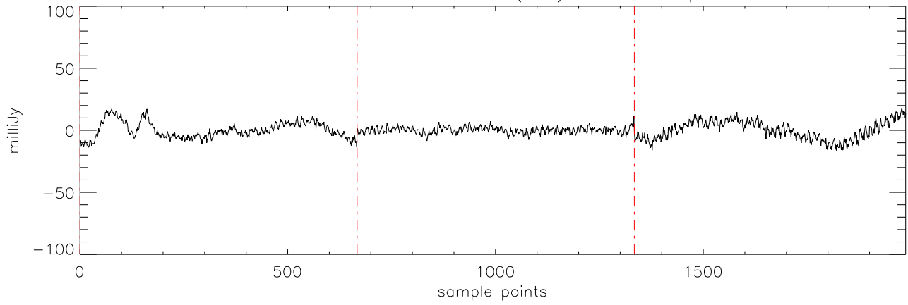
a2471 J07271824 19nov11 (AST) StokesI freq:5176.
