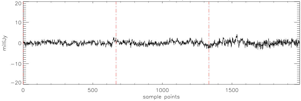
a2471 J07271824 19nov11 (AST) StokesV freq:5176.
