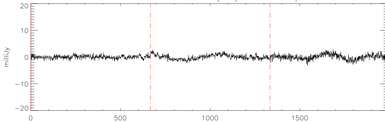
a2471 J07271824 19nov11 (AST) StokesU freq:4892.
