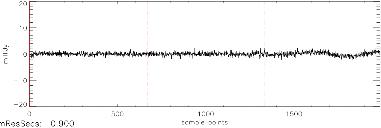
a2471 J07271824 19nov11 (AST) StokesV freq:4466.
