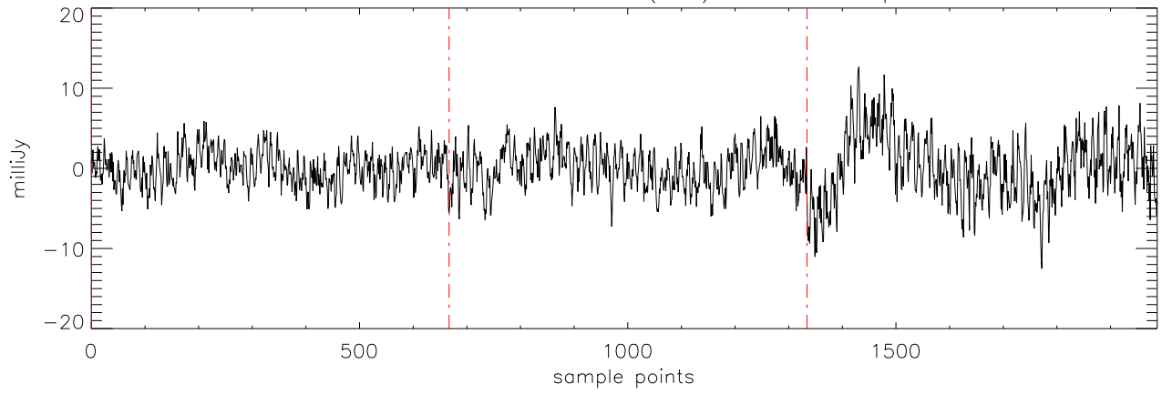
a2471 J07271824 19nov11 (AST) StokesQ freq:5176.
