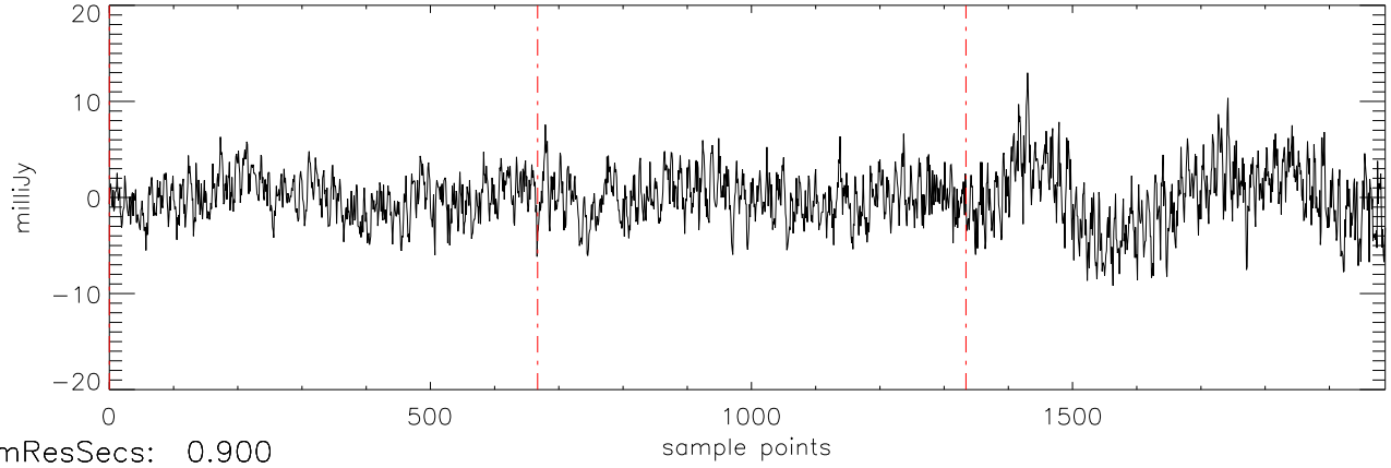
a2471 J07271824 19nov11 (AST) StokesQ freq:5034.
