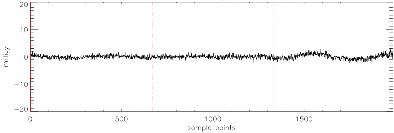
a2471 J07271824 19nov11 (AST) StokesV freq:4750.
