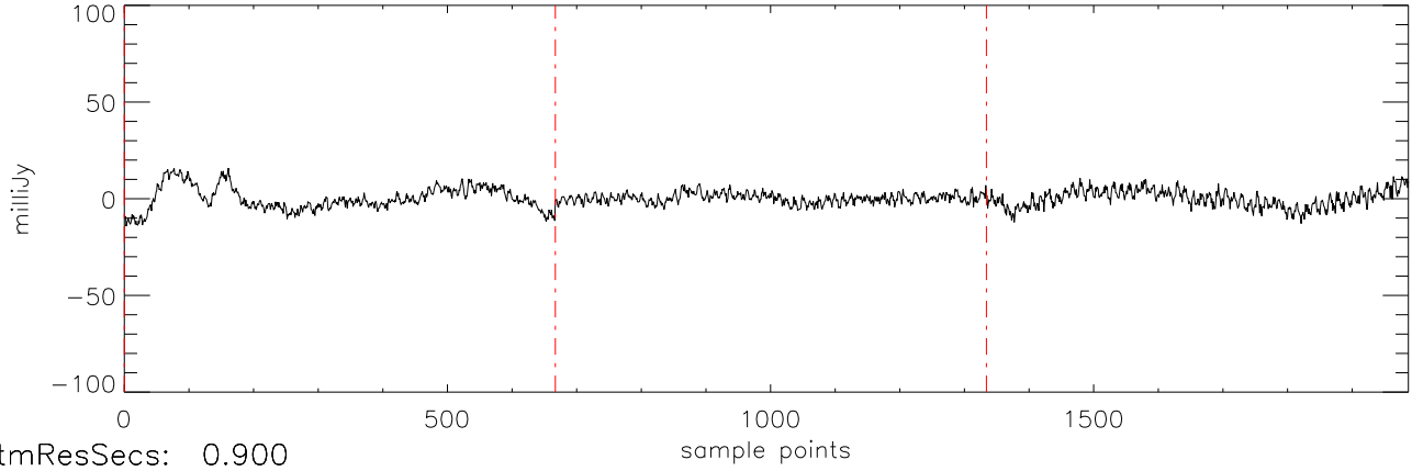
a2471 J07271824 19nov11 (AST) StokesI freq:5034.
