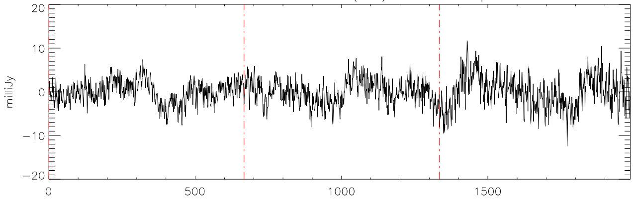
a2471 J07271824 19nov11 (AST) StokesQ freq:4466.
