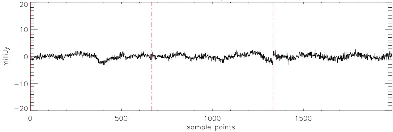
a2471 J07271824 19nov11 (AST) StokesU freq:4750.
