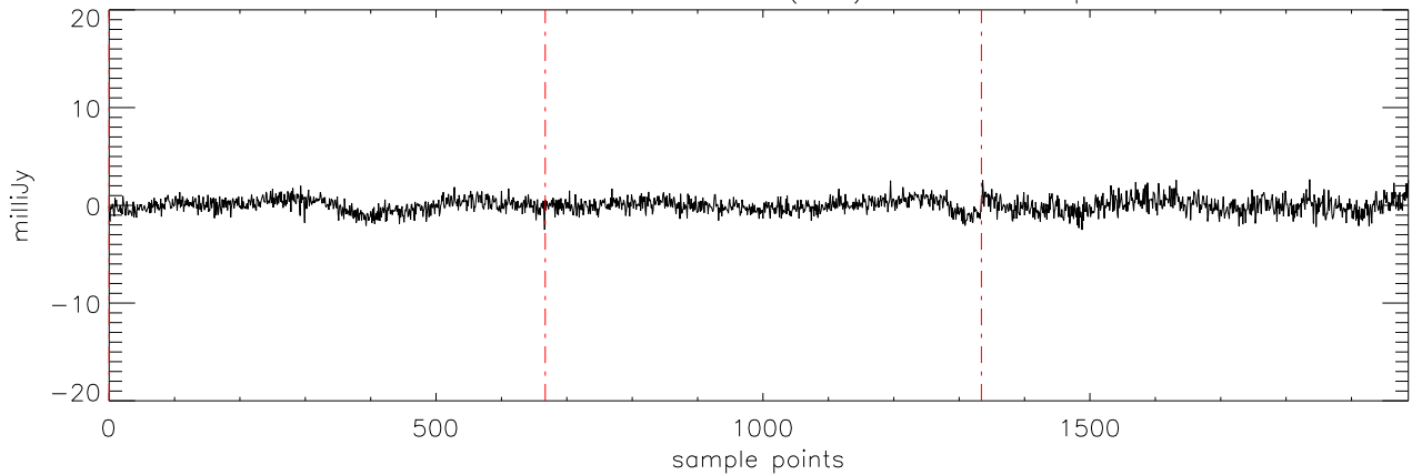
a2471 J07271824 19nov11 (AST) StokesU freq:4608.
