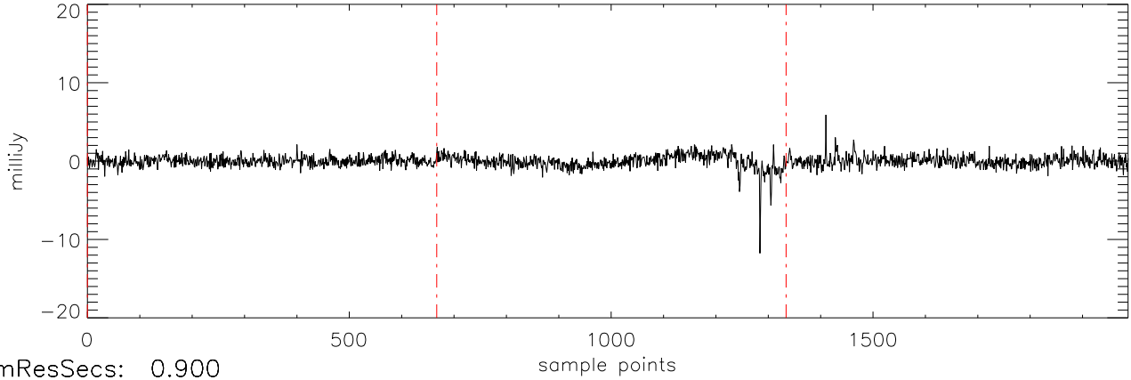
a2471 J07271824 19nov11 (AST) StokesU freq:4466.
