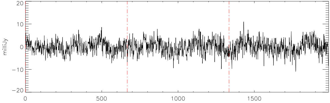
a2471 J07271824 19nov11 (AST) StokesQ freq:4325.
