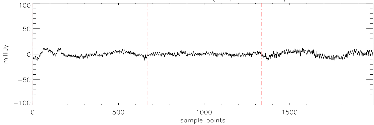
a2471 J07271824 19nov11 (AST) StokesI freq:4608.
