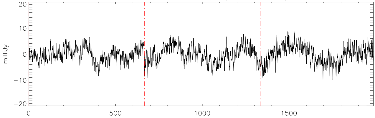
a2471 J07271824 19nov11 (AST) StokesQ freq:4608.
