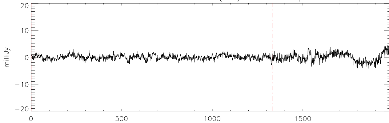
a2471 J07271824 19nov11 (AST) StokesU freq:5176.
