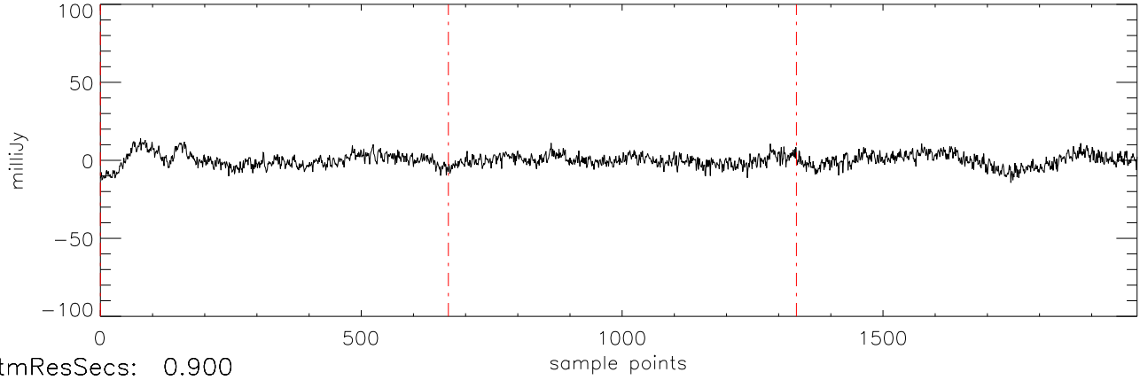
a2471 J07271824 19nov11 (AST) StokesI freq:4466.
