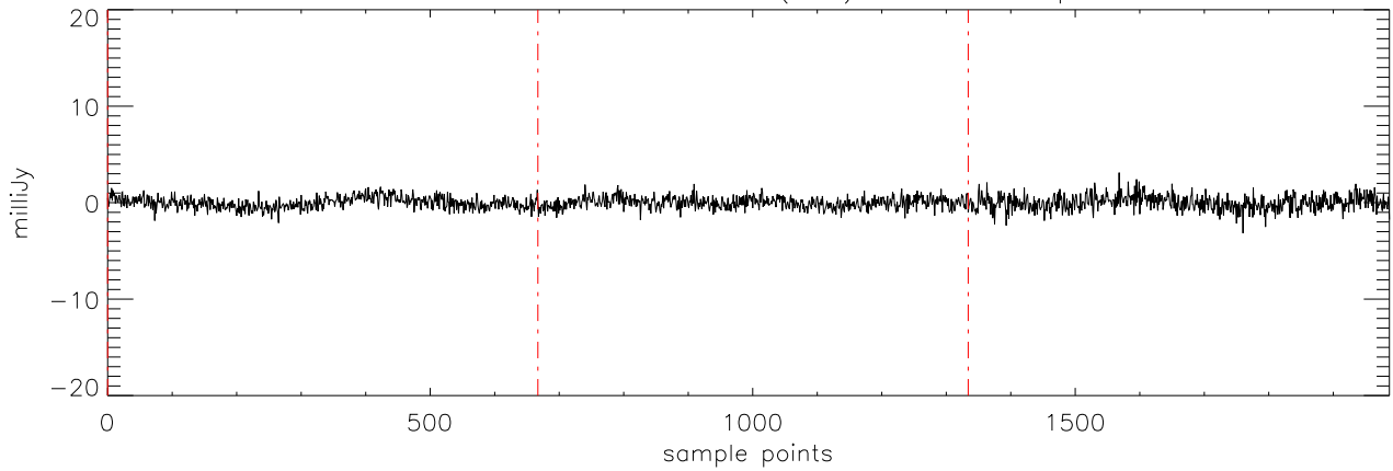
a2471 J07271824 19nov11 (AST) StokesV freq:4608.
