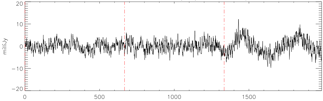
a2471 J07271824 19nov11 (AST) StokesQ freq:4750.
