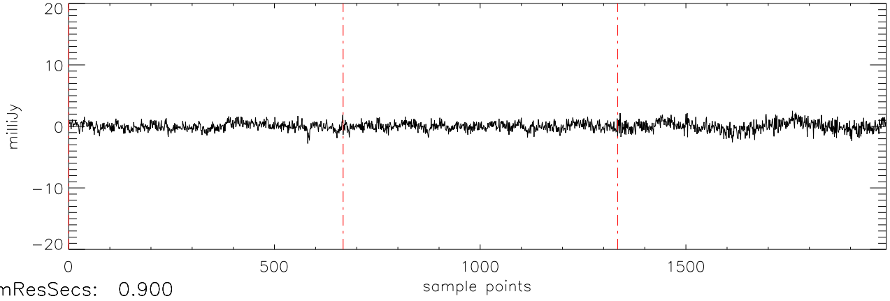
a2471 J07271824 19nov11 (AST) StokesV freq:5034.
