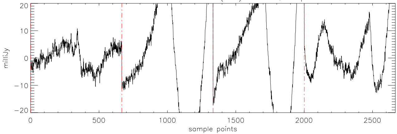
a2471 J07003664 09feb12 (AST) StokesQ freq:4608.
