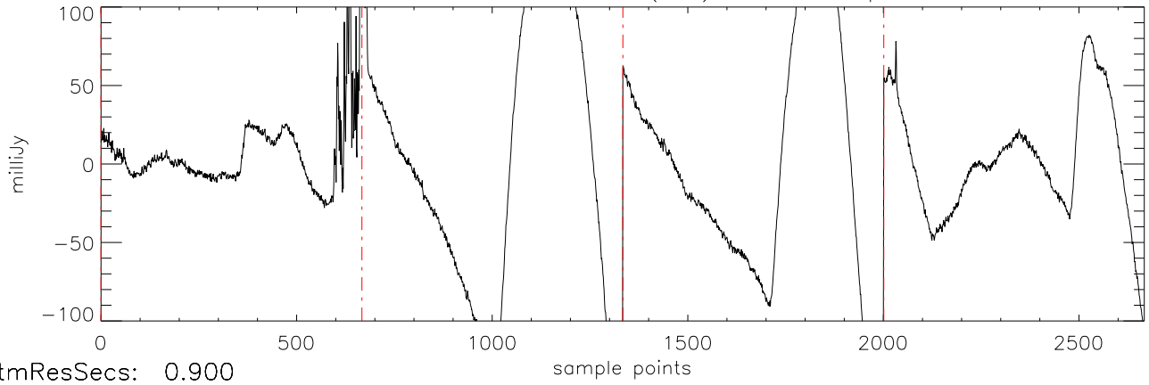
a2471 J07003664 09feb12 (AST) StokesI freq:4466.
