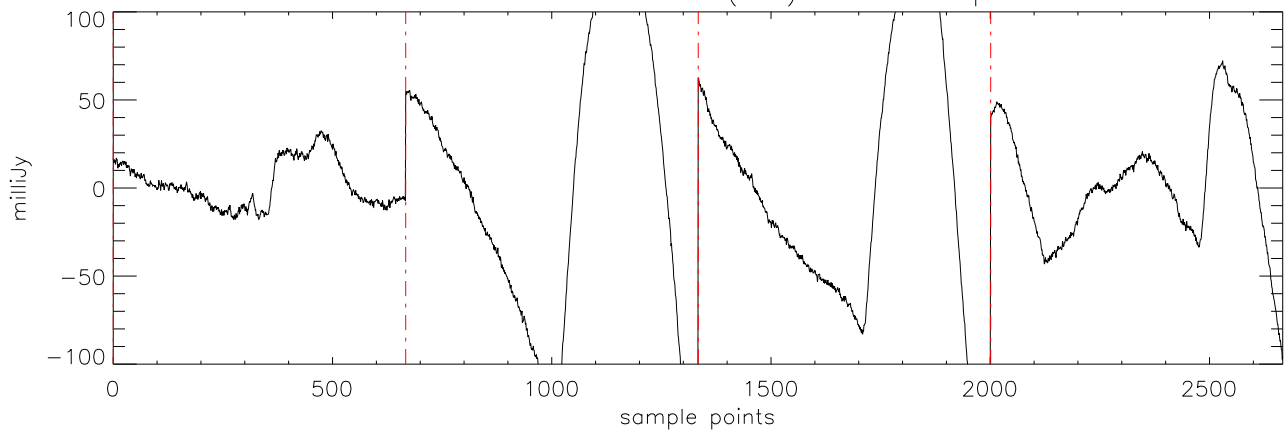
a2471 J07003664 09feb12 (AST) StokesI freq:4750.
