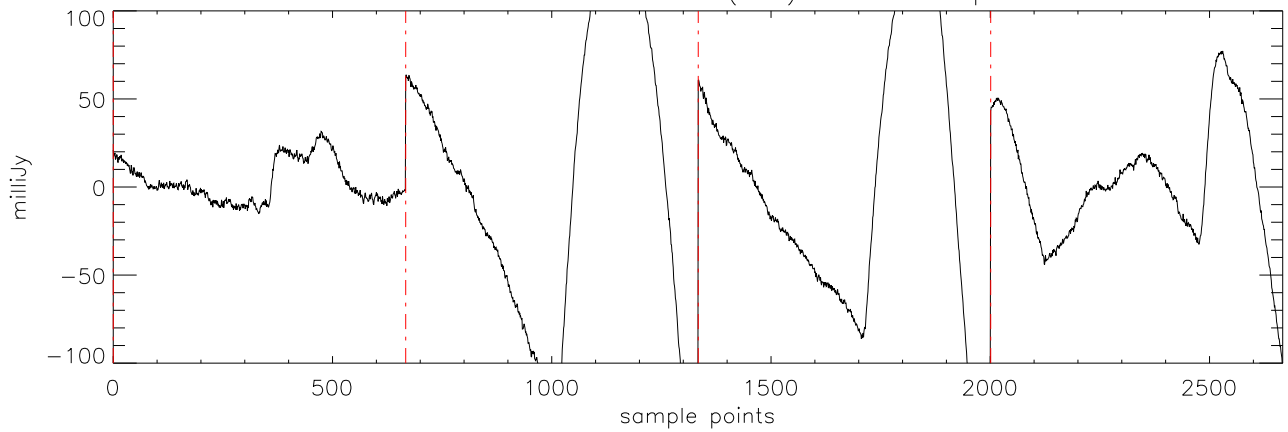
a2471 J07003664 09feb12 (AST) StokesI freq:4608.
