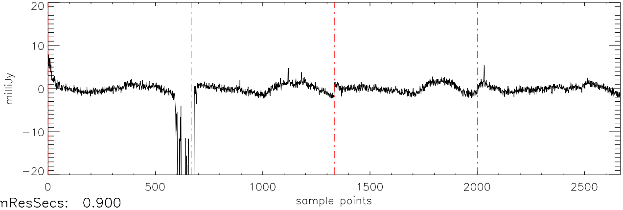
a2471 J07003664 09feb12 (AST) StokesU freq:4466.
