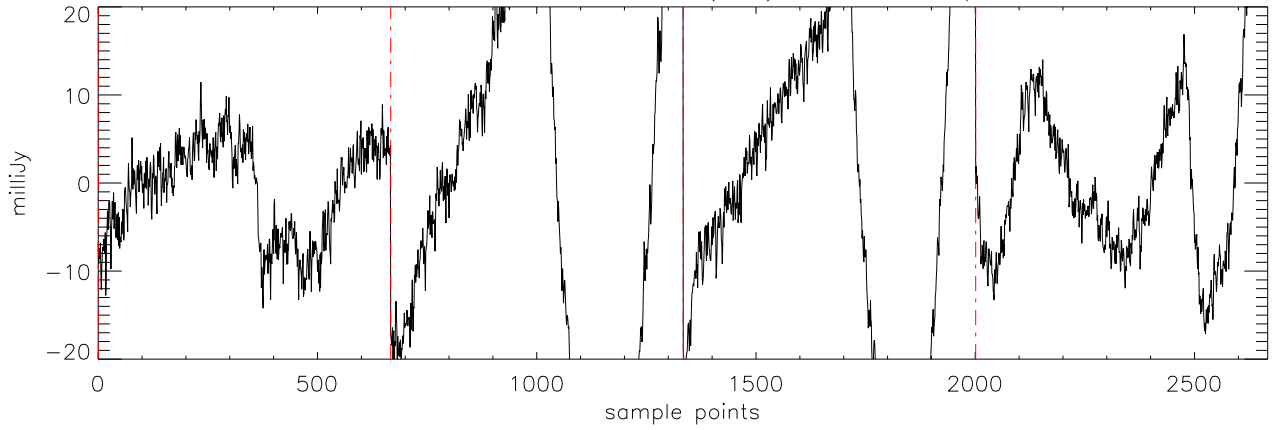
a2471 J07003664 09feb12 (AST) StokesQ freq:5176.
