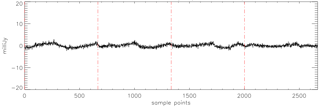
a2471 J07003664 09feb12 (AST) StokesU freq:4750.
