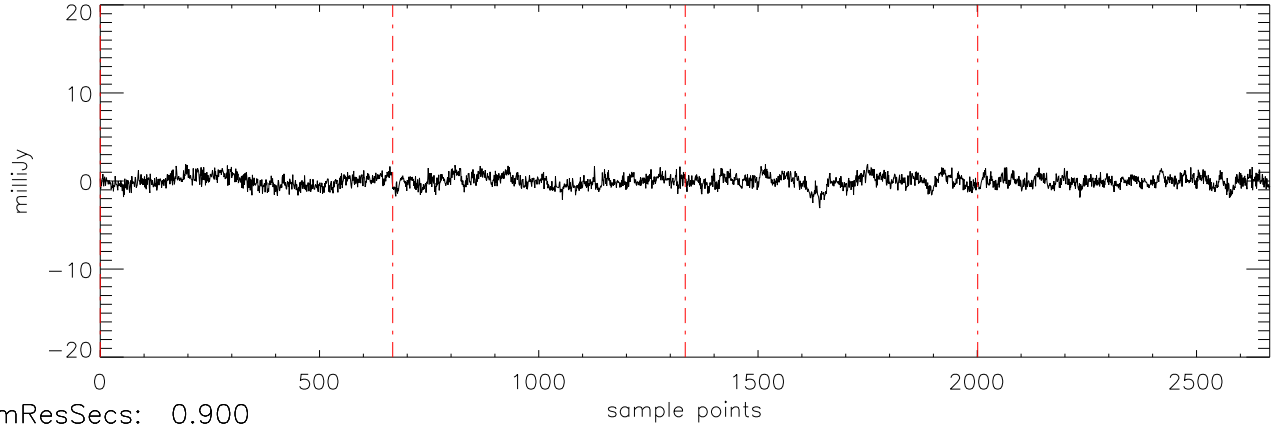
a2471 J07003664 09feb12 (AST) StokesV freq:5034.
