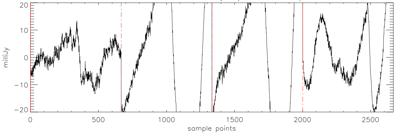
a2471 J07003664 09feb12 (AST) StokesQ freq:4750.
