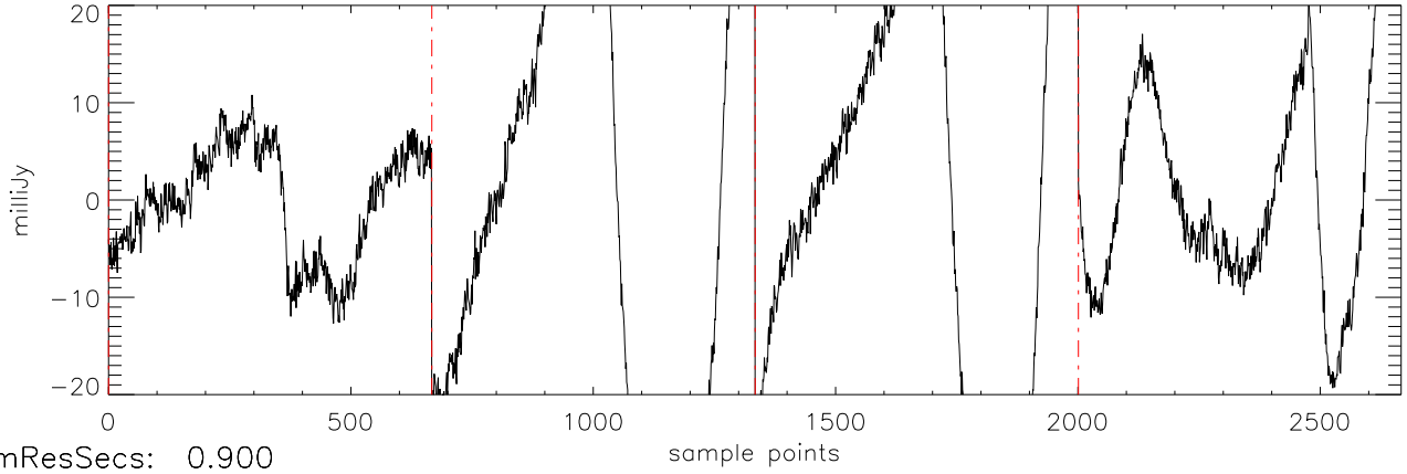
a2471 J07003664 09feb12 (AST) StokesQ freq:5034.
