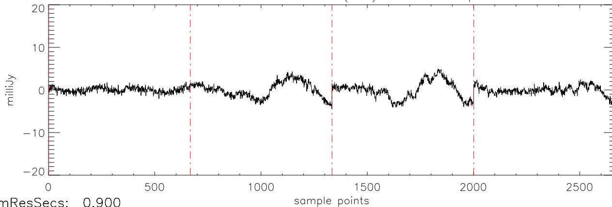
a2471 J07003664 09feb12 (AST) StokesU freq:5034.
