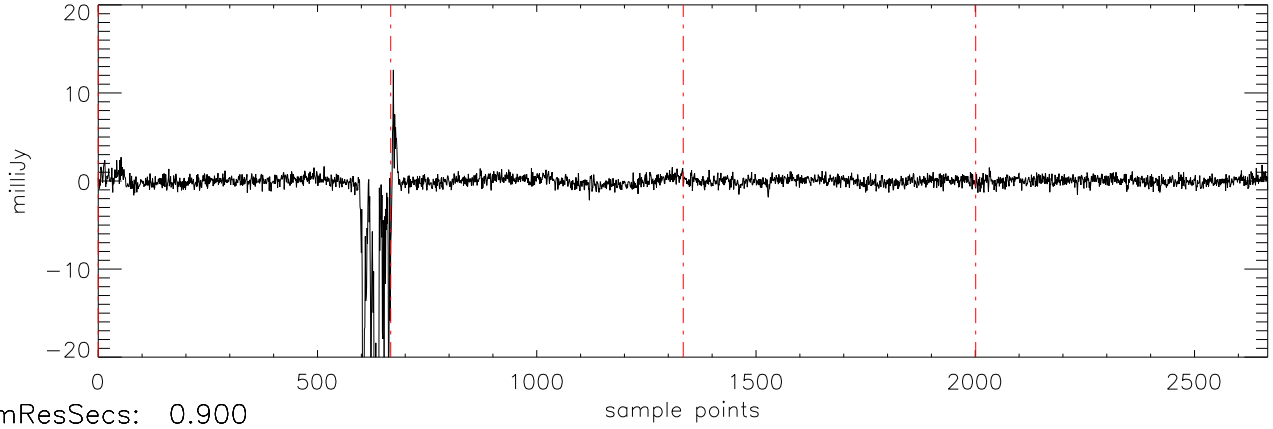
a2471 J07003664 09feb12 (AST) StokesV freq:4466.
