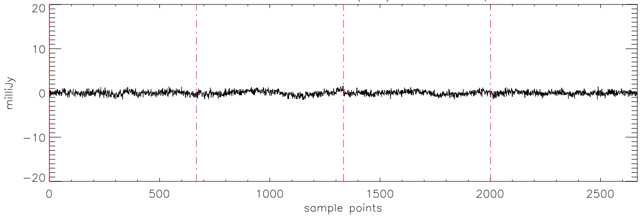
a2471 J07003664 09feb12 (AST) StokesV freq:4608.
