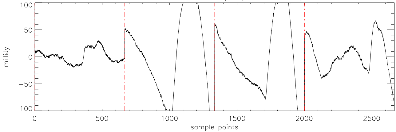
a2471 J07003664 09feb12 (AST) StokesI freq:5176.
