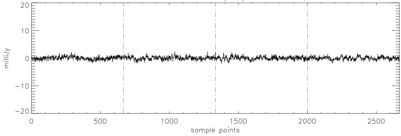
a2471 J07003664 09feb12 (AST) StokesV freq:5176.
