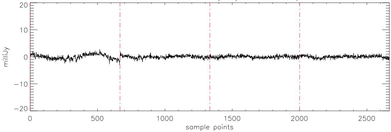
a2471 J07003664 09feb12 (AST) StokesU freq:4608.
