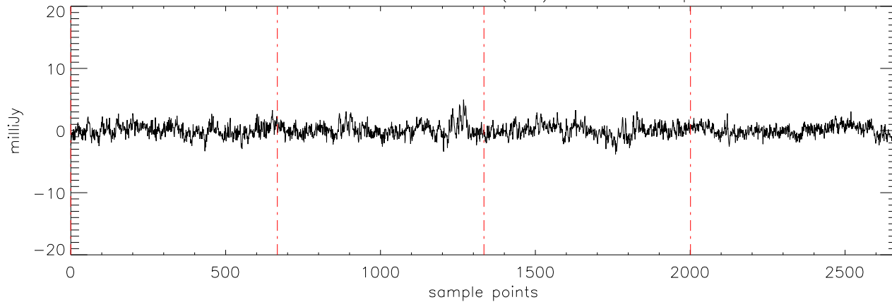
a2471 J07003664 09feb12 (AST) StokesU freq:5176.
