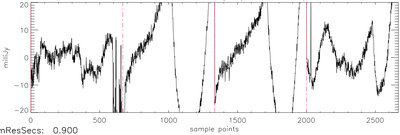
a2471 J07003664 09feb12 (AST) StokesQ freq:4466.
