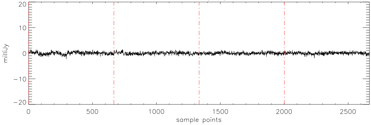
a2471 J07003664 09feb12 (AST) StokesV freq:4750.
