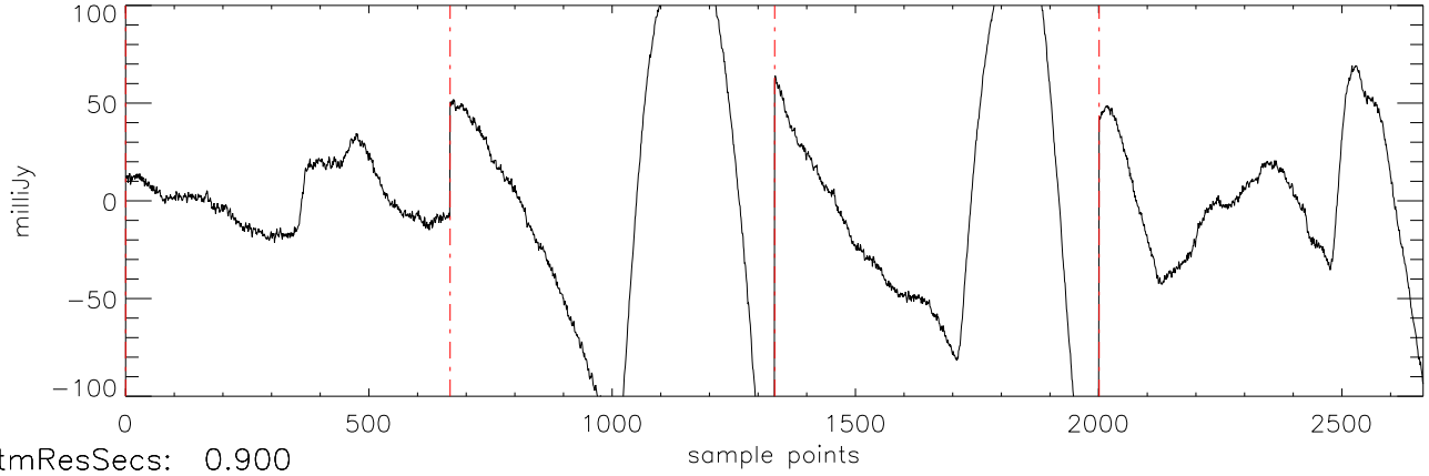
a2471 J07003664 09feb12 (AST) StokesI freq:5034.
