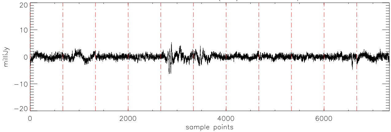
a2471 J07003664 19nov11 (AST) StokesU freq:4608.
