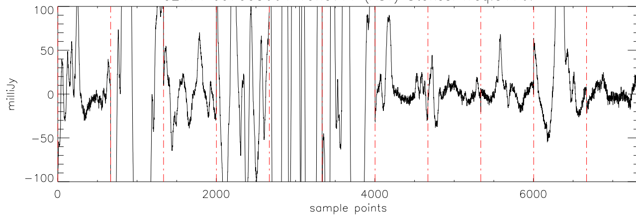
a2471 J07003664 19nov11 (AST) StokesI freq:5176.
