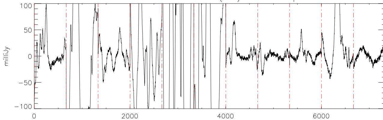
a2471 J07003664 19nov11 (AST) StokesI freq:4750.
