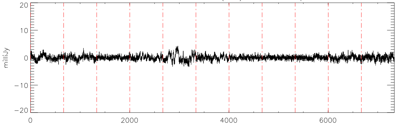
α2471 J07003664 19nov11 (AST) StokesV freq:5034.
