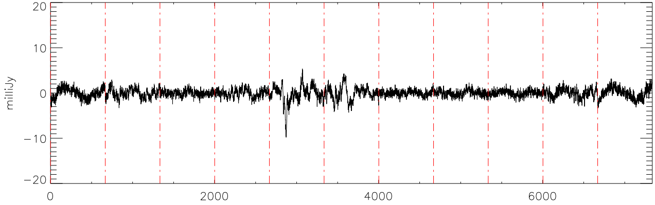
a2471 J07003664 19nov11 (AST) StokesU freq:4892.
