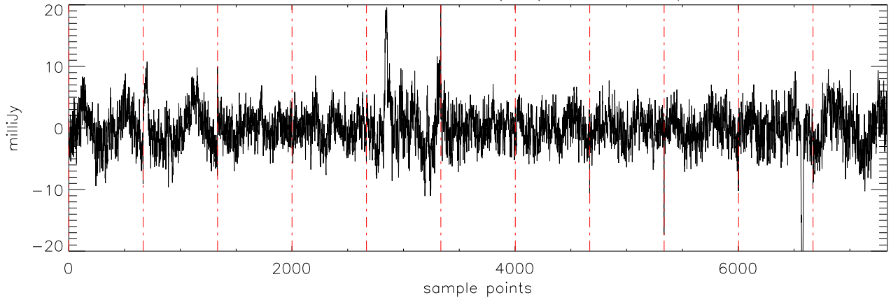
a2471 J07003664 19nov11 (AST) StokesQ freq:4750.
