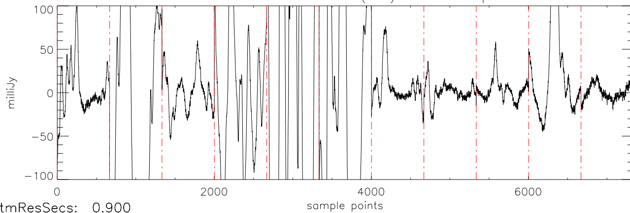
a2471 J07003664 19nov11 (AST) StokesI freq:5034.
