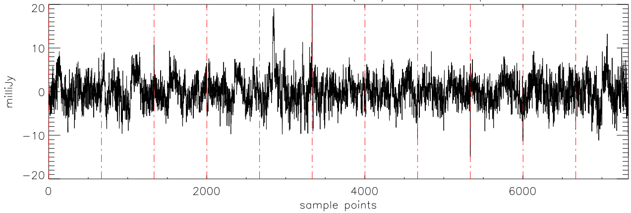
a2471 J07003664 19nov11 (AST) StokesQ freq:4608.
