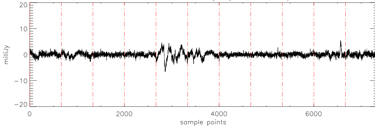
a2471 J07003664 19nov11 (AST) StokesV freq:4750.
