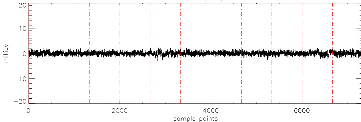
a2471 J07003664 19nov11 (AST) StokesV freq:4608.
