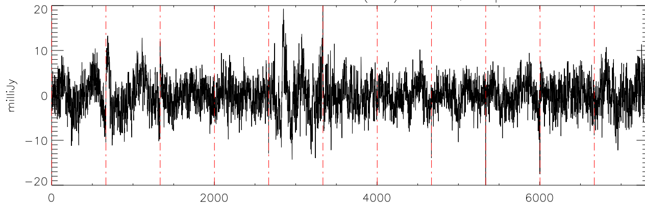
a2471 J07003664 19nov11 (AST) StokesQ freq:5176.
