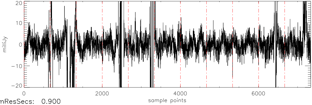
a2471 J07003664 19nov11 (AST) StokesQ freq:4466.
