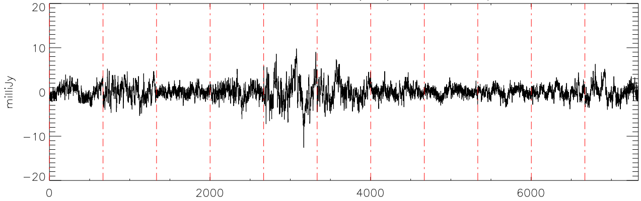
a2471 J07003664 19nov11 (AST) StokesU freq:5176.
