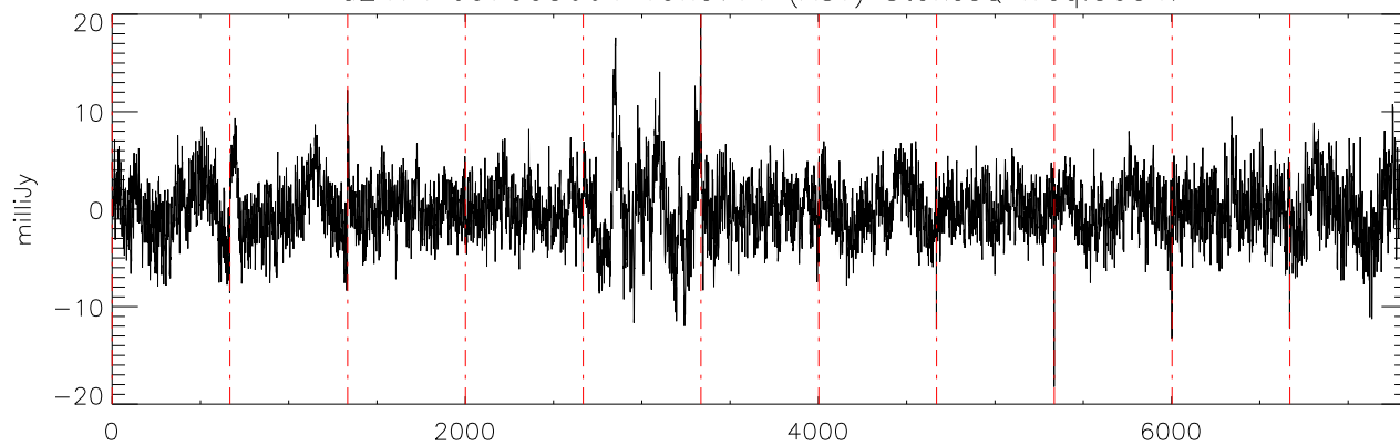
a2471 J07003664 19nov11 (AST) StokesQ freq:5034.
