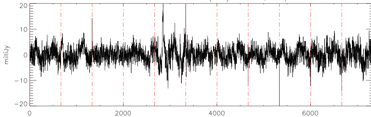
a2471 J07003664 19nov11 (AST) StokesQ freq:4892.
