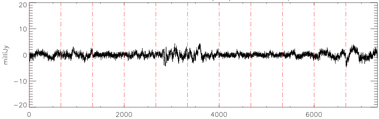
a2471 J07003664 19nov11 (AST) StokesU freq:5034.
