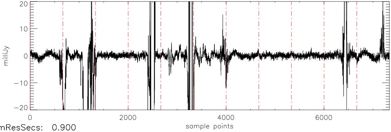
a2471 J07003664 19nov11 (AST) StokesU freq:4466.
