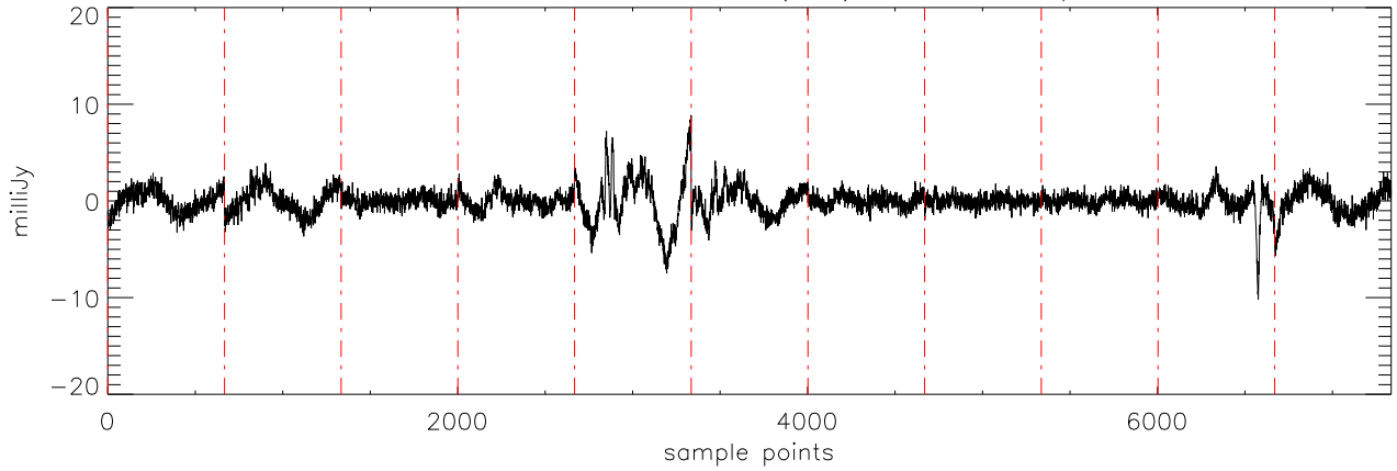
a2471 J07003664 19nov11 (AST) StokesU freq:4750.
