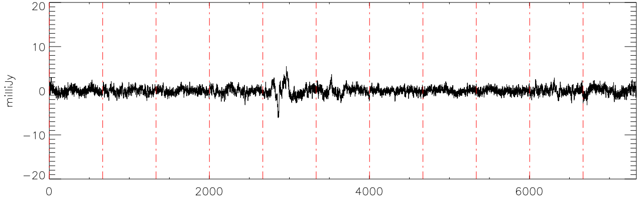
α2471 J07003664 19nov11 (AST) StokesV freq:4892.
