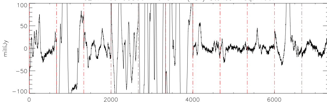
a2471 J07003664 19nov11 (AST) StokesI freq:4466.
