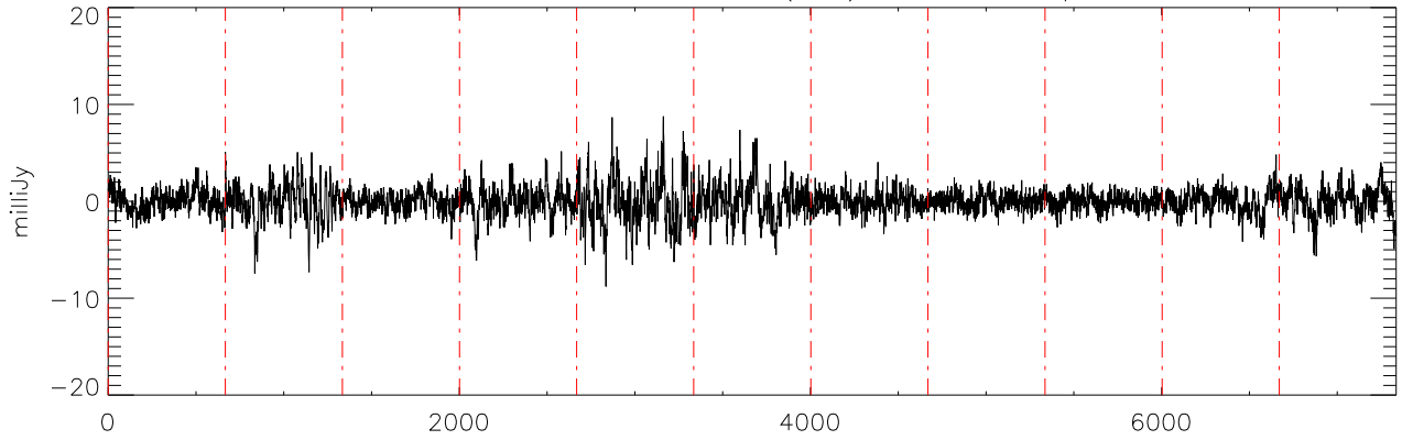
α2471 J07003664 19nov11 (AST) StokesV freq:5176.
