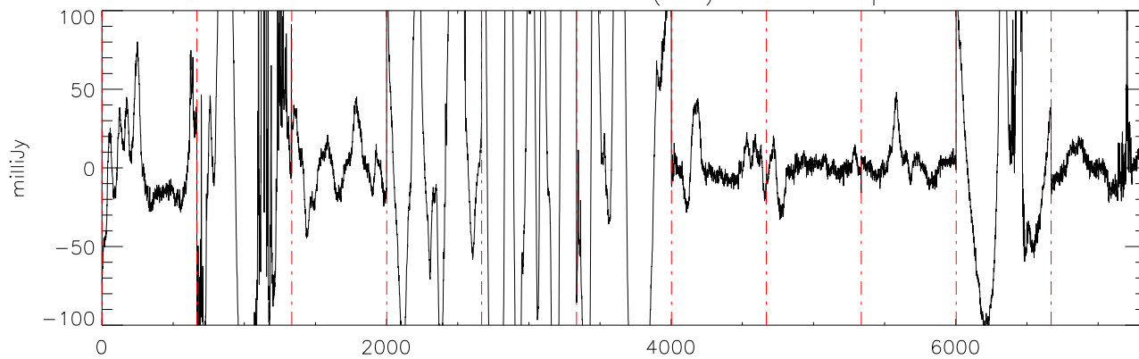
a2471 J07003664 19nov11 (AST) StokesI freq:4325.
