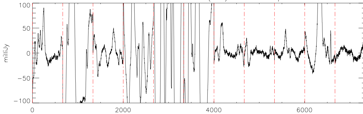
a2471 J07003664 19nov11 (AST) StokesI freq:4608.
