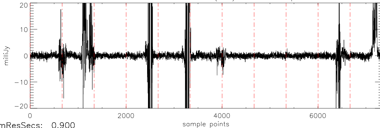
a2471 J07003664 19nov11 (AST) StokesV freq:4466.
