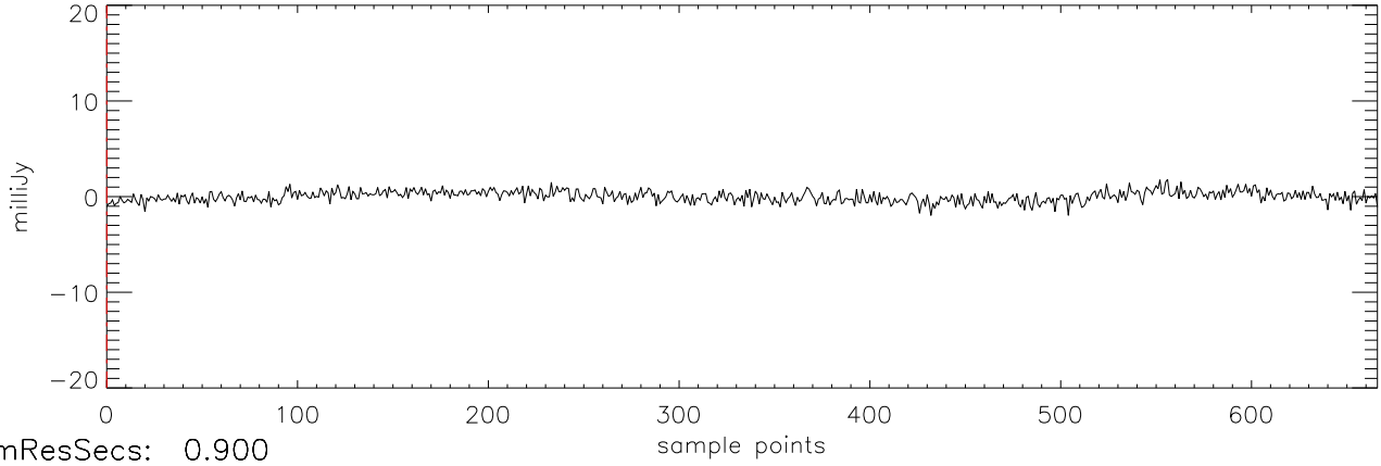
a2471 J03454316 21oct11 (AST) StokesV freq:4466.
