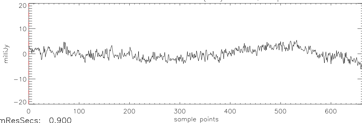
a2471 J03454316 21oct11 (AST) StokesQ freq:5034.
