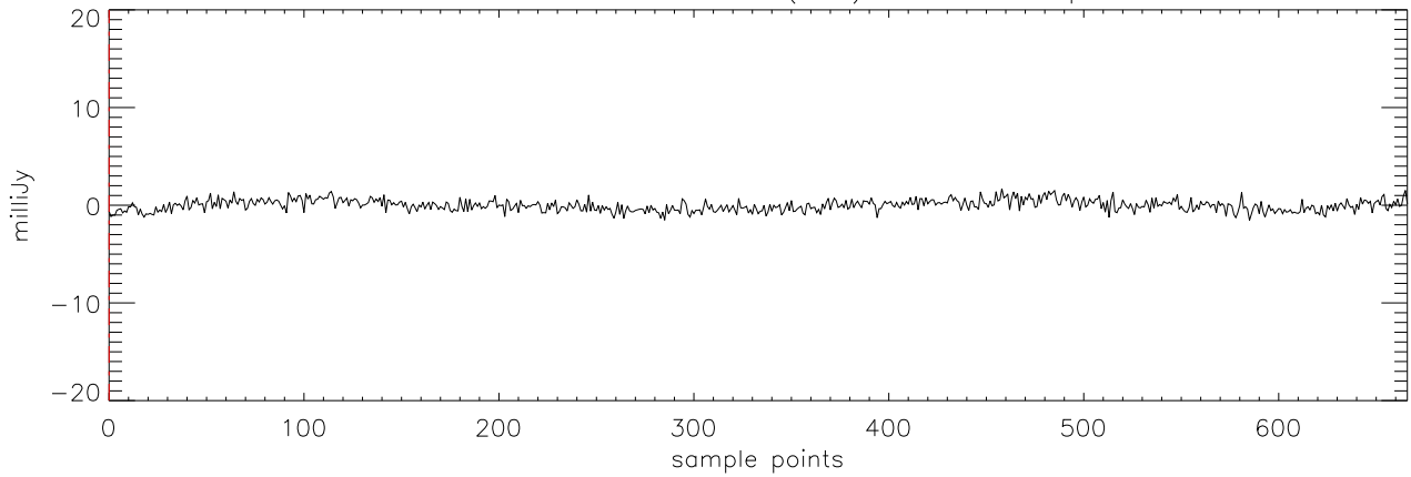
a2471 J03454316 21oct11 (AST) StokesV freq:4750.
