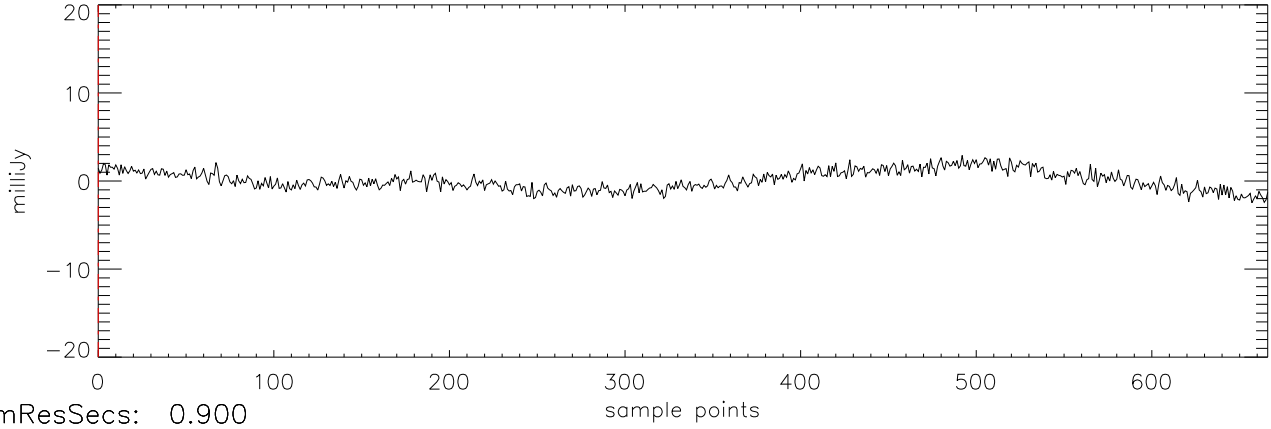
a2471 J03454316 21oct11 (AST) StokesU freq:5034.
