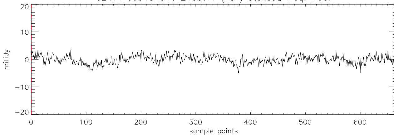
a2471 J03454316 21oct11 (AST) StokesQ freq:4750.
