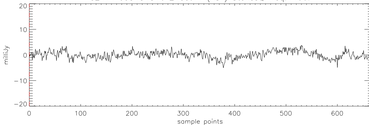
a2471 J03454316 21oct11 (AST) StokesQ freq:4608.
