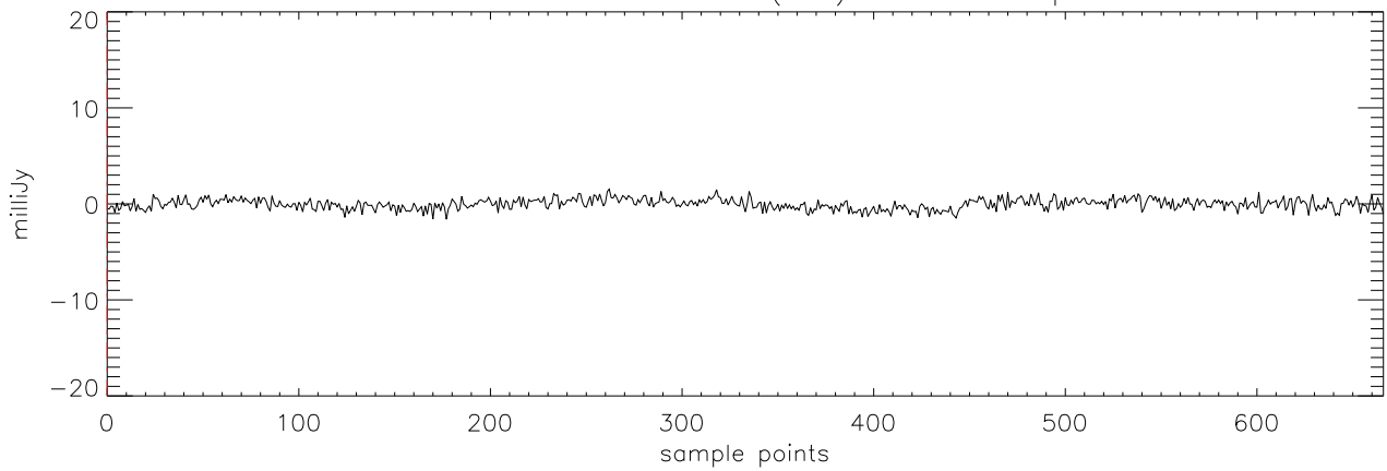
a2471 J03454316 21oct11 (AST) StokesU freq:4608.
