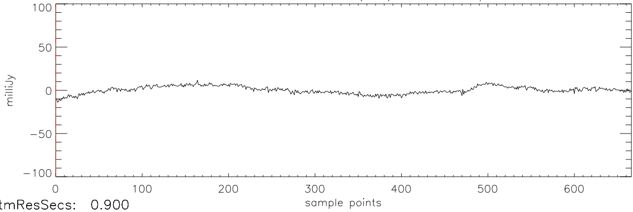
a2471 J03454316 21oct11 (AST) StokesI freq:4466.
