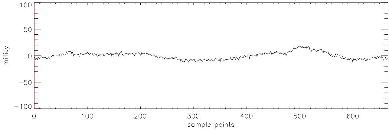
a2471 J03454316 21oct11 (AST) StokesI freq:5176.
