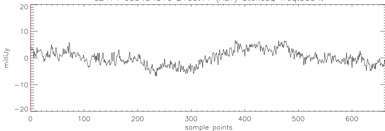
a2471 J03454316 21oct11 (AST) StokesQ freq:5176.
