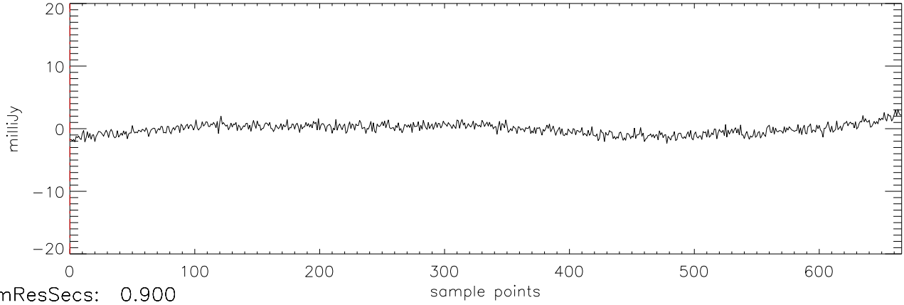
a2471 J03454316 21oct11 (AST) StokesU freq:4466.
