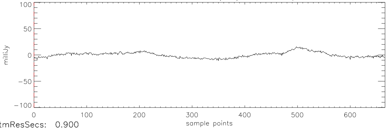
a2471 J03454316 21oct11 (AST) StokesI freq:5034.
