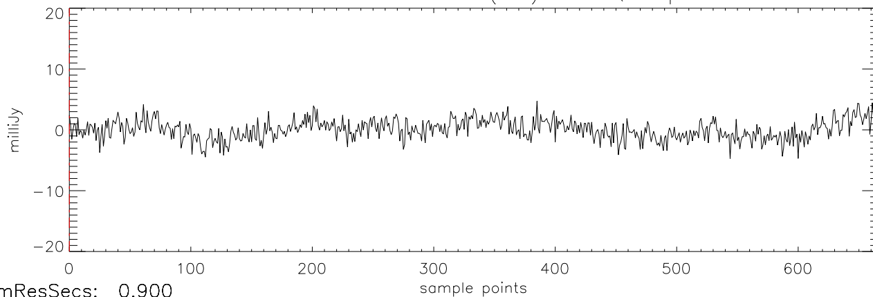
a2471 J03454316 21oct11 (AST) StokesQ freq:4466.
