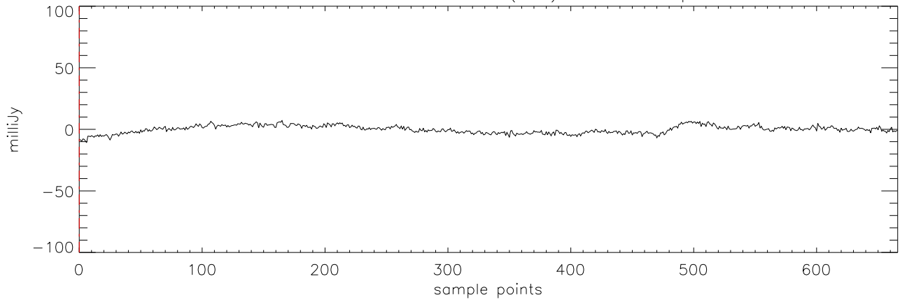
a2471 J03454316 21oct11 (AST) StokesI freq:4750.
