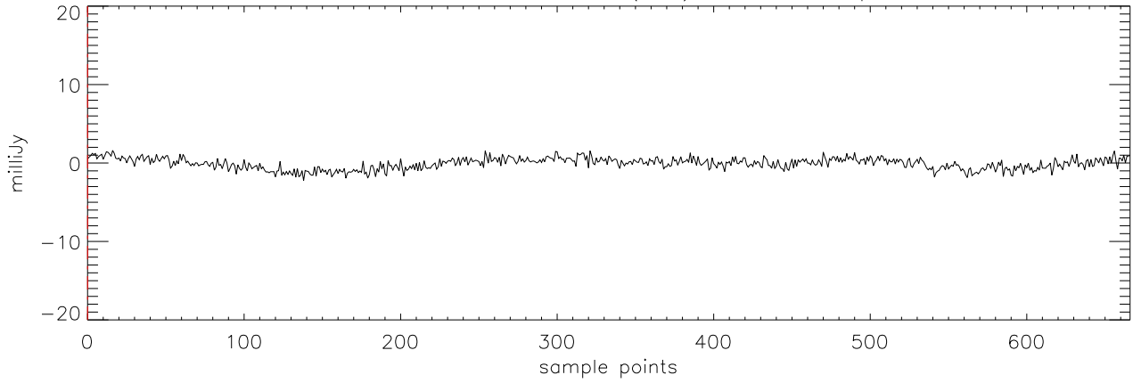
a2471 J03454316 21oct11 (AST) StokesU freq:4750.
