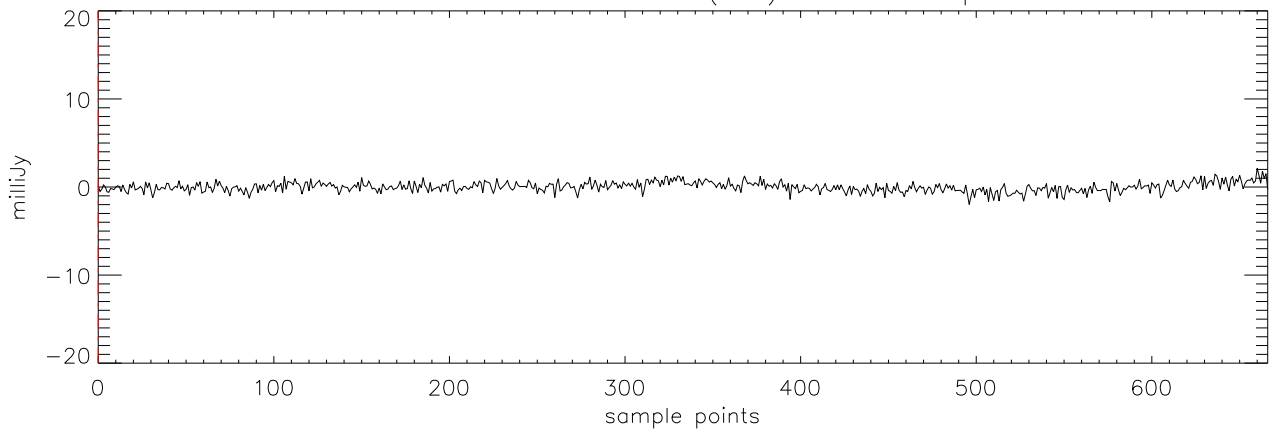
a2471 J03454316 21oct11 (AST) StokesV freq:4608.
