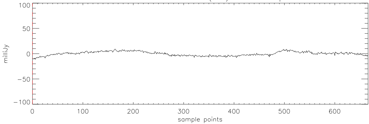
a2471 J03454316 21oct11 (AST) StokesI freq:4608.
