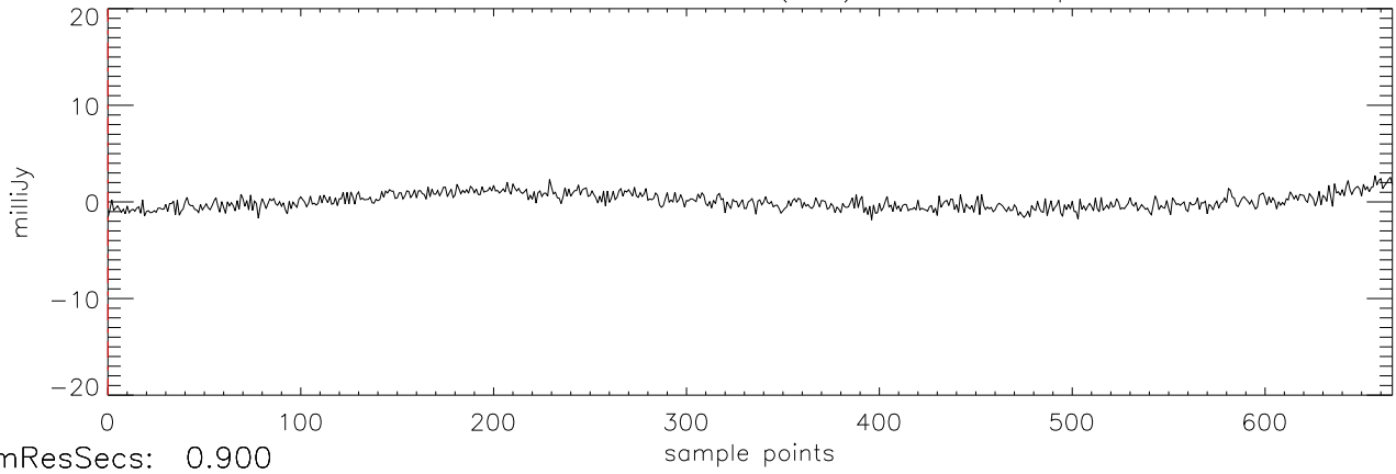
a2471 J03454316 21oct11 (AST) StokesV freq:5034.
