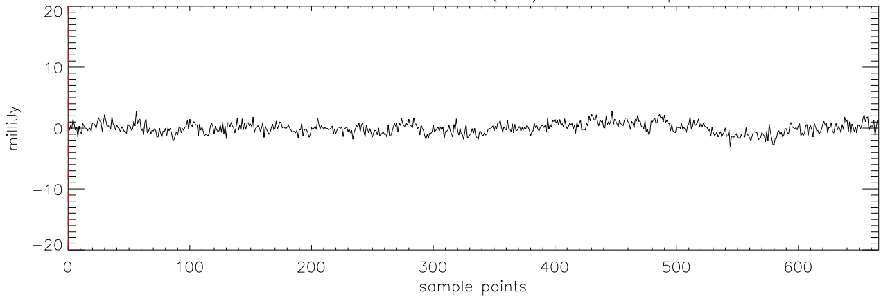
a2471 J03454316 21oct11 (AST) StokesV freq:5176.
