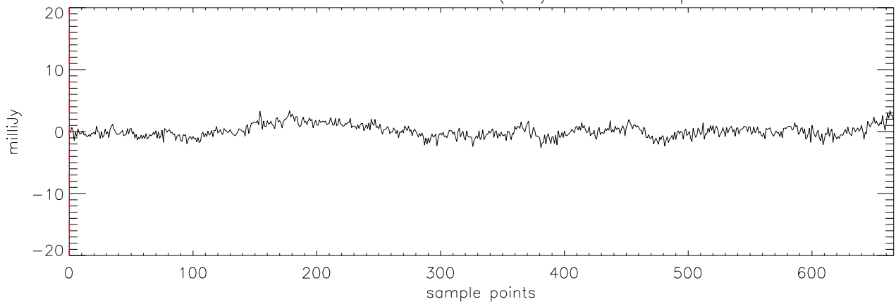
a2471 J03454316 21oct11 (AST) StokesU freq:5176.
