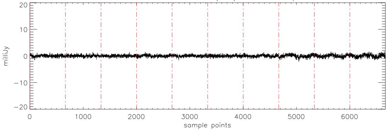
a2471 J03454316 10oct11 (AST) StokesV freq:4608.
