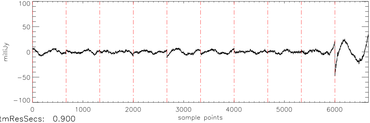
\alpha 2471 J03454316 10oct11 (AST) StokesI freq:5034.
