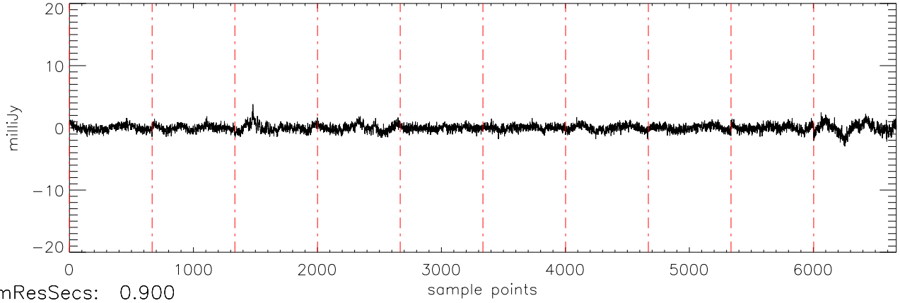
α2471 J03454316 10oct11 (AST) StokesU freq:5034.
