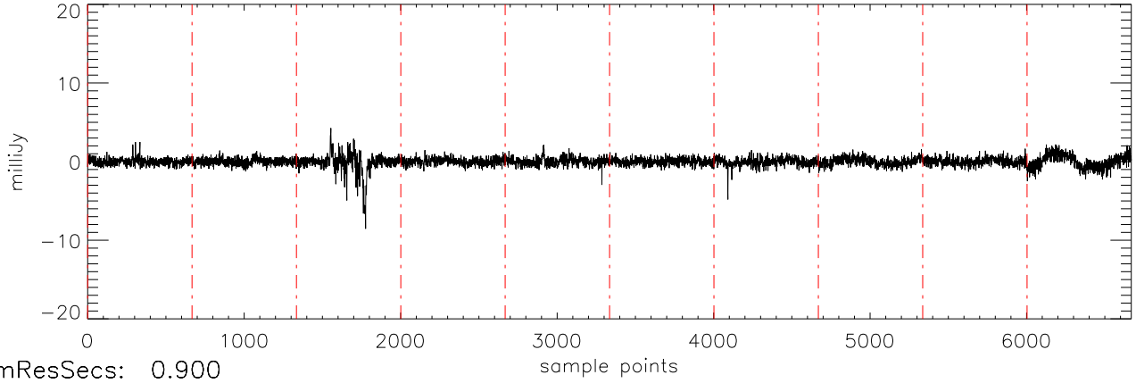
a2471 J03454316 10oct11 (AST) StokesV freq:4466.
