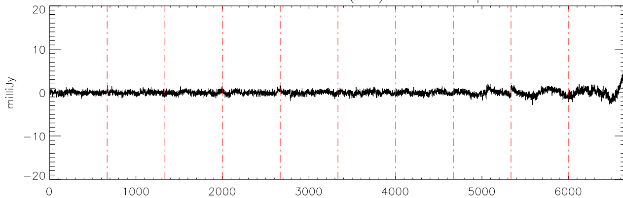
a2471 J03454316 10oct11 (AST) StokesU freq:4750.
