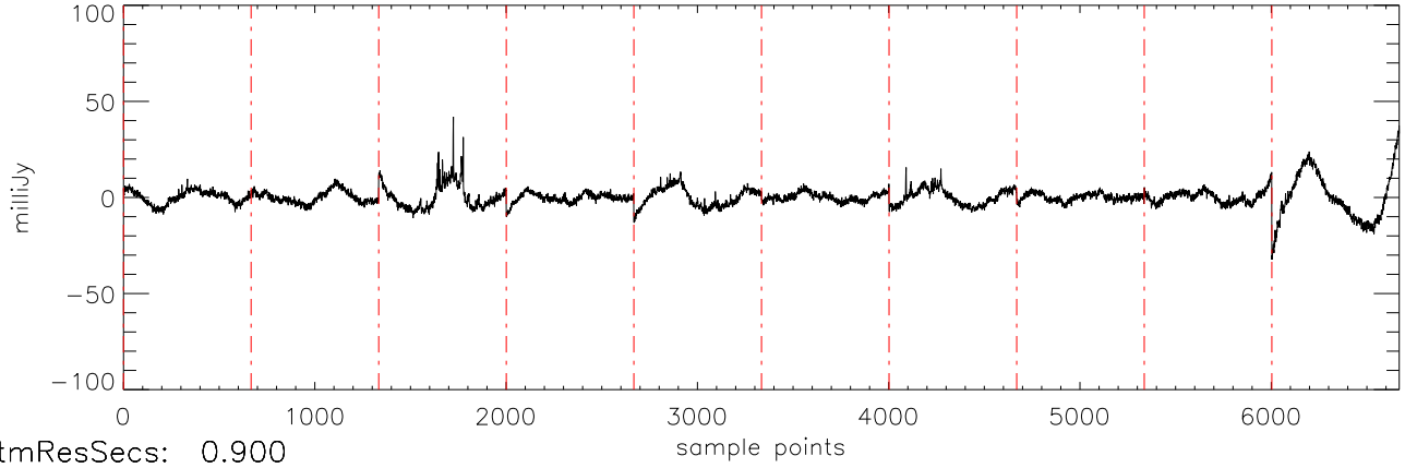
\alpha 2471 J03454316 10oct11 (AST) StokesI freq:4466.
