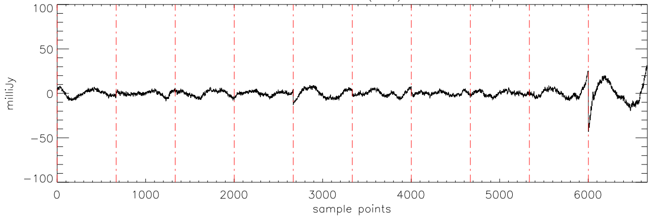
\alpha 2471 J03454316 10oct11 (AST) StokesI freq:5176.
