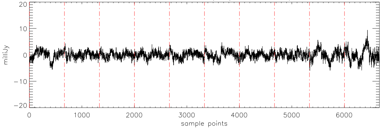
α2471 J03454316 10oct11 (AST) StokesQ freq:4750.
