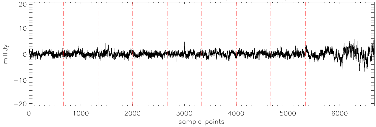
α2471 J03454316 10oct11 (AST) StokesU freq:5176.
