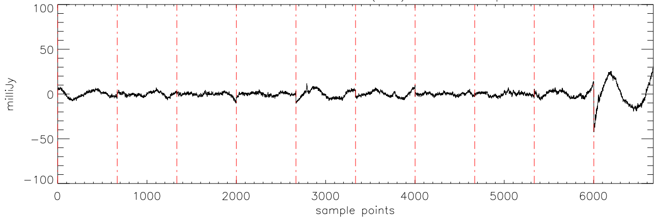
\alpha 2471 J03454316 10oct11 (AST) StokesI freq:4750.
