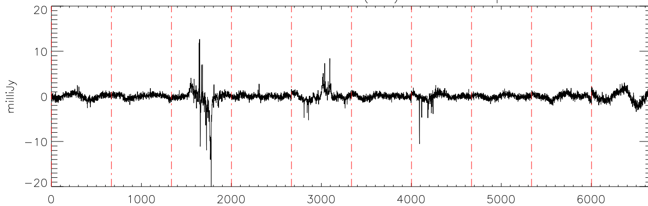
a2471 J03454316 10oct11 (AST) StokesU freq:4325.
