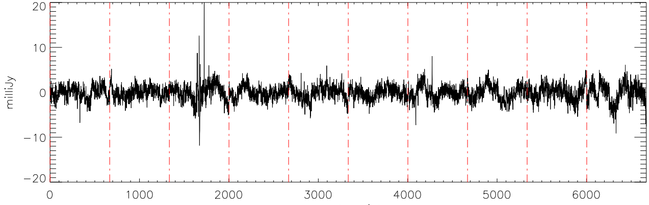
α2471 J03454316 10oct11 (AST) StokesQ freq:4325.
