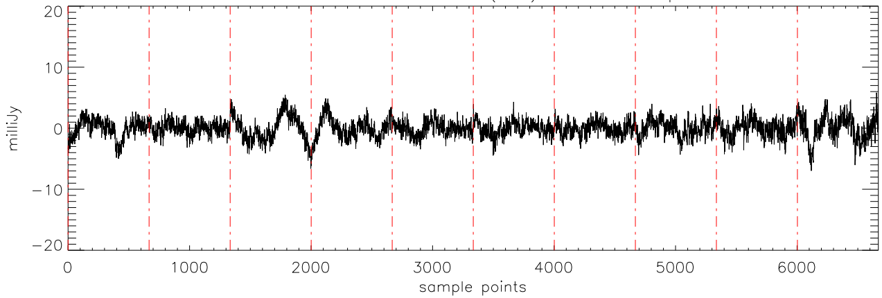
α2471 J03454316 10oct11 (AST) StokesQ freq:4608.
