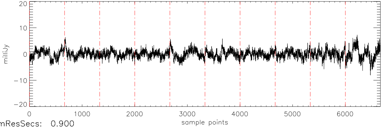
α2471 J03454316 10oct11 (AST) StokesQ freq:5034.
