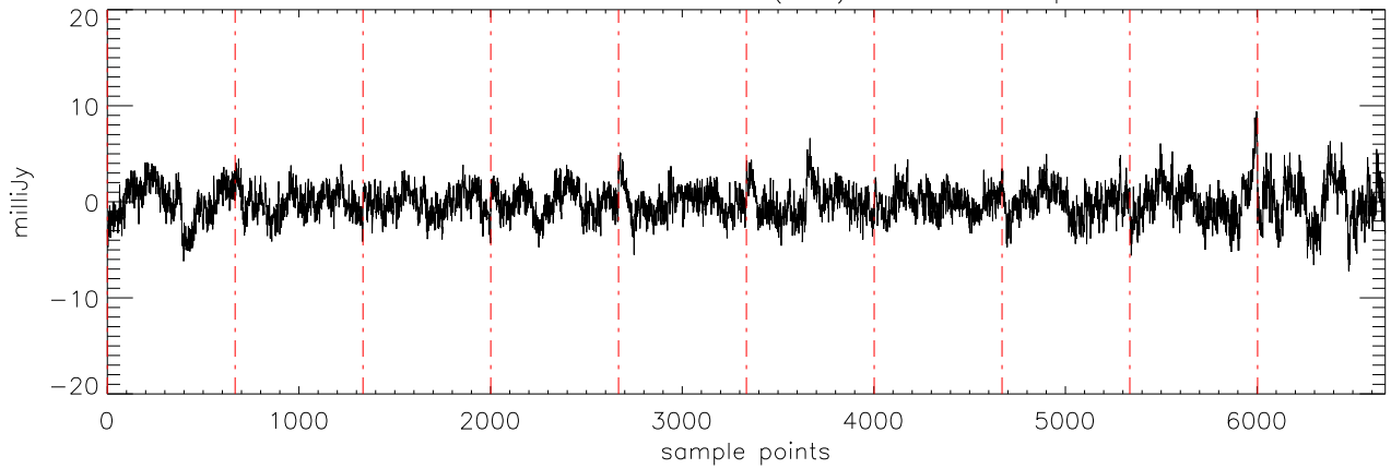
α2471 J03454316 10oct11 (AST) StokesQ freq:5176.
