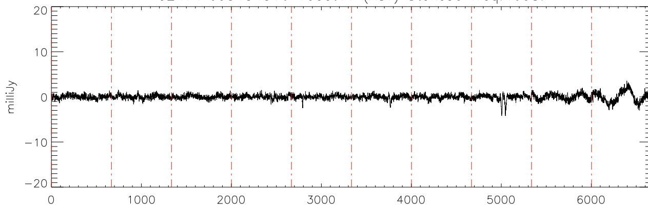
a2471 J03454316 10oct11 (AST) StokesU freq:4608.
