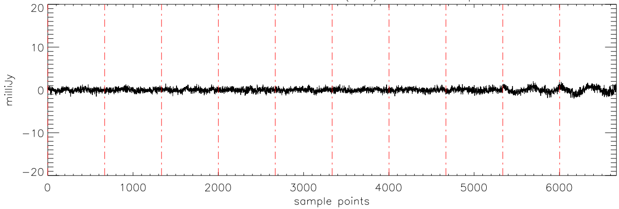
a2471 J03454316 10oct11 (AST) StokesV freq:4750.
