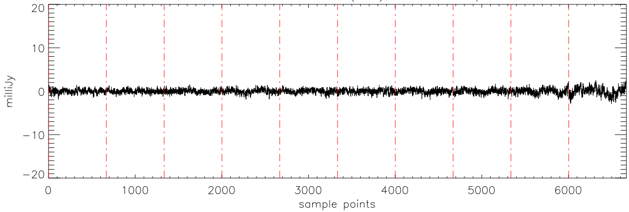
a2471 J03454316 10oct11 (AST) StokesV freq:5176.
