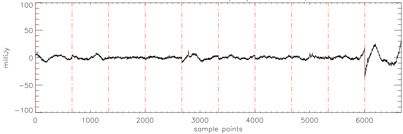
\alpha 2471 J03454316 10oct11 (AST) StokesI freq:4608.
