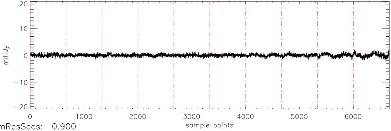
a2471 J03454316 10oct11 (AST) StokesV freq:5034.
