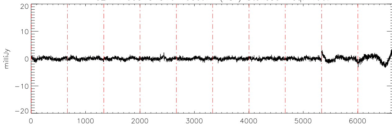
a2471 J03454316 10oct11 (AST) StokesU freq:4466.
