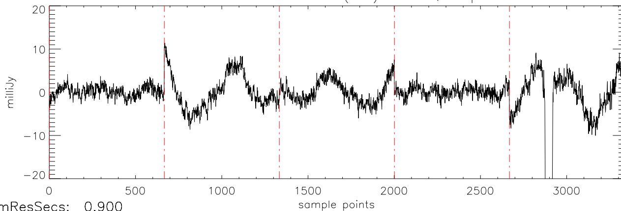
a2471 J0326137 20oct11 (AST) StokesQ freq:5034.
