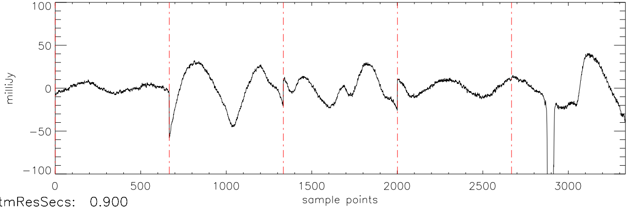
a2471 J0326137 20oct11 (AST) StokesI freq:5034.
