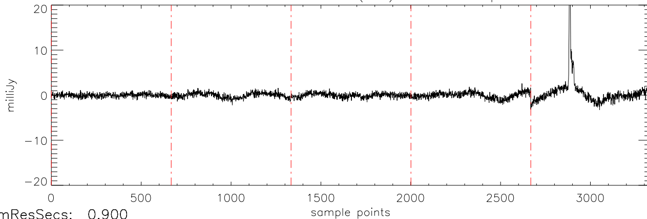
a2471 J0326137 20oct11 (AST) StokesU freq:5034.
