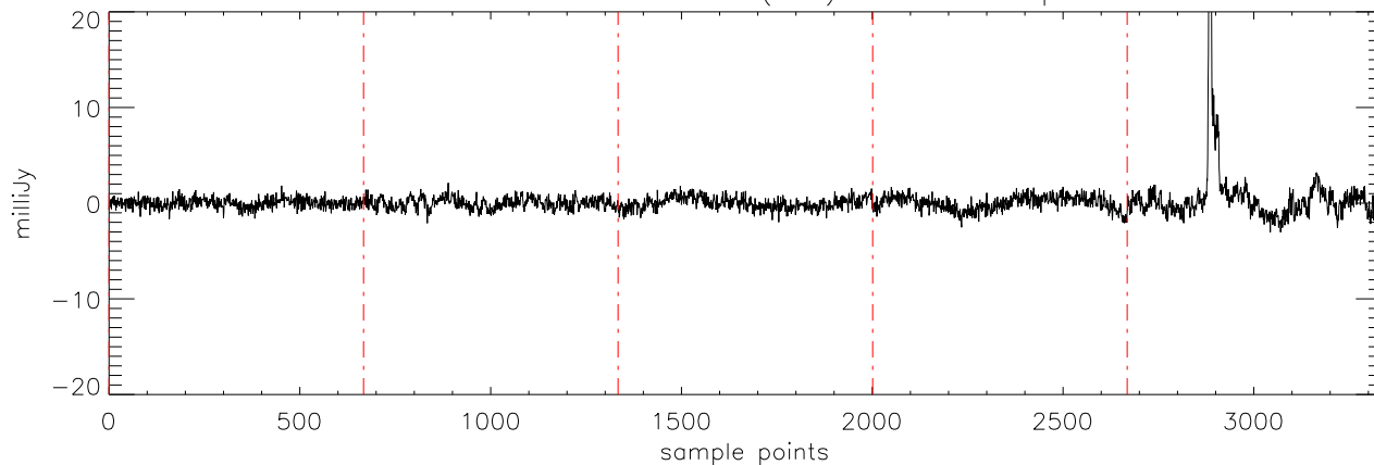
a2471 J0326137 20oct11 (AST) StokesU freq:5176.
