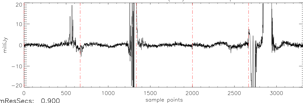
a2471 J0326137 20oct11 (AST) StokesU freq:4466.
