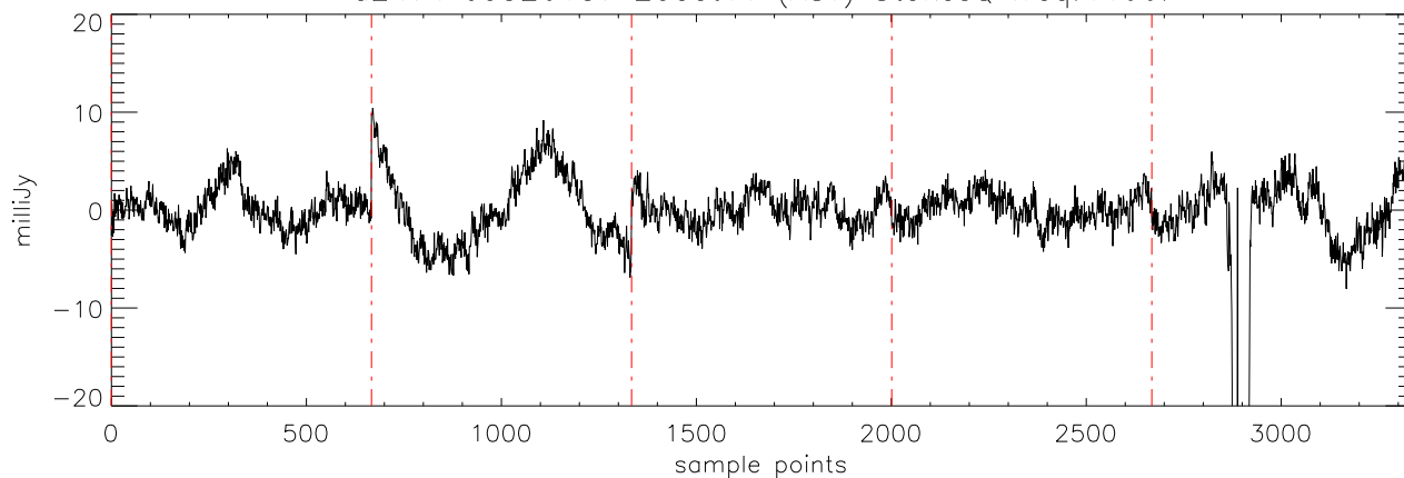
a2471 J0326137 20oct11 (AST) StokesQ freq:4608.
