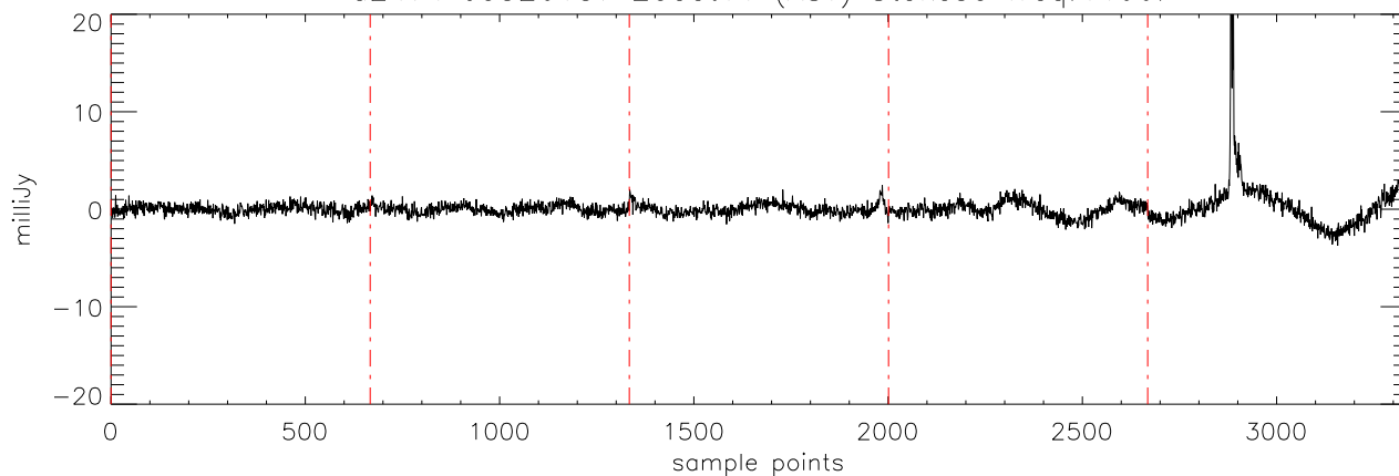
a2471 J0326137 20oct11 (AST) StokesU freq:4608.
