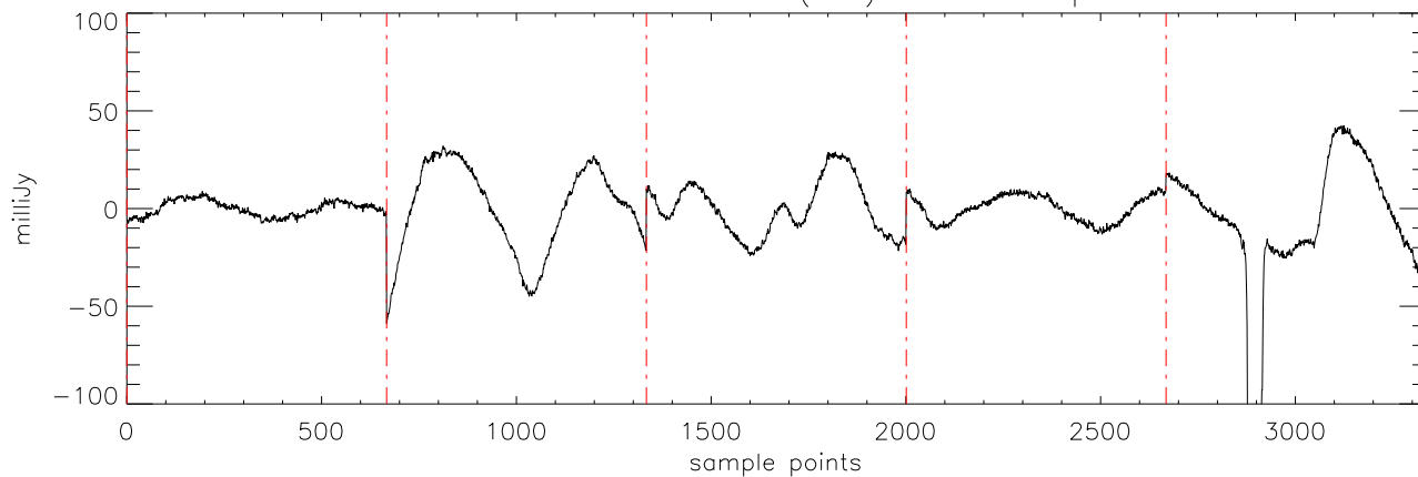
a2471 J0326137 20oct11 (AST) StokesI freq:4750.
