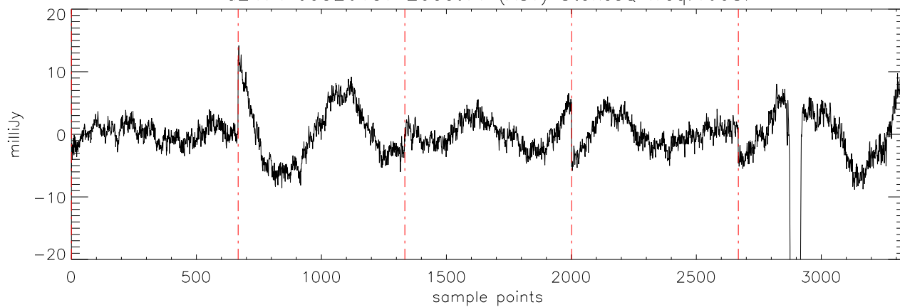
a2471 J0326137 20oct11 (AST) StokesQ freq:4750.
