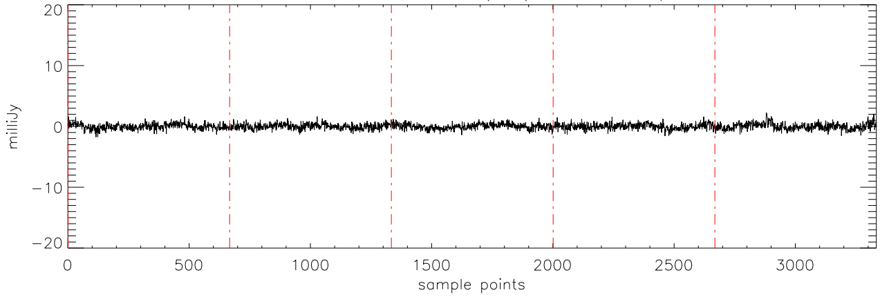
a2471 J0326137 20oct11 (AST) StokesV freq:4750.
