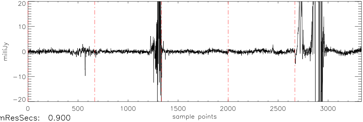
a2471 J0326137 20oct11 (AST) StokesV freq:4466.
