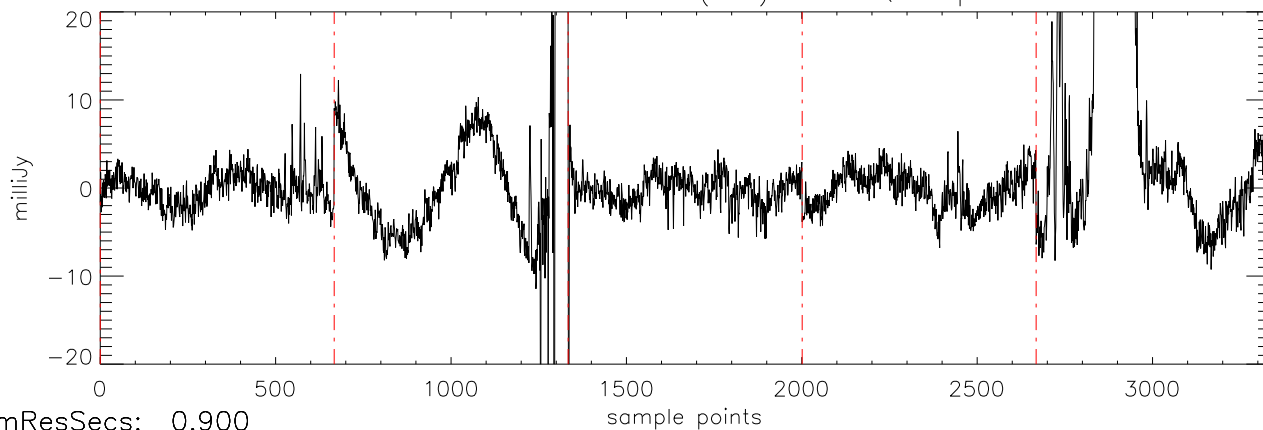
a2471 J0326137 20oct11 (AST) StokesQ freq:4466.
