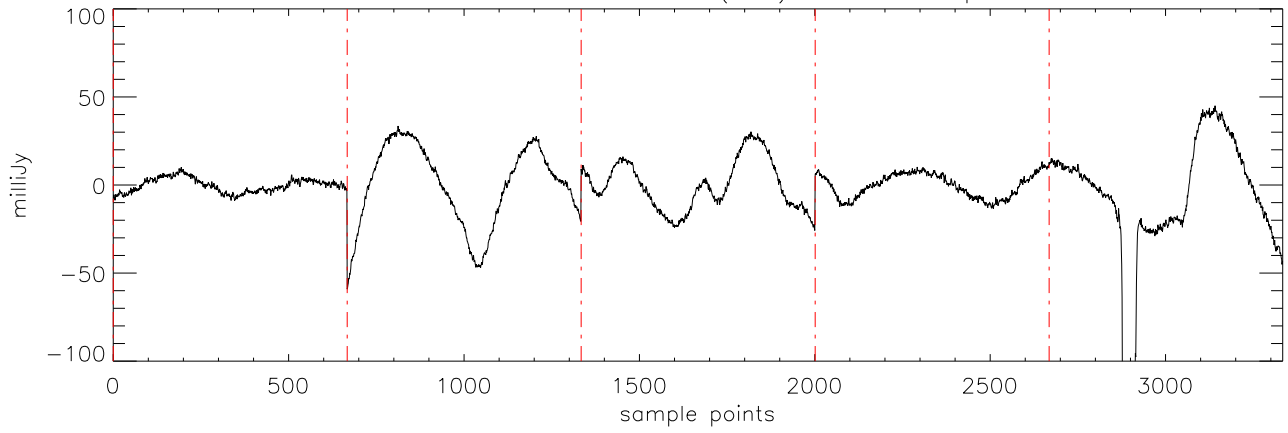
a2471 J0326137 20oct11 (AST) StokesI freq:5176.
