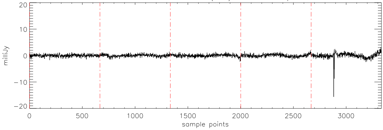
a2471 J0326137 20oct11 (AST) StokesV freq:4608.
