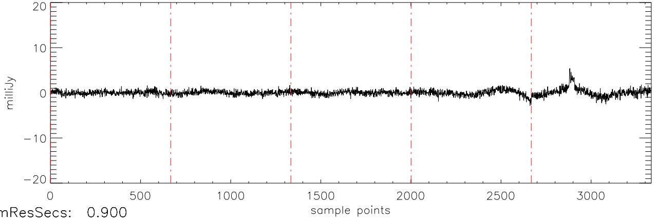
a2471 J0326137 20oct11 (AST) StokesV freq:5034.
