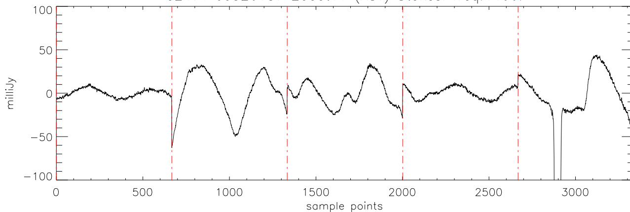
a2471 J0326137 20oct11 (AST) StokesI freq:4608.
