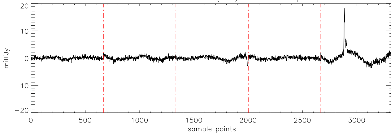
a2471 J0326137 20oct11 (AST) StokesU freq:4750.
