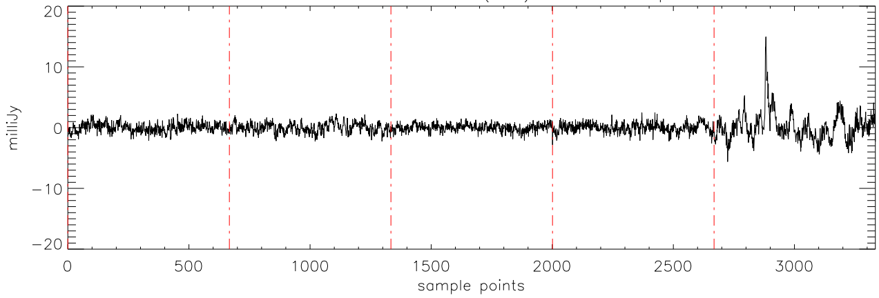
a2471 J0326137 20oct11 (AST) StokesV freq:5176.
