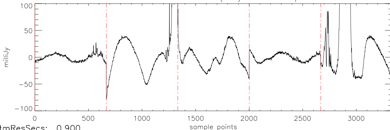
a2471 J0326137 20oct11 (AST) StokesI freq:4466.
