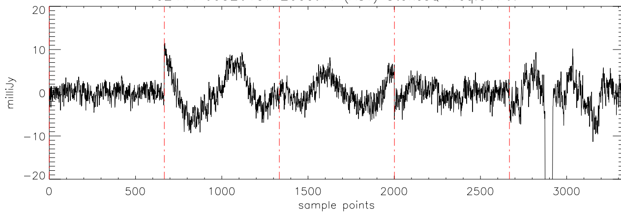
a2471 J0326137 20oct11 (AST) StokesQ freq:5176.
