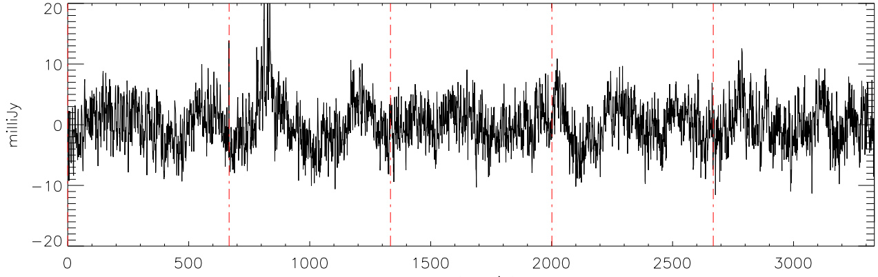
a2471 J02074284 19nov11 (AST) StokesQ freq:4325.
