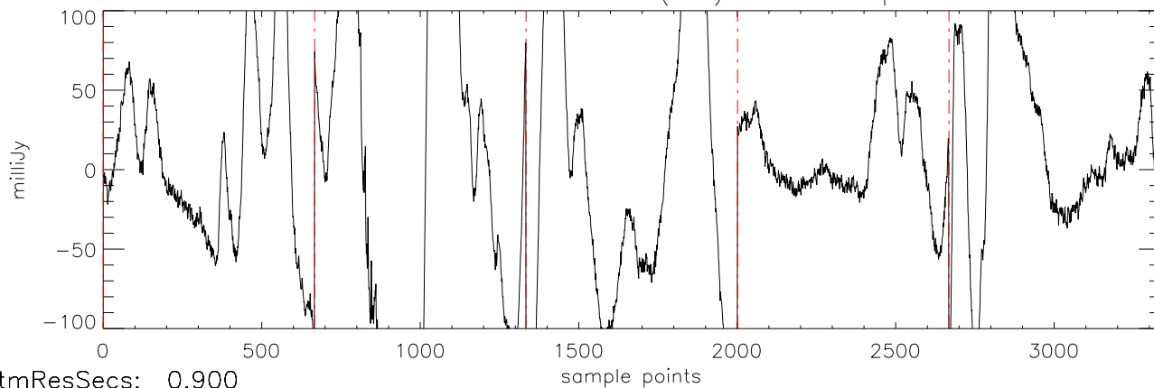
a2471 J02074284 19nov11 (AST) StokesI freq:4466.
