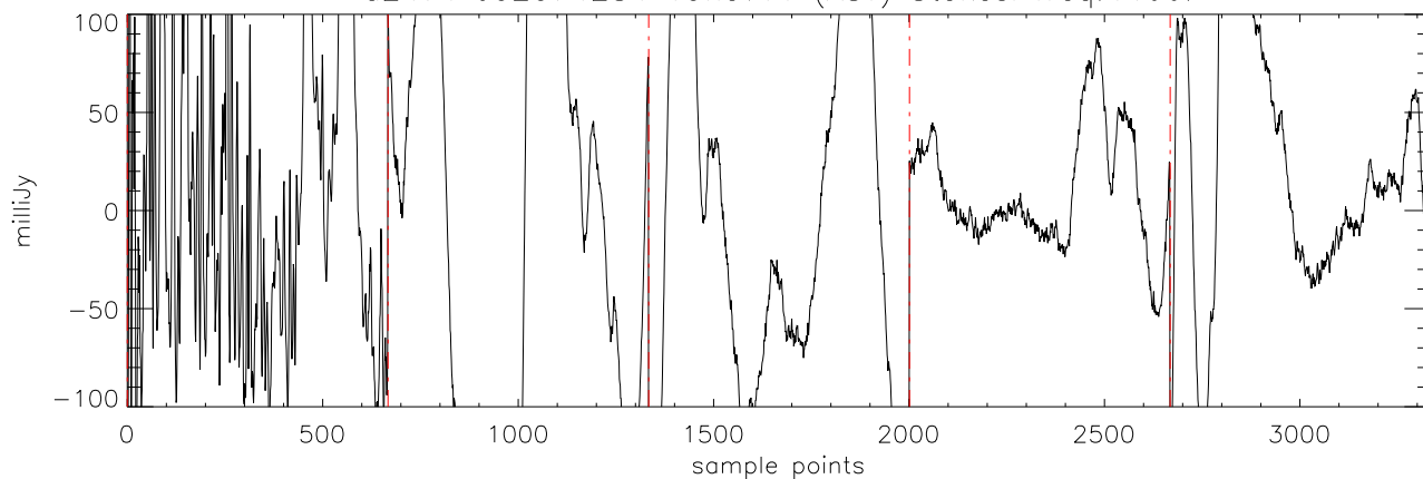
a2471 J02074284 19nov11 (AST) StokesI freq:4608.
