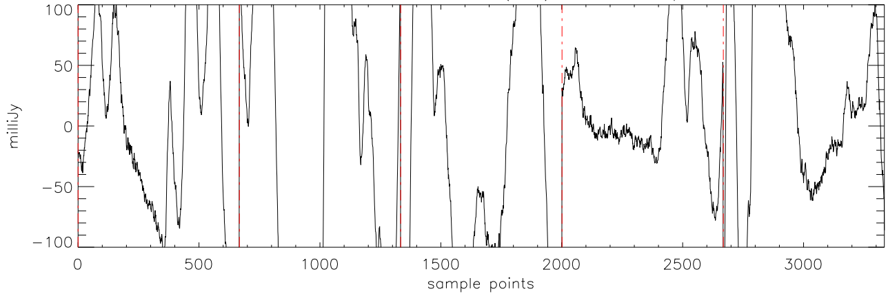
a2471 J02074284 19nov11 (AST) StokesI freq:5176.
