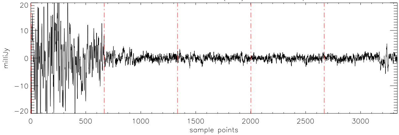
a2471 J02074284 19nov11 (AST) StokesV freq:4608.
