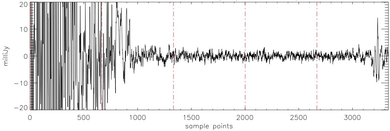
a2471 J02074284 19nov11 (AST) StokesV freq:4750.
