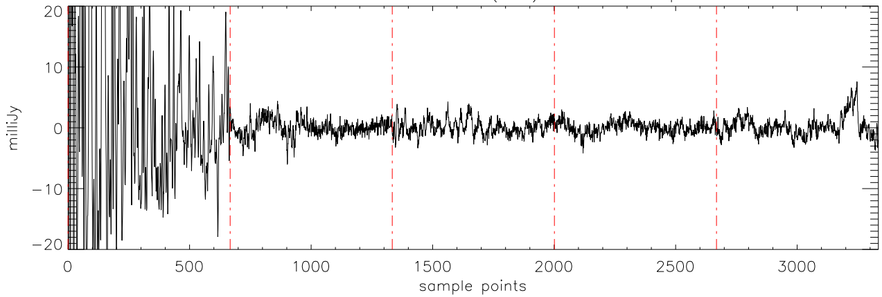
a2471 J02074284 19nov11 (AST) StokesU freq:4608.
