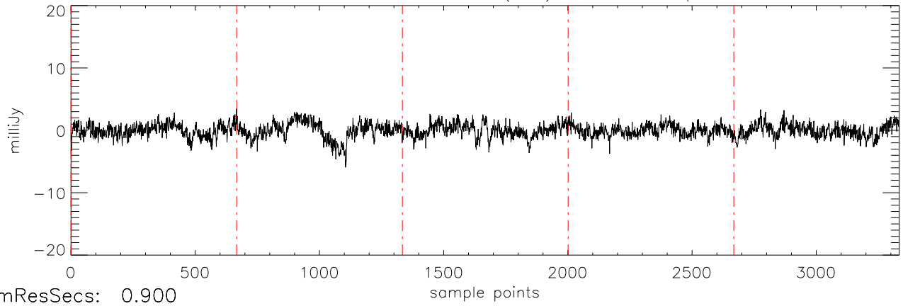
a2471 J02074284 19nov11 (AST) StokesU freq:5034.
