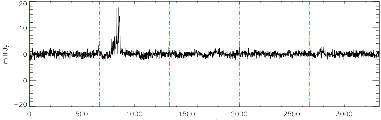
a2471 J02074284 19nov11 (AST) StokesV freq:4325.
