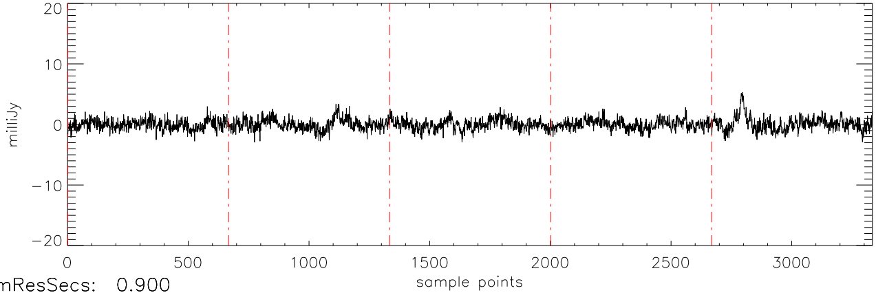
α2471 J02074284 19nov11 (AST) StokesV freq:5034.
