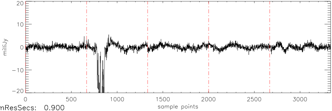
a2471 J02074284 19nov11 (AST) StokesU freq:4466.
