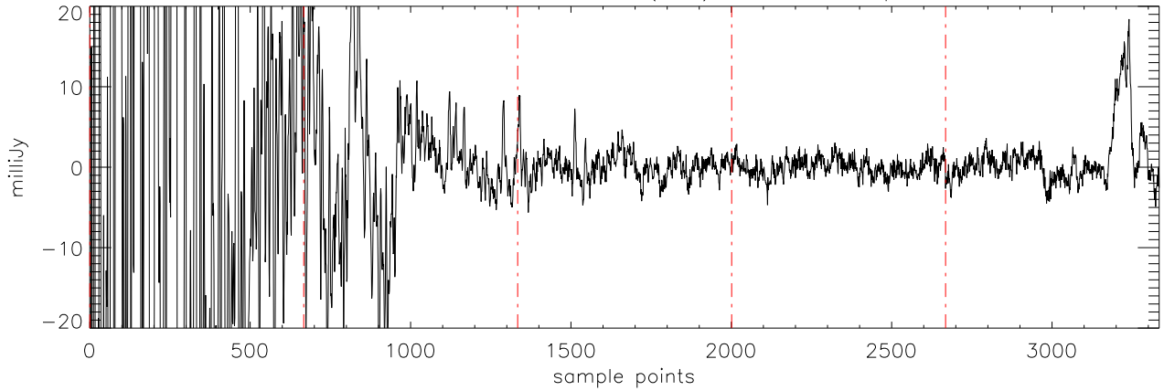
a2471 J02074284 19nov11 (AST) StokesU freq:4750.
