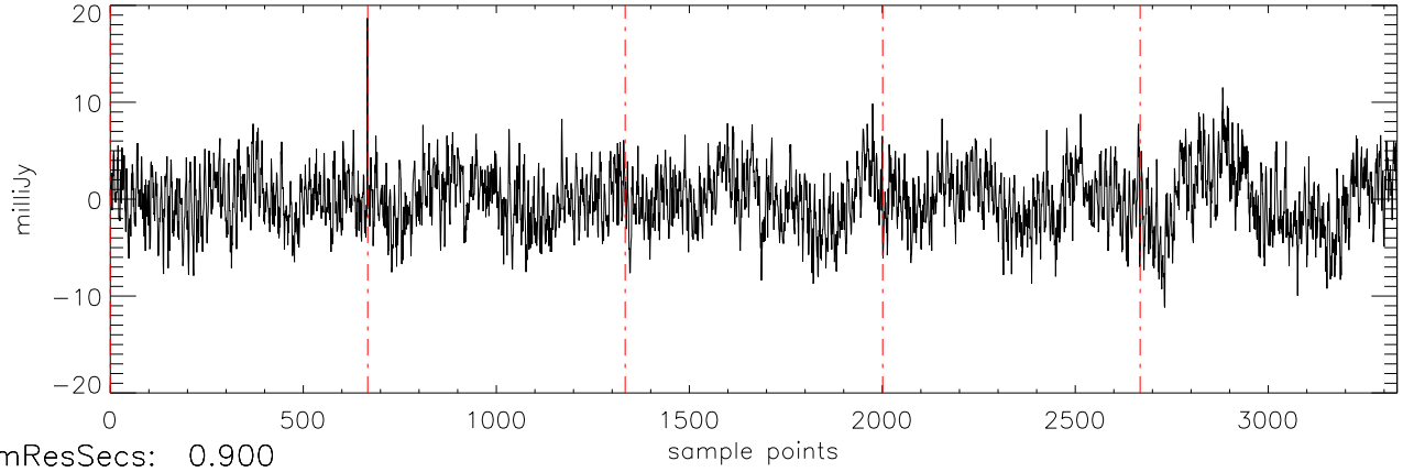
a2471 J02074284 19nov11 (AST) StokesQ freq:5034.
