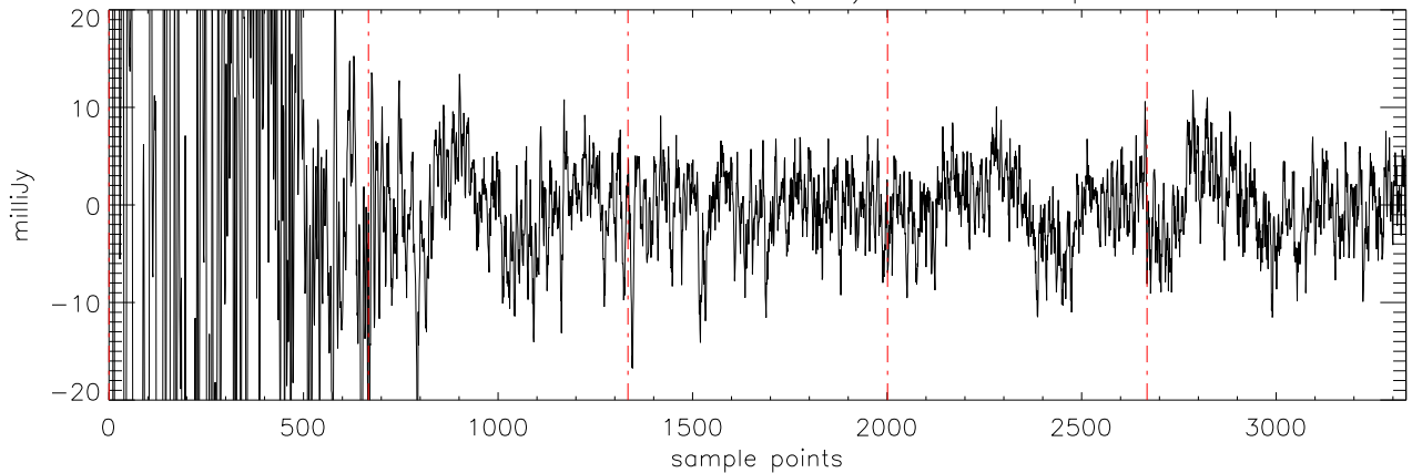
a2471 J02074284 19nov11 (AST) StokesQ freq:4750.
