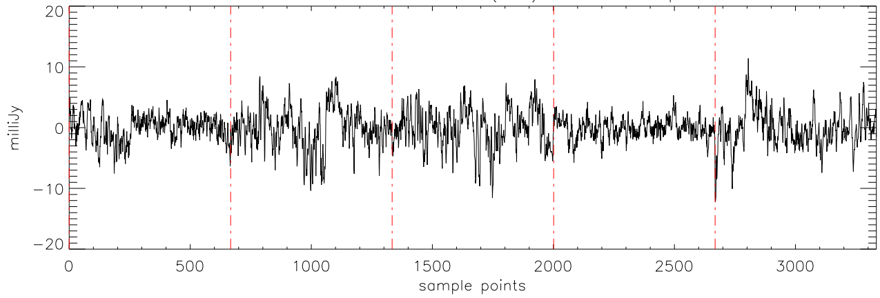
a2471 J02074284 19nov11 (AST) StokesU freq:5176.
