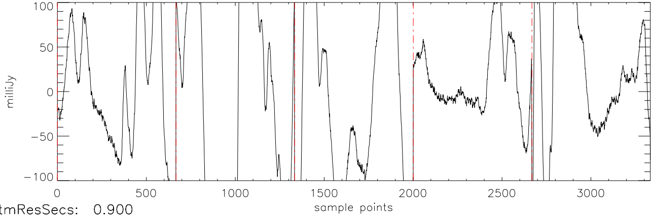
a2471 J02074284 19nov11 (AST) StokesI freq:5034.
