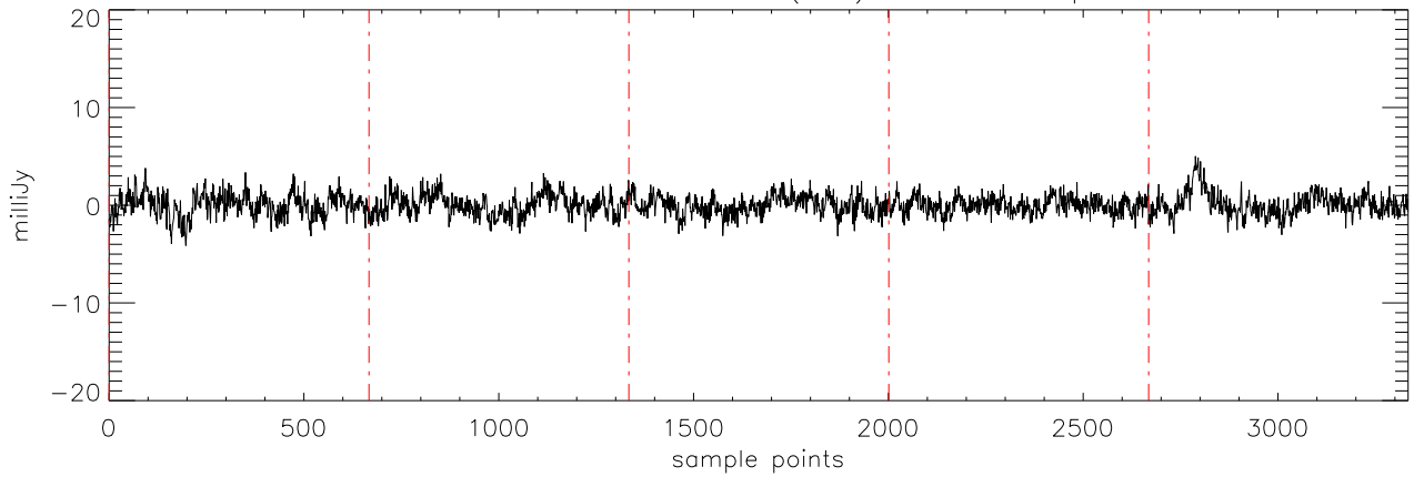
α2471 J02074284 19nov11 (AST) StokesV freq:5176.
