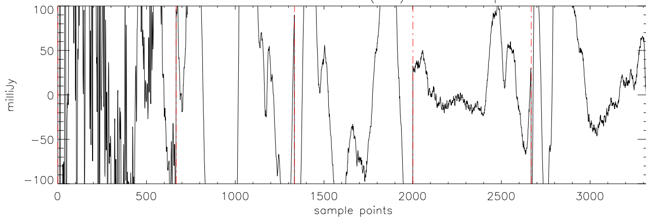
a2471 J02074284 19nov11 (AST) StokesI freq:4750.
