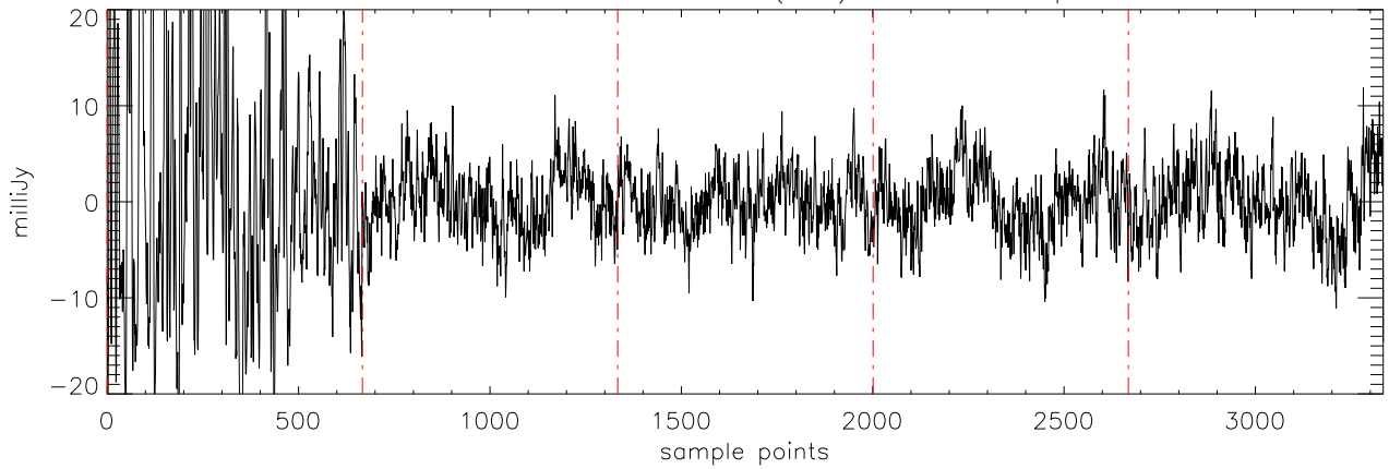
a2471 J02074284 19nov11 (AST) StokesQ freq:4608.
