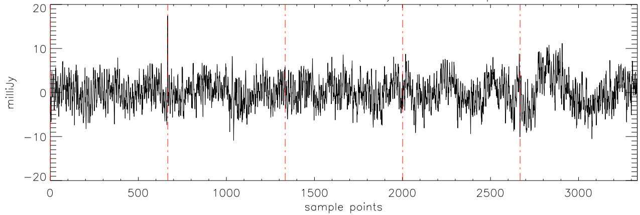
a2471 J02074284 19nov11 (AST) StokesQ freq:5176.
