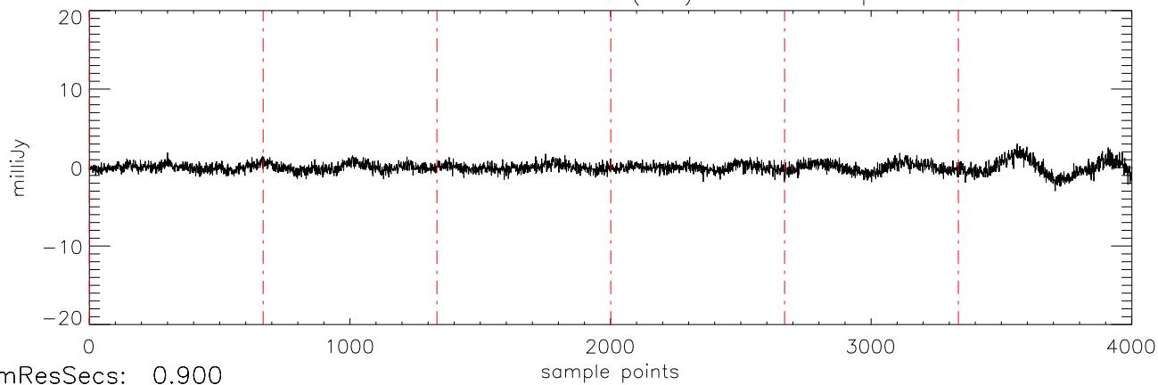
a2471 J01514155 27oct11 (AST) StokesU freq:5034.
