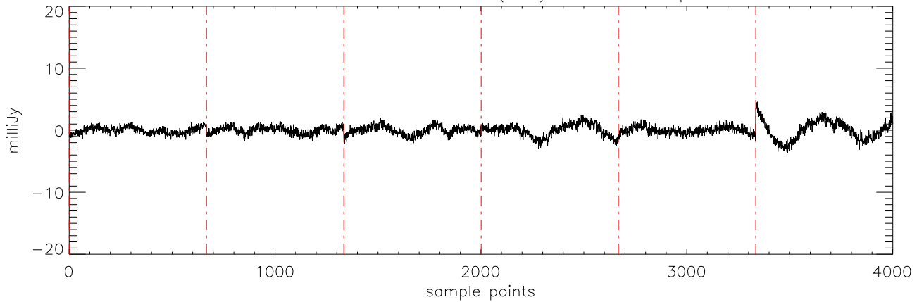
a2471 J01514155 27oct11 (AST) StokesU freq:4750.
