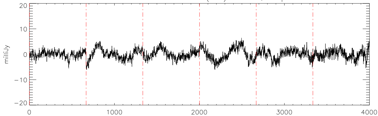
a2471 J01514155 27oct11 (AST) StokesQ freq:4892.
