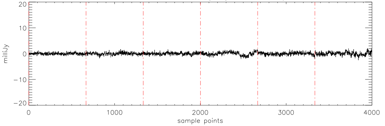
a2471 J01514155 27oct11 (AST) StokesV freq:4750.
