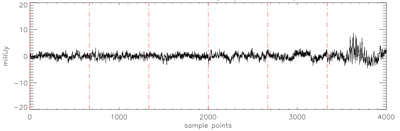
a2471 J01514155 27oct11 (AST) StokesV freq:5176.
