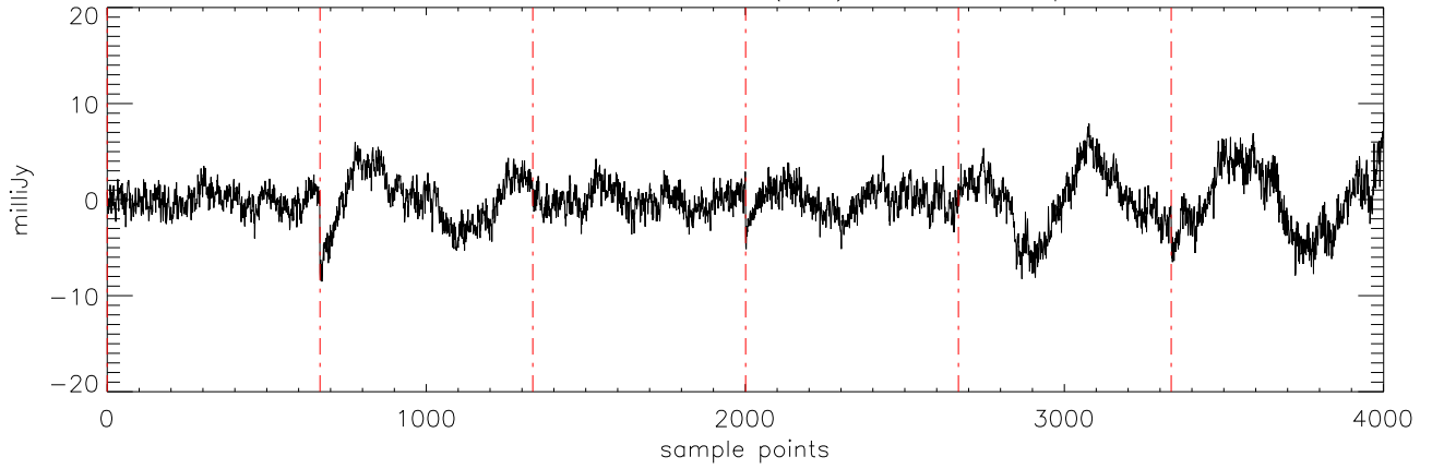
a2471 J01514155 27oct11 (AST) StokesQ freq:4750.
