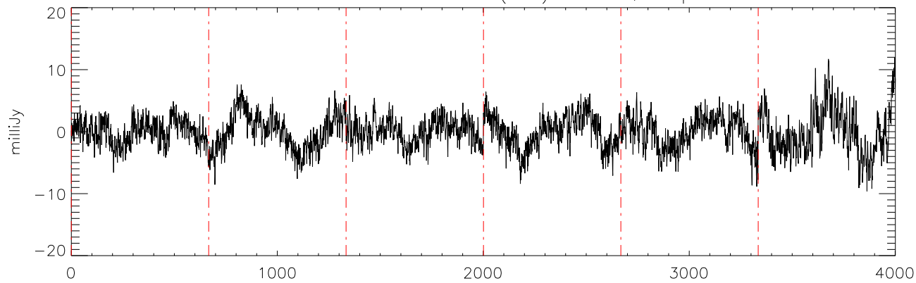
a2471 J01514155 27oct11 (AST) StokesQ freq:5176.
