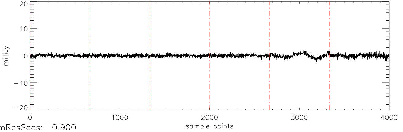
a2471 J01514155 27oct11 (AST) StokesV freq:5034.
