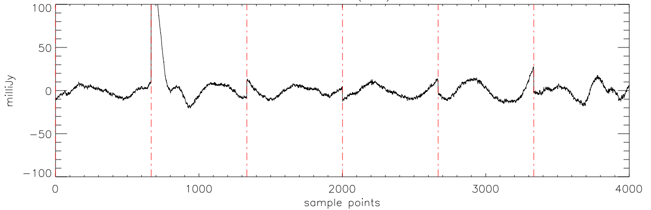
\alpha 2471 J01514155 27oct11 (AST) StokesI freq:4750.
