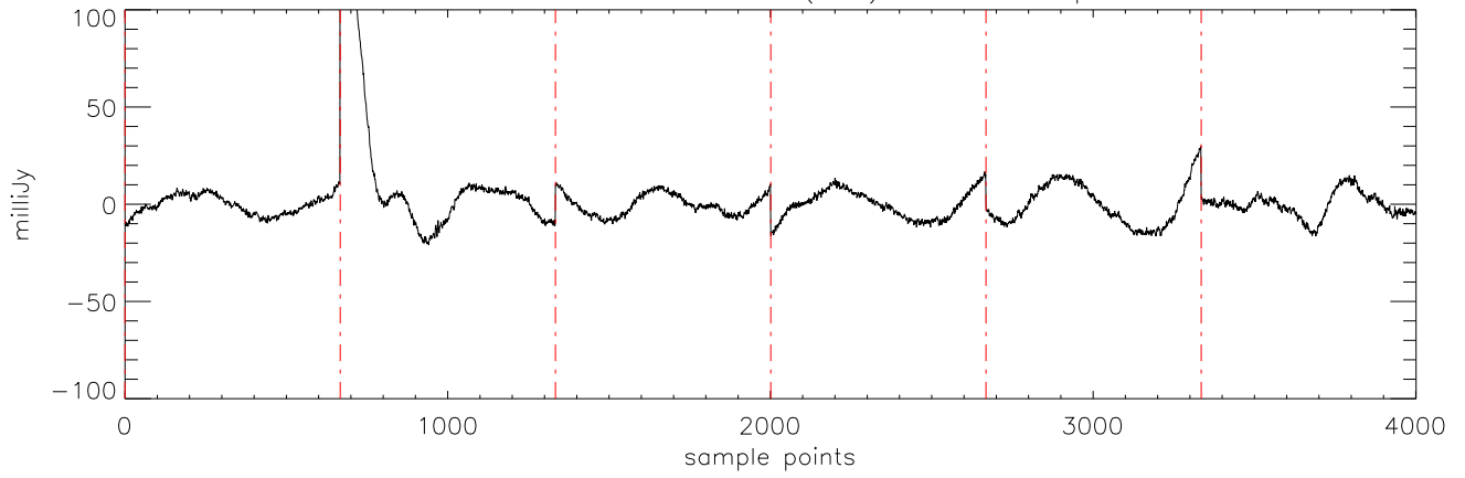
\alpha 2471 J01514155 27oct11 (AST) StokesI freq:4608.
