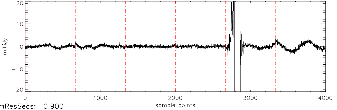
a2471 J01514155 27oct11 (AST) StokesU freq:4466.
