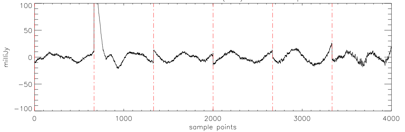
\alpha 2471 J01514155 27oct11 (AST) StokesI freq:5176.
