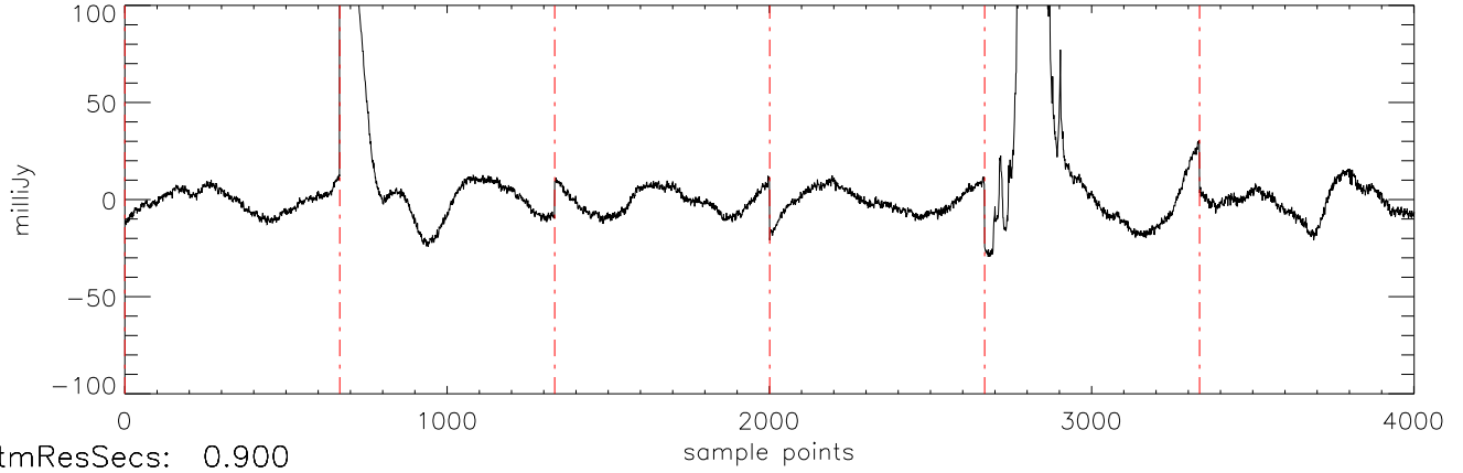
\alpha 2471 J01514155 27oct11 (AST) StokesI freq:4466.
