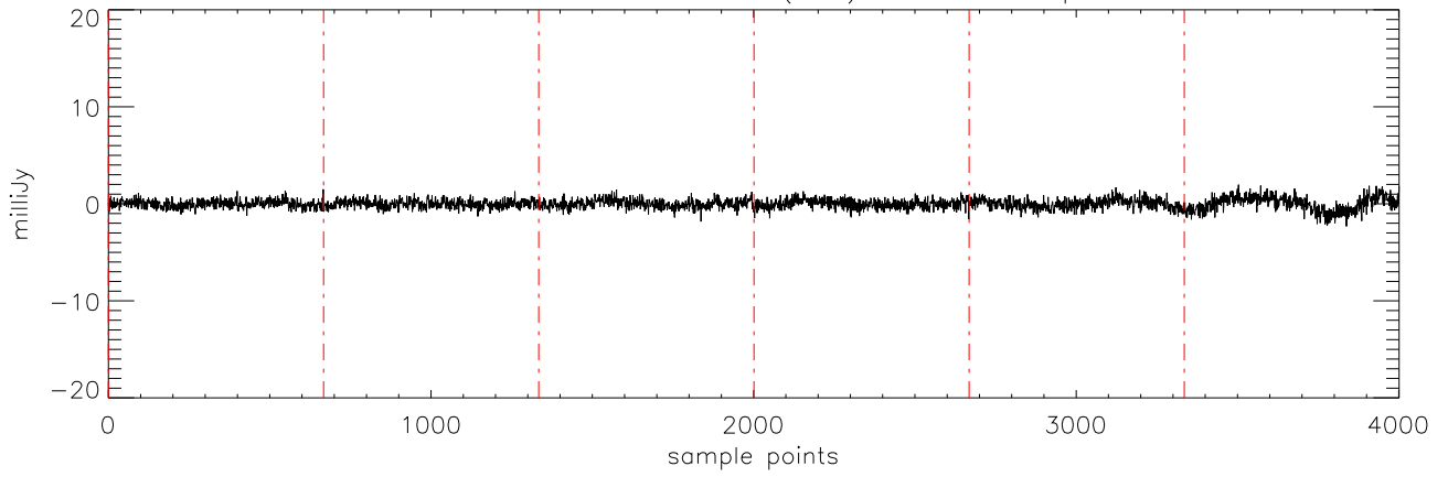
a2471 J01514155 27oct11 (AST) StokesV freq:4608.
