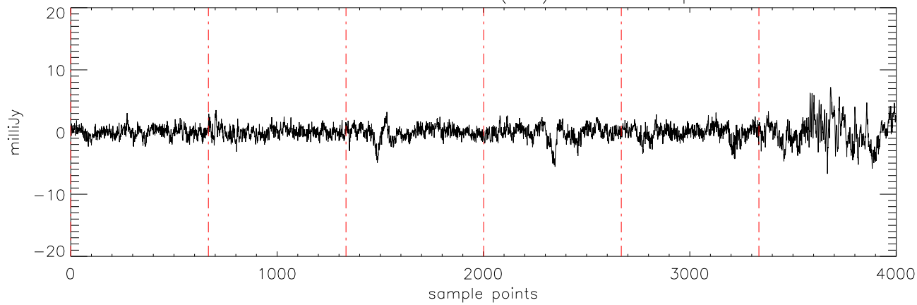
a2471 J01514155 27oct11 (AST) StokesU freq:5176.
