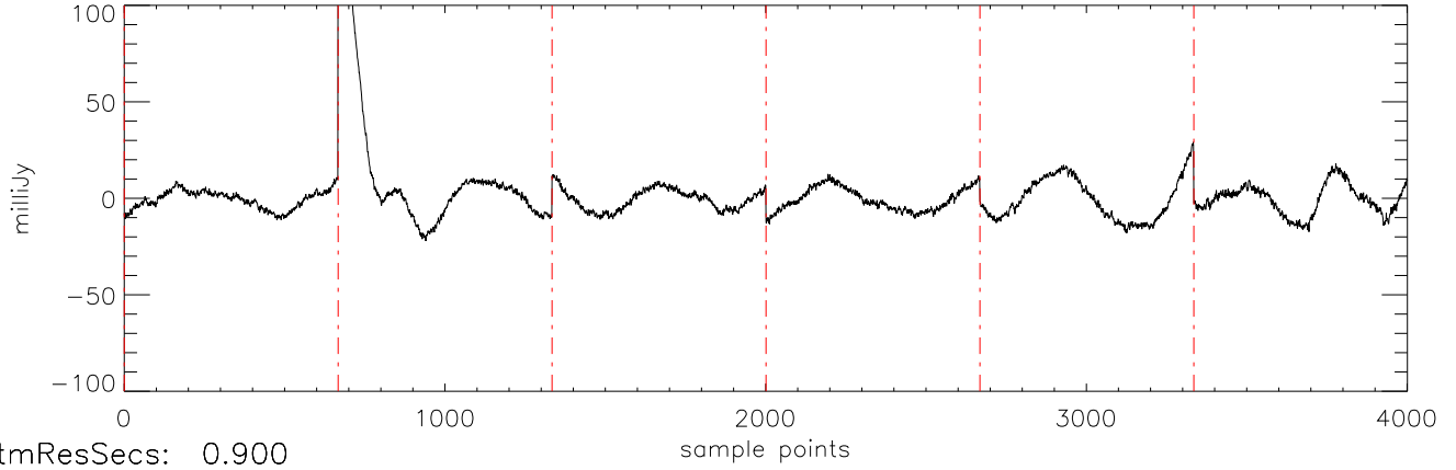
\alpha 2471 J01514155 27oct11 (AST) StokesI freq:5034.
