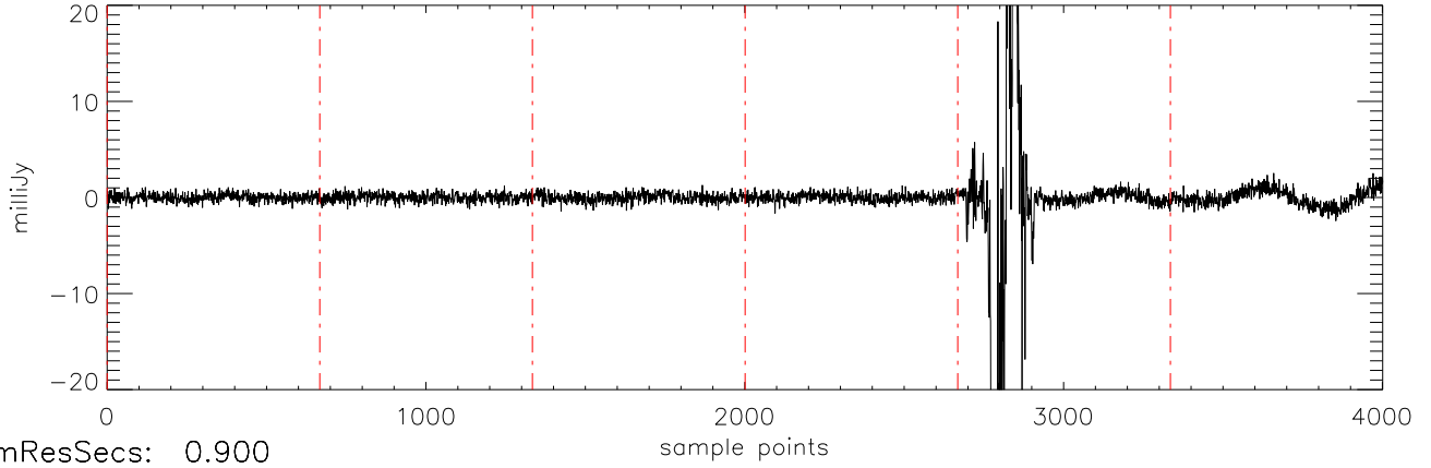
a2471 J01514155 27oct11 (AST) StokesV freq:4466.
