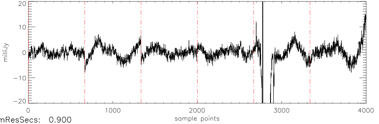
a2471 J01514155 27oct11 (AST) StokesQ freq:4466.
