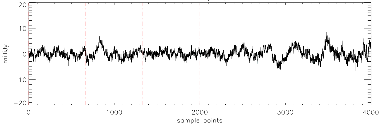
a2471 J01514155 27oct11 (AST) StokesQ freq:4608.
