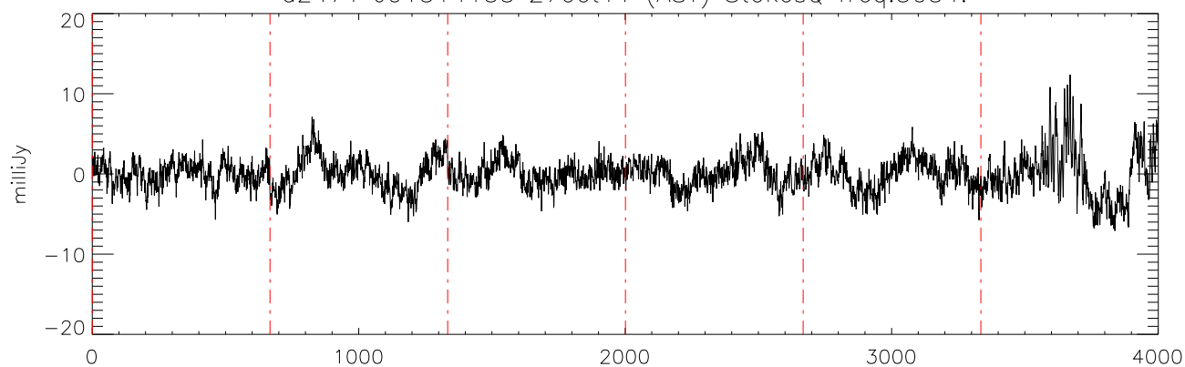
a2471 J01514155 27oct11 (AST) StokesQ freq:5034.
