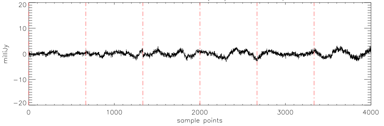
a2471 J01514155 27oct11 (AST) StokesU freq:4608.
