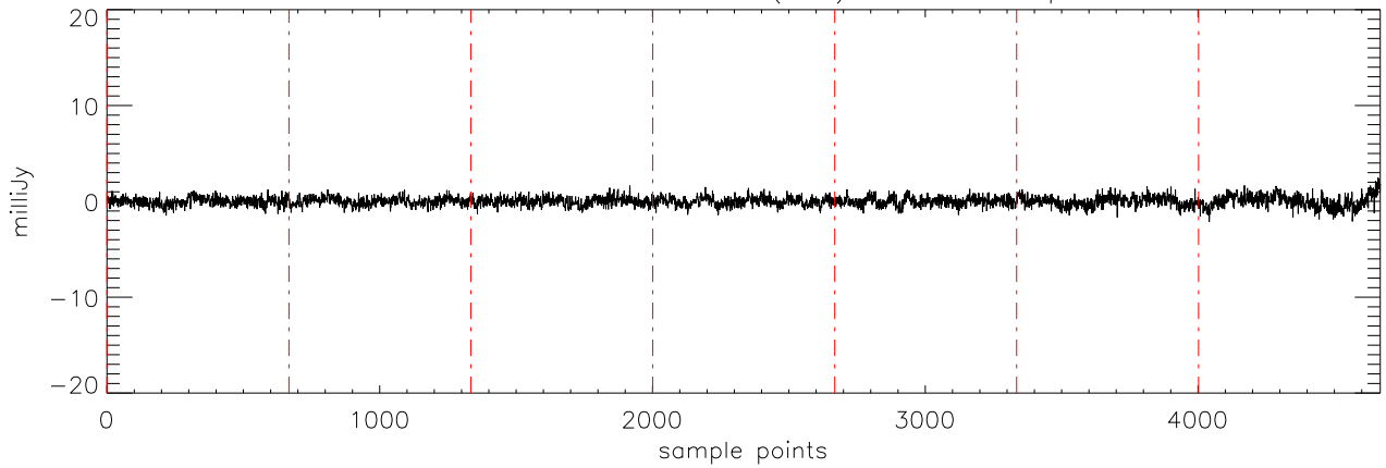
a2471 J01514155 10oct11 (AST) StokesV freq:4750.
