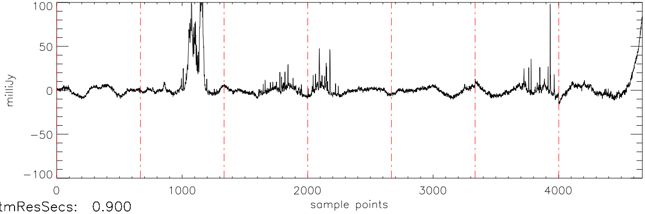
a2471 J01514155 10oct11 (AST) StokesI freq:4466.
