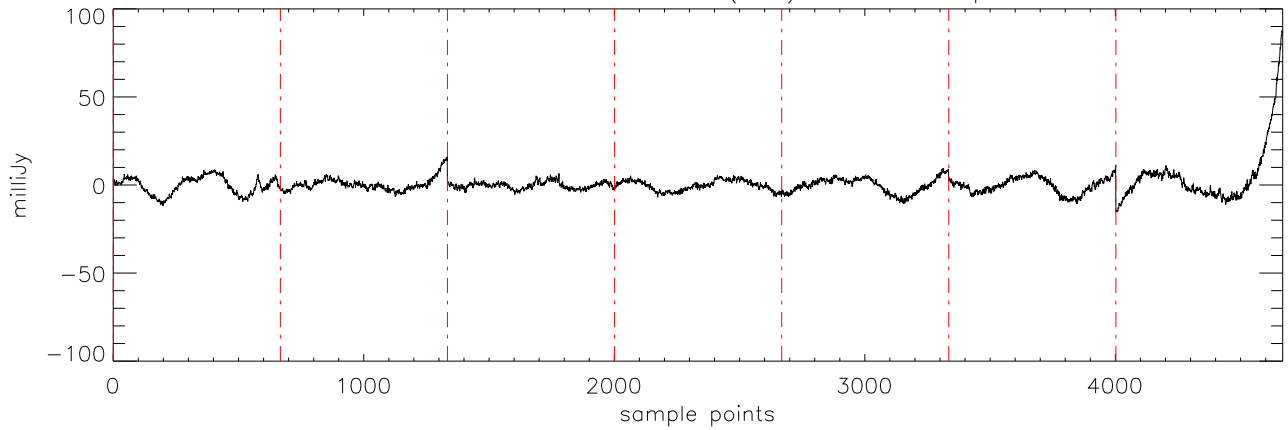
a2471 J01514155 10oct11 (AST) StokesI freq:4608.
