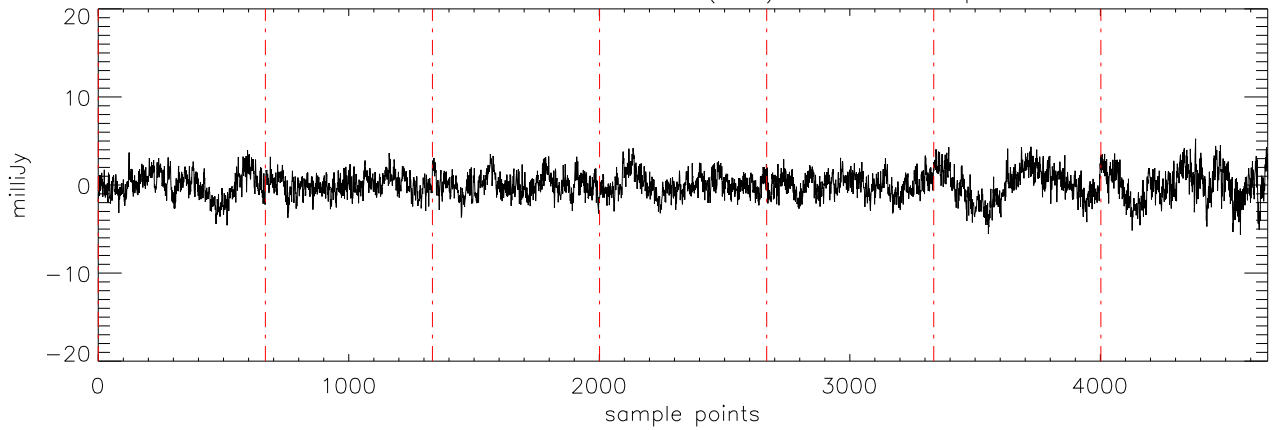
a2471 J01514155 10oct11 (AST) StokesQ freq:4608.
