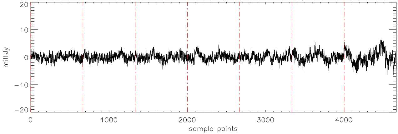
a2471 J01514155 10oct11 (AST) StokesQ freq:4750.
