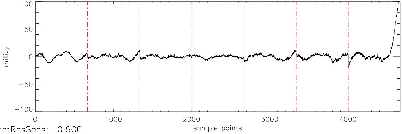
a2471 J01514155 10oct11 (AST) StokesI freq:5034.
