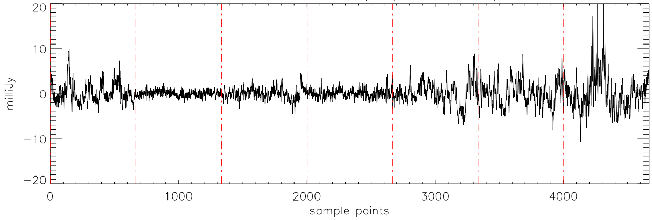
a2471 J01514155 10oct11 (AST) StokesV freq:5176.
