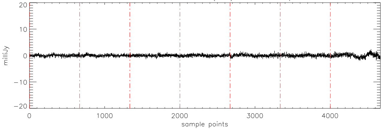
a2471 J01514155 10oct11 (AST) StokesV freq:4608.
