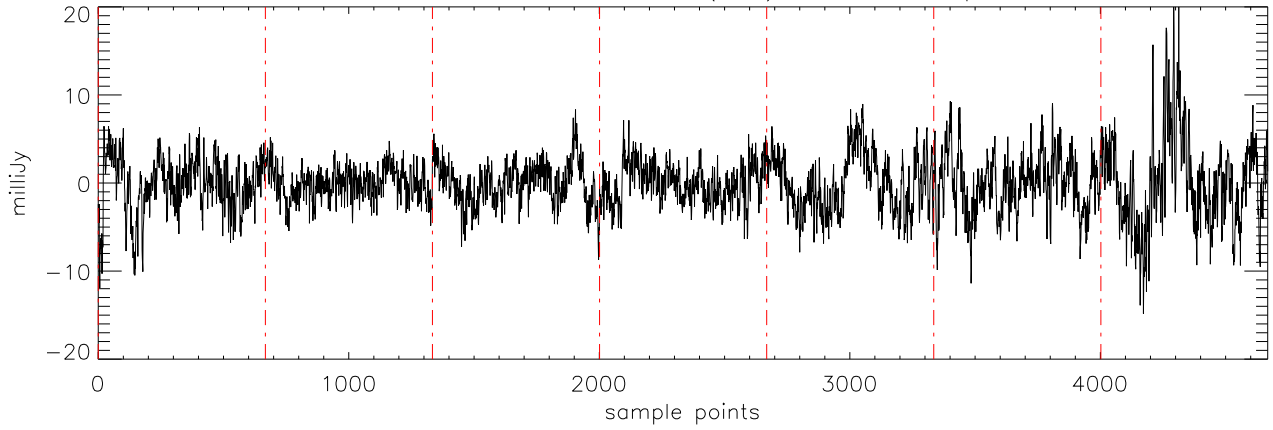
a2471 J01514155 10oct11 (AST) StokesQ freq:5176.
