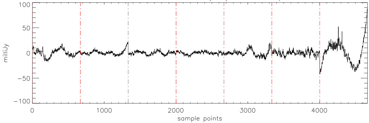
a2471 J01514155 10oct11 (AST) StokesI freq:5176.
