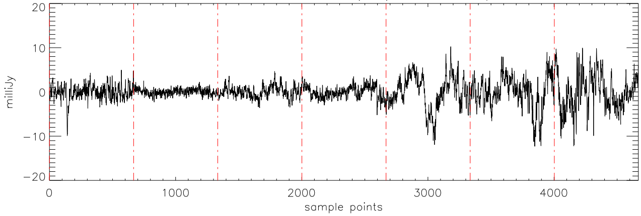
a2471 J01514155 10oct11 (AST) StokesU freq:5176.
