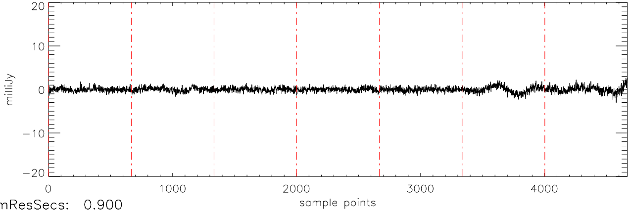
a2471 J01514155 10oct11 (AST) StokesV freq:5034.
