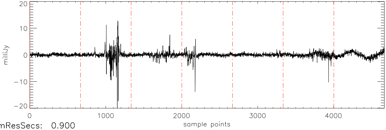
a2471 J01514155 10oct11 (AST) StokesV freq:4466.
