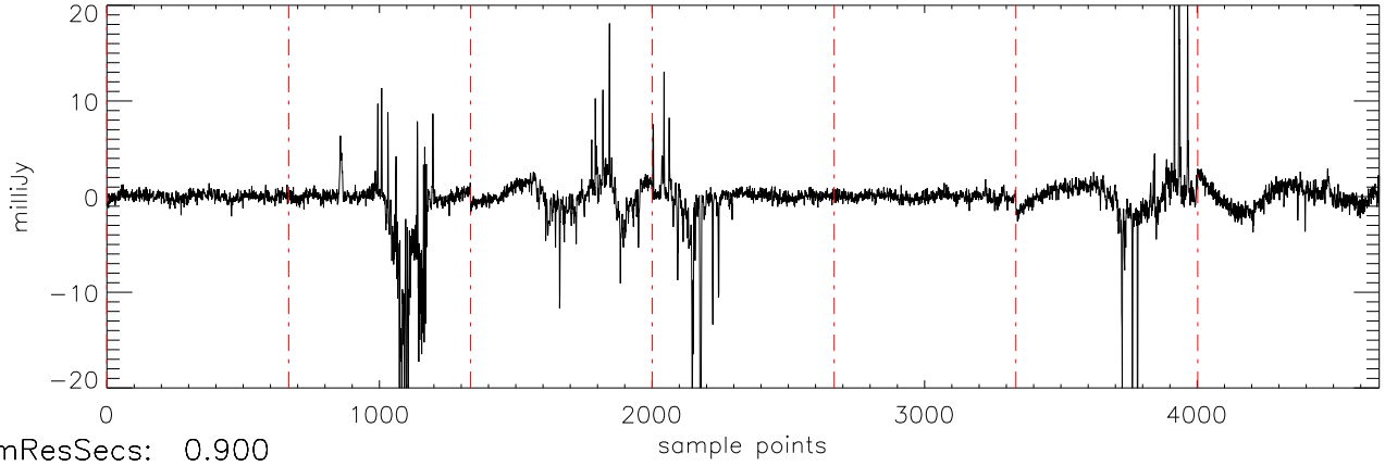
a2471 J01514155 10oct11 (AST) StokesU freq:4466.
