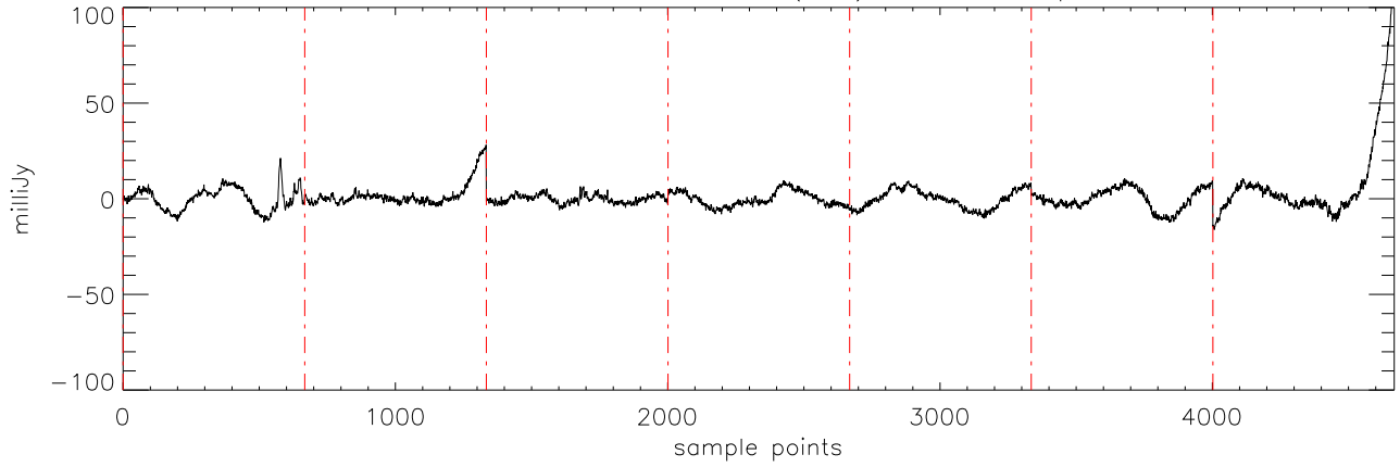
a2471 J01514155 10oct11 (AST) StokesI freq:4750.
