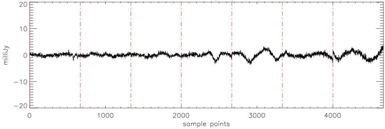
a2471 J01514155 10oct11 (AST) StokesU freq:4750.
