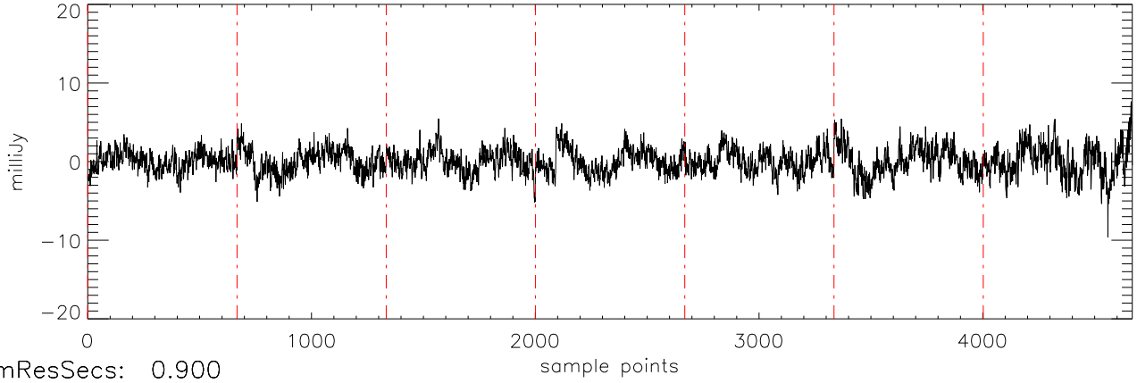
a2471 J01514155 10oct11 (AST) StokesQ freq:5034.
