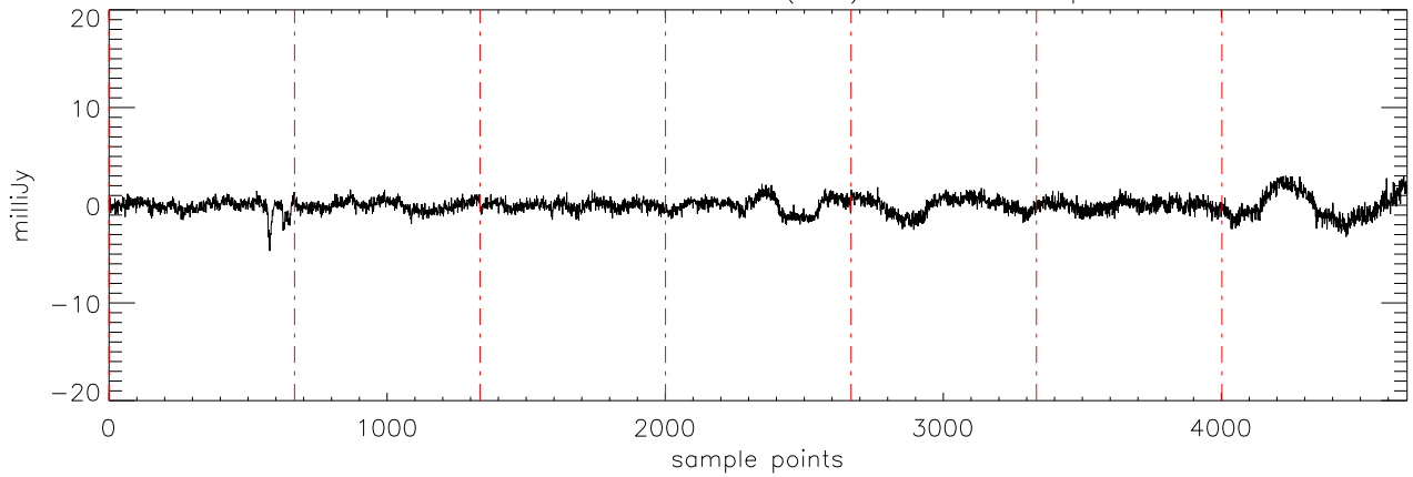
a2471 J01514155 10oct11 (AST) StokesU freq:4608.
