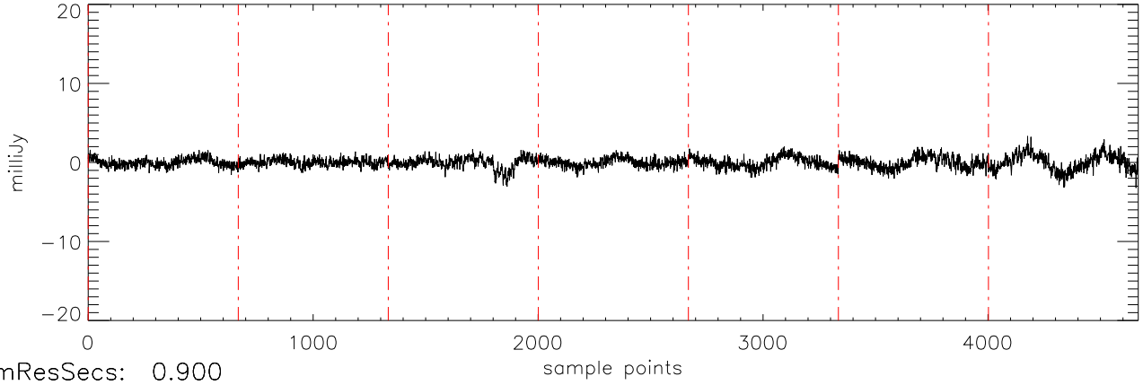
a2471 J01514155 10oct11 (AST) StokesU freq:5034.
