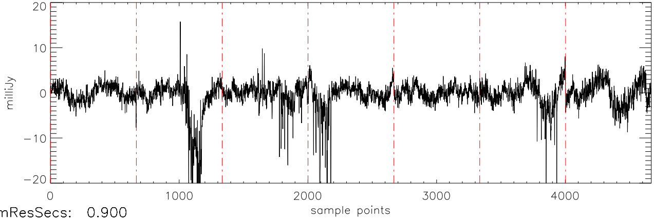
a2471 J01514155 10oct11 (AST) StokesQ freq:4466.
