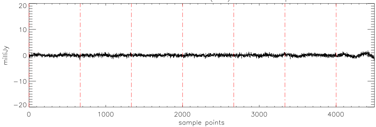
a2471 J01514155 17dec10 (AST) StokesV freq:4750.
