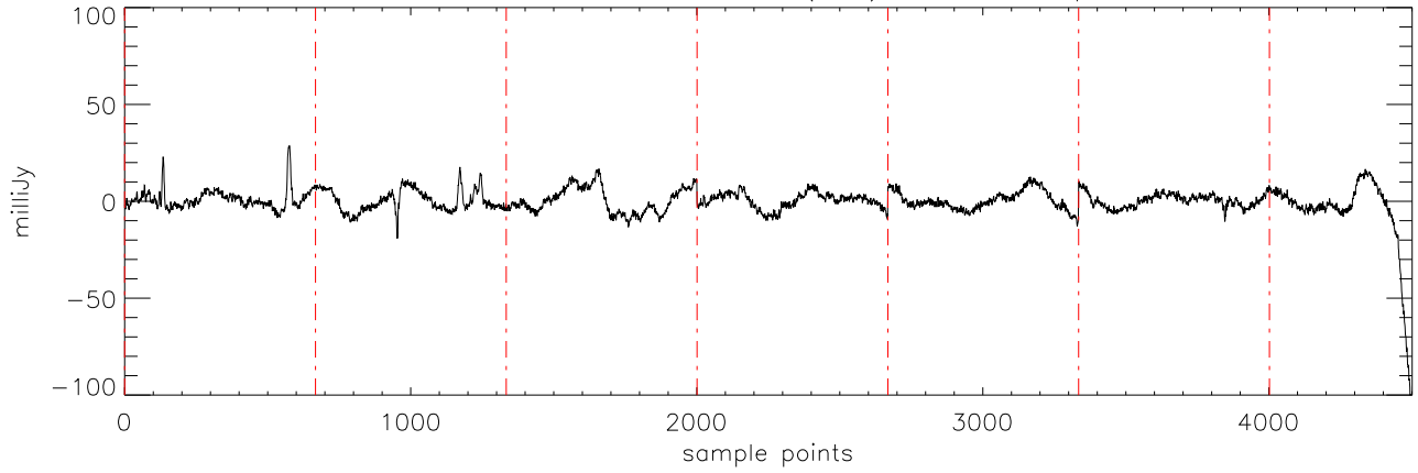
a2471 J01514155 17dec10 (AST) StokesI freq:4750.
