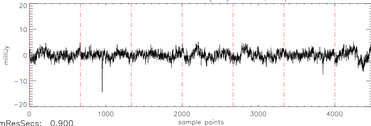
a2471 J01514155 17dec10 (AST) StokesQ freq:5034.
