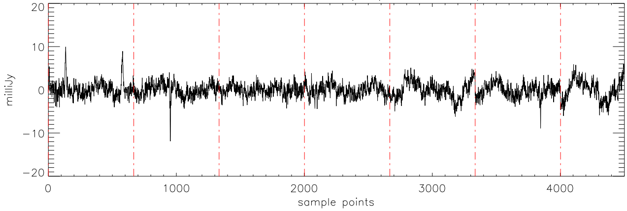
a2471 J01514155 17dec10 (AST) StokesQ freq:4750.
