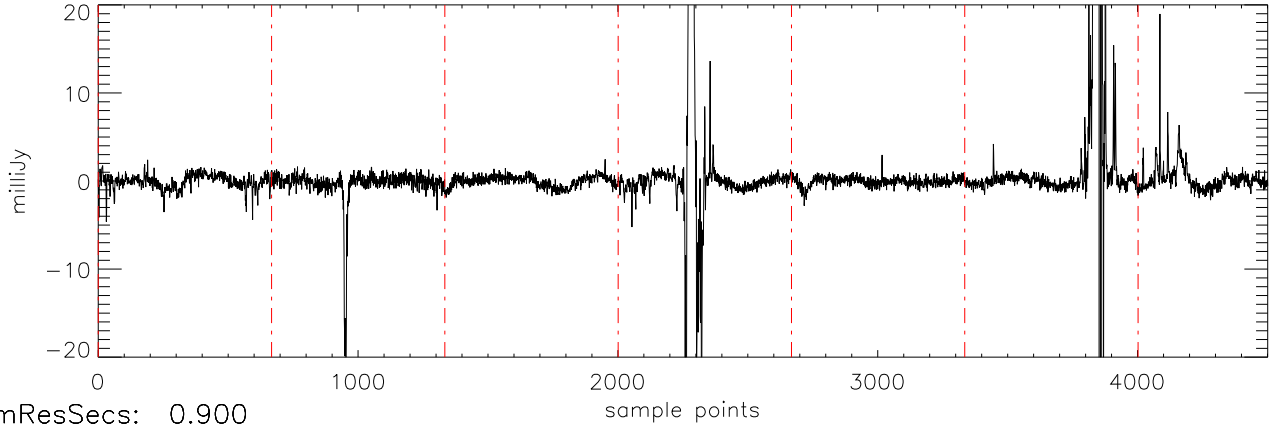
a2471 J01514155 17dec10 (AST) StokesU freq:4466.
