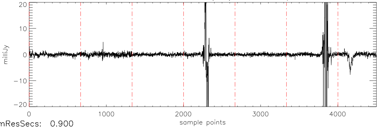
a2471 J01514155 17dec10 (AST) StokesV freq:4466.
