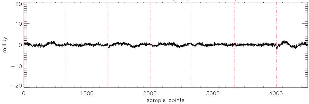
a2471 J01514155 17dec10 (AST) StokesU freq:4608.
