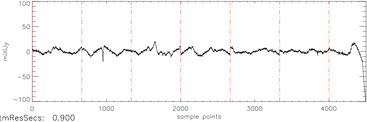
a2471 J01514155 17dec10 (AST) StokesI freq:5034.
