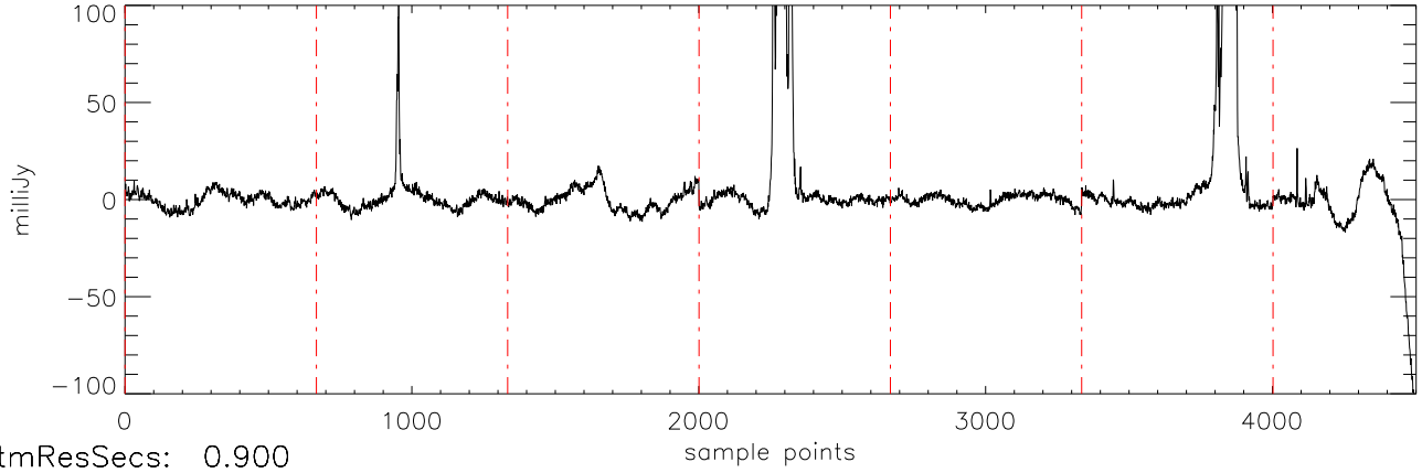
a2471 J01514155 17dec10 (AST) StokesI freq:4466.
