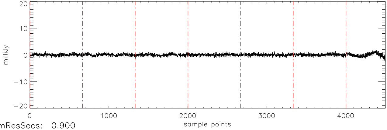
a2471 J01514155 17dec10 (AST) StokesV freq:5034.
