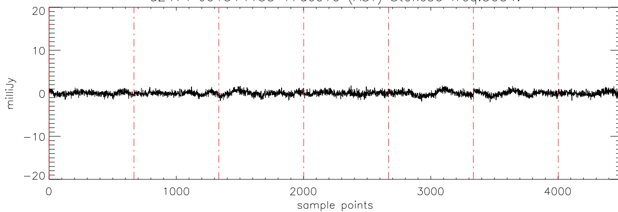
a2471 J01514155 17dec10 (AST) StokesU freq:5176.
