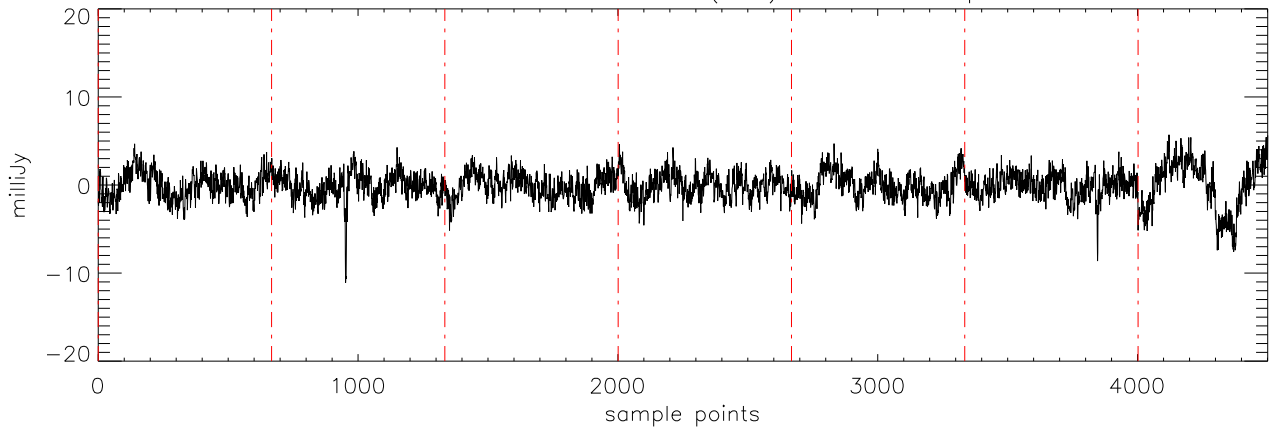
a2471 J01514155 17dec10 (AST) StokesQ freq:4608.
