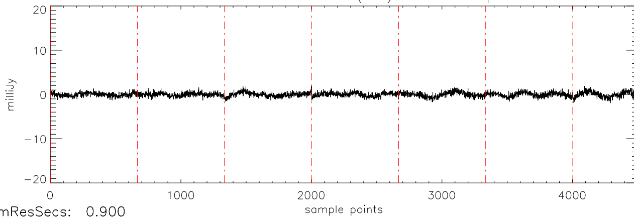
a2471 J01514155 17dec10 (AST) StokesU freq:5034.
