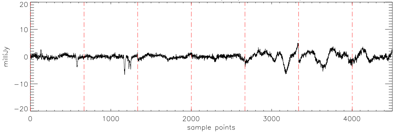
a2471 J01514155 17dec10 (AST) StokesU freq:4750.
