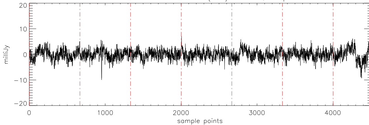
a2471 J01514155 17dec10 (AST) StokesQ freq:5176.
