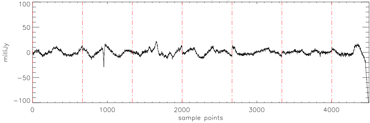
a2471 J01514155 17dec10 (AST) StokesI freq:5176.
