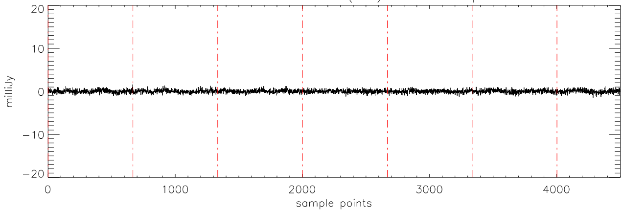
a2471 J01514155 17dec10 (AST) StokesV freq:4608.
