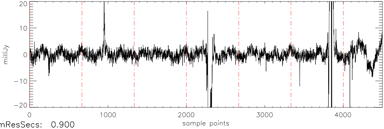
a2471 J01514155 17dec10 (AST) StokesQ freq:4466.
