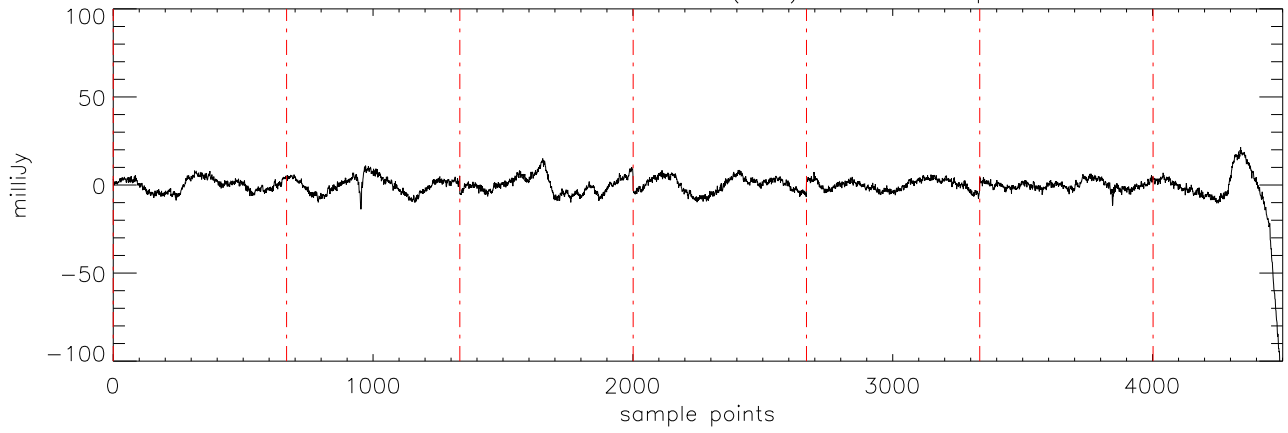
a2471 J01514155 17dec10 (AST) StokesI freq:4608.
