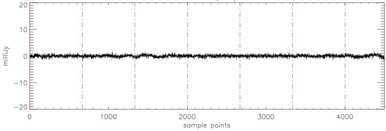
a2471 J01514155 17dec10 (AST) StokesV freq:5176.
