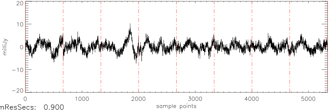
a2471 J0039191 18dec10 (AST) StokesQ freq:5034.
