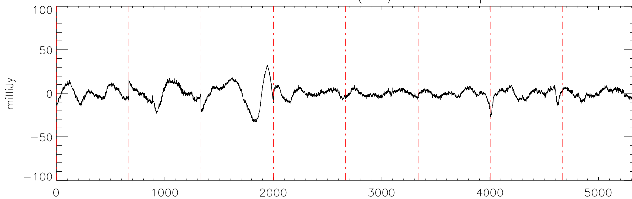
a2471 J0039191 18dec10 (AST) StokesI freq:4466.
