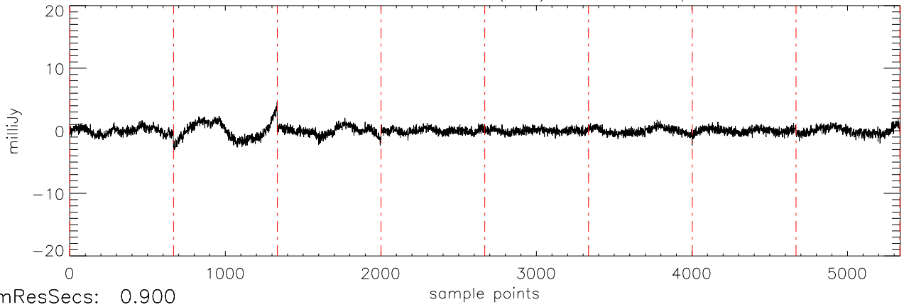
a2471 J0039191 18dec10 (AST) StokesU freq:5034.
