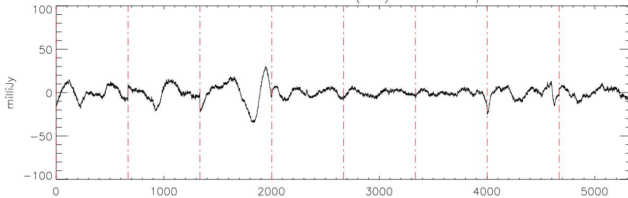
a2471 J0039191 18dec10 (AST) StokesI freq:4750.
