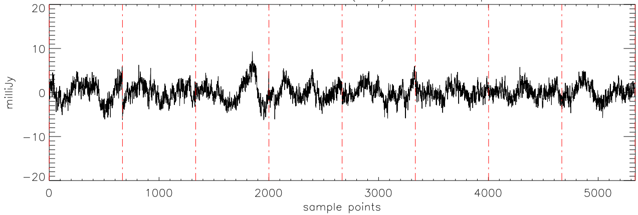
a2471 J0039191 18dec10 (AST) StokesQ freq:5176.
