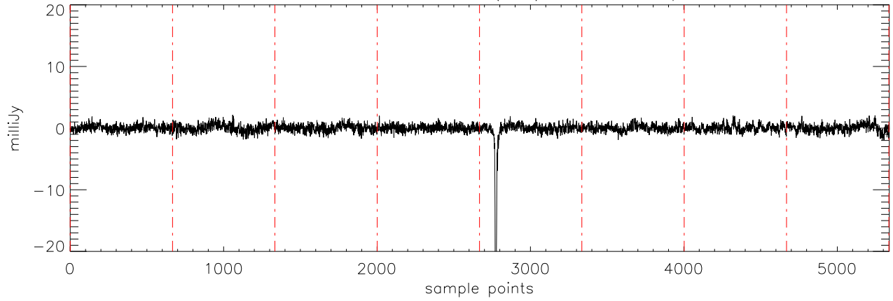
a2471 J0039191 18dec10 (AST) StokesV freq:5176.
