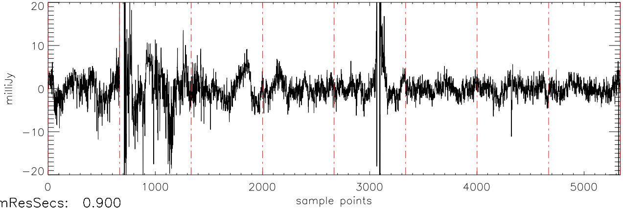
α2471 J0039191 18dec10 (AST) StokesQ freq:4466.
