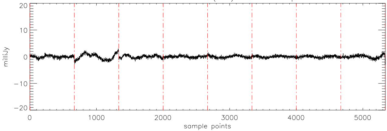
α2471 J0039191 18dec10 (AST) StokesU freq:4608.
