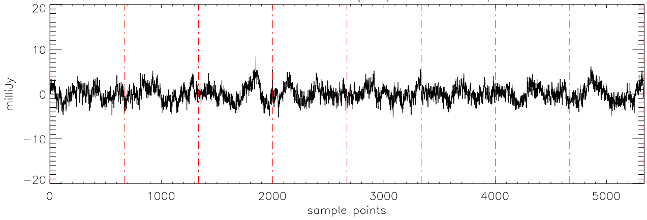
α2471 J0039191 18dec10 (AST) StokesQ freq:4608.
