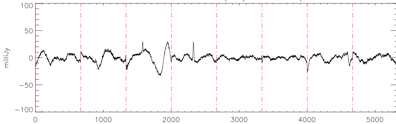
a2471 J0039191 18dec10 (AST) StokesI freq:4608.
