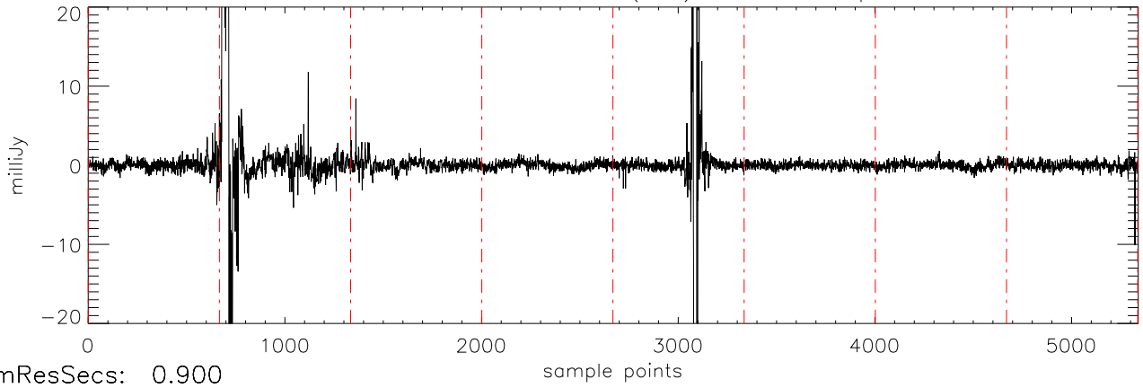
a2471 J0039191 18dec10 (AST) StokesV freq:4466.
