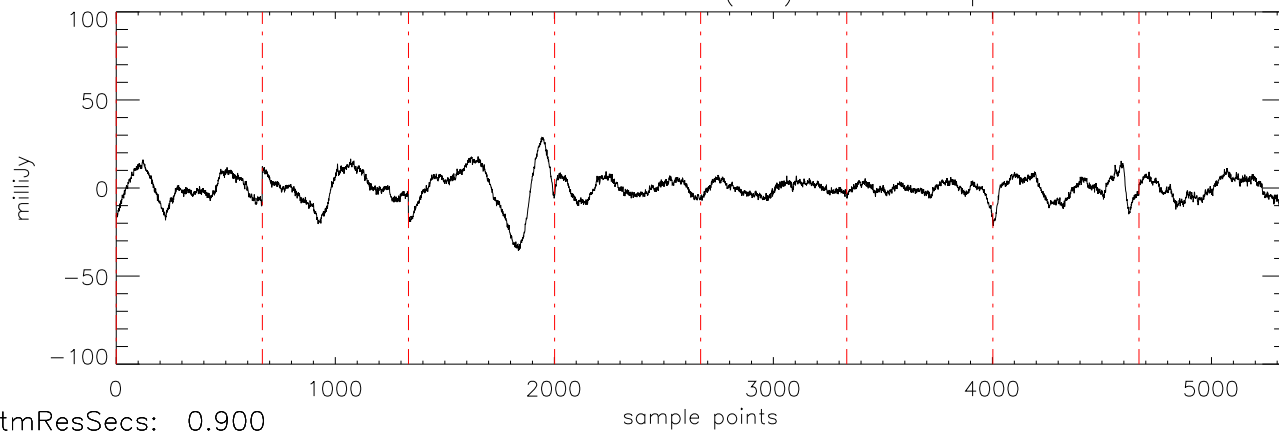
α2471 J0039191 18dec10 (AST) StokesI freq:5034.
