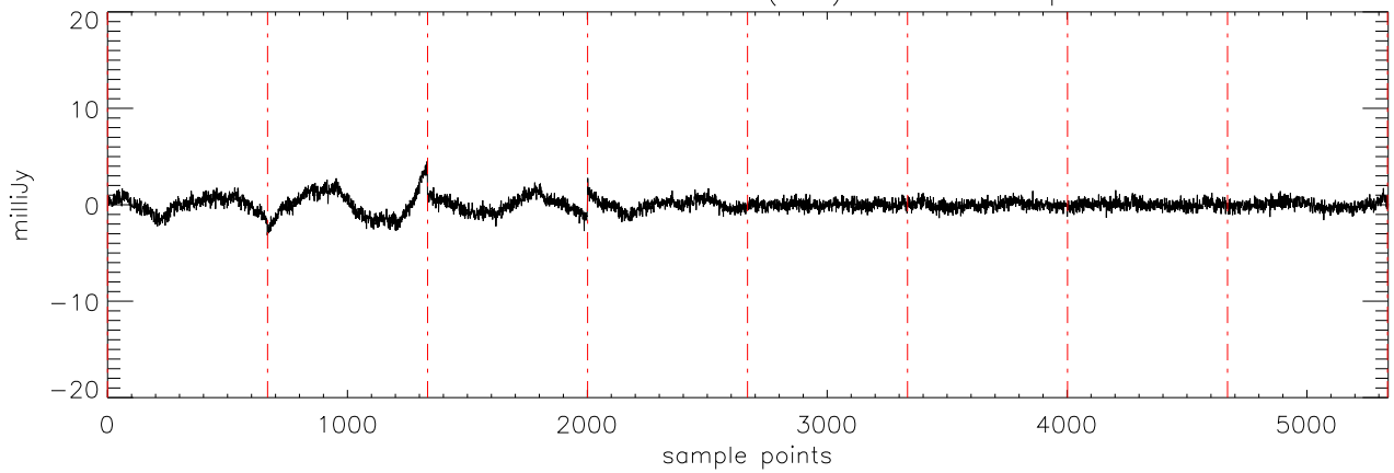
a2471 J0039191 18dec10 (AST) StokesU freq:5176.
