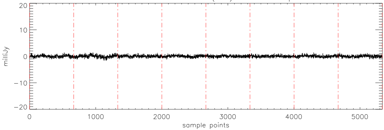
a2471 J0039191 18dec10 (AST) StokesV freq:4608.
