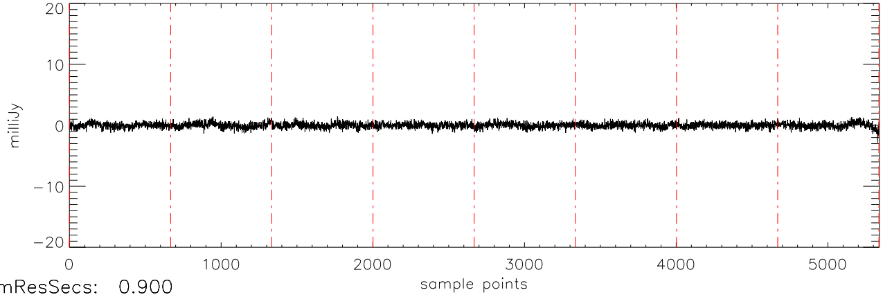
a2471 J0039191 18dec10 (AST) StokesV freq:5034.
