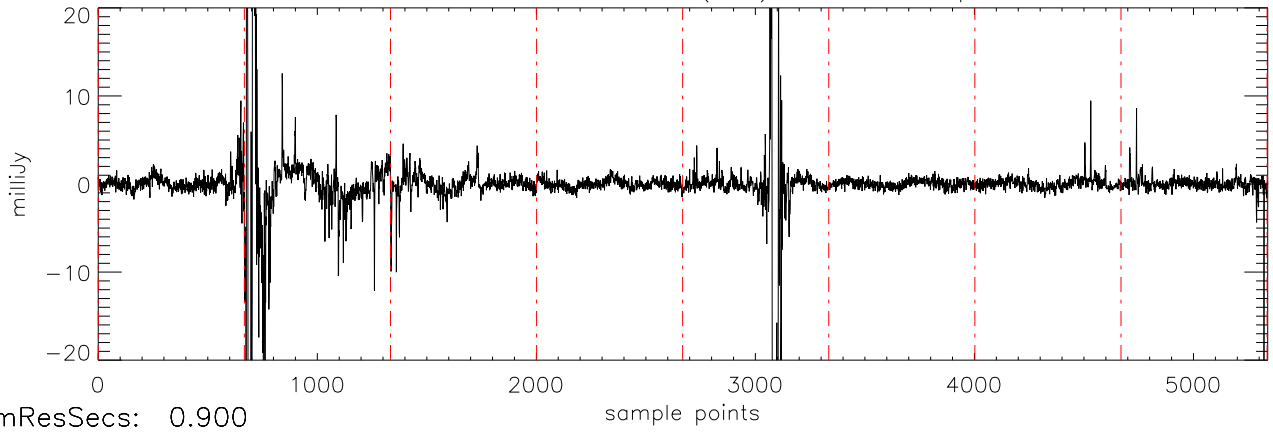
α2471 J0039191 18dec10 (AST) StokesU freq:4466.
