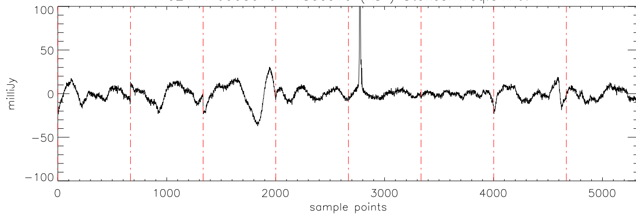
α2471 J0039191 18dec10 (AST) StokesI freq:5176.
