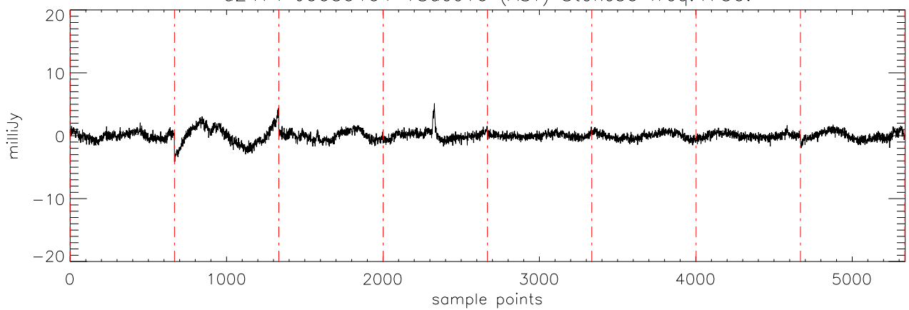
α2471 J0039191 18dec10 (AST) StokesU freq:4750.
