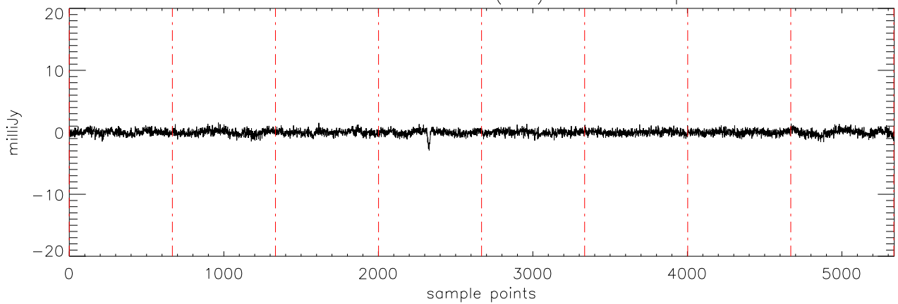
a2471 J0039191 18dec10 (AST) StokesV freq:4750.
