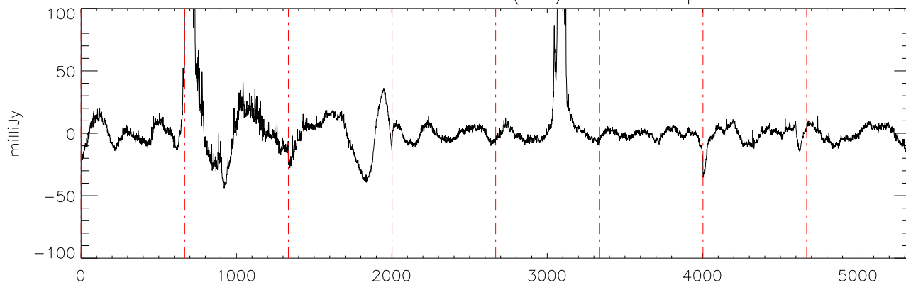
a2471 J0039191 18dec10 (AST) StokesI freq:4325.
