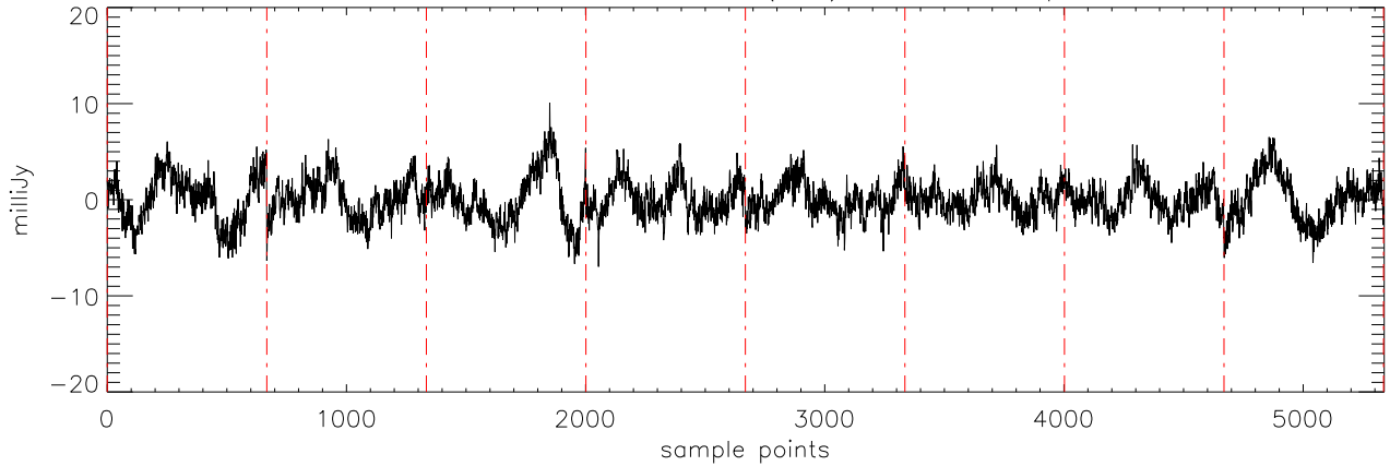
α2471 J0039191 18dec10 (AST) StokesQ freq:4750.
