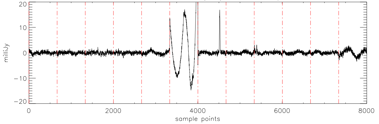
a2471 J0036159 05nov11 (AST) StokesU freq:4750.
