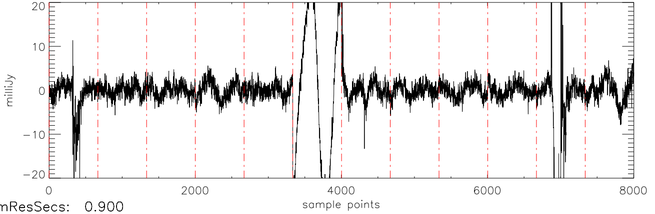
a2471 J0036159 05nov11 (AST) StokesQ freq:4466.
