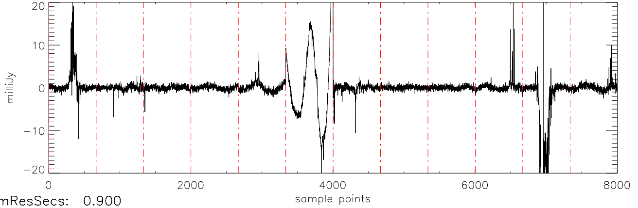
a2471 J0036159 05nov11 (AST) StokesU freq:4466.
