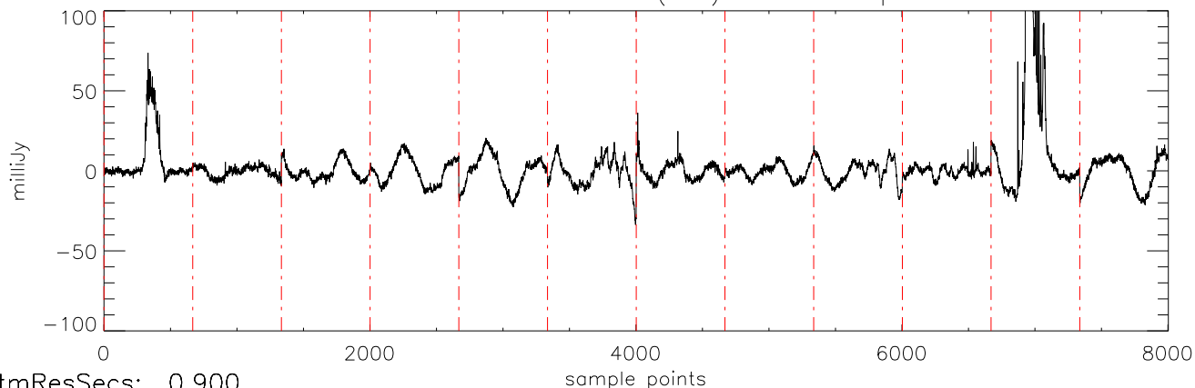
a2471 J0036159 05nov11 (AST) StokesI freq:4466.
