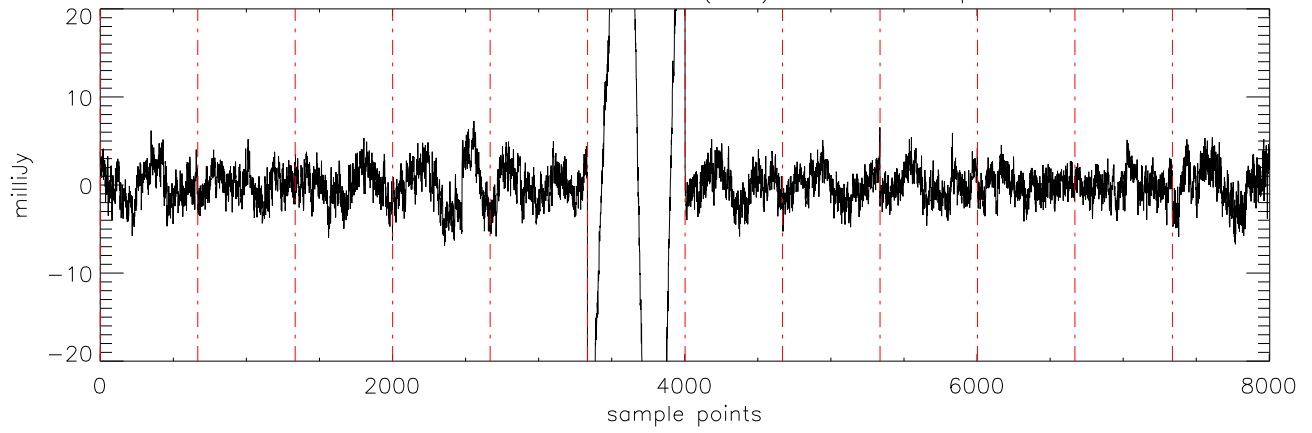
a2471 J0036159 05nov11 (AST) StokesQ freq:5176.
