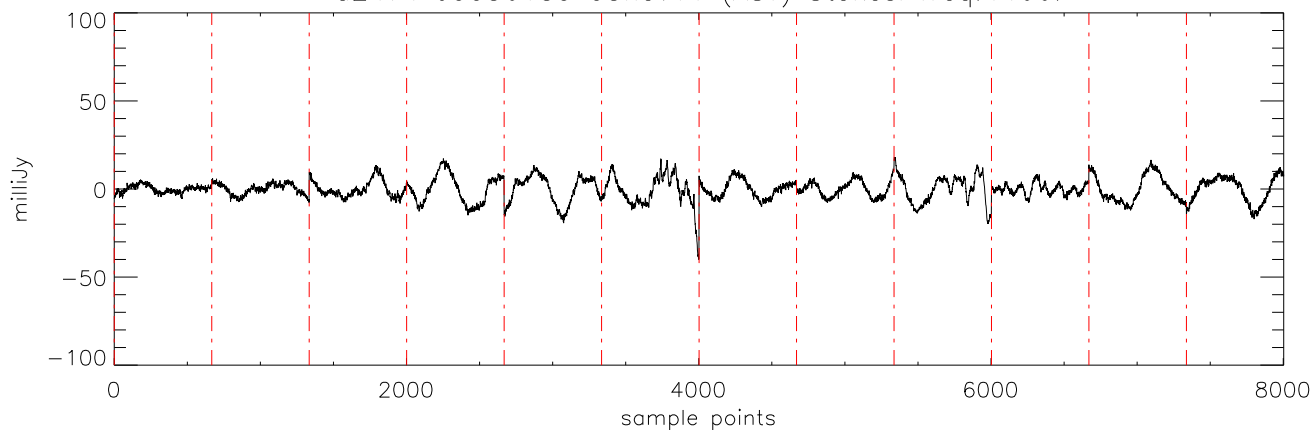
a2471 J0036159 05nov11 (AST) StokesI freq:4608.
