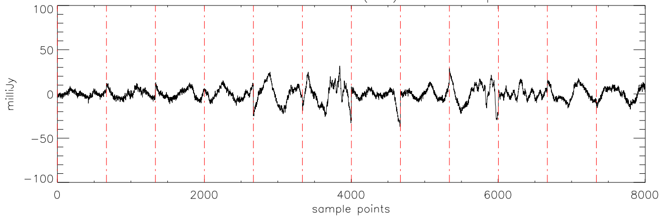
a2471 J0036159 05nov11 (AST) StokesI freq:5176.
