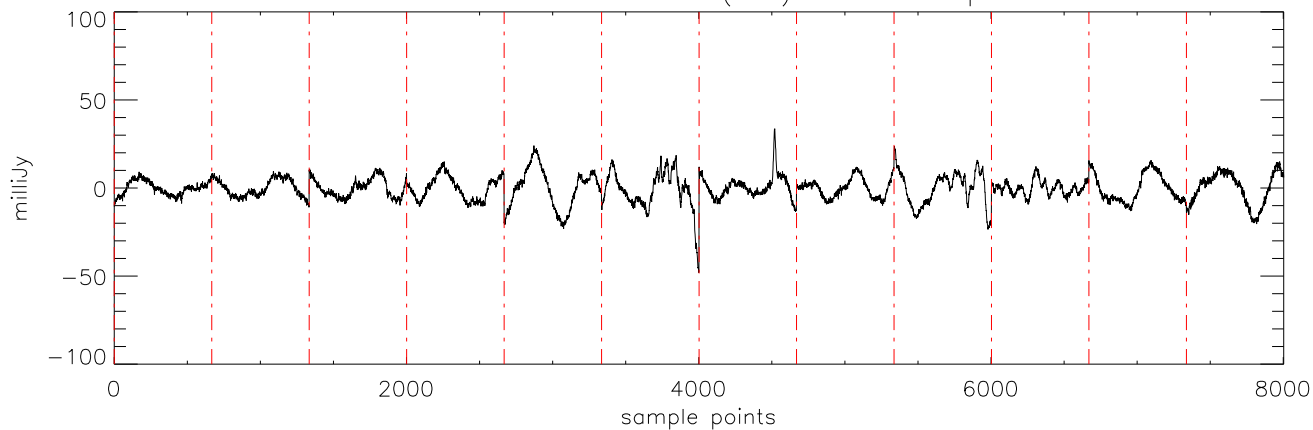
a2471 J0036159 05nov11 (AST) StokesI freq:4750.
