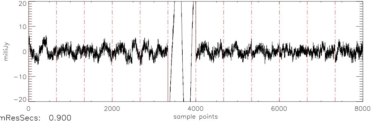
a2471 J0036159 05nov11 (AST) StokesQ freq:5034.
