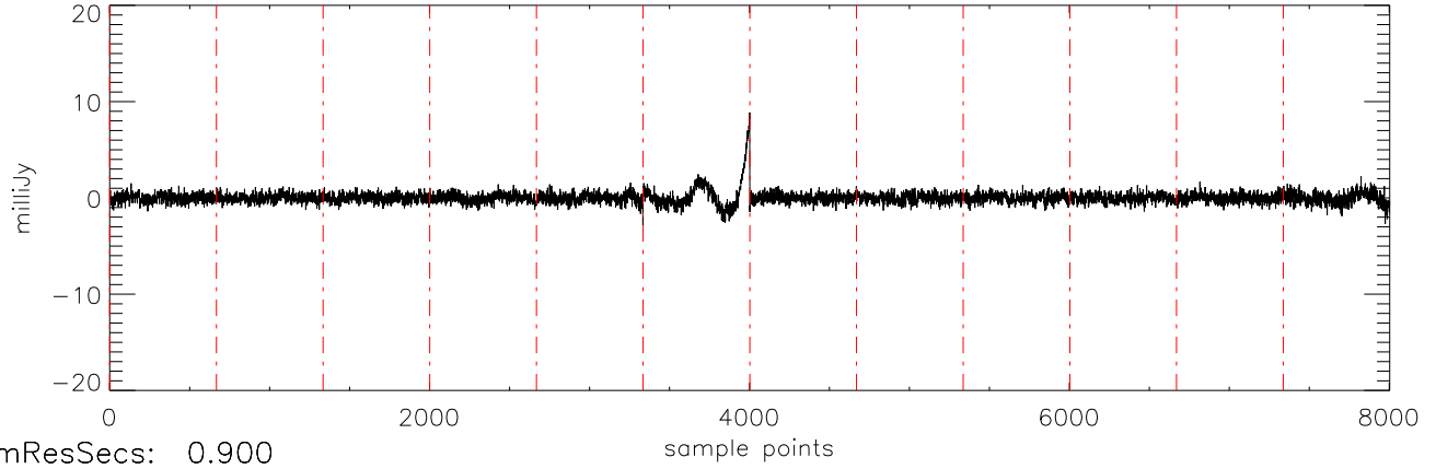
a2471 J0036159 05nov11 (AST) StokesV freq:5034.
