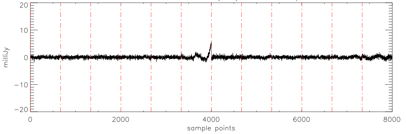
a2471 J0036159 05nov11 (AST) StokesV freq:4608.
