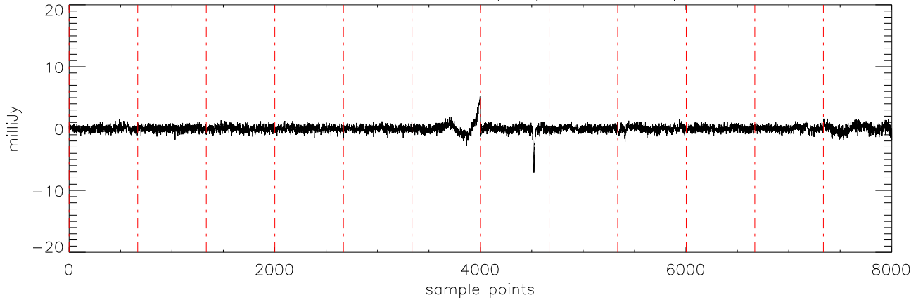
a2471 J0036159 05nov11 (AST) StokesV freq:4750.
