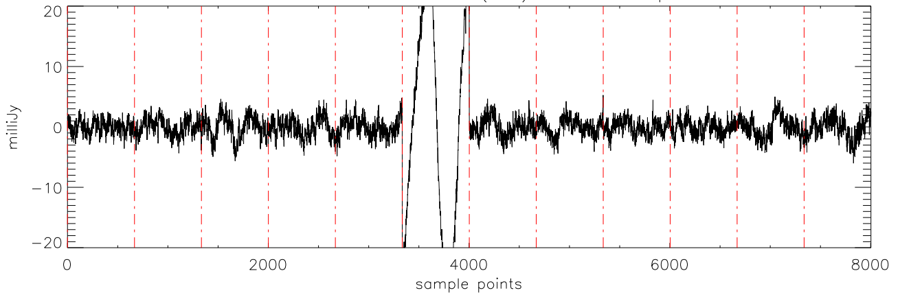
a2471 J0036159 05nov11 (AST) StokesQ freq:4608.
