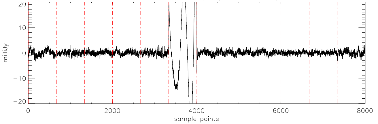
a2471 J0036159 05nov11 (AST) StokesU freq:5176.
