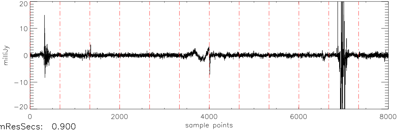
a2471 J0036159 05nov11 (AST) StokesV freq:4466.
