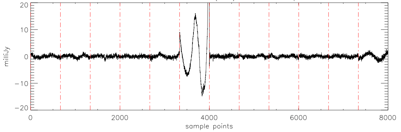
a2471 J0036159 05nov11 (AST) StokesU freq:4608.
