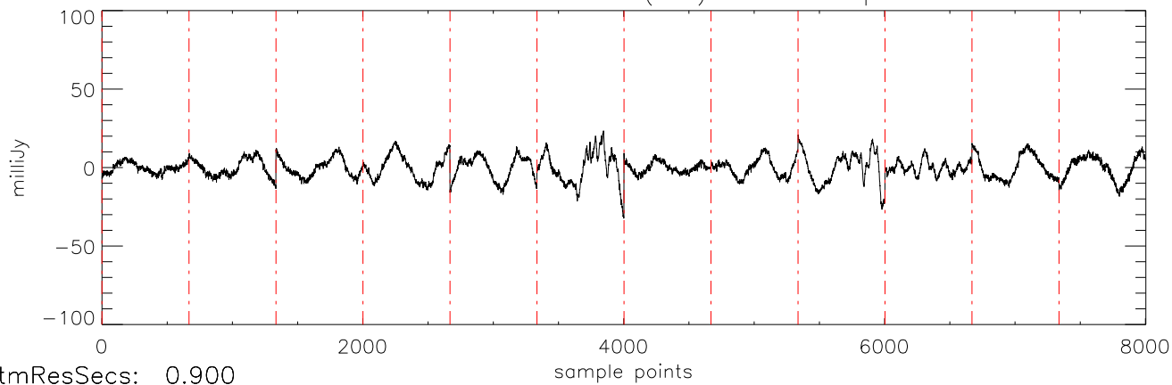
a2471 J0036159 05nov11 (AST) StokesI freq:5034.
