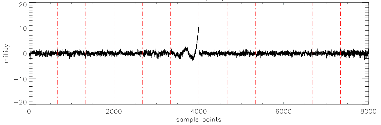
a2471 J0036159 05nov11 (AST) StokesV freq:5176.
