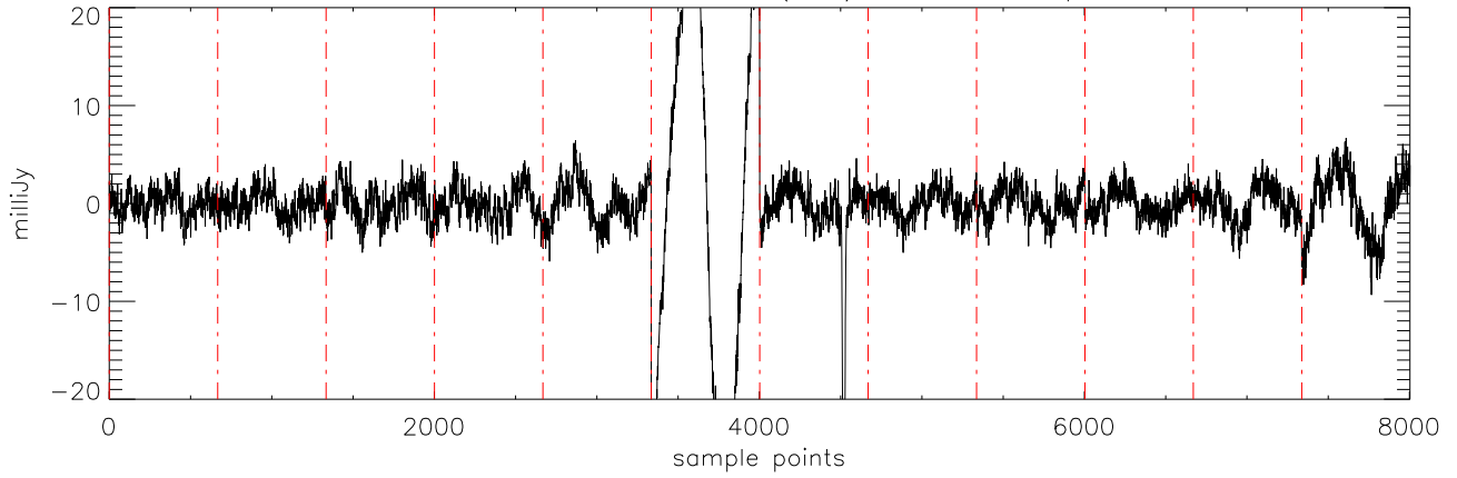
a2471 J0036159 05nov11 (AST) StokesQ freq:4750.
