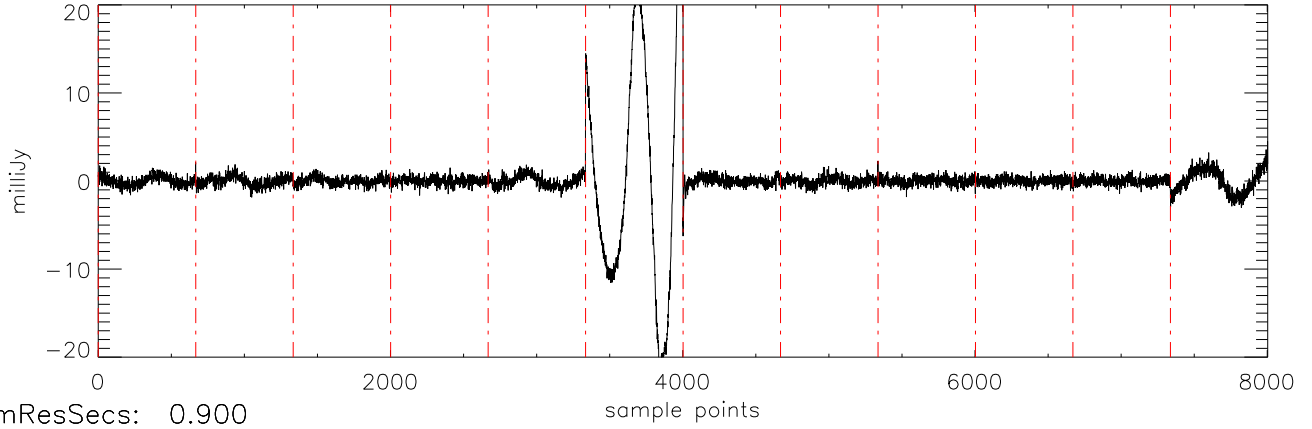
a2471 J0036159 05nov11 (AST) StokesU freq:5034.
