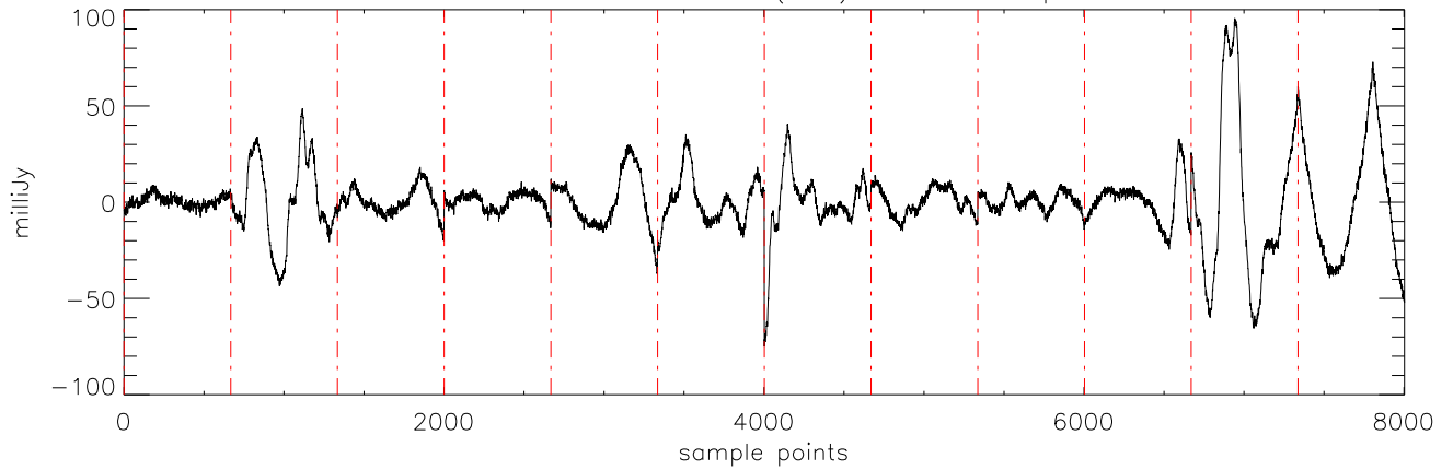
a2471 HR8799 17dec10 (AST) StokesI freq:5176.
