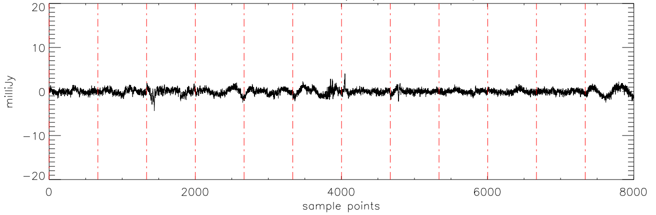
a2471 HR8799 17dec10 (AST) StokesU freq:4750.
