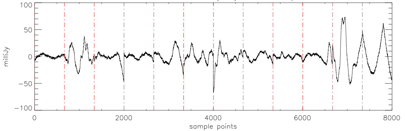
a2471 HR8799 17dec10 (AST) StokesI freq:4750.
