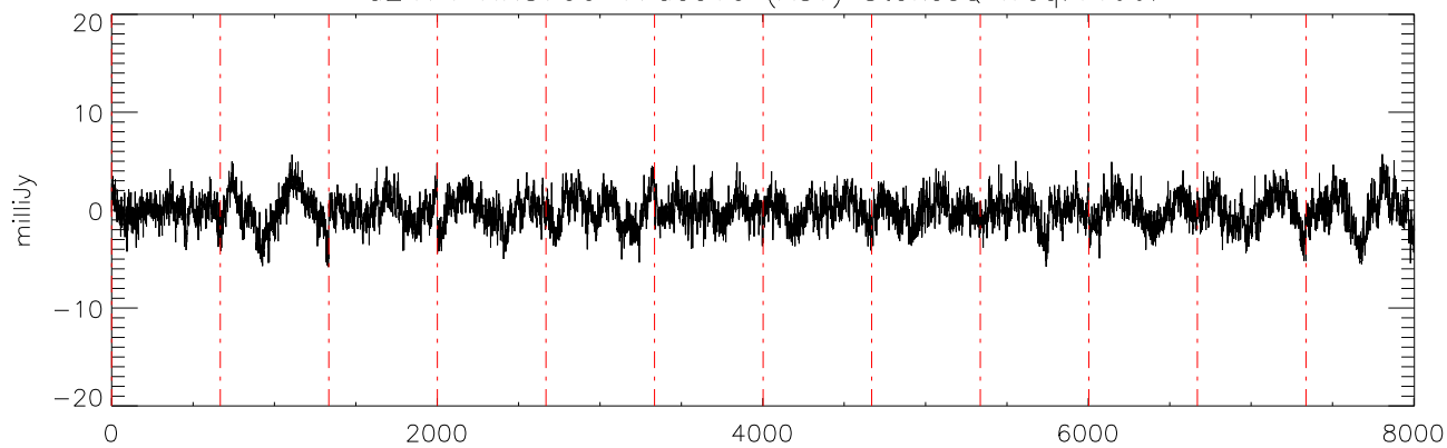
a2471 HR8799 17dec10 (AST) StokesQ freq:4466.
