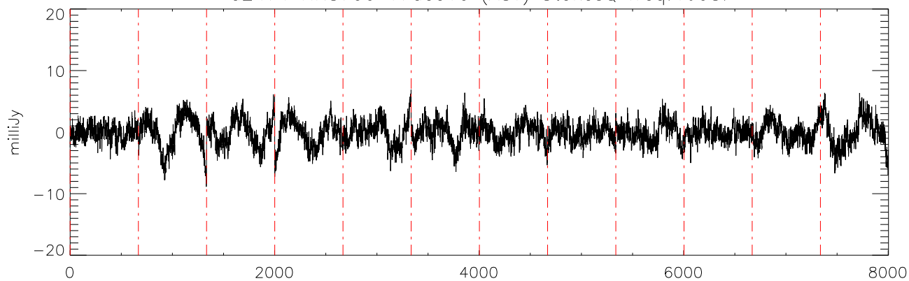
a2471 HR8799 17dec10 (AST) StokesQ freq:4608.
