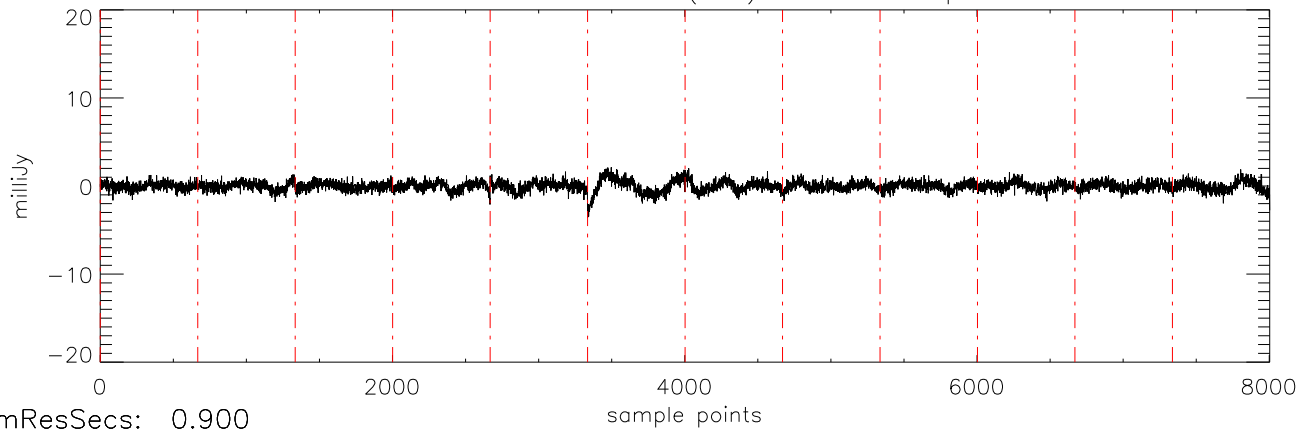
a2471 HR8799 17dec10 (AST) StokesU freq:5034.
