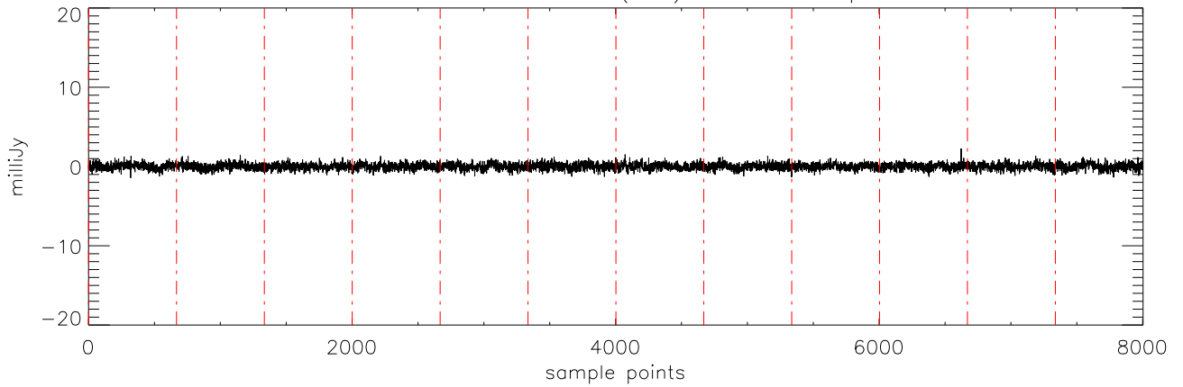
a2471 HR8799 17dec10 (AST) StokesV freq:4608.
