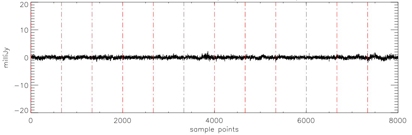
a2471 HR8799 17dec10 (AST) StokesV freq:4750.
