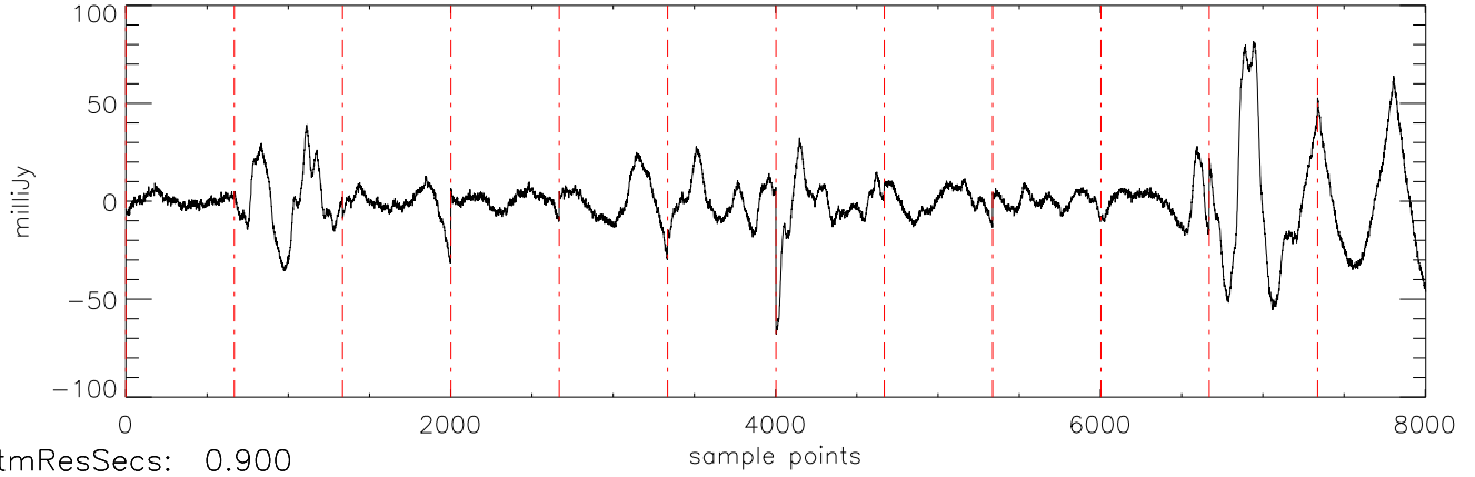
a2471 HR8799 17dec10 (AST) StokesI freq:5034.
