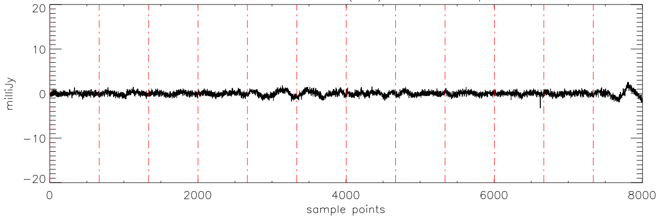
a2471 HR8799 17dec10 (AST) StokesU freq:4608.
