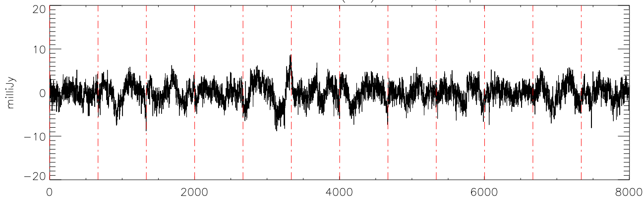
a2471 HR8799 17dec10 (AST) StokesQ freq:5176.
