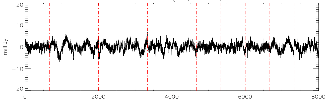
a2471 HR8799 17dec10 (AST) StokesQ freq:4750.
