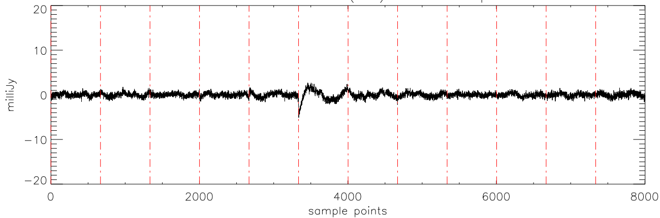
a2471 HR8799 17dec10 (AST) StokesU freq:5176.
