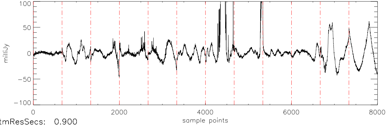
a2471 HR8799 17dec10 (AST) StokesI freq:4466.
