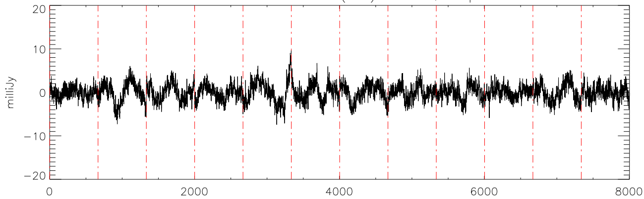
a2471 HR8799 17dec10 (AST) StokesQ freq:5034.
