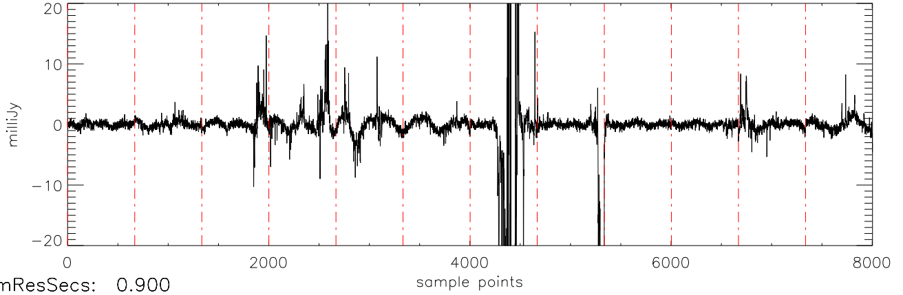
a2471 HR8799 17dec10 (AST) StokesU freq:4466.
