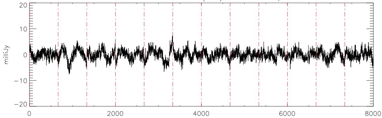
a2471 HR8799 17dec10 (AST) StokesQ freq:4892.
