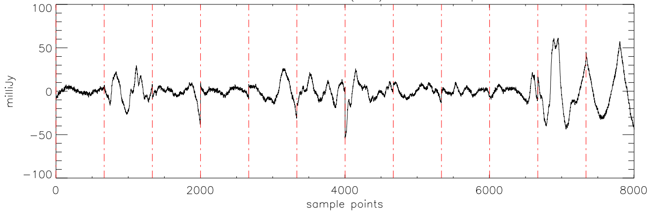
a2471 HR8799 17dec10 (AST) StokesI freq:4608.
