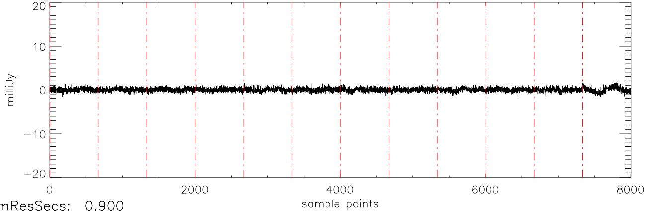
α2471 HR8799 17dec10 (AST) StokesV freq:5034.
