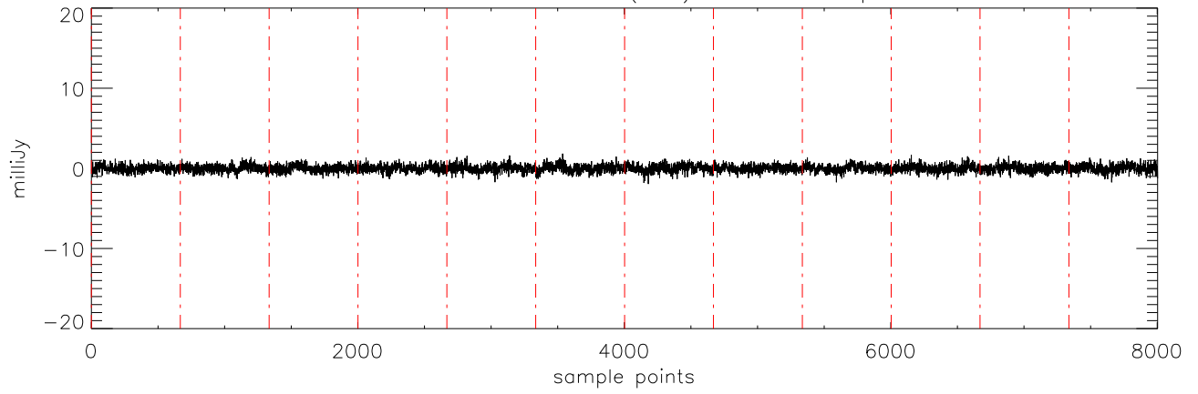
α2471 HR8799 17dec10 (AST) StokesV freq:5176.
