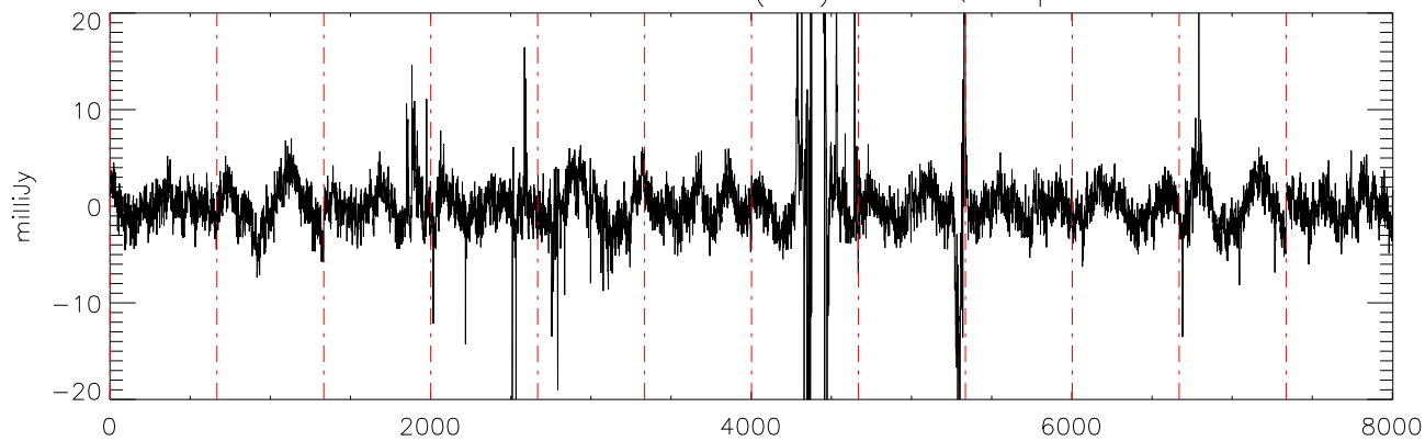
a2471 HR8799 17dec10 (AST) StokesQ freq:4325.
