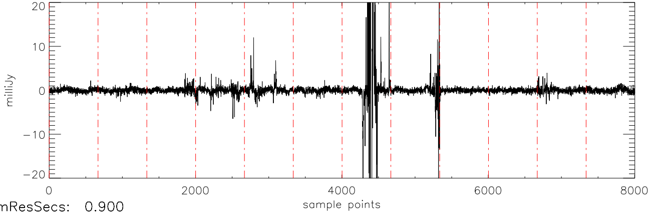
a2471 HR8799 17dec10 (AST) StokesV freq:4466.
