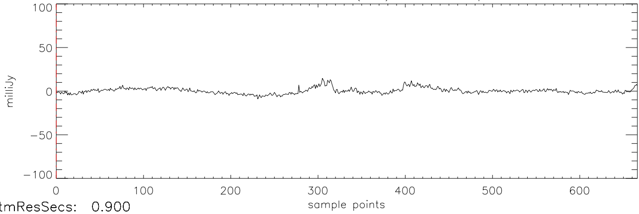
a2471 HD50554 18dec10 (AST) StokesI freq:4466.
