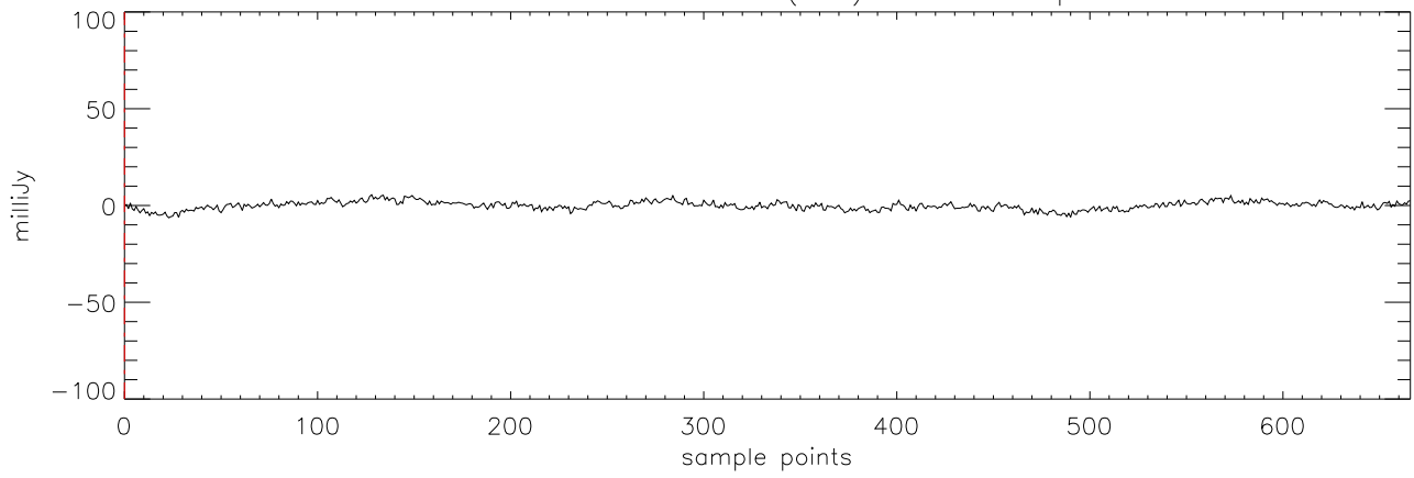
a2471 HD50554 18dec10 (AST) StokesI freq:5176.
