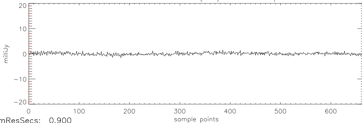
a2471 HD50554 18dec10 (AST) StokesU freq:5034.
