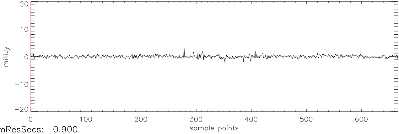
a2471 HD50554 18dec10 (AST) StokesV freq:4466.
