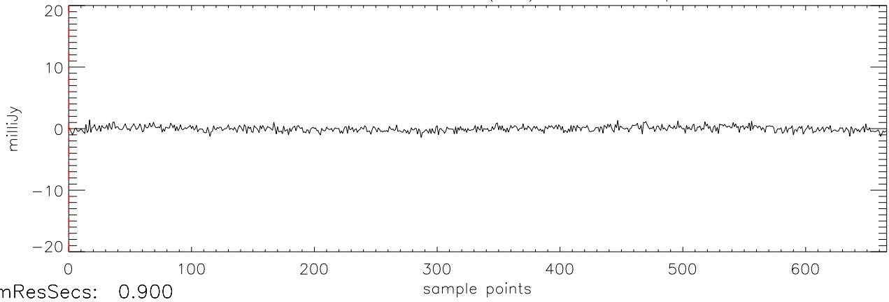
a2471 HD50554 18dec10 (AST) StokesV freq:5034.
