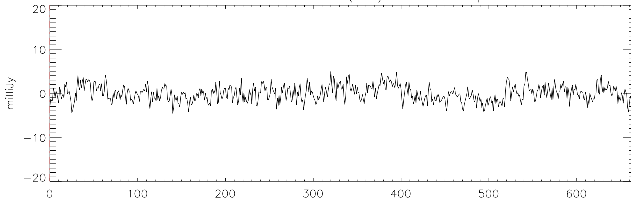
a2471 HD50554 18dec10 (AST) StokesQ freq:5176.
