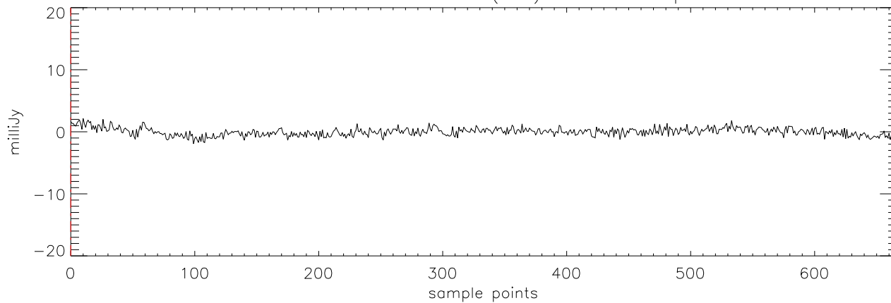
a2471 HD50554 18dec10 (AST) StokesU freq:5176.
