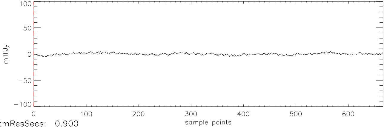
a2471 HD50554 18dec10 (AST) StokesI freq:5034.
