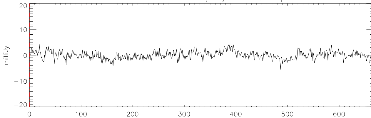
a2471 HD50554 18dec10 (AST) StokesQ freq:4892.
