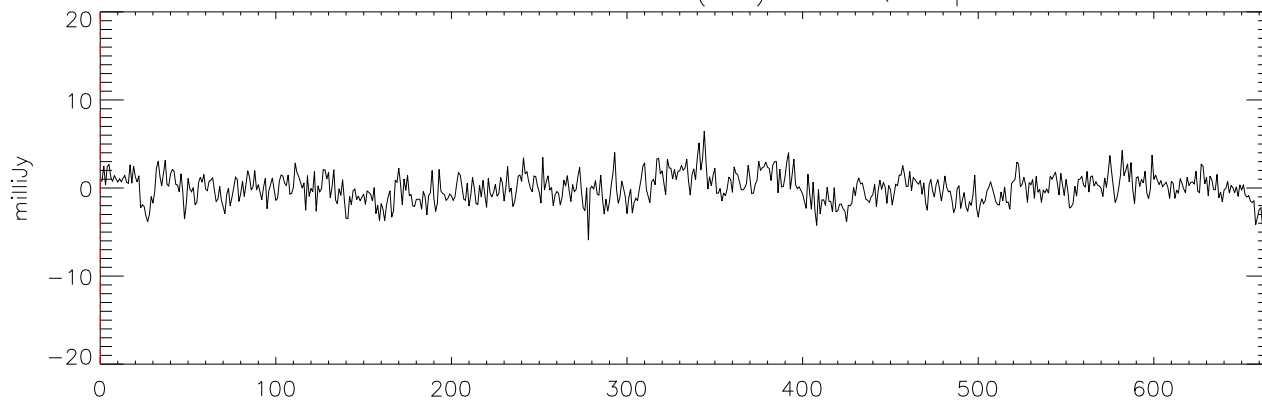
a2471 HD50554 18dec10 (AST) StokesQ freq:4325.
