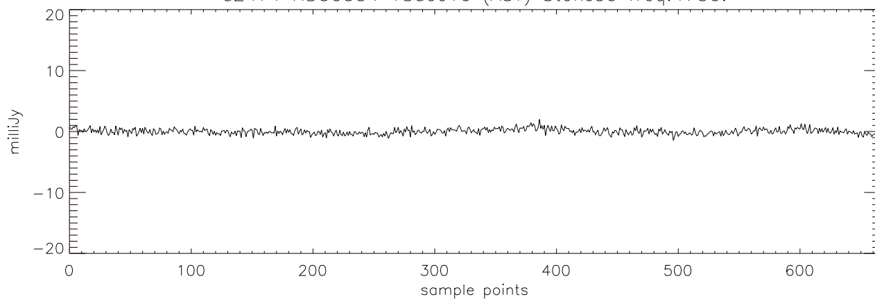
a2471 HD50554 18dec10 (AST) StokesU freq:4750.
