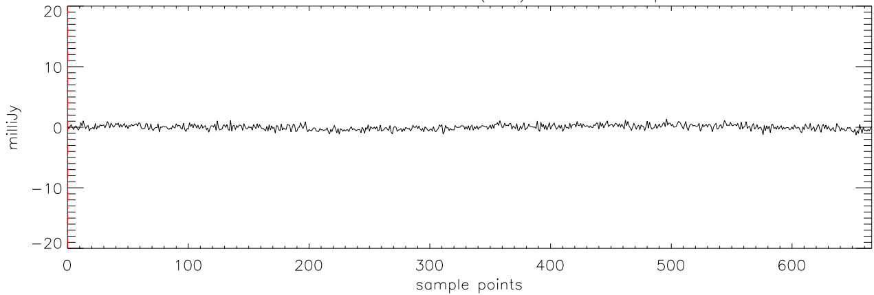
a2471 HD50554 18dec10 (AST) StokesV freq:4750.
