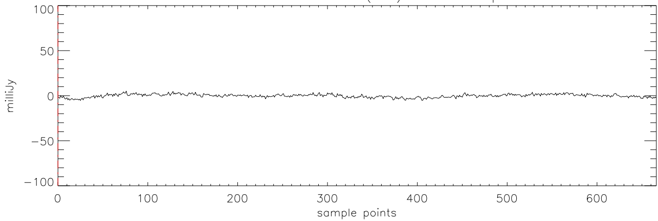
a2471 HD50554 18dec10 (AST) StokesI freq:4608.
