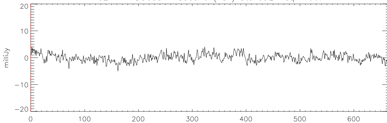
a2471 HD50554 18dec10 (AST) StokesQ freq:4466.
