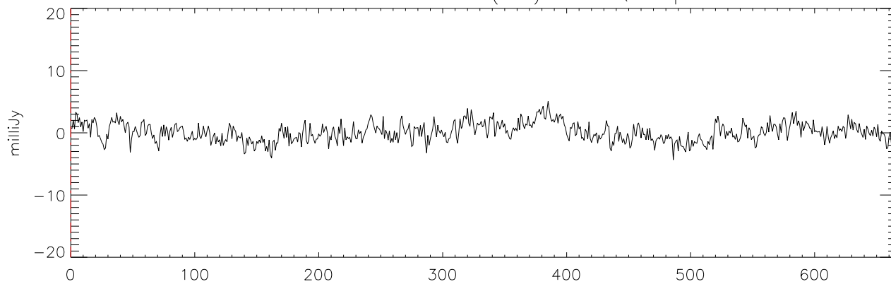
a2471 HD50554 18dec10 (AST) StokesQ freq:4750.
