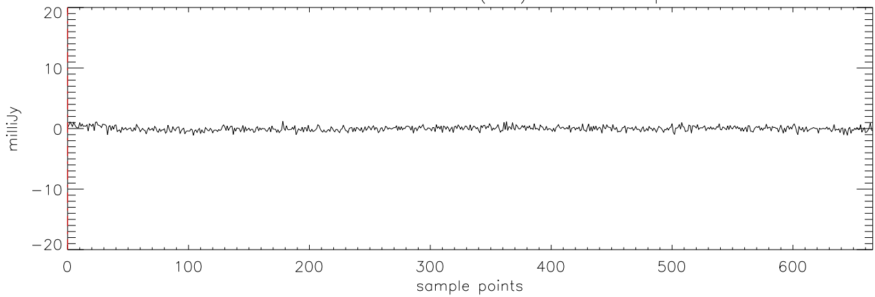
a2471 HD50554 18dec10 (AST) StokesV freq:4608.
