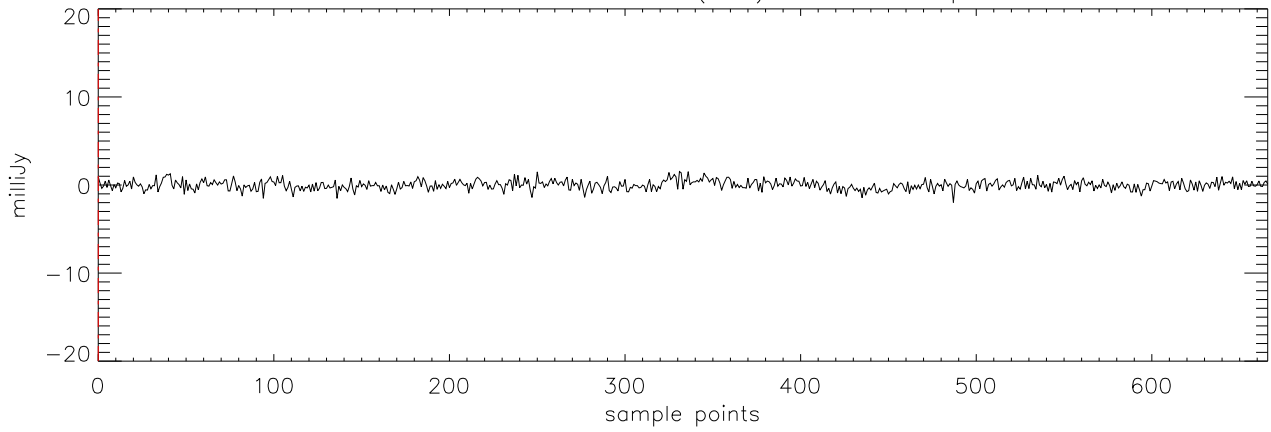
a2471 HD50554 18dec10 (AST) StokesV freq:5176.
