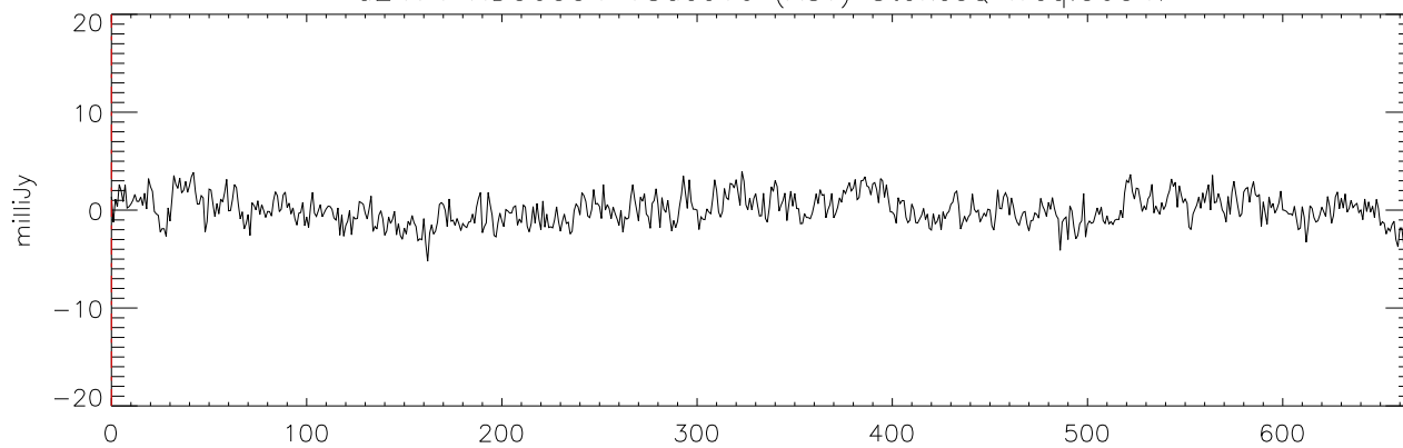
a2471 HD50554 18dec10 (AST) StokesQ freq:5034.
