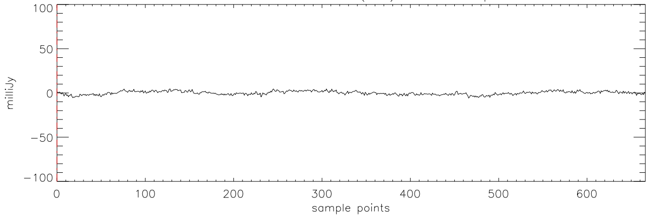
a2471 HD50554 18dec10 (AST) StokesI freq:4750.
