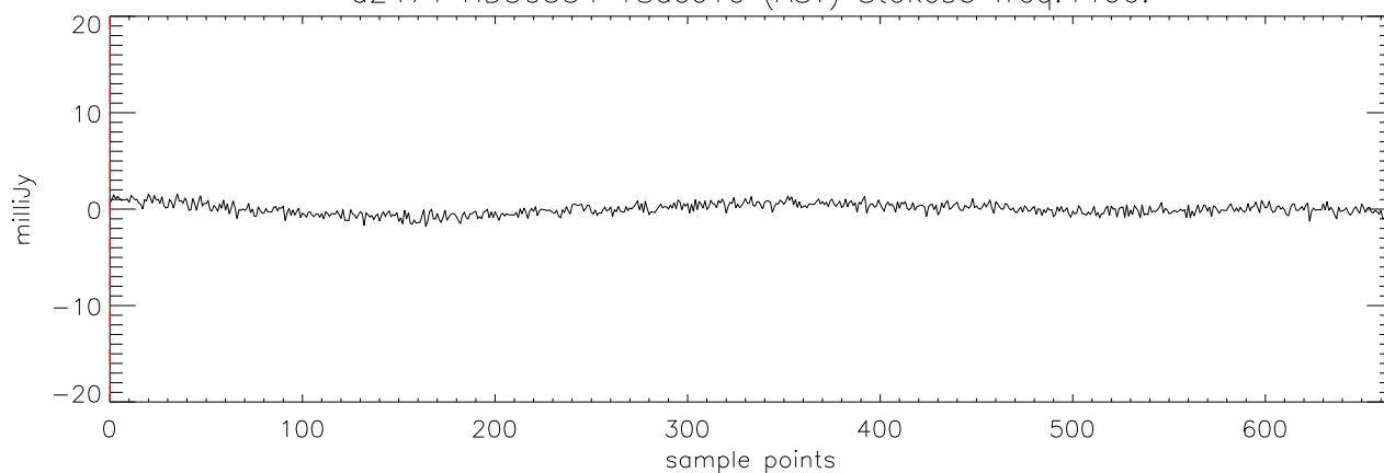
a2471 HD50554 18dec10 (AST) StokesU freq:4608.
