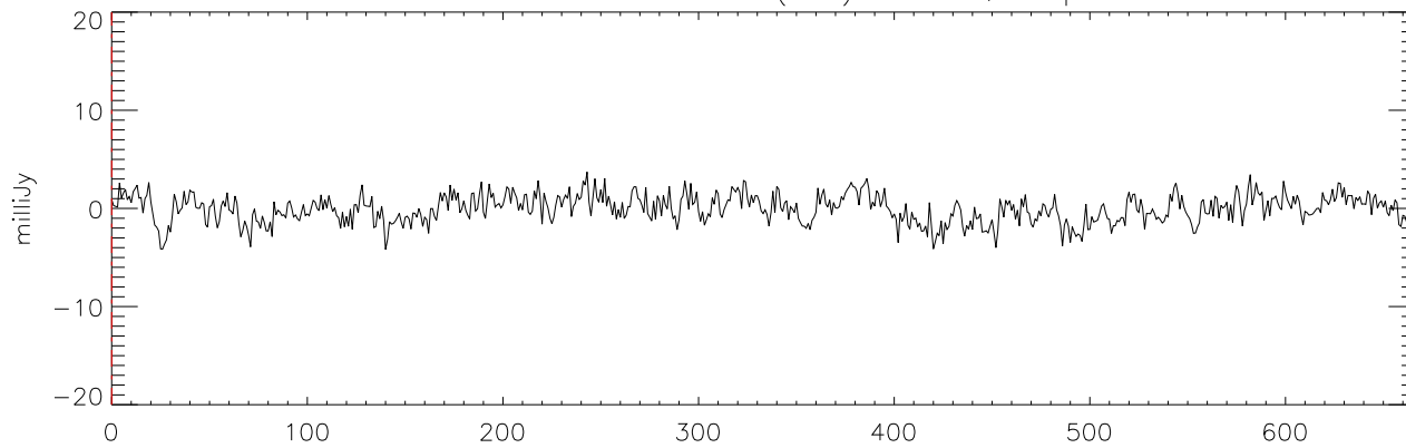
a2471 HD50554 18dec10 (AST) StokesQ freq:4608.
