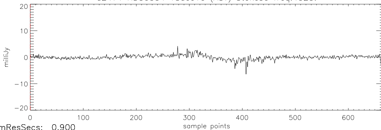
a2471 HD50554 18dec10 (AST) StokesU freq:4466.
