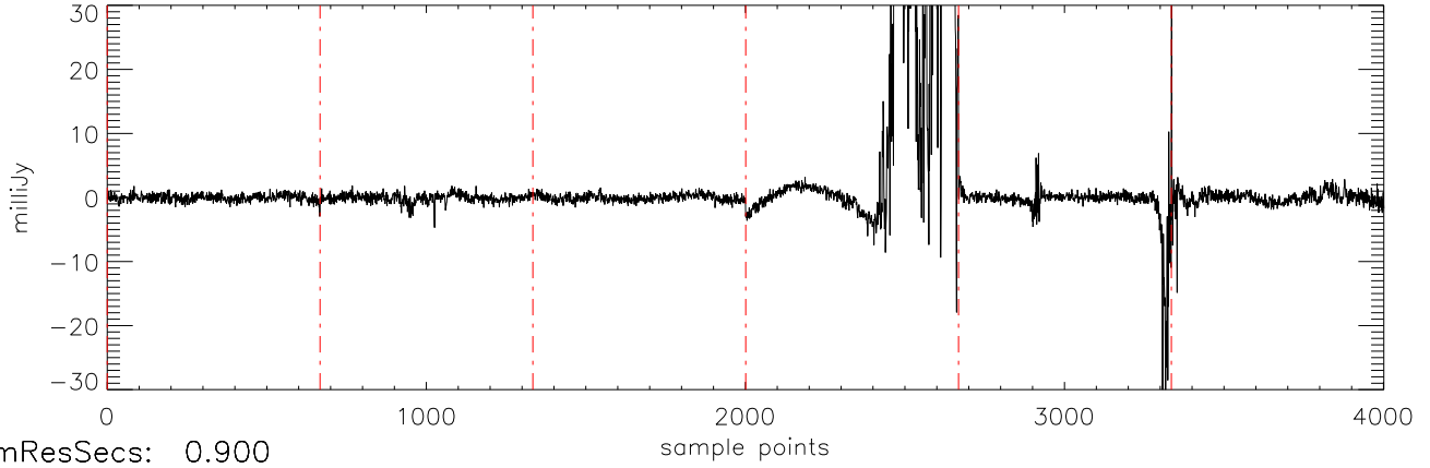
a2471 HD38529 08jan10 (AST) StokesV freq:4466.
