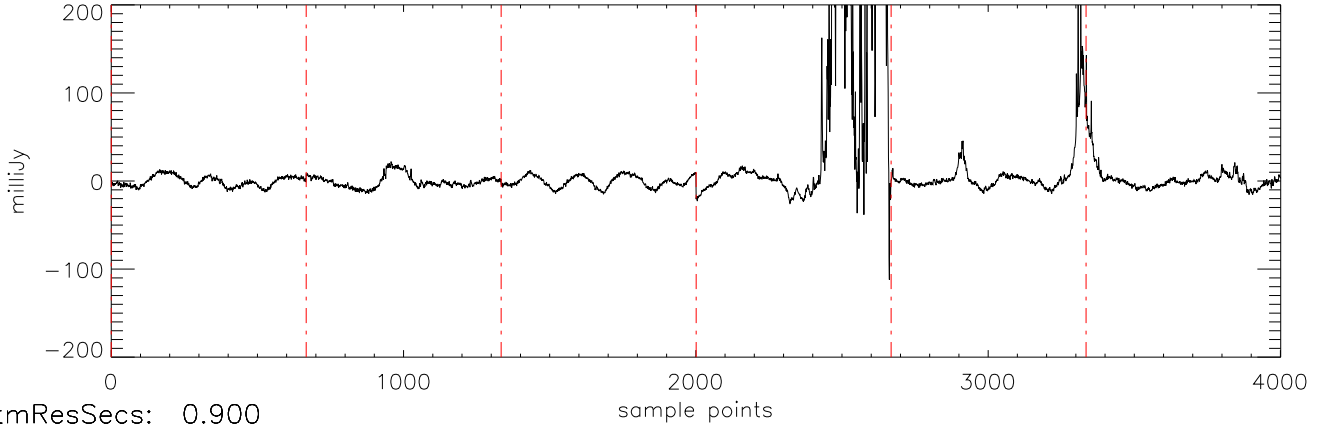
a2471 HD38529 08jan10 (AST) StokesI freq:4466.
