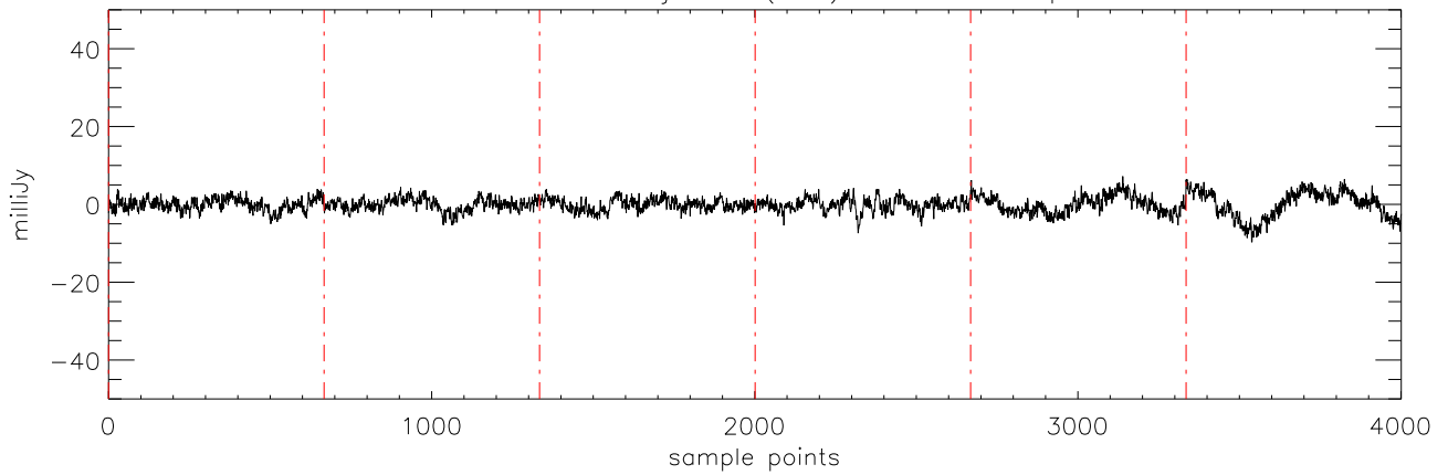
a2471 HD38529 08jan10 (AST) StokesQ freq:4608.
