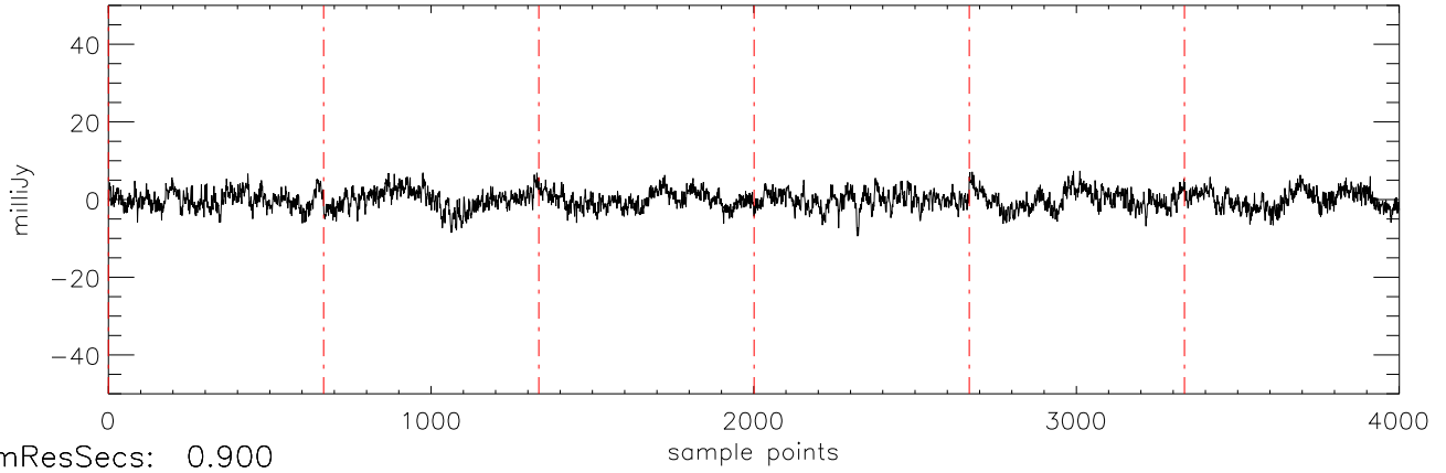
a2471 HD38529 08jan10 (AST) StokesQ freq:5034.
