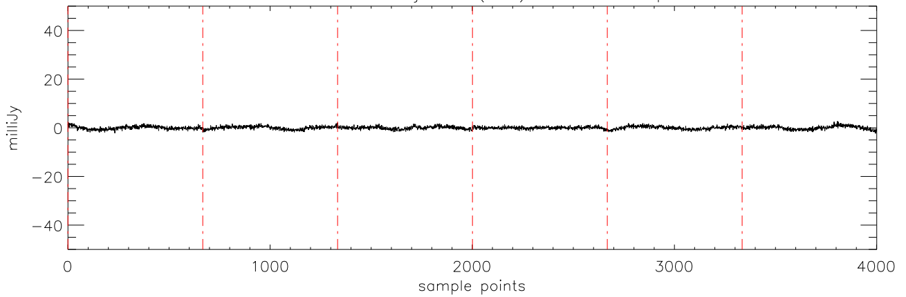
a2471 HD38529 08jan10 (AST) StokesU freq:4608.
