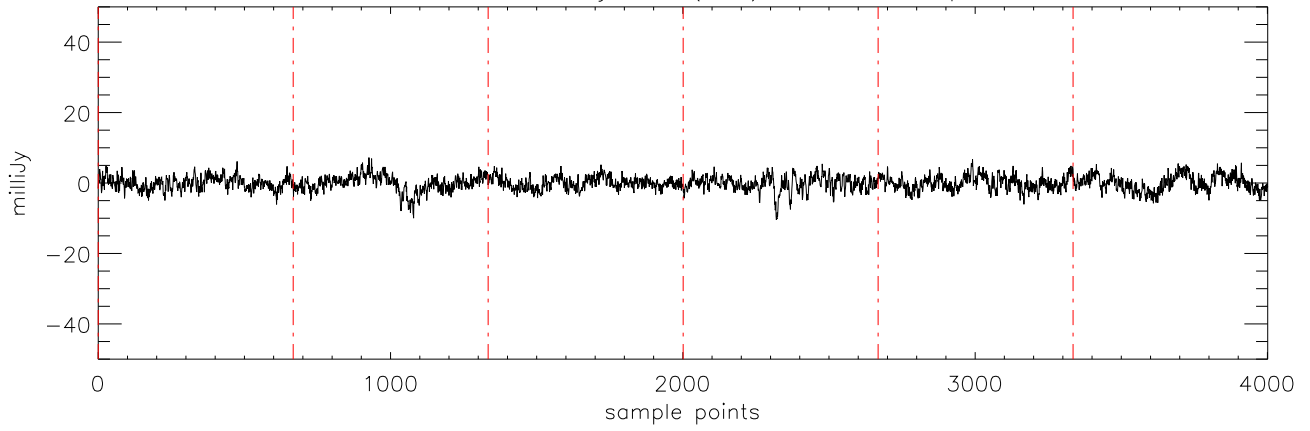
a2471 HD38529 08jan10 (AST) StokesQ freq:5176.
