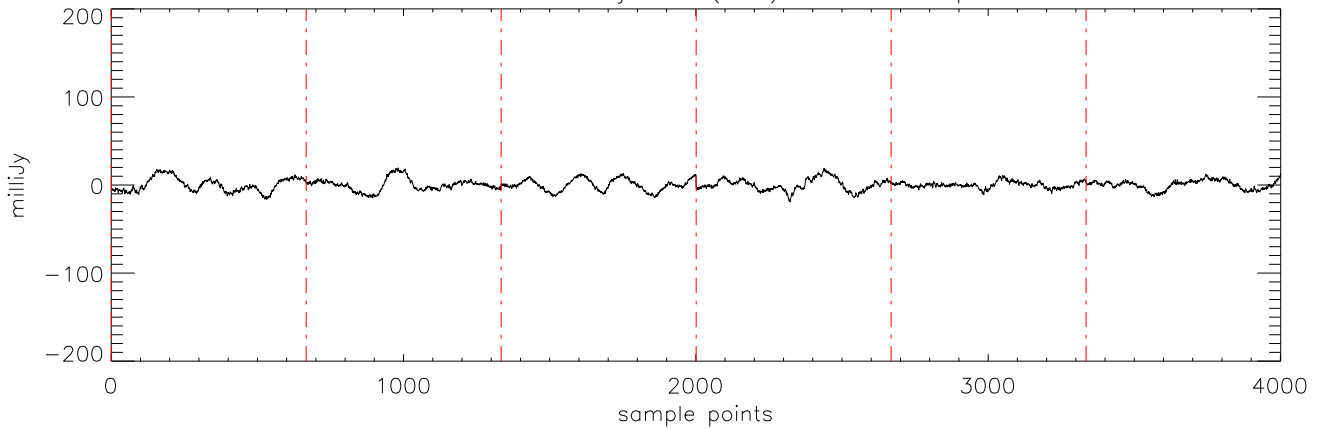
a2471 HD38529 08jan10 (AST) StokesI freq:4750.
