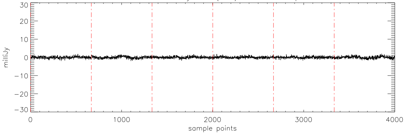
a2471 HD38529 08jan10 (AST) StokesV freq:4750.
