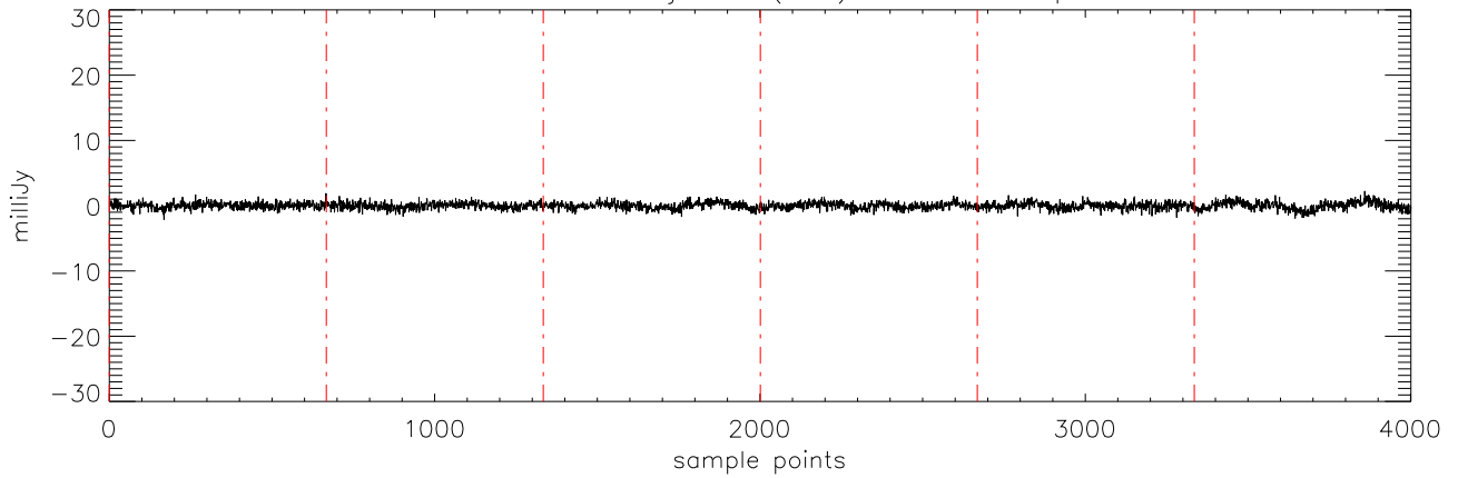
a2471 HD38529 08jan10 (AST) StokesV freq:4608.
