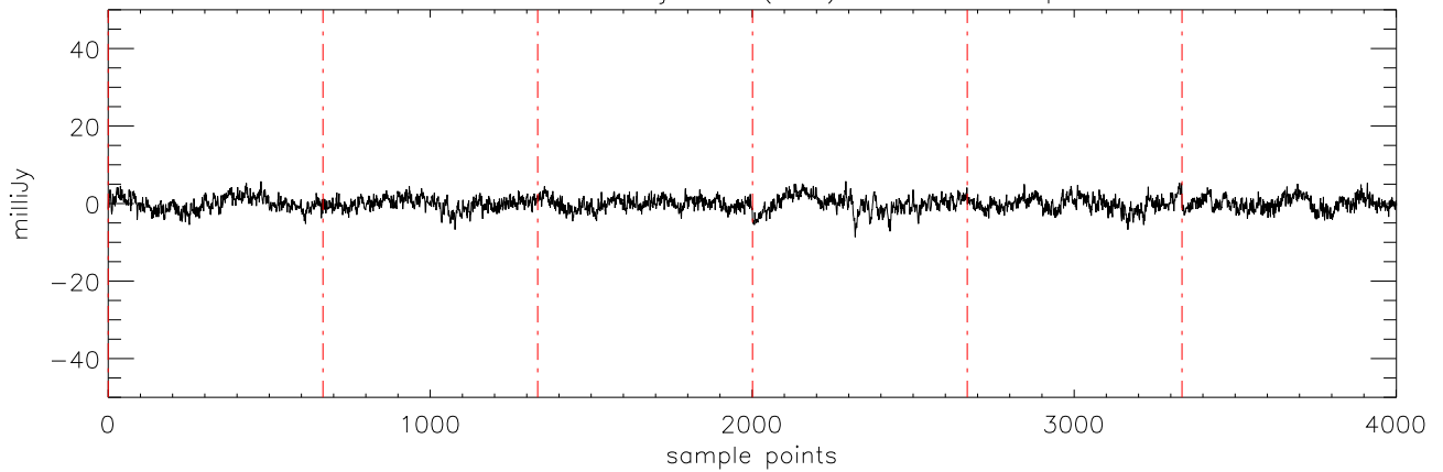
a2471 HD38529 08jan10 (AST) StokesQ freq:4750.
