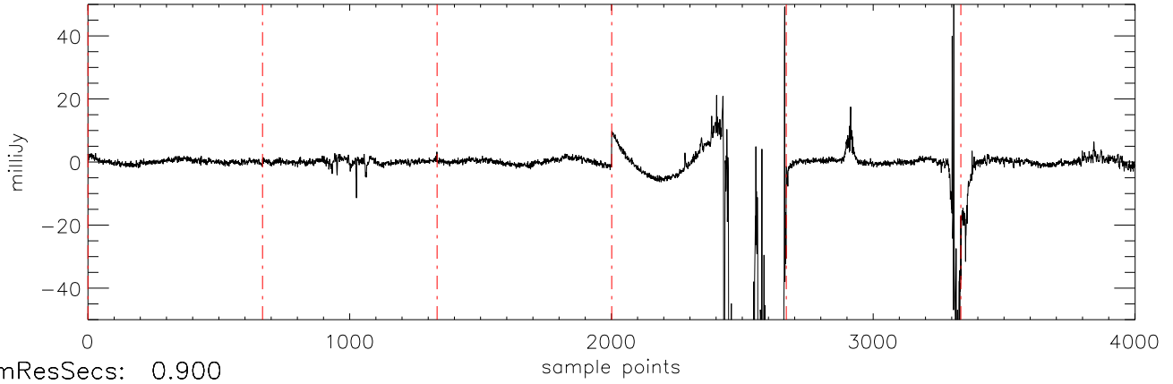
a2471 HD38529 08jan10 (AST) StokesU freq:4466.
