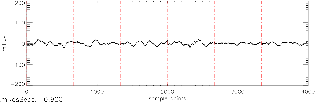
a2471 HD38529 08jan10 (AST) StokesI freq:5034.
