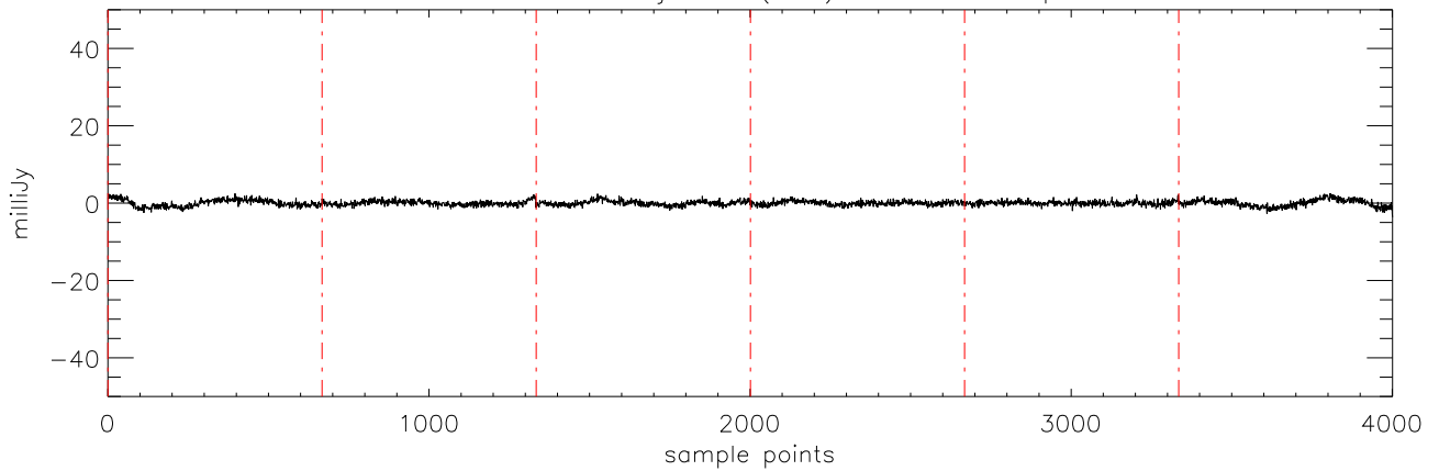
a2471 HD38529 08jan10 (AST) StokesU freq:4750.
