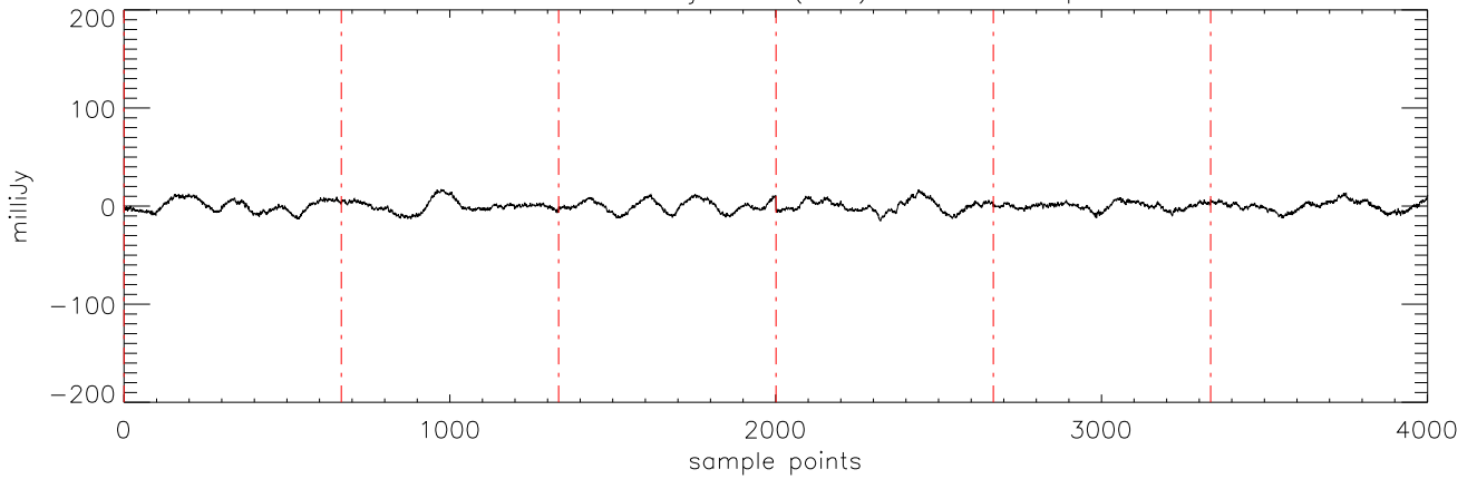
a2471 HD38529 08jan10 (AST) StokesI freq:4608.
