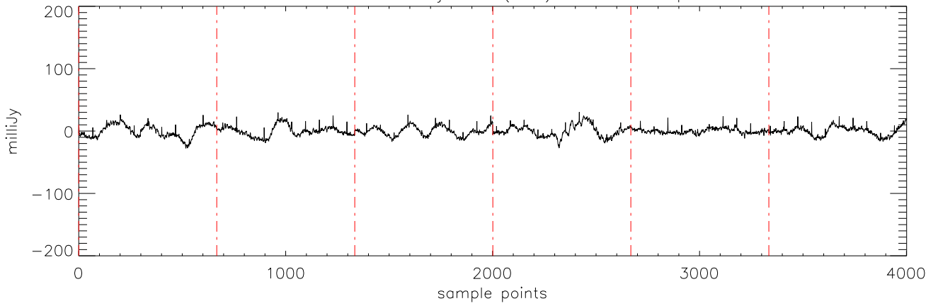
a2471 HD38529 08jan10 (AST) StokesI freq:5176.
