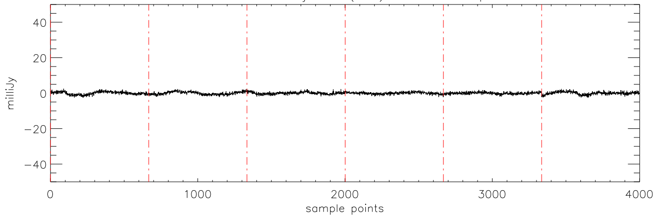
a2471 HD38529 08jan10 (AST) StokesU freq:5176.
