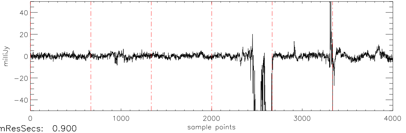
a2471 HD38529 08jan10 (AST) StokesQ freq:4466.
