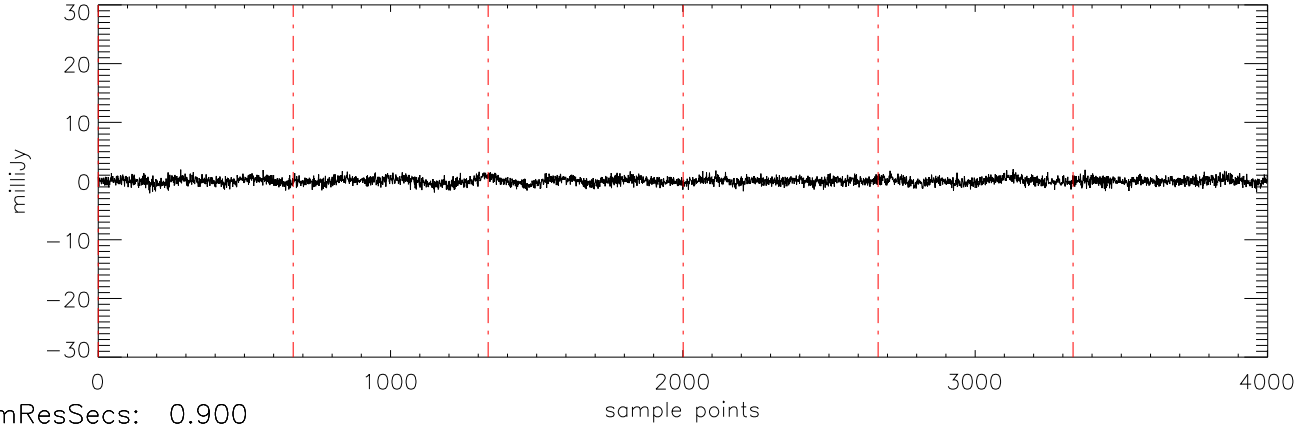
a2471 HD38529 08jan10 (AST) StokesV freq:5034.
