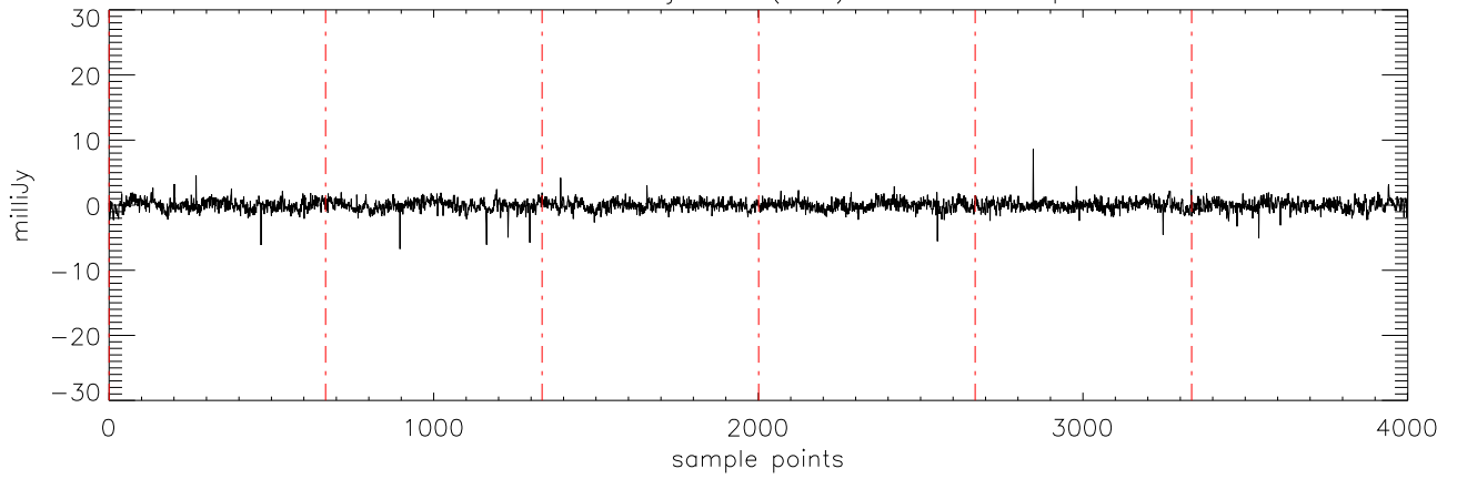
a2471 HD38529 08jan10 (AST) StokesV freq:5176.
