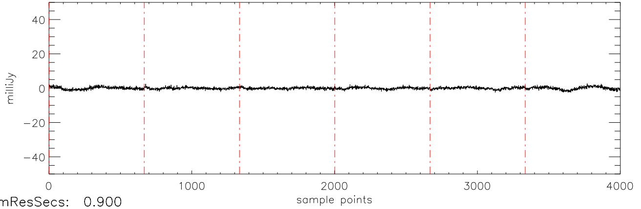
a2471 HD38529 08jan10 (AST) StokesU freq:5034.
