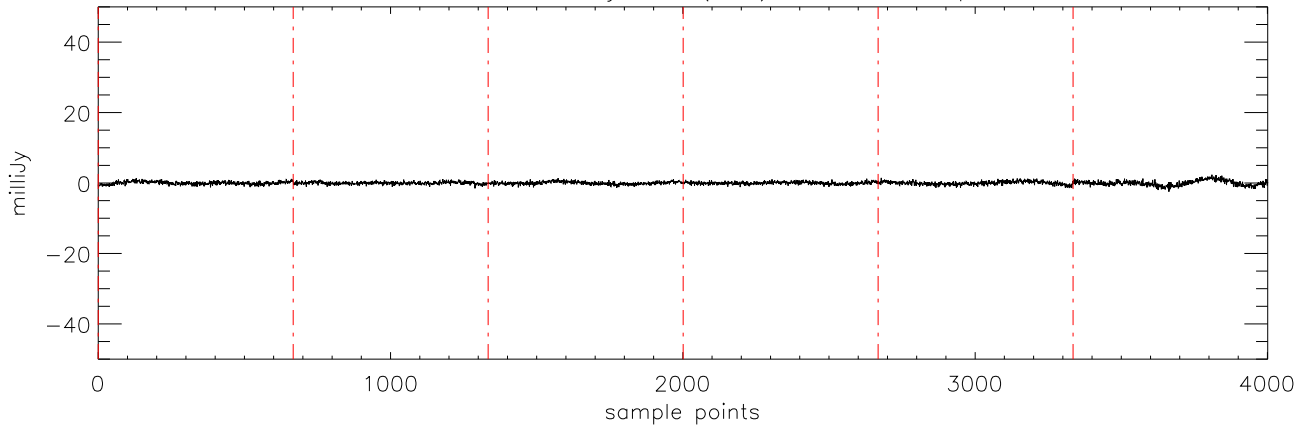
a2471 HD285968 09jan10 (AST) StokesU freq:4750.
