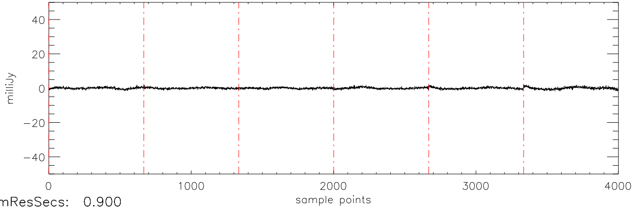
a2471 HD285968 09jan10 (AST) StokesU freq:5034.
