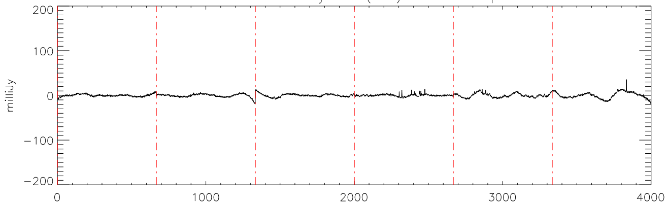
a2471 HD285968 09jan10 (AST) StokesI freq:4325.
