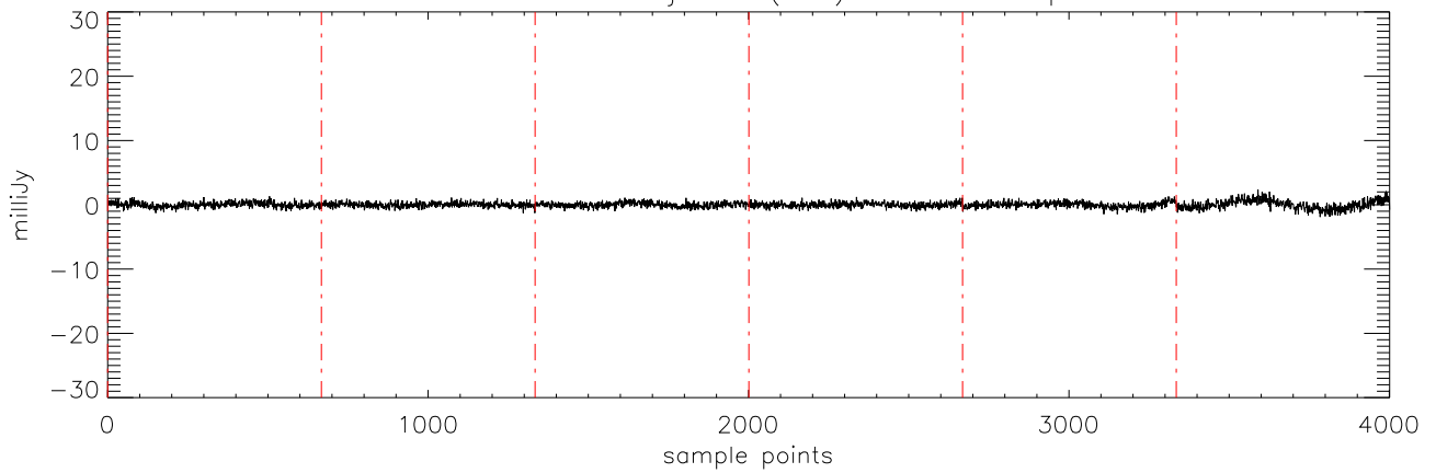
a2471 HD285968 09jan10 (AST) StokesV freq:4750.
