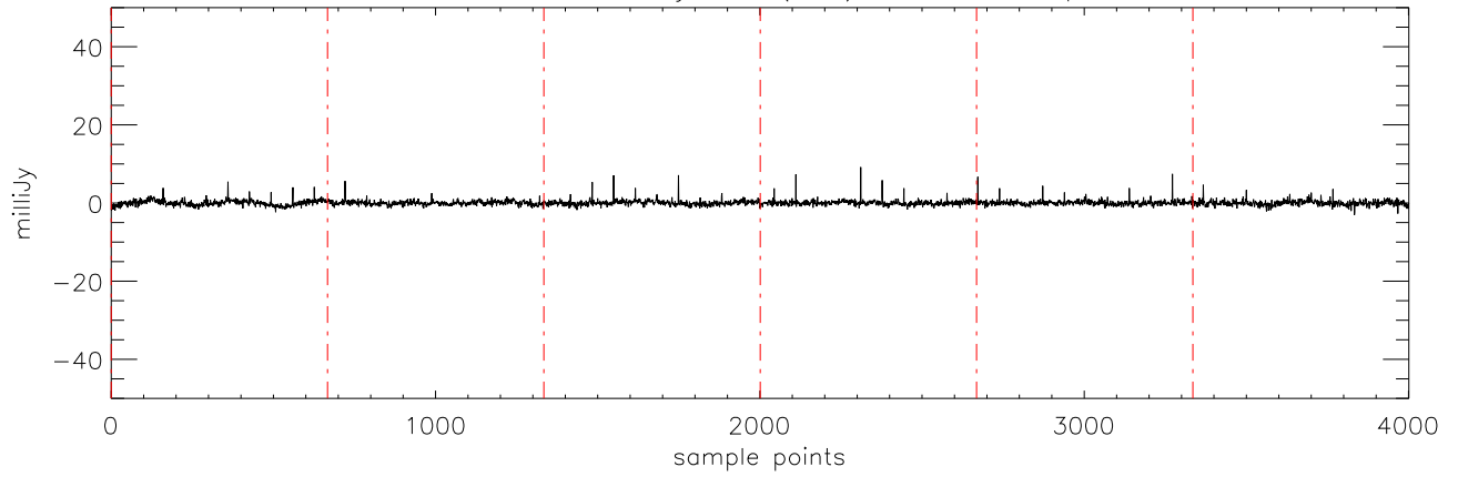
a2471 HD285968 09jan10 (AST) StokesU freq:5176.
