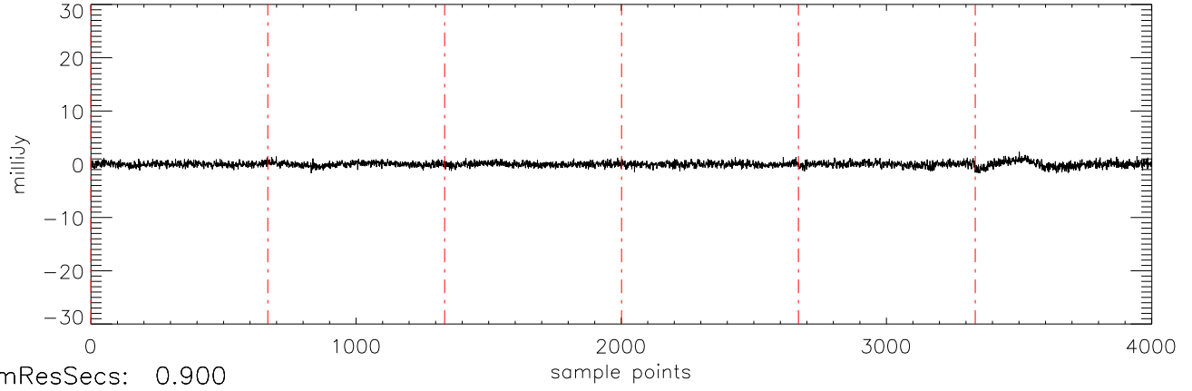
a2471 HD285968 09jan10 (AST) StokesV freq:5034.
