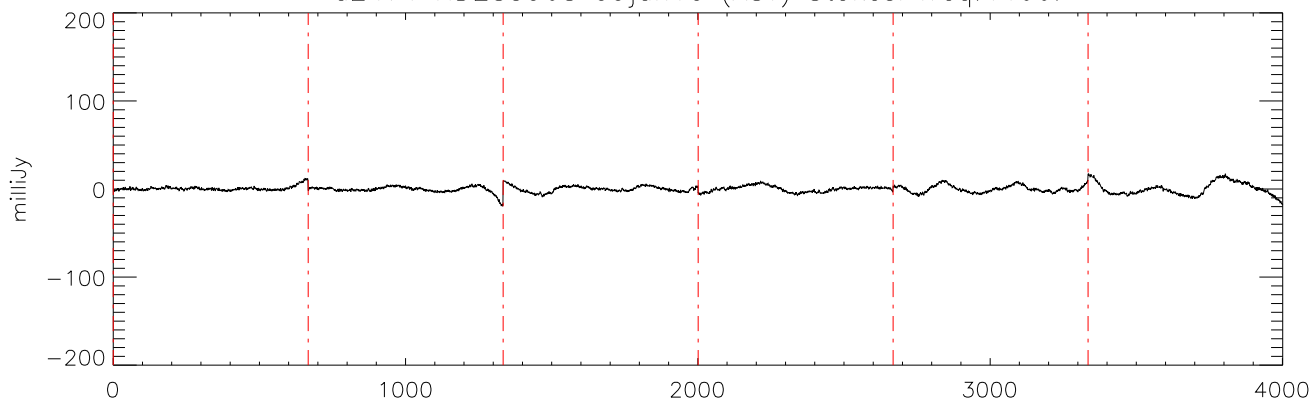
a2471 HD285968 09jan10 (AST) StokesI freq:4466.
