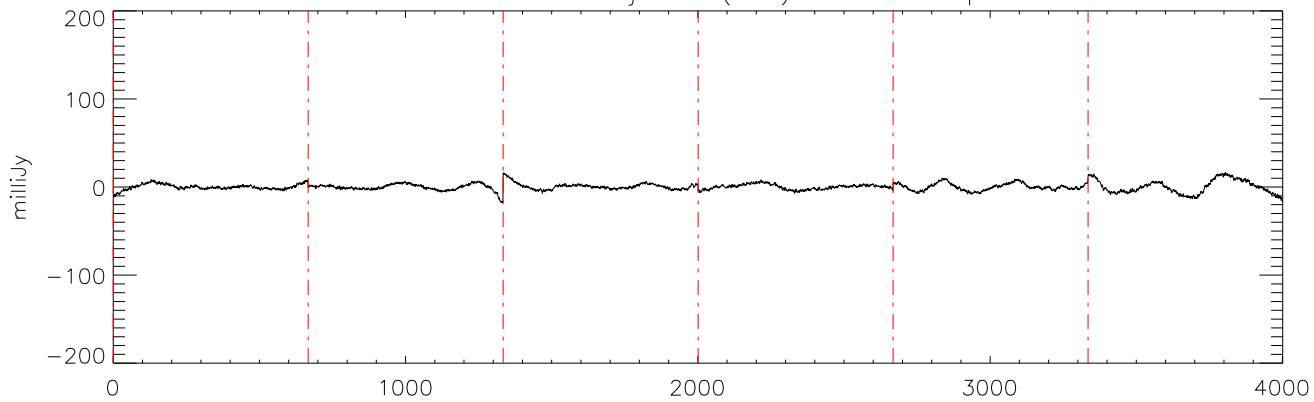
a2471 HD285968 09jan10 (AST) StokesI freq:4608.
