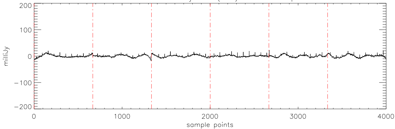
a2471 HD285968 09jan10 (AST) StokesI freq:5176.
