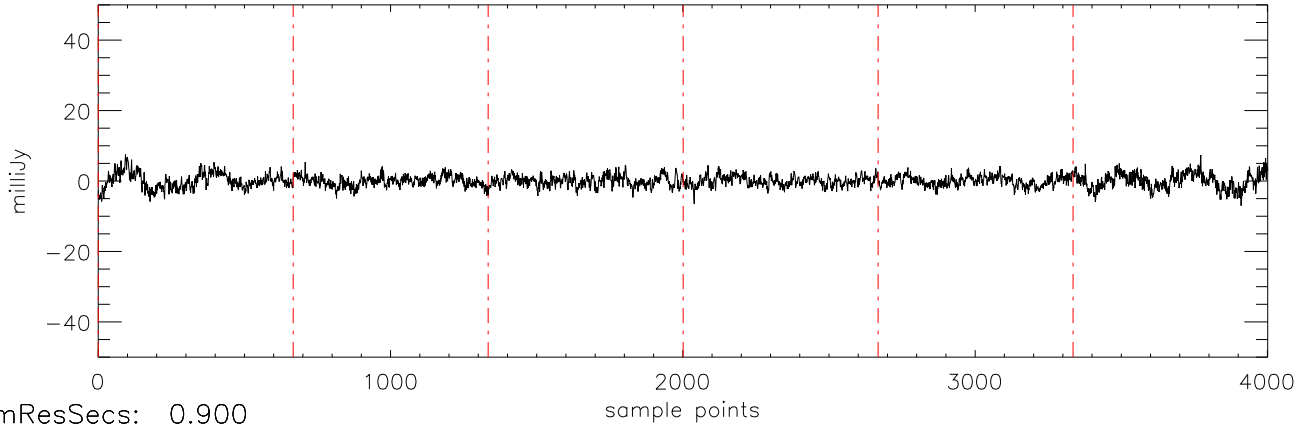
a2471 HD285968 09jan10 (AST) StokesQ freq:5034.
