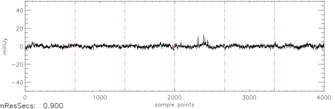
a2471 HD285968 09jan10 (AST) StokesQ freq:4466.
