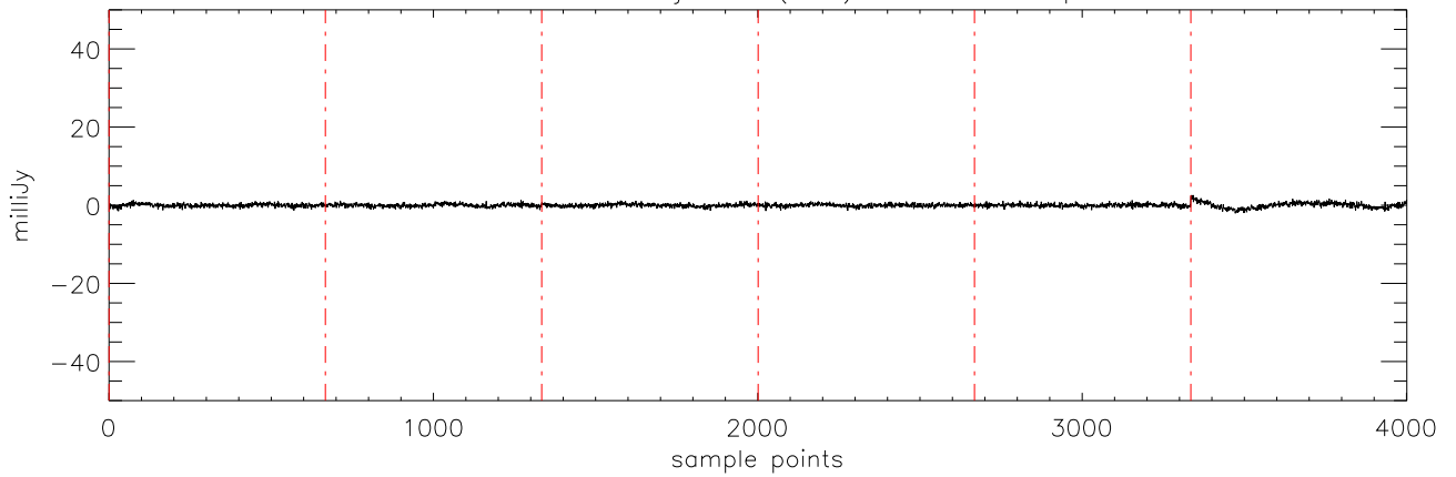
a2471 HD285968 09jan10 (AST) StokesU freq:4608.
