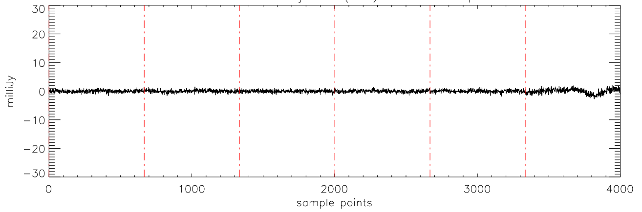
a2471 HD285968 09jan10 (AST) StokesV freq:5176.
