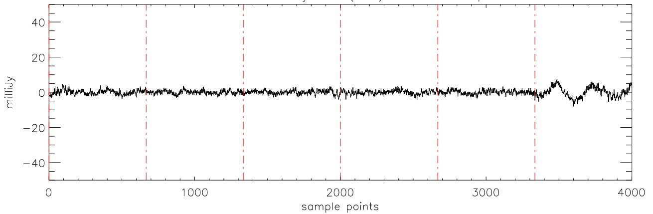
a2471 HD285968 09jan10 (AST) StokesQ freq:4750.
