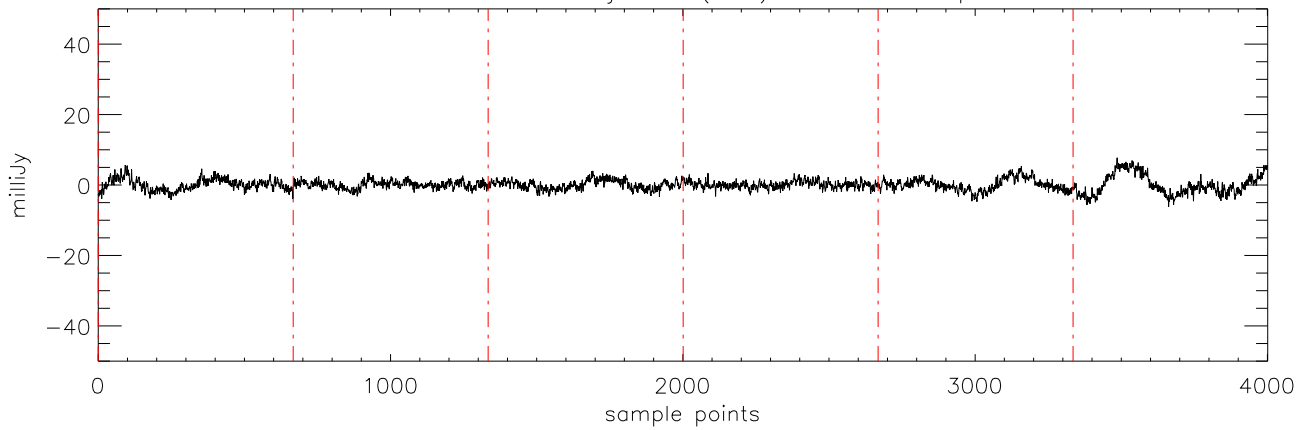
a2471 HD285968 09jan10 (AST) StokesQ freq:4608.
