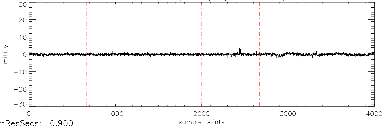
a2471 HD285968 09jan10 (AST) StokesV freq:4466.
