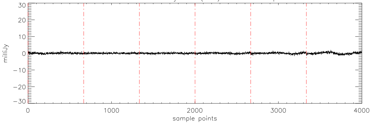
a2471 HD285968 09jan10 (AST) StokesV freq:4608.
