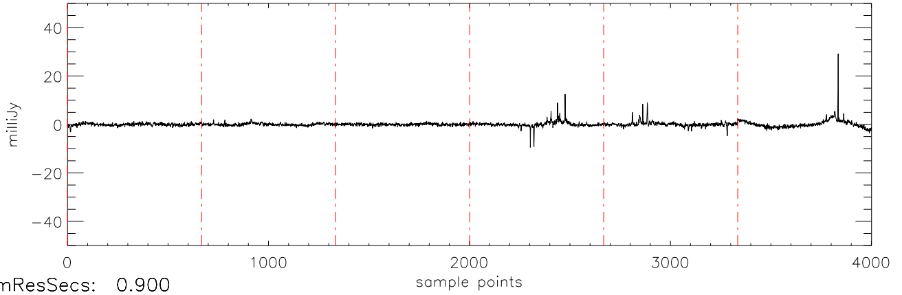
a2471 HD285968 09jan10 (AST) StokesU freq:4466.
