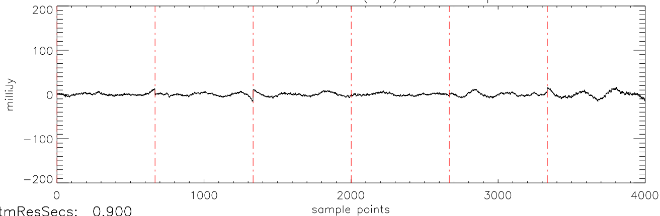
a2471 HD285968 09jan10 (AST) StokesI freq:5034.
