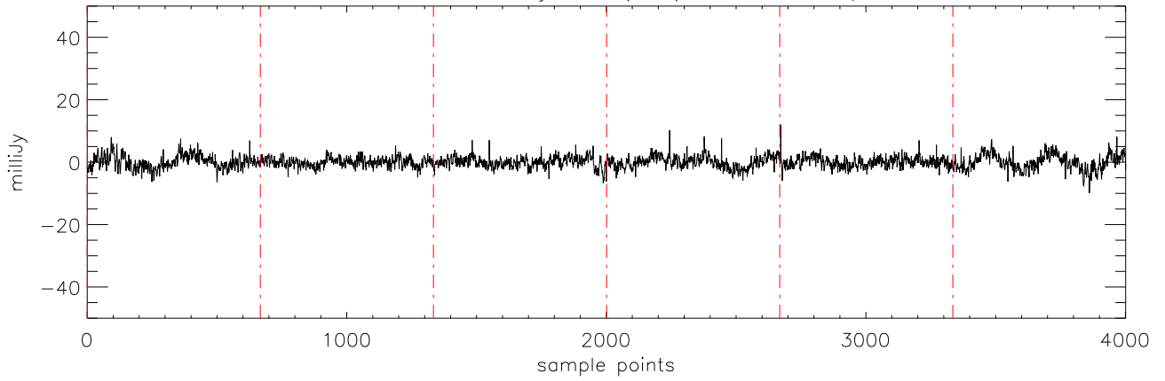
a2471 HD285968 09jan10 (AST) StokesQ freq:5176.
