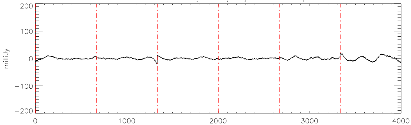
a2471 HD285968 09jan10 (AST) StokesI freq:4750.
