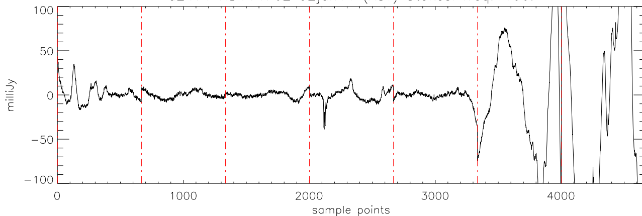
a2471 HD114762 02jan11 (AST) StokesI freq:4608.
