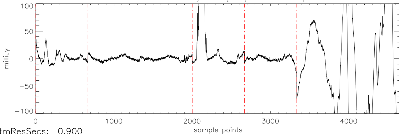
a2471 HD114762 02jan11 (AST) StokesI freq:4466.
