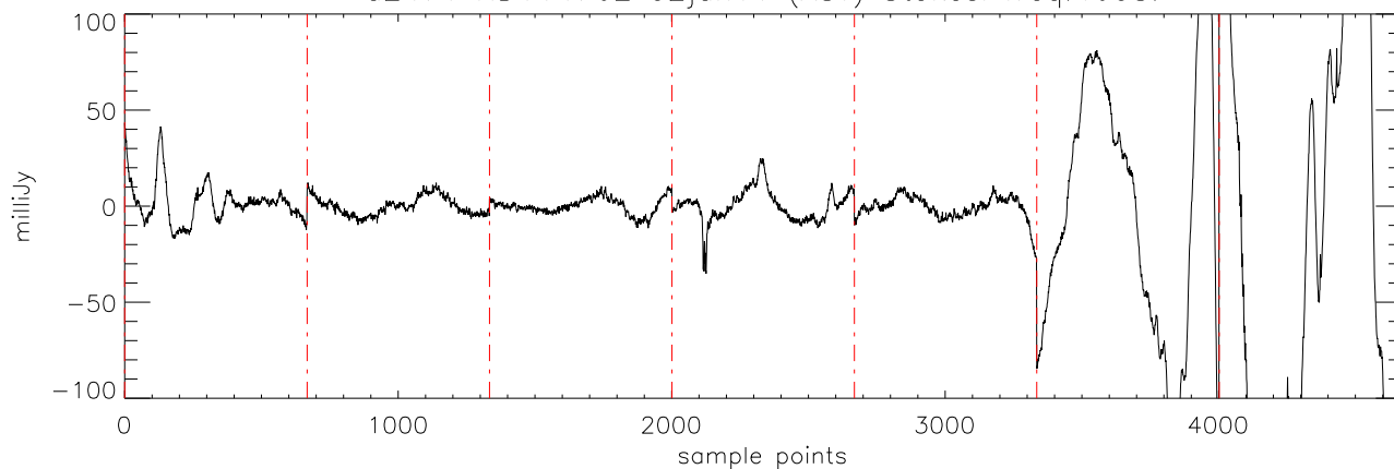
a2471 HD114762 02jan11 (AST) StokesI freq:4750.
