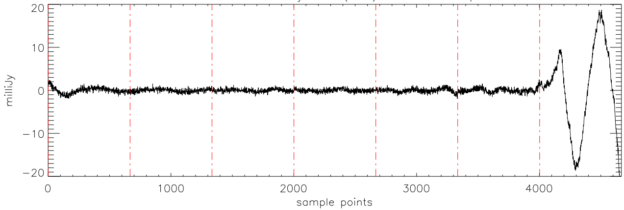
a2471 HD114762 02jan11 (AST) StokesU freq:4608.
