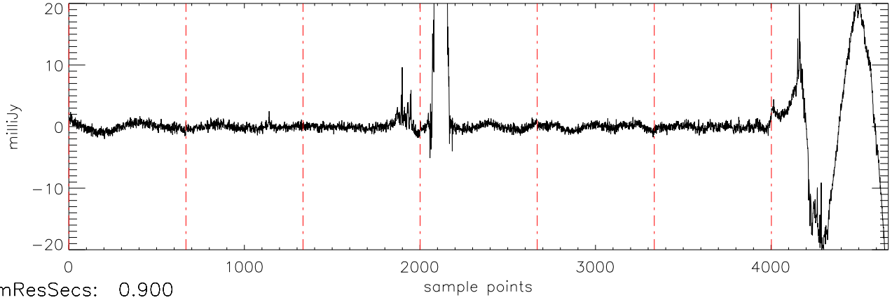
a2471 HD114762 02jan11 (AST) StokesU freq:4466.
