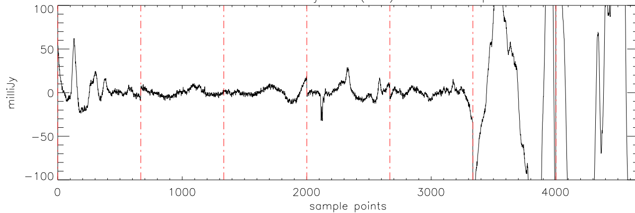
a2471 HD114762 02jan11 (AST) StokesI freq:5176.
