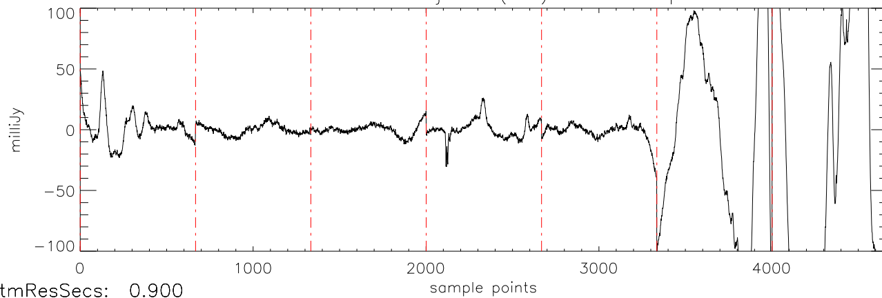
a2471 HD114762 02jan11 (AST) StokesI freq:5034.
