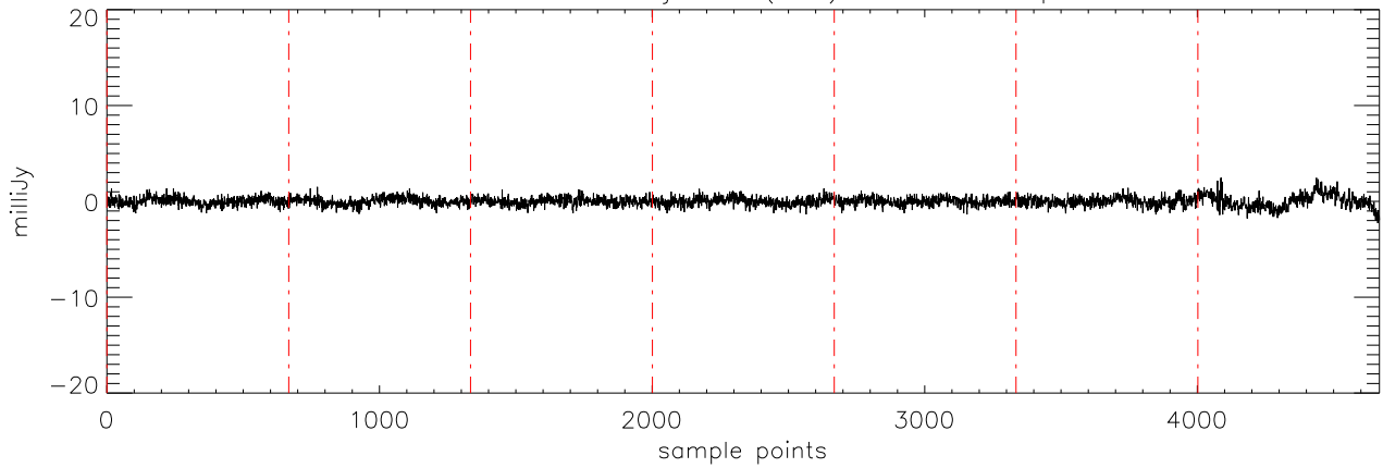
a2471 HD114762 02jan11 (AST) StokesV freq:4750.
