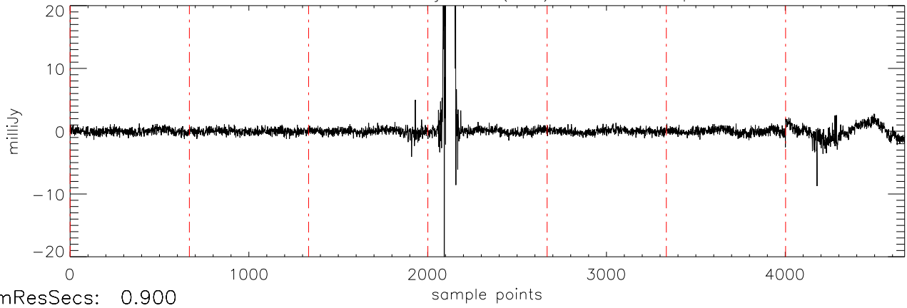
a2471 HD114762 02jan11 (AST) StokesV freq:4466.
