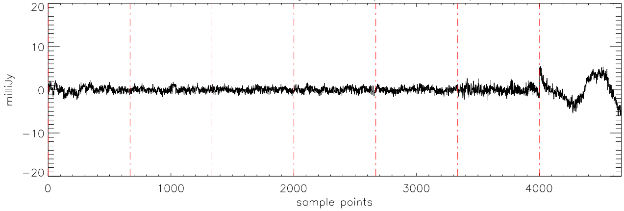
a2471 HD114762 02jan11 (AST) StokesV freq:5176.
