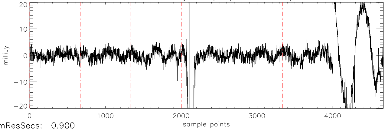
a2471 HD114762 02jan11 (AST) StokesQ freq:4466.
