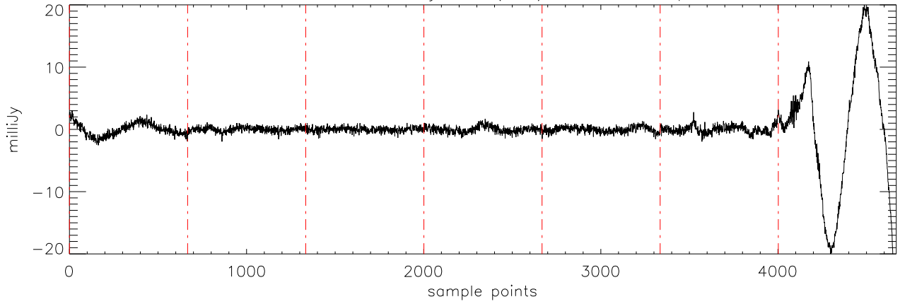
a2471 HD114762 02jan11 (AST) StokesU freq:4750.
