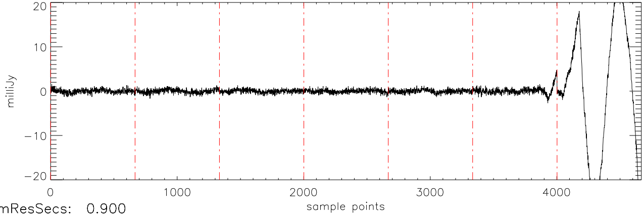
α2471 HD114762 02jan11 (AST) StokesU freq:5034.
