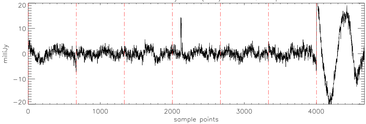
a2471 HD114762 02jan11 (AST) StokesQ freq:4608.
