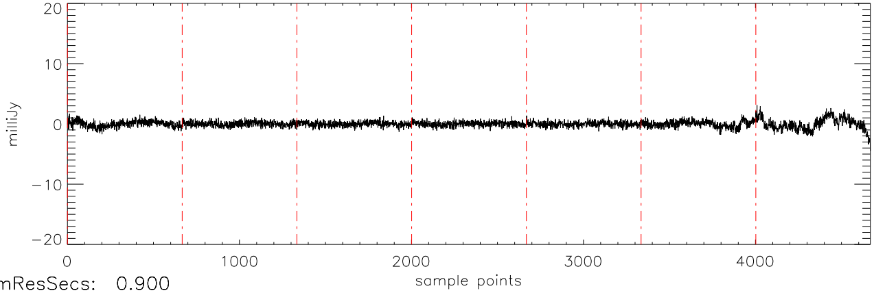
a2471 HD114762 02jan11 (AST) StokesV freq:5034.
