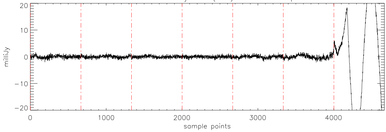
α2471 HD114762 02jan11 (AST) StokesU freq:5176.
