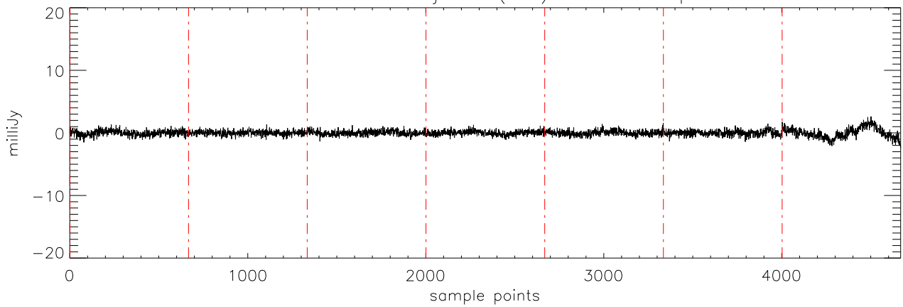
a2471 HD114762 02jan11 (AST) StokesV freq:4608.
