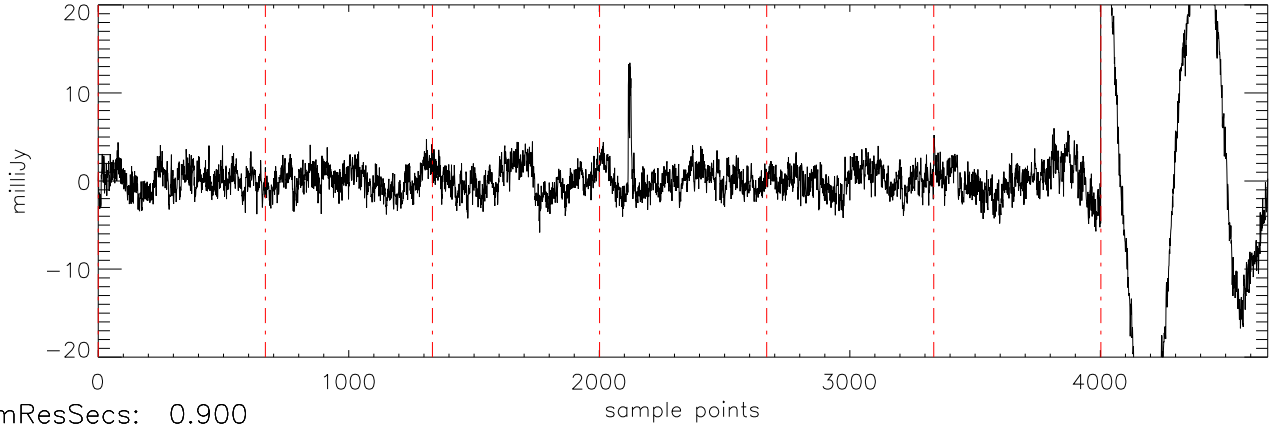
a2471 HD114762 02jan11 (AST) StokesQ freq:5034.
