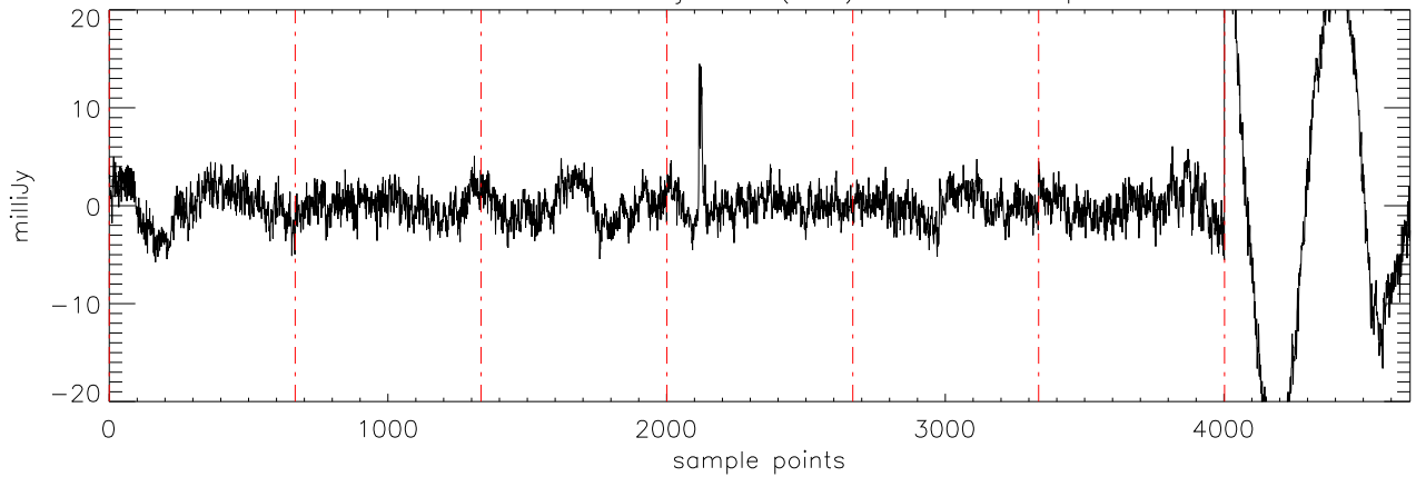
a2471 HD114762 02jan11 (AST) StokesQ freq:4750.
