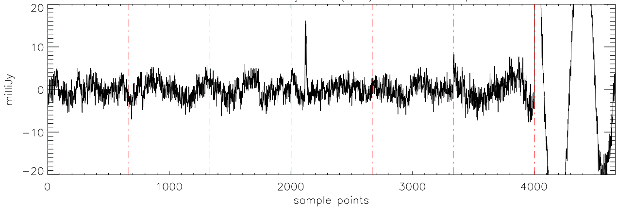
a2471 HD114762 02jan11 (AST) StokesQ freq:5176.
