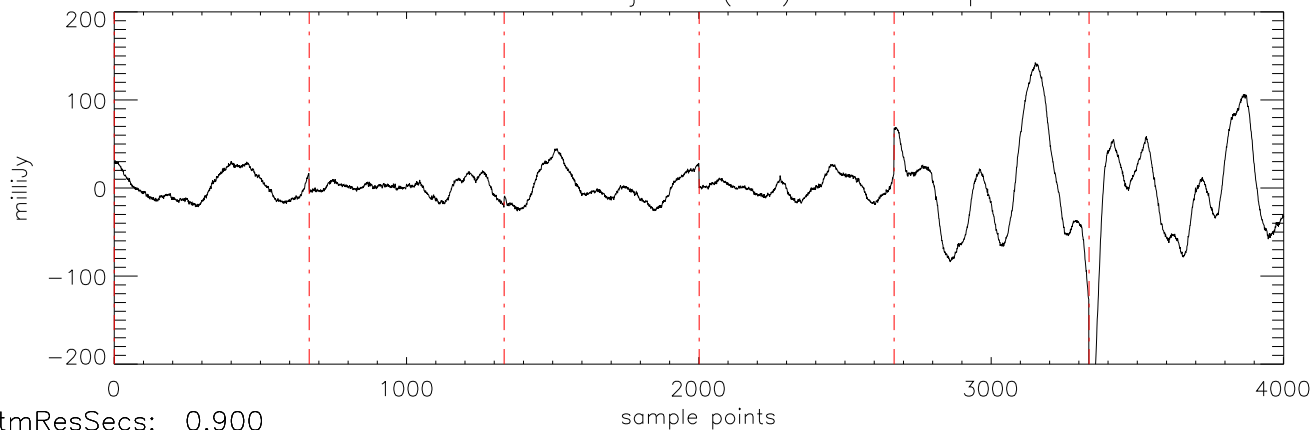
a2471 HD106252 07jan10 (AST) StokesI freq:5034.
