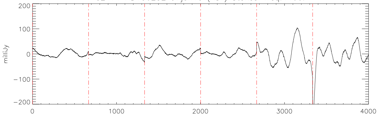
a2471 HD106252 07jan10 (AST) StokesI freq:4466.
