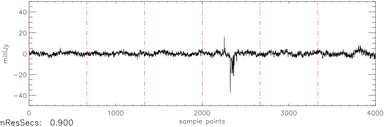
a2471 HD106252 07jan10 (AST) StokesQ freq:4466.
