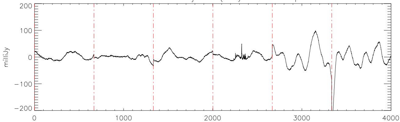
a2471 HD106252 07jan10 (AST) StokesI freq:4325.
