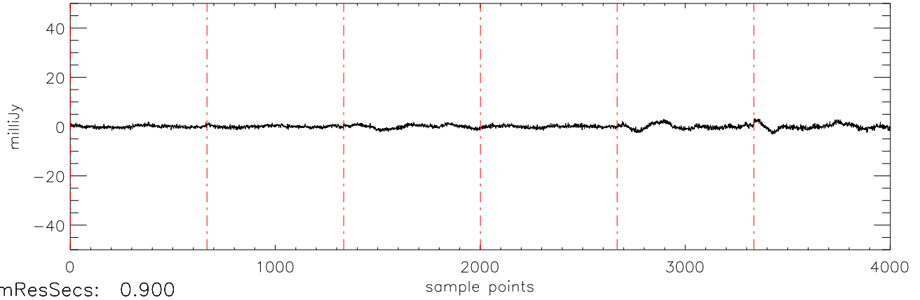
a2471 HD106252 07jan10 (AST) StokesU freq:5034.
