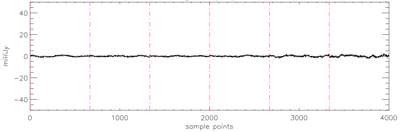
a2471 HD106252 07jan10 (AST) StokesU freq:4750.
