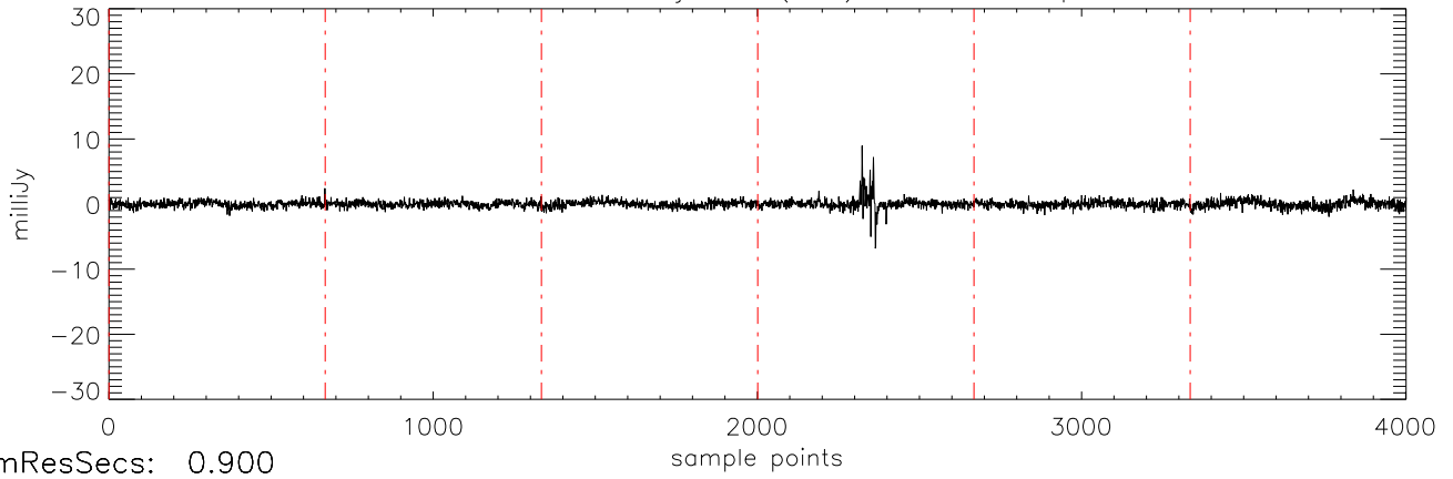
a2471 HD106252 07jan10 (AST) StokesV freq:4466.
