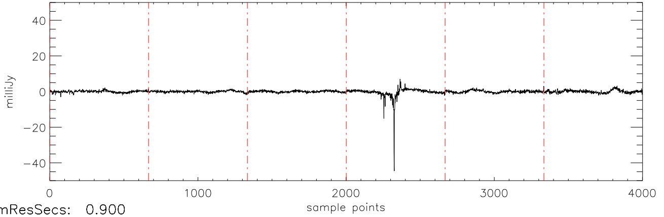
a2471 HD106252 07jan10 (AST) StokesU freq:4466.
