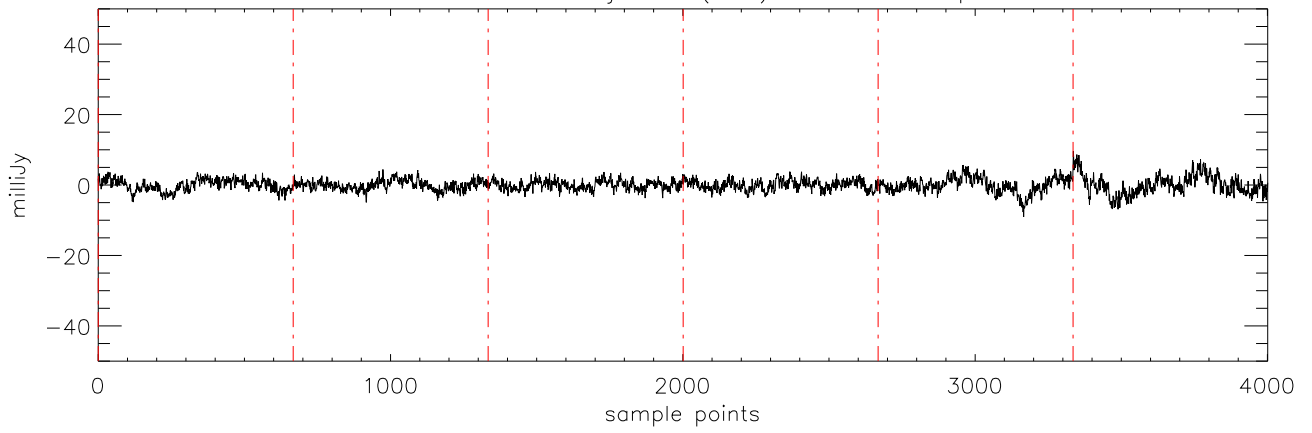
a2471 HD106252 07jan10 (AST) StokesQ freq:5176.
