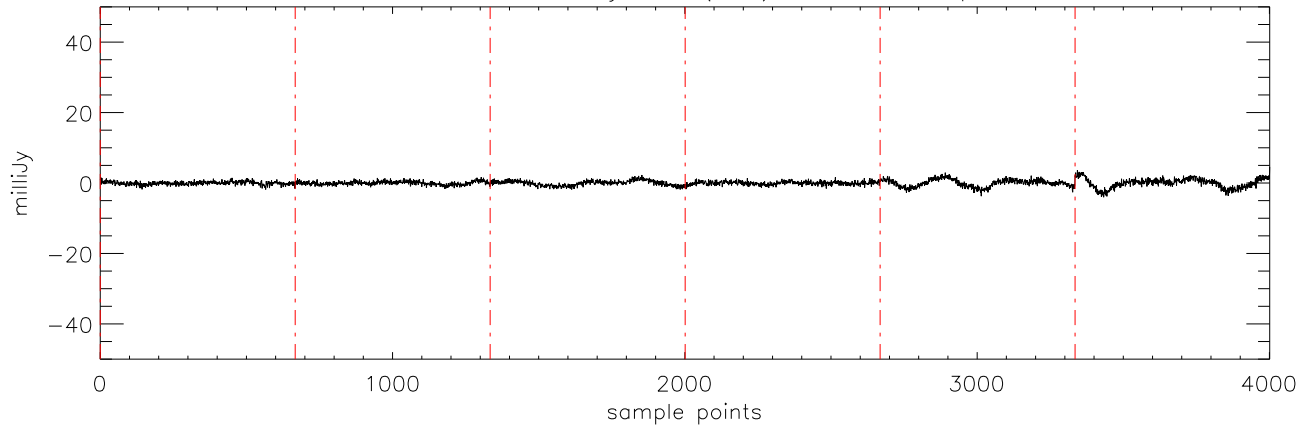
a2471 HD106252 07jan10 (AST) StokesU freq:5176.
