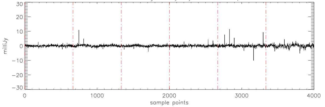
a2471 HD106252 07jan10 (AST) StokesV freq:5176.
