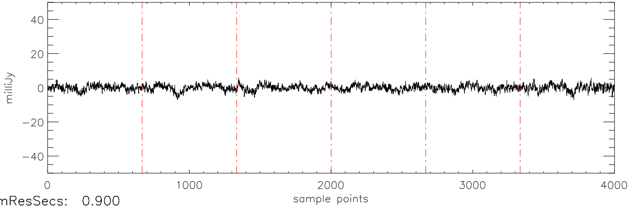
a2471 HD106252 07jan10 (AST) StokesQ freq:5034.
