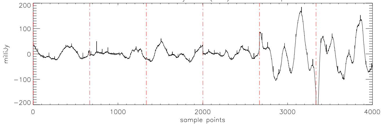
a2471 HD106252 07jan10 (AST) StokesI freq:5176.
