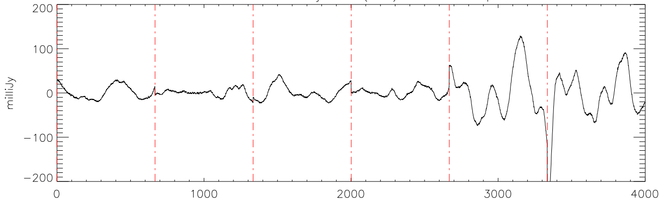
a2471 HD106252 07jan10 (AST) StokesI freq:4750.
