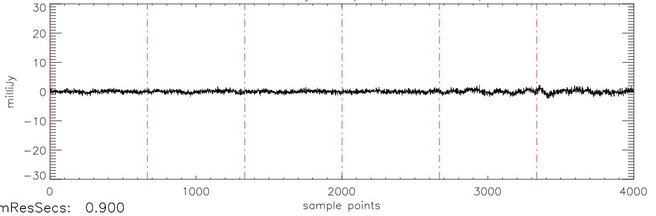
a2471 HD106252 07jan10 (AST) StokesV freq:5034.
