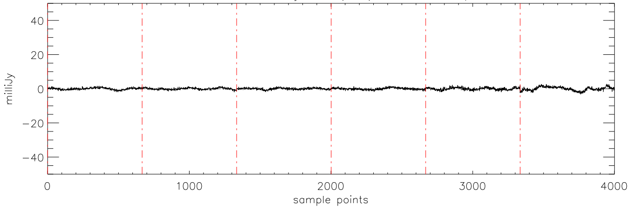
a2471 HD106252 07jan10 (AST) StokesU freq:4608.
