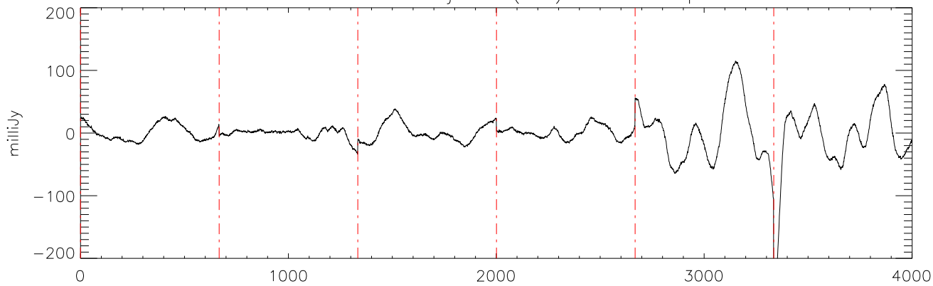
a2471 HD106252 07jan10 (AST) StokesI freq:4608.
