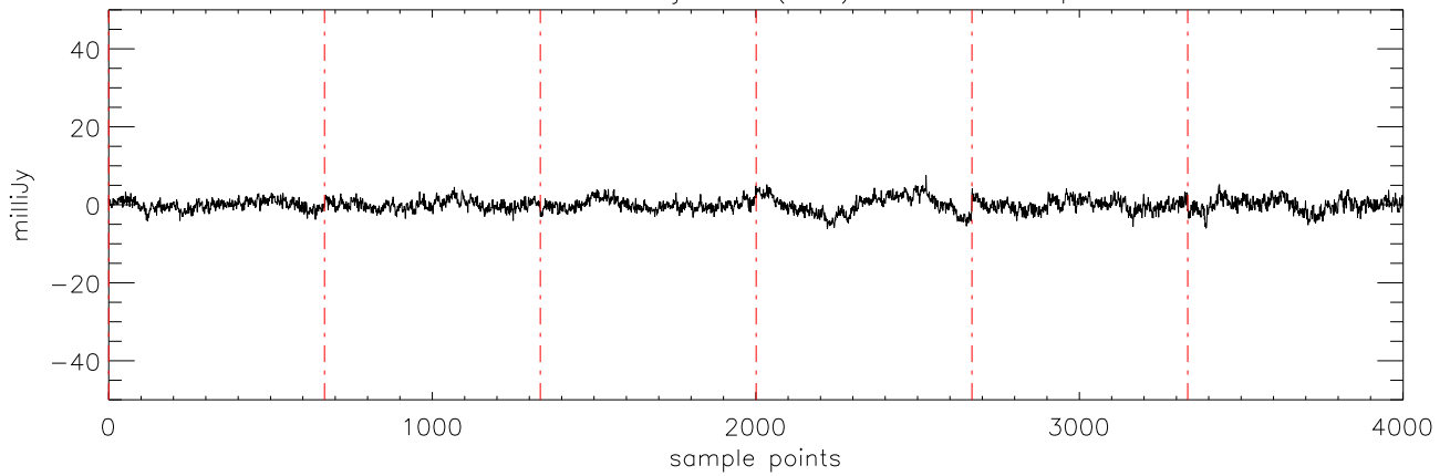
a2471 HD106252 07jan10 (AST) StokesQ freq:4608.
