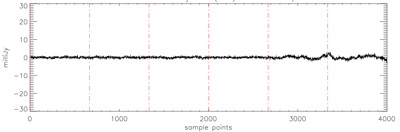
a2471 HD106252 07jan10 (AST) StokesV freq:4750.
