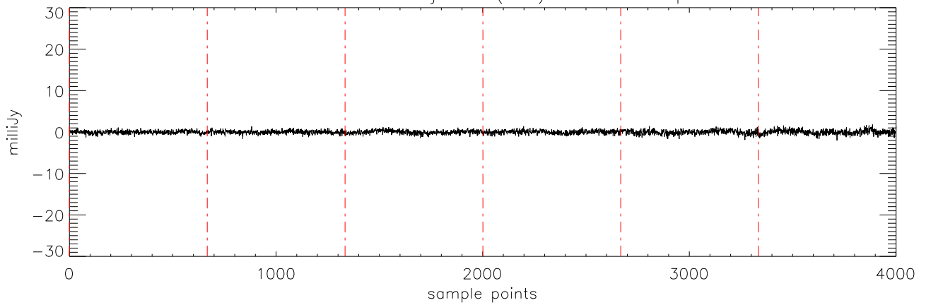
a2471 HD106252 07jan10 (AST) StokesV freq:4608.
