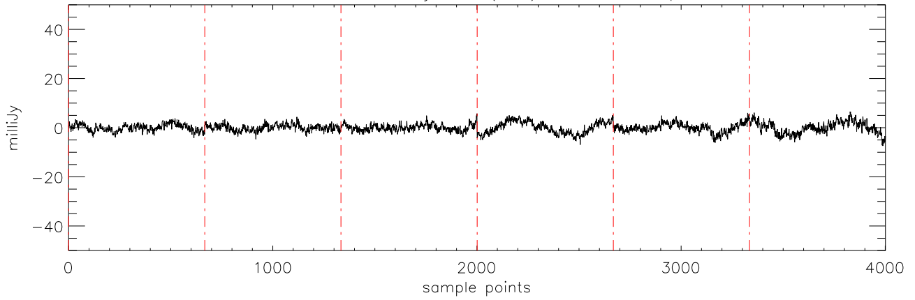
a2471 HD106252 07jan10 (AST) StokesQ freq:4750.
