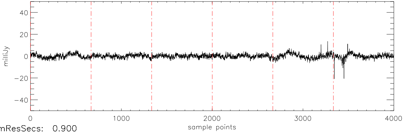
a2471 HD102195 07jan10 (AST) StokesQ freq:4466.
