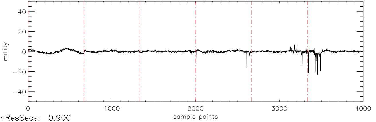
a2471 HD102195 07jan10 (AST) StokesU freq:4466.
