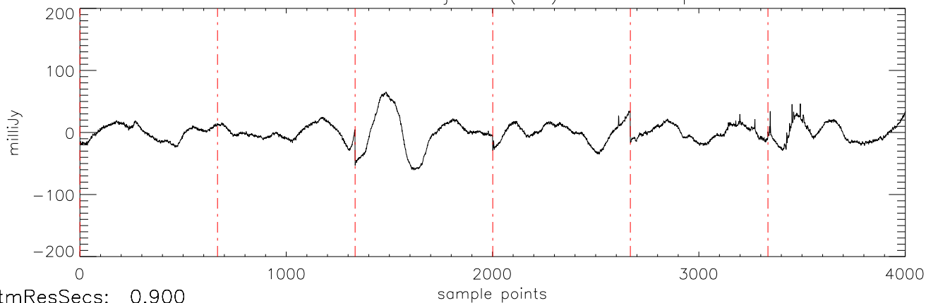
a2471 HD102195 07jan10 (AST) StokesI freq:4466.
