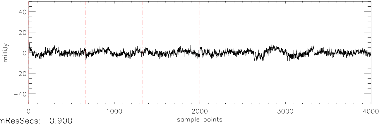
a2471 HD102195 07jan10 (AST) StokesQ freq:5034.
