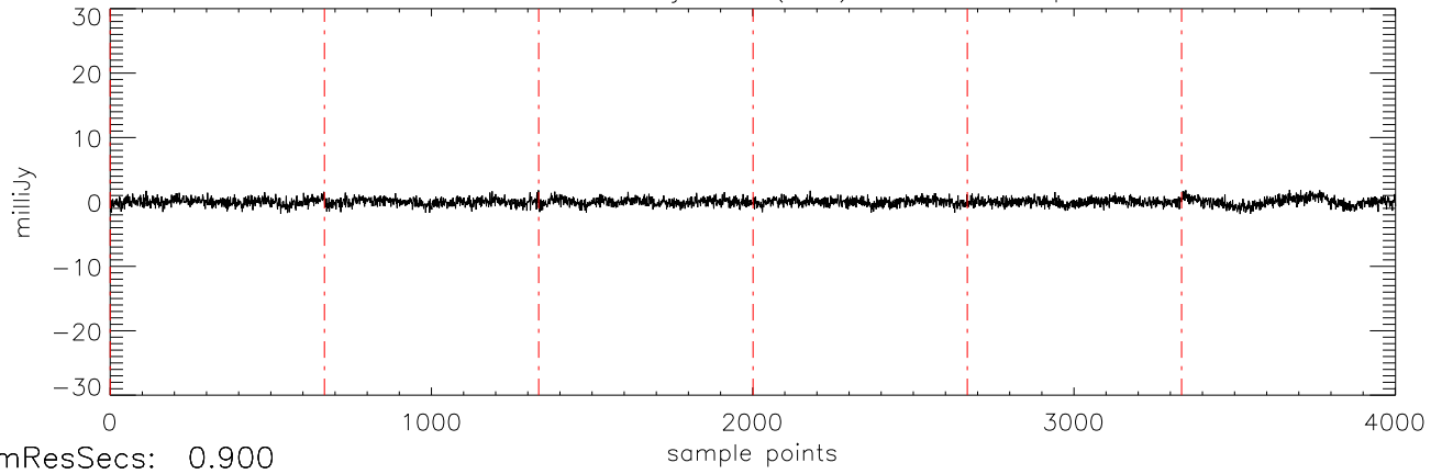
a2471 HD102195 07jan10 (AST) StokesV freq:5034.
