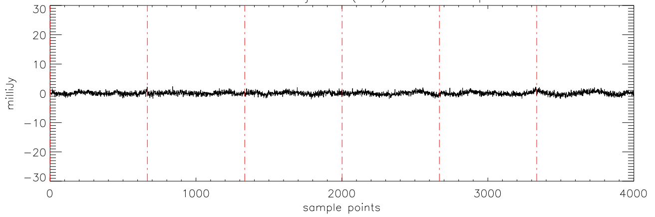
a2471 HD102195 07jan10 (AST) StokesV freq:5176.
