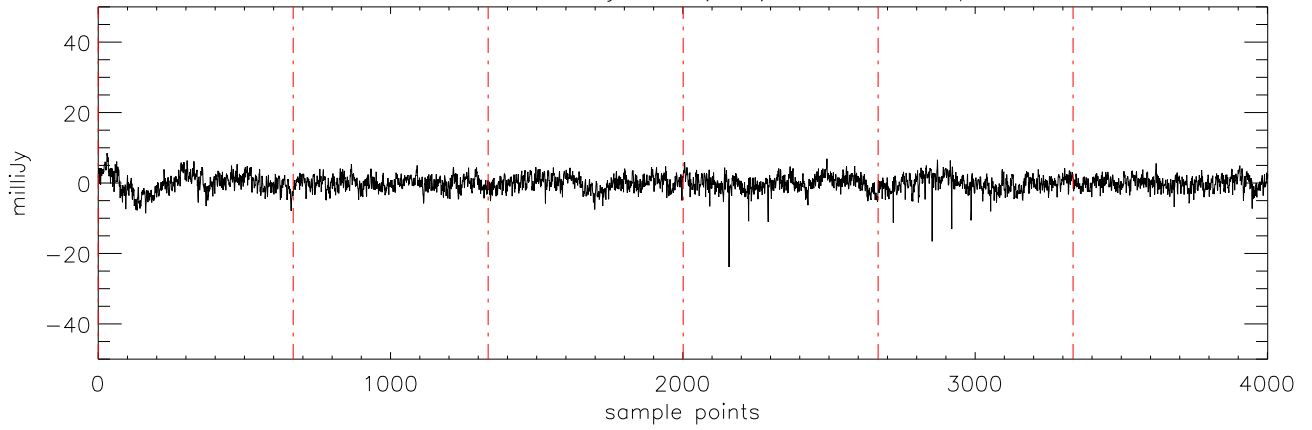
a2471 HD102195 07jan10 (AST) StokesQ freq:5176.
