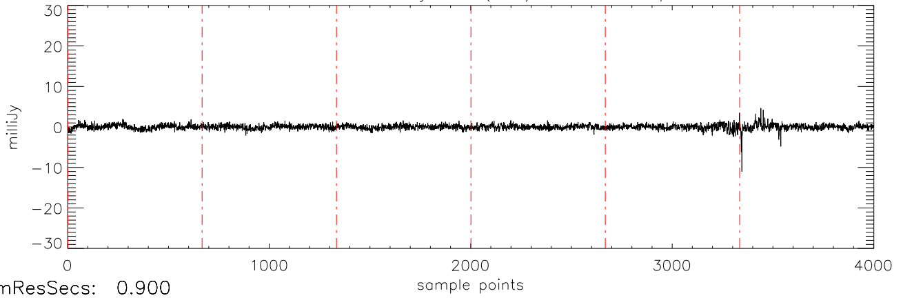
a2471 HD102195 07jan10 (AST) StokesV freq:4466.
