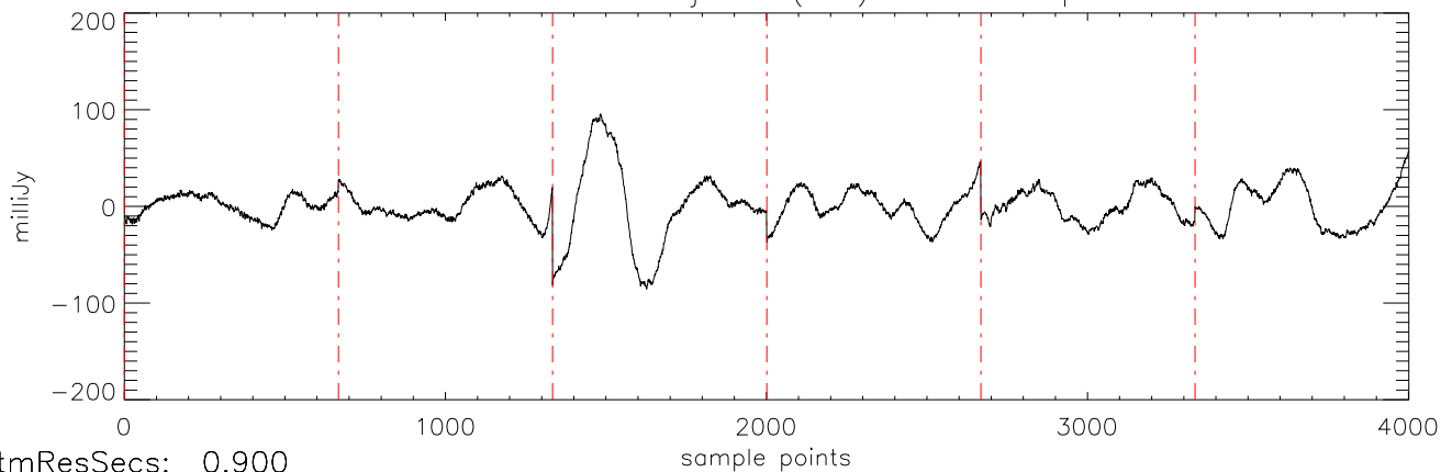
a2471 HD102195 07jan10 (AST) StokesI freq:5034.
