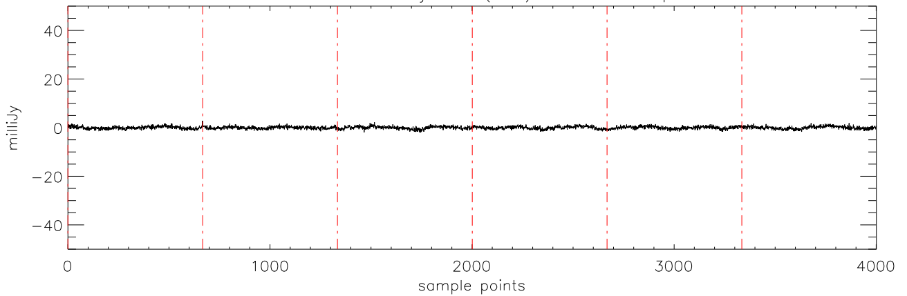
a2471 HD102195 07jan10 (AST) StokesU freq:4750.
