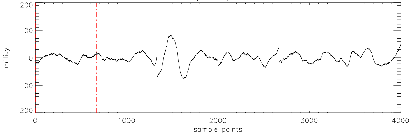
a2471 HD102195 07jan10 (AST) StokesI freq:4750.
