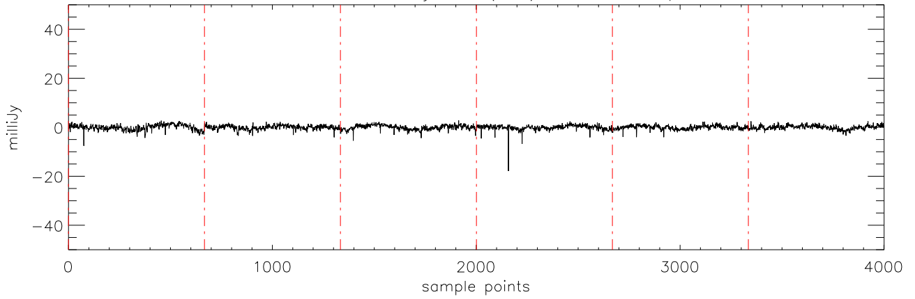
a2471 HD102195 07jan10 (AST) StokesU freq:5176.
