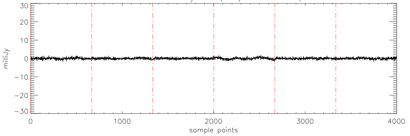
a2471 HD102195 07jan10 (AST) StokesV freq:4608.
