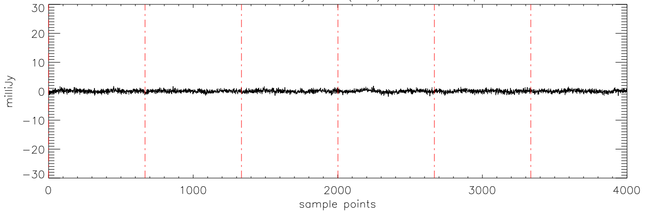
a2471 HD102195 07jan10 (AST) StokesV freq:4750.
