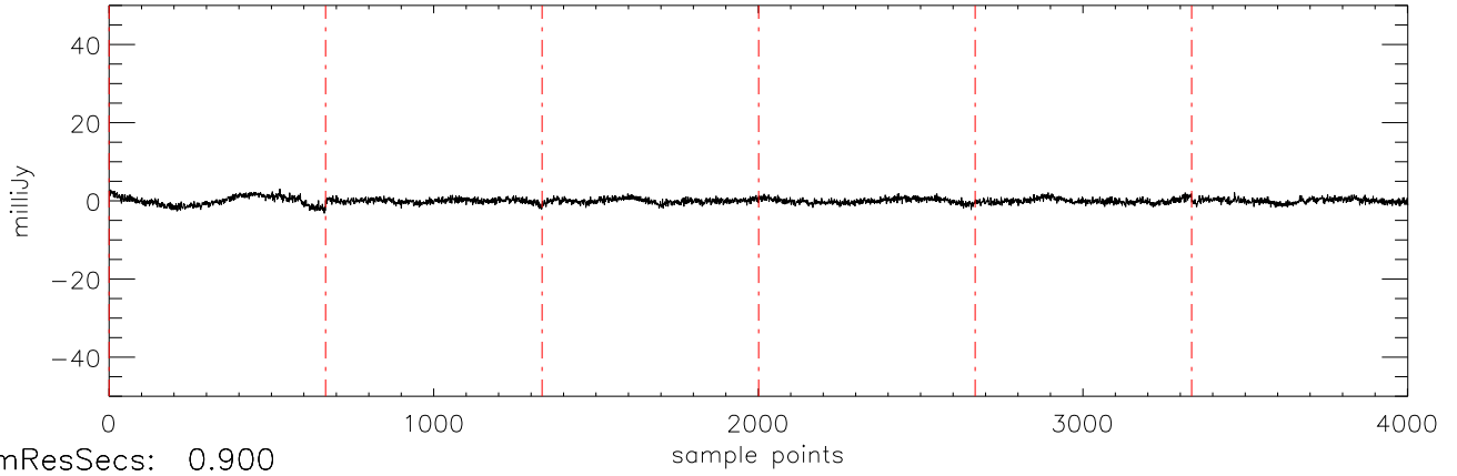
a2471 HD102195 07jan10 (AST) StokesU freq:5034.
