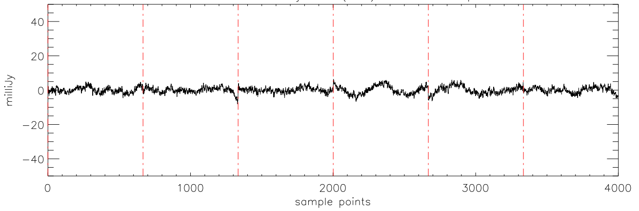
a2471 HD102195 07jan10 (AST) StokesQ freq:4608.
