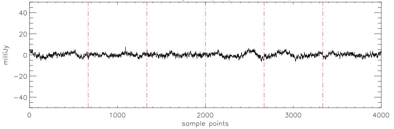
a2471 HD102195 07jan10 (AST) StokesQ freq:4750.
