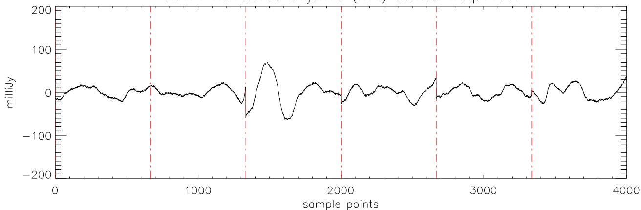
a2471 HD102195 07jan10 (AST) StokesI freq:4608.
