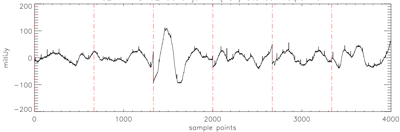
a2471 HD102195 07jan10 (AST) StokesI freq:5176.
