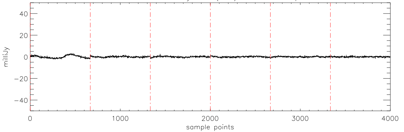
a2471 HD102195 07jan10 (AST) StokesU freq:4608.
