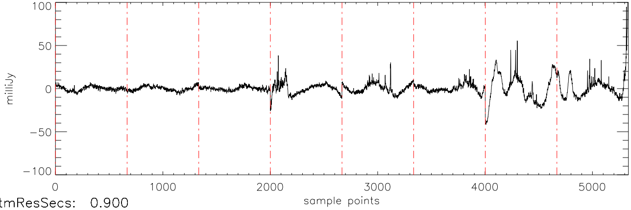
a2471 55Cnc 02jan11 (AST) StokesI freq:4466.
