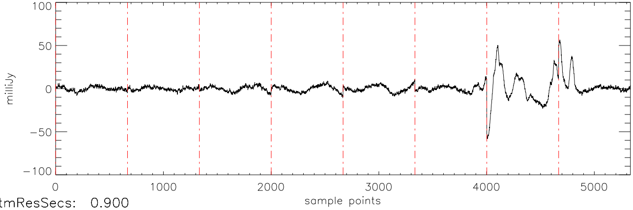
a2471 55Cnc 02jan11 (AST) StokesI freq:5034.
