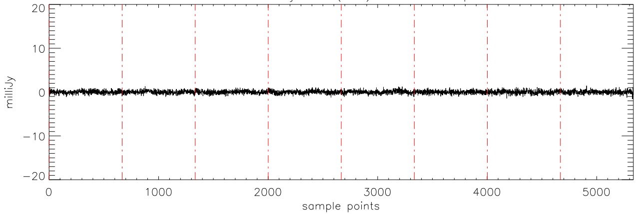
a2471 55Cnc 02jan11 (AST) StokesV freq:4608.
