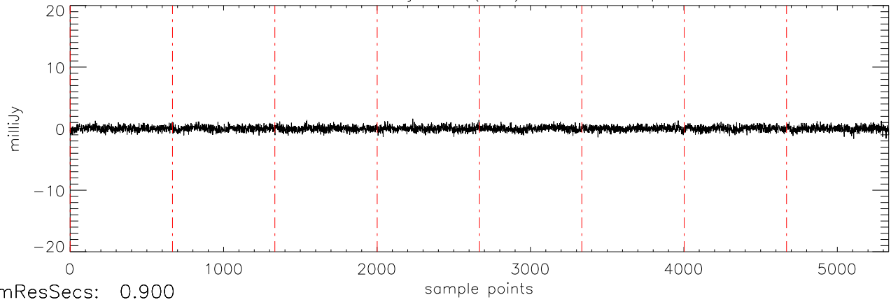
a2471 55Cnc 02jan11 (AST) StokesV freq:5034.
