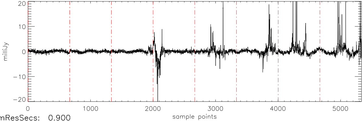
a2471 55Cnc 02jan11 (AST) StokesU freq:4466.
