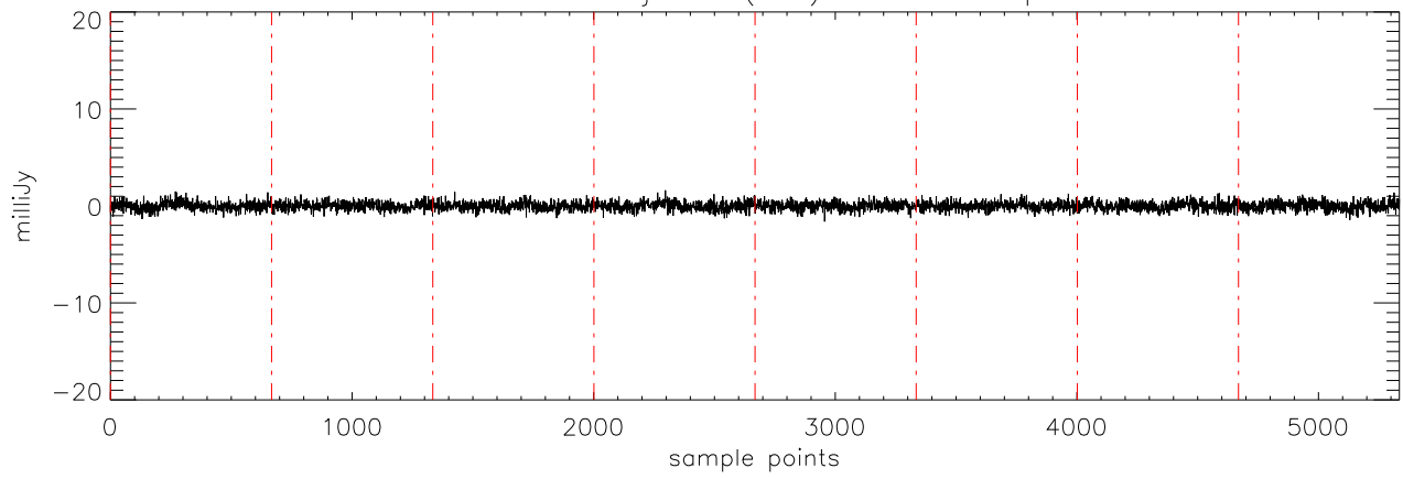
a2471 55Cnc 02jan11 (AST) StokesV freq:5176.
