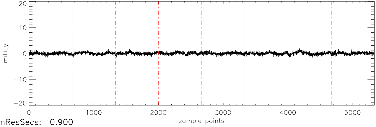
a2471 55Cnc 02jan11 (AST) StokesU freq:5034.
