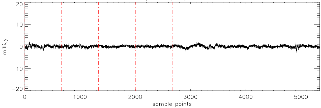
a2471 55Cnc 02jan11 (AST) StokesU freq:4750.
