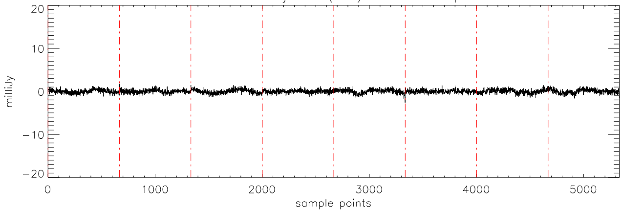
a2471 55Cnc 02jan11 (AST) StokesU freq:4608.
