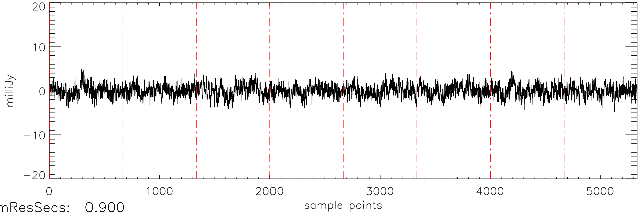
a2471 55Cnc 02jan11 (AST) StokesQ freq:5034.
