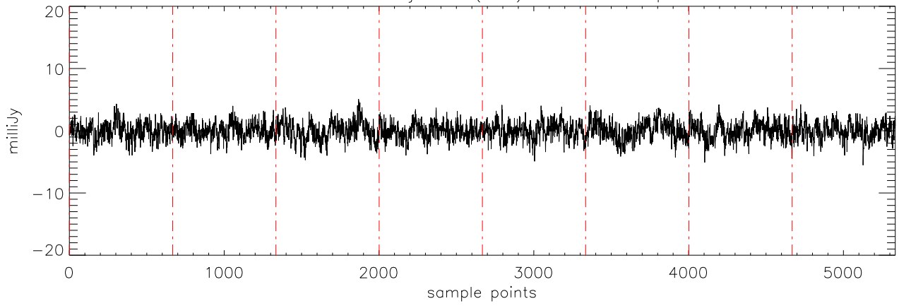
a2471 55Cnc 02jan11 (AST) StokesQ freq:5176.
