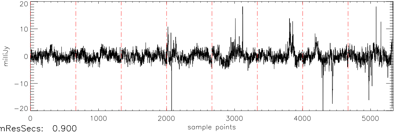
a2471 55Cnc 02jan11 (AST) StokesQ freq:4466.
