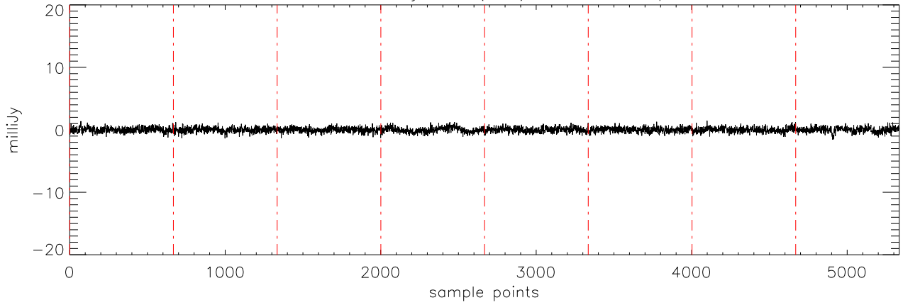
a2471 55Cnc 02jan11 (AST) StokesV freq:4750.
