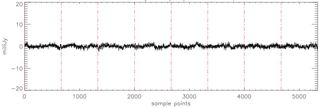
a2471 55Cnc 02jan11 (AST) StokesU freq:5176.
