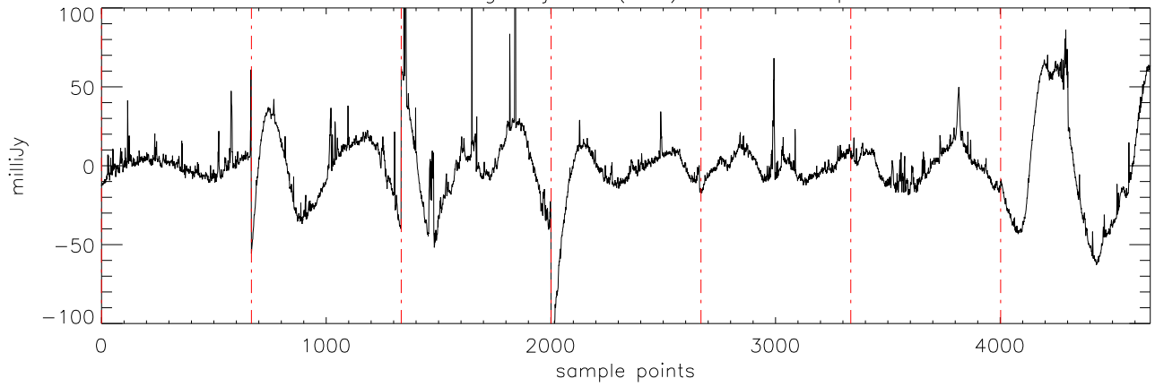
a2471 51Peg 19jul11 (AST) StokesI freq:4750.
