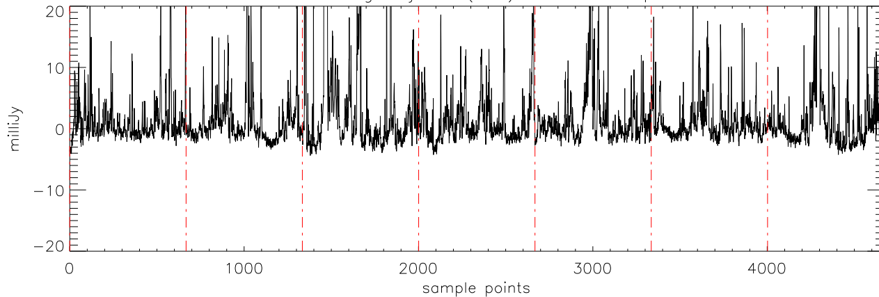
a2471 51Peg 19jul11 (AST) StokesV freq:4750.
