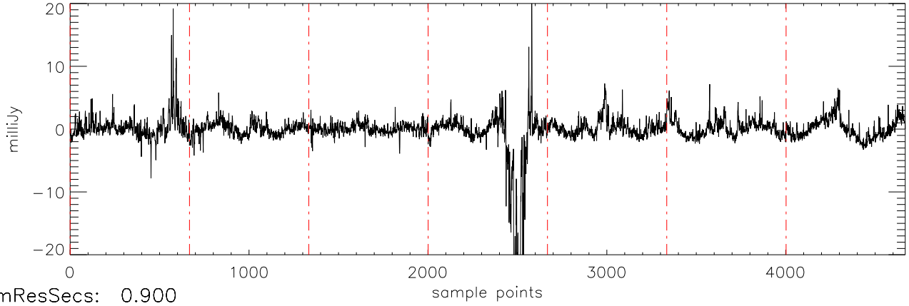
a2471 51Peg 19jul11 (AST) StokesU freq:4466.
