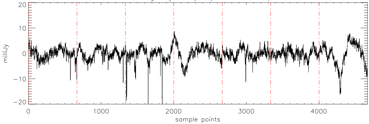
a2471 51Peg 19jul11 (AST) StokesQ freq:4608.
