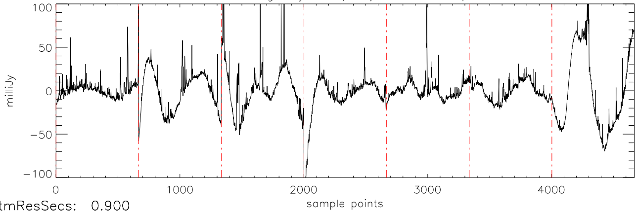
a2471 51Peg 19jul11 (AST) StokesI freq:5034.
