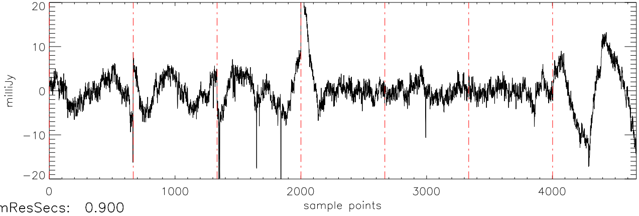
a2471 51Peg 19jul11 (AST) StokesQ freq:5034.
