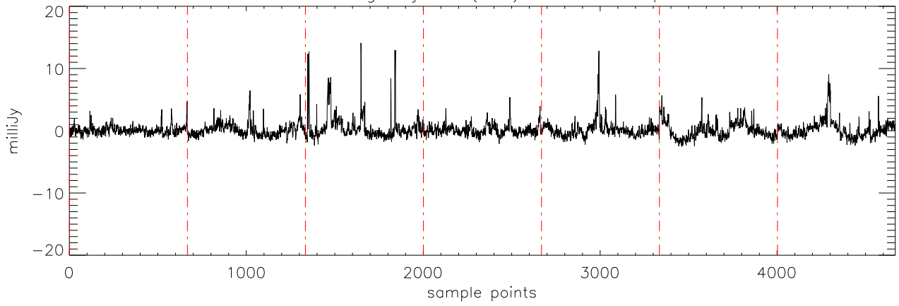
a2471 51Peg 19jul11 (AST) StokesU freq:4608.
