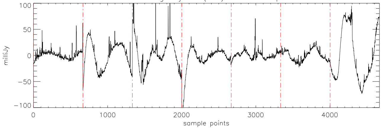
a2471 51Peg 19jul11 (AST) StokesI freq:4608.
