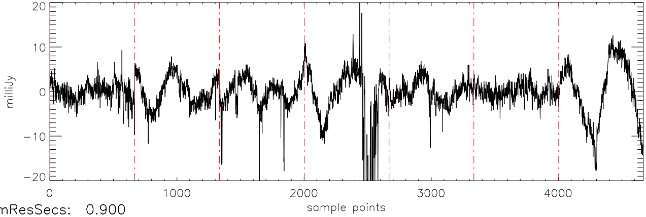
a2471 51Peg 19jul11 (AST) StokesQ freq:4466.
