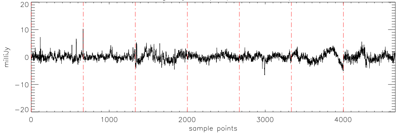
a2471 51Peg 19jul11 (AST) StokesU freq:5176.
