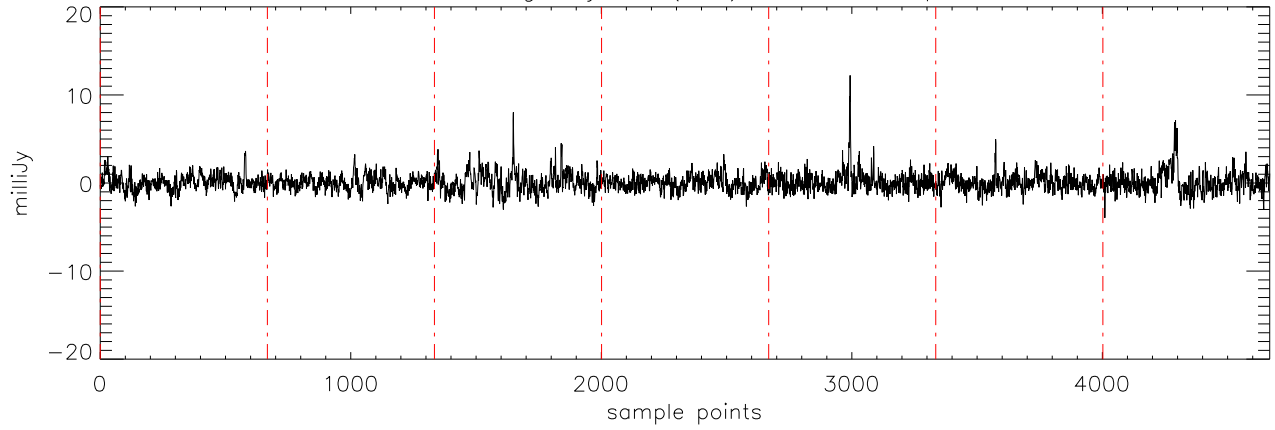
a2471 51Peg 19jul11 (AST) StokesV freq:5176.
