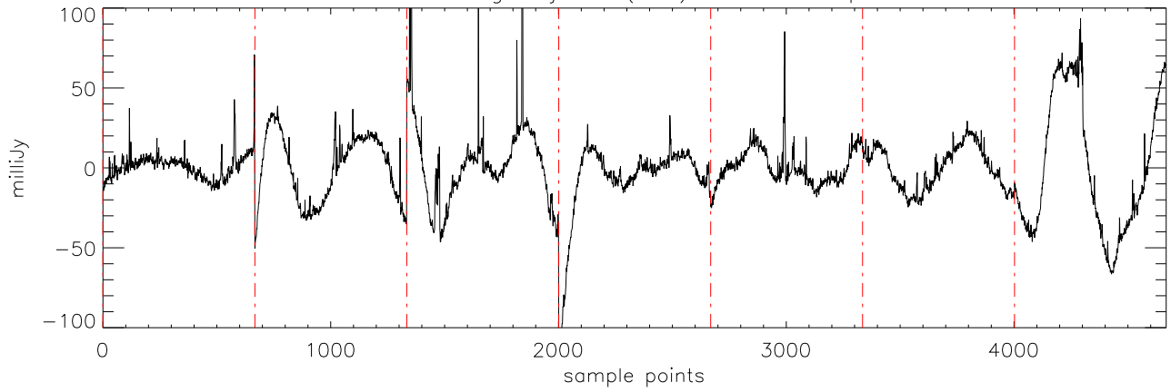
a2471 51Peg 19jul11 (AST) StokesI freq:5176.
