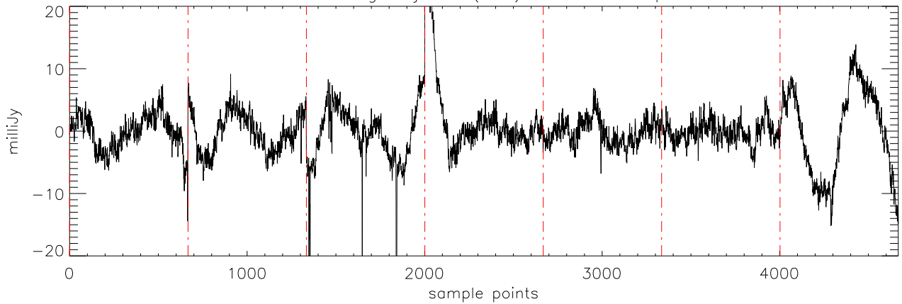
a2471 51Peg 19jul11 (AST) StokesQ freq:4750.
