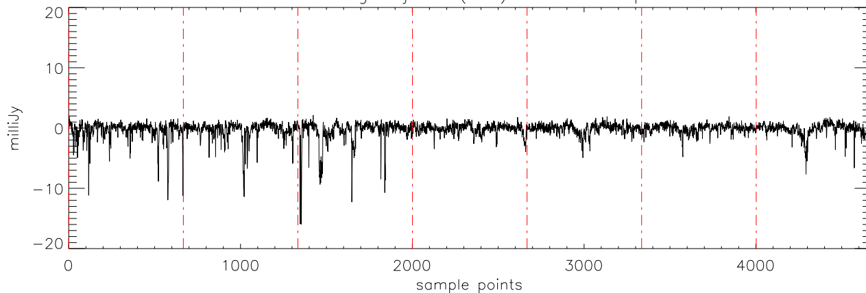
a2471 51Peg 19jul11 (AST) StokesV freq:4608.
