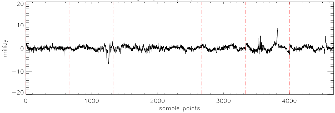
a2471 51Peg 19jul11 (AST) StokesU freq:4750.
