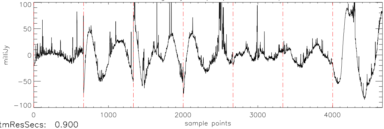
a2471 51Peg 19jul11 (AST) StokesI freq:4466.
