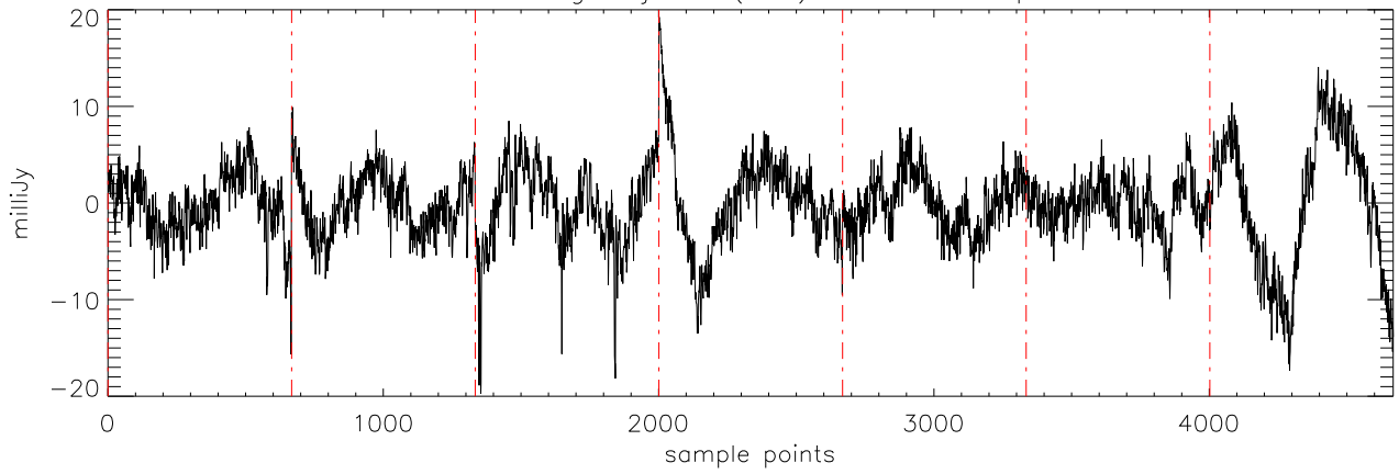
a2471 51Peg 19jul11 (AST) StokesQ freq:5176.
