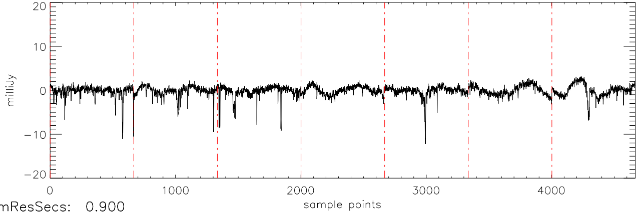
a2471 51Peg 19jul11 (AST) StokesU freq:5034.
