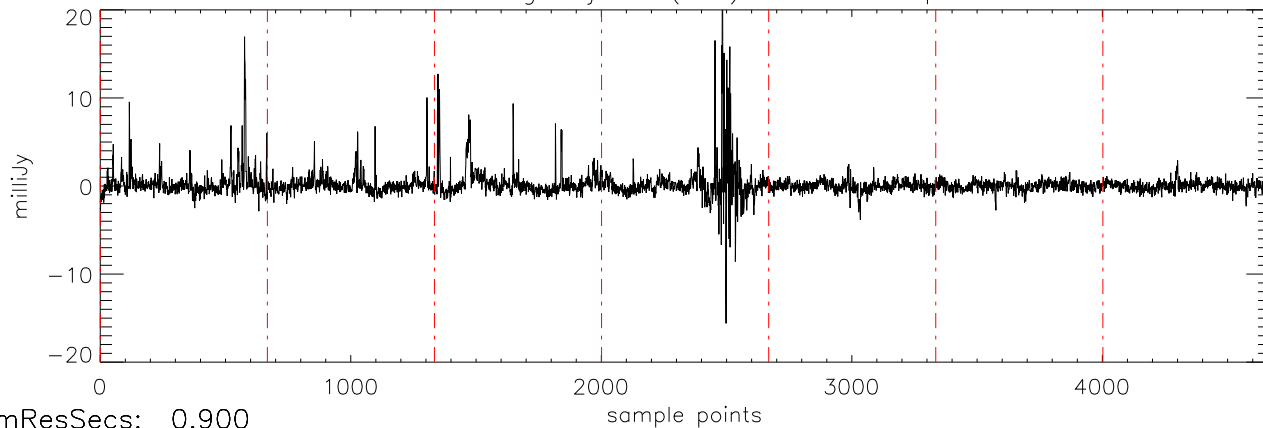
a2471 51Peg 19jul11 (AST) StokesV freq:4466.
