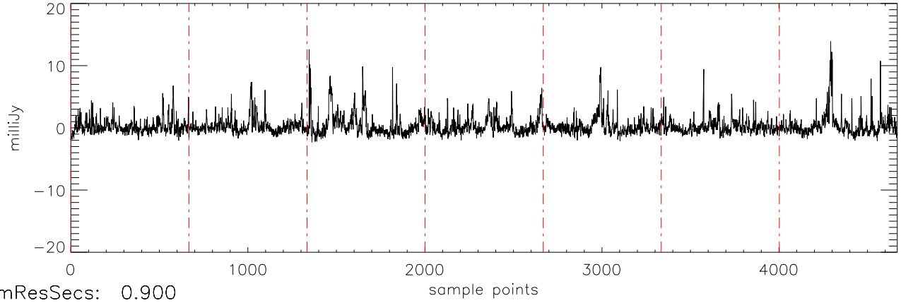
a2471 51Peg 19jul11 (AST) StokesV freq:5034.
