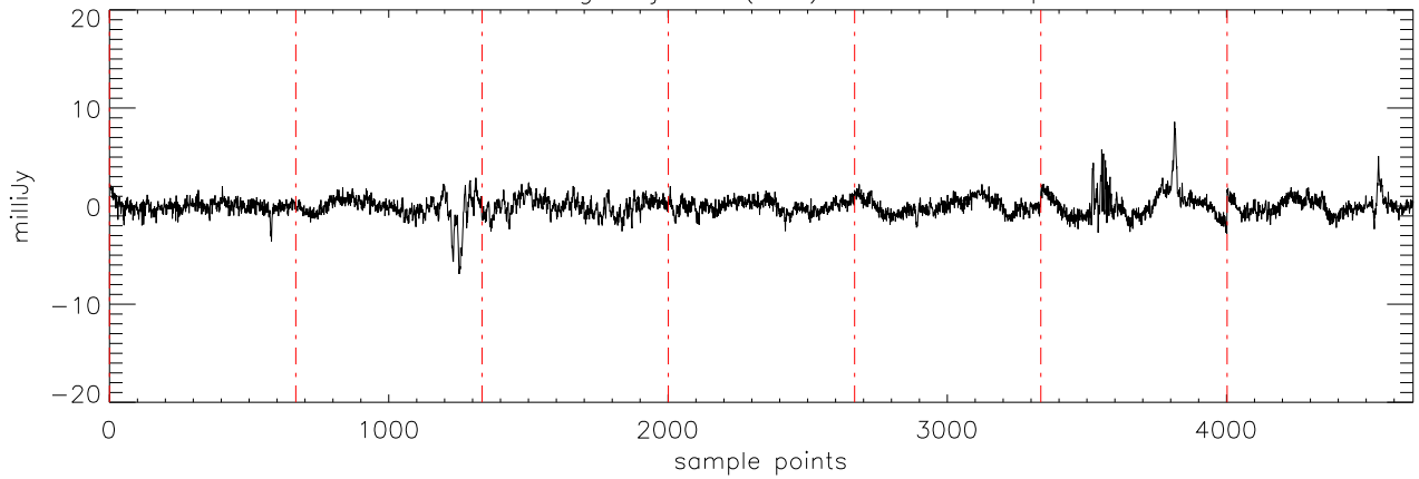
a2471 51Peg 18jul11 (AST) StokesU freq:4750.
