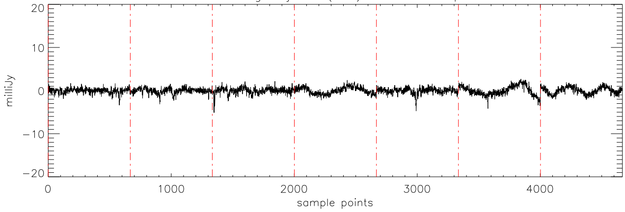
a2471 51Peg 18jul11 (AST) StokesU freq:5176.
