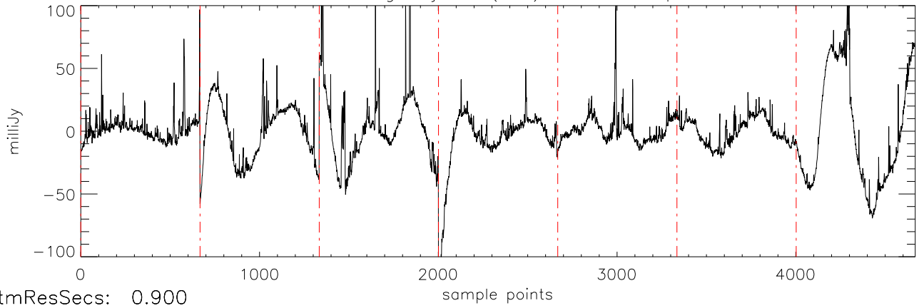
a2471 51Peg 18jul11 (AST) StokesI freq:5034.
