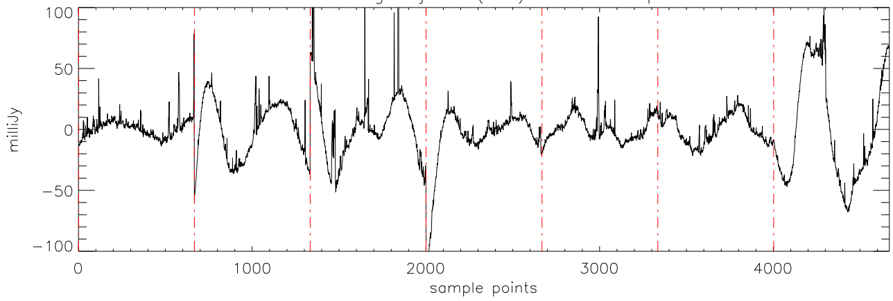
a2471 51Peg 18jul11 (AST) StokesI freq:5176.
