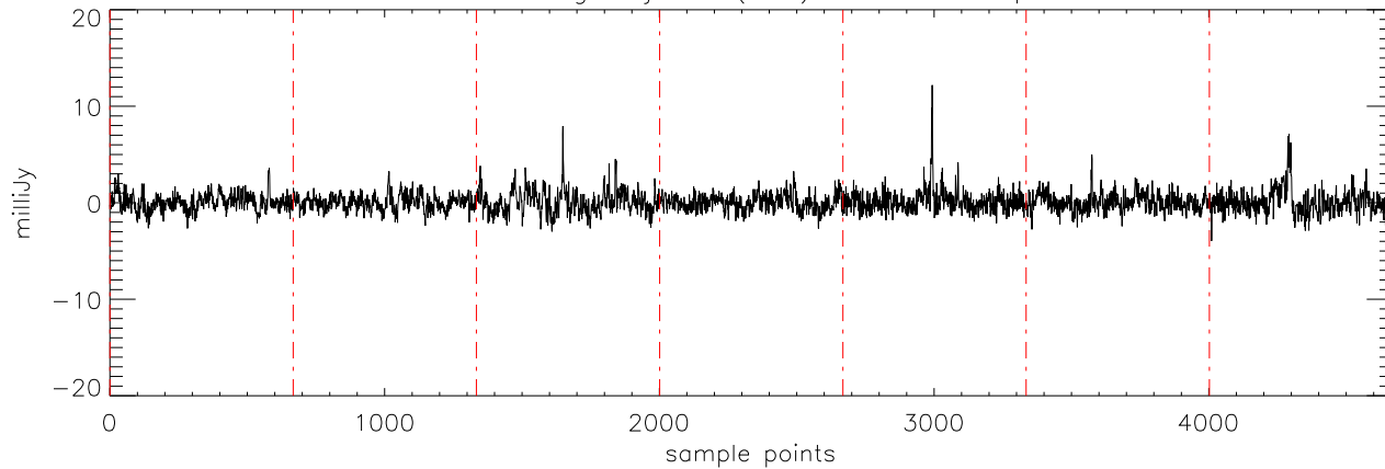
a2471 51Peg 18jul11 (AST) StokesV freq:5176.
