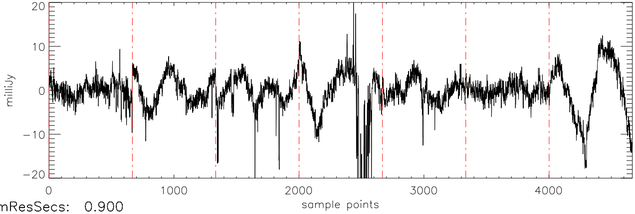
a2471 51Peg 18jul11 (AST) StokesQ freq:4466.
