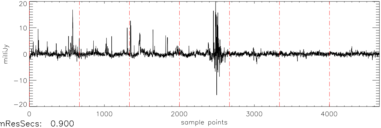
a2471 51Peg 18jul11 (AST) StokesV freq:4466.
