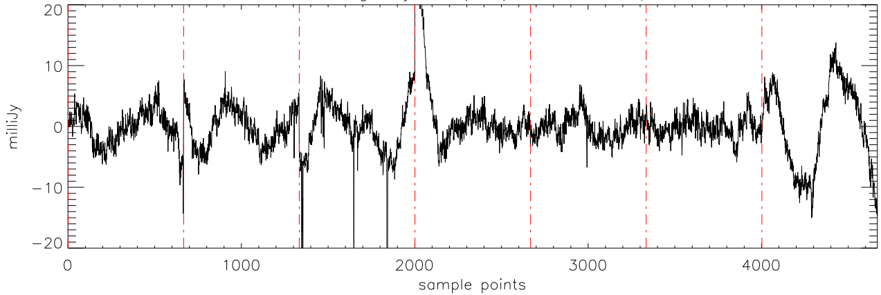
a2471 51Peg 18jul11 (AST) StokesQ freq:4750.
