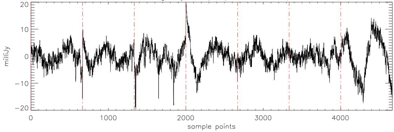
a2471 51Peg 18jul11 (AST) StokesQ freq:5176.
