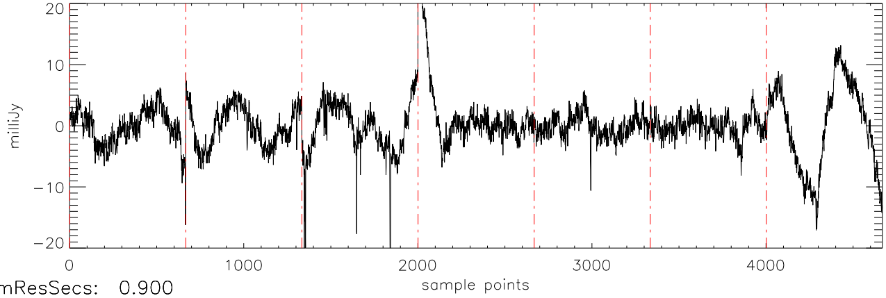
a2471 51Peg 18jul11 (AST) StokesQ freq:5034.
